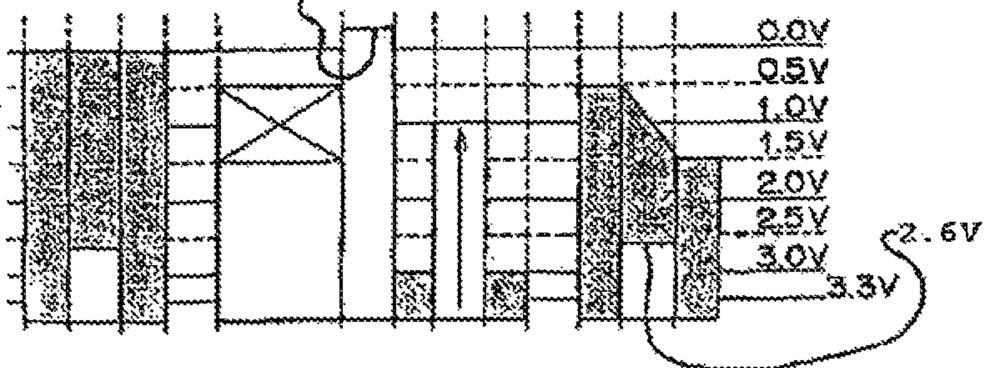
FIG. 13D t_3 < t < t_4 FD RESET
