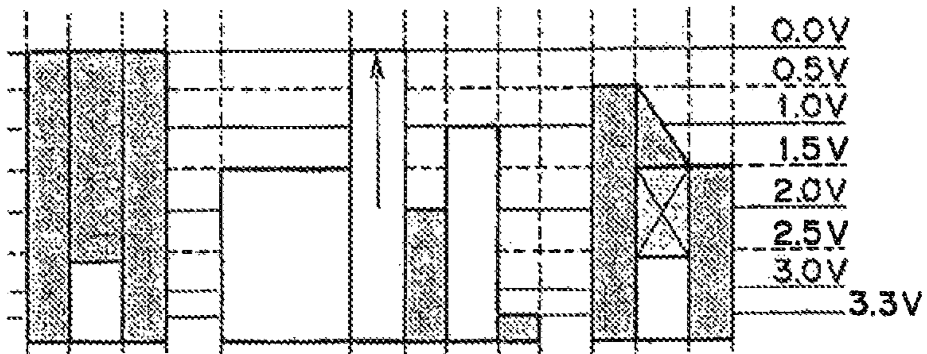
FIG. 14B t_5 < t < t_6 SIGNAL LEVEL READ-OUT
