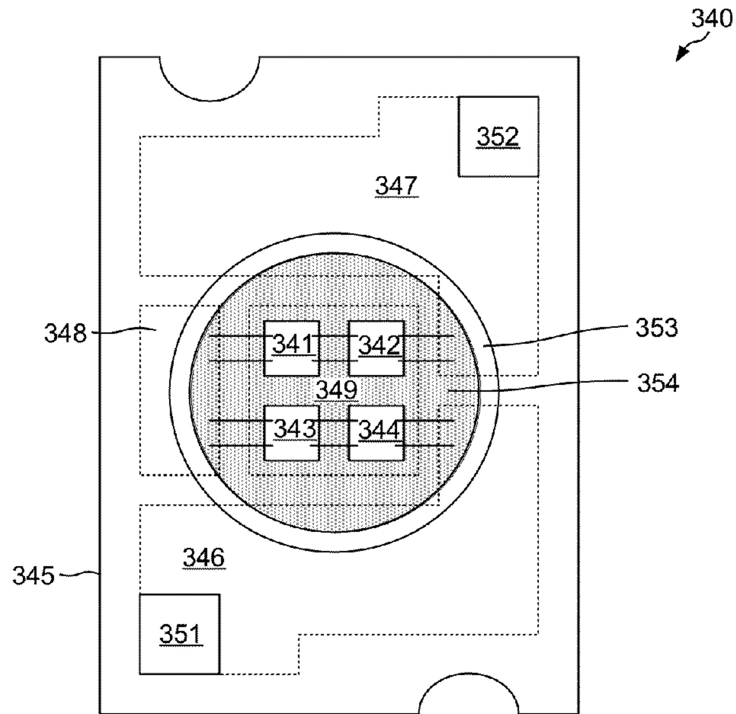
TOP-DOWN VIEW OF A WHITE LED ASSEMBLY FIG. 49
