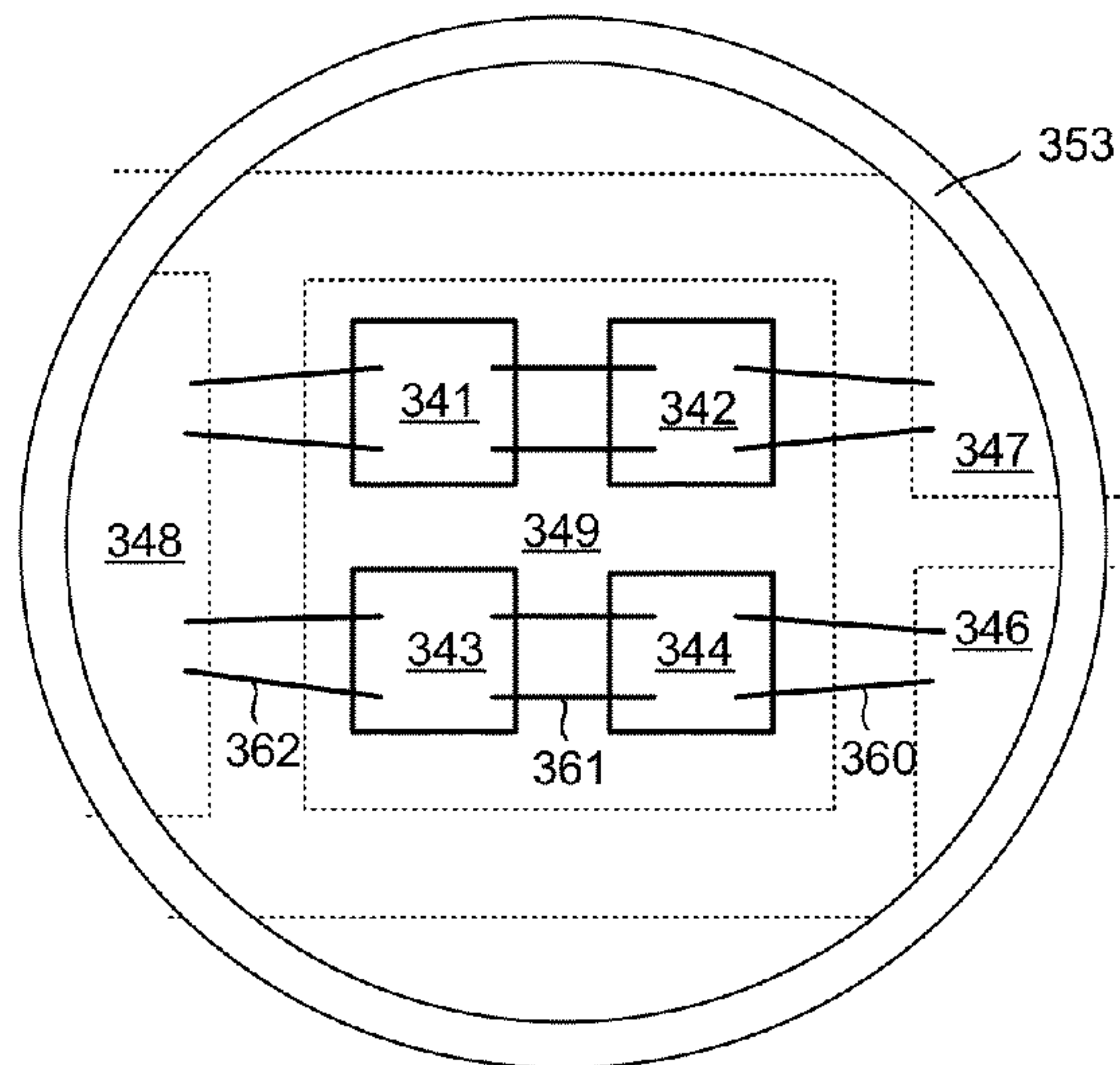
TOP-DOWN VIEW OF DIE PLACEMENT AREA AFTER FORMATION OF THE RETAINING RING FIG. 55
