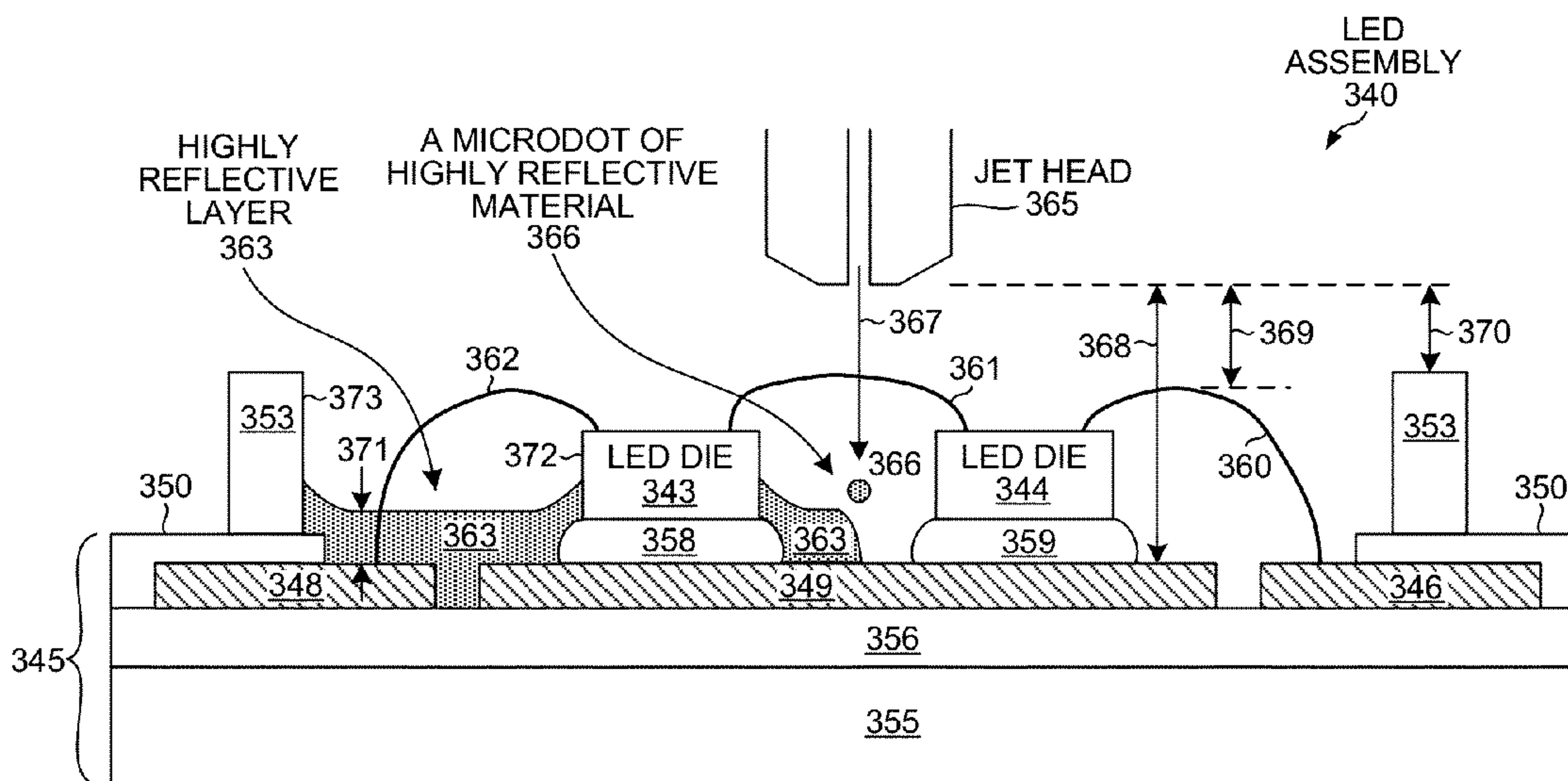
JETTING MICRODOTS OF HR MATERIAL FIG. 56
