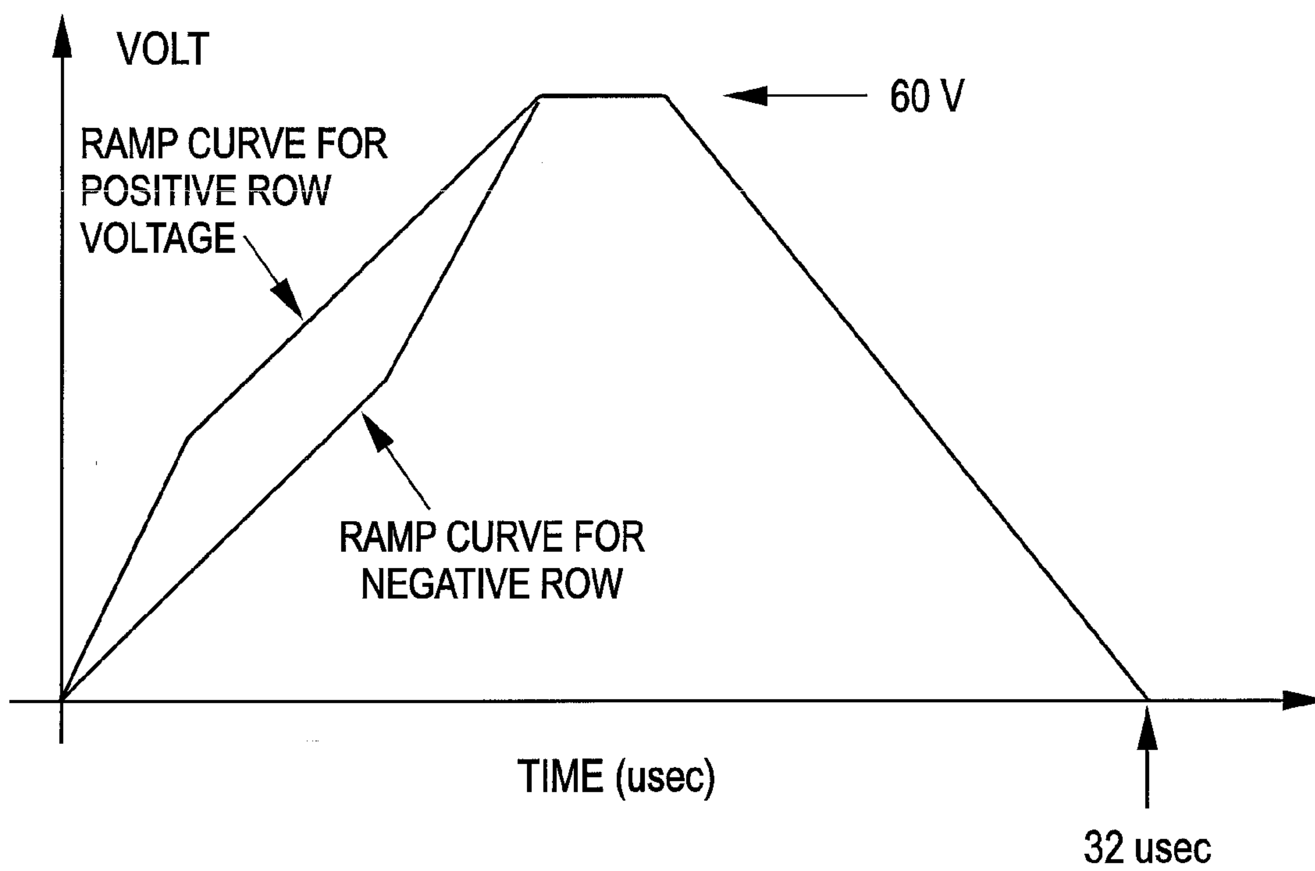
STEPWISE LINEAR APPROXIMATION OF GAMMA CORRECTION CURVE
