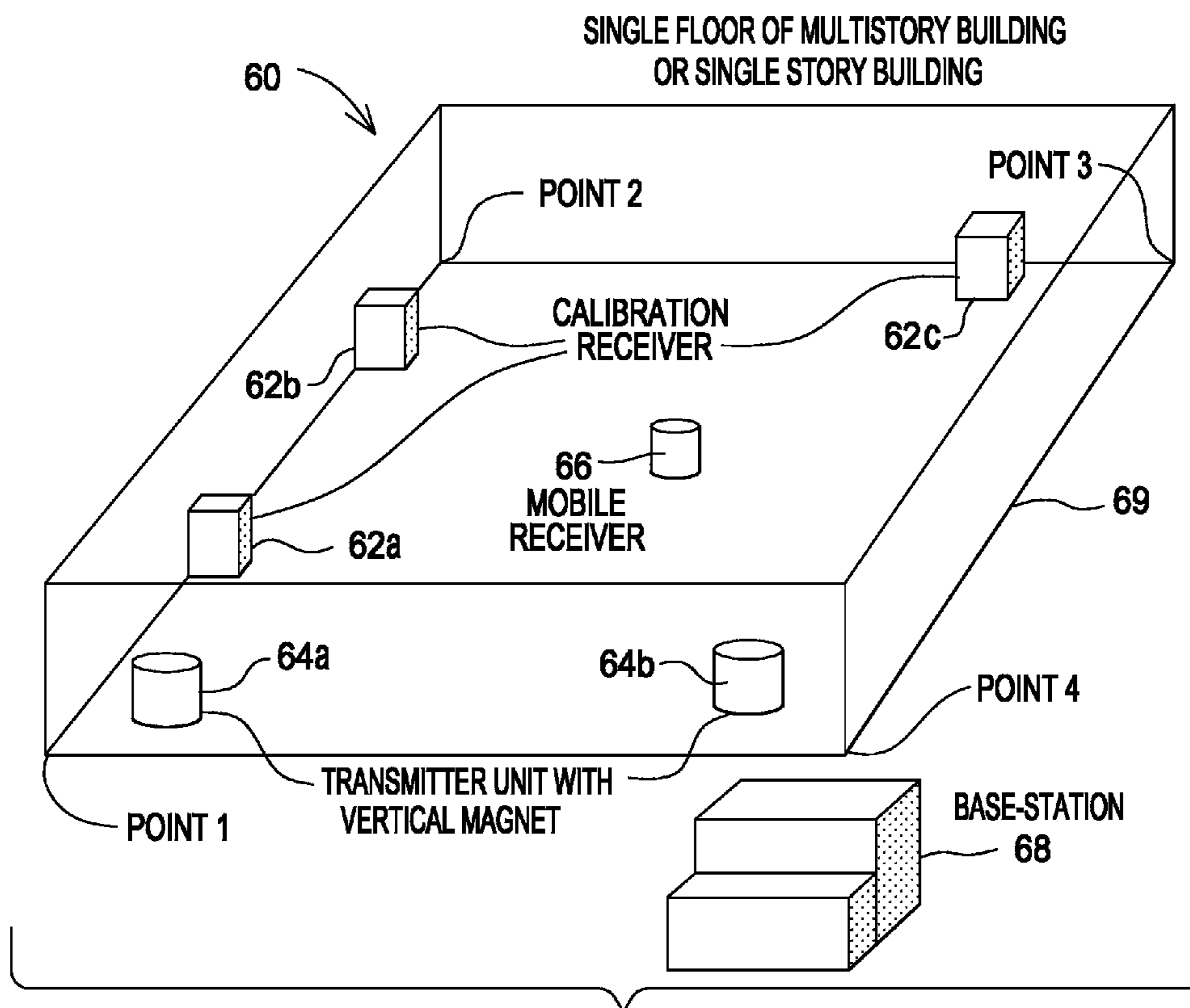
FIG.3 PERSONNEL TRACKING SYSTEM
