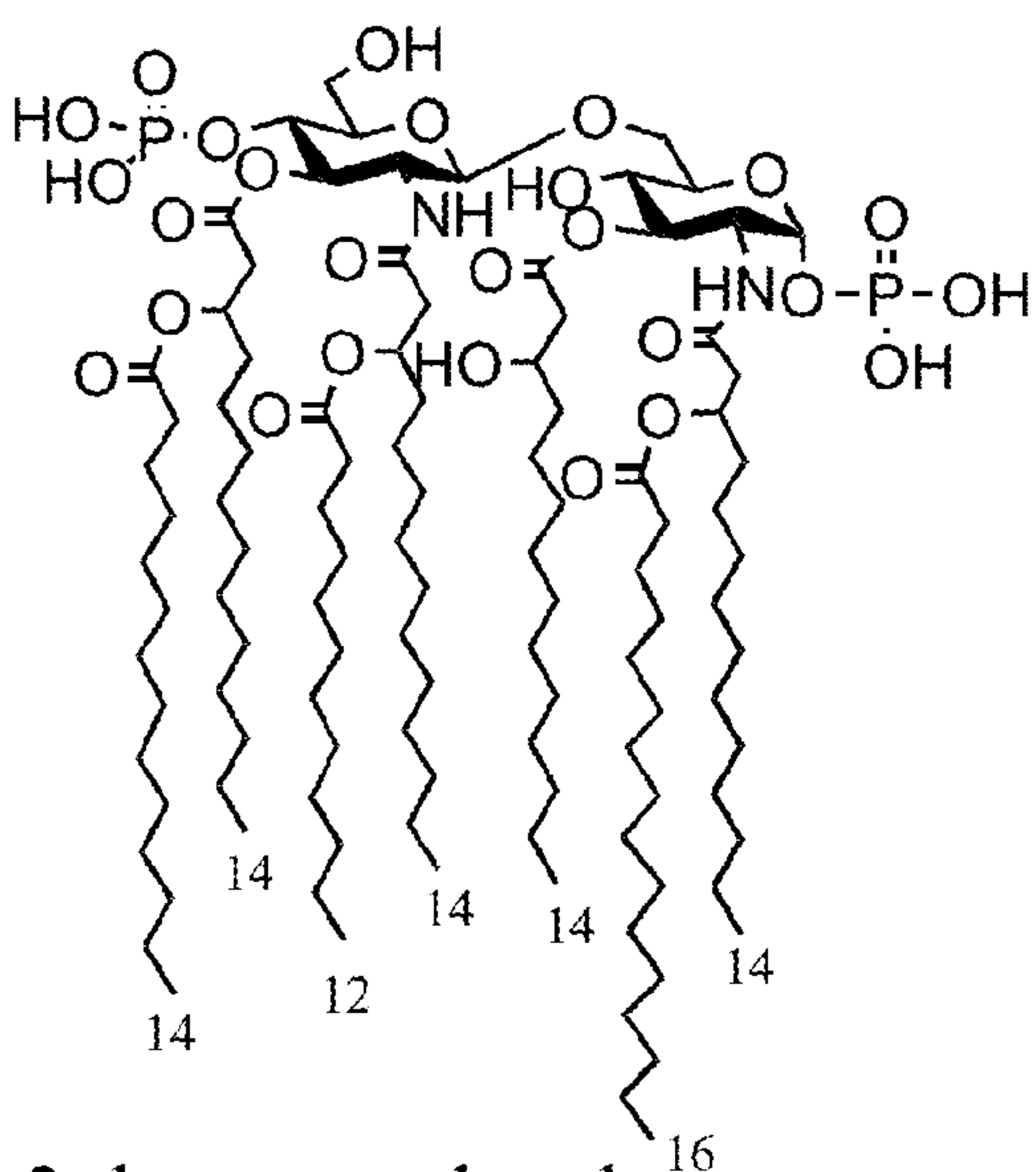
3. hepta-acylated S. typhimurium lipid A
