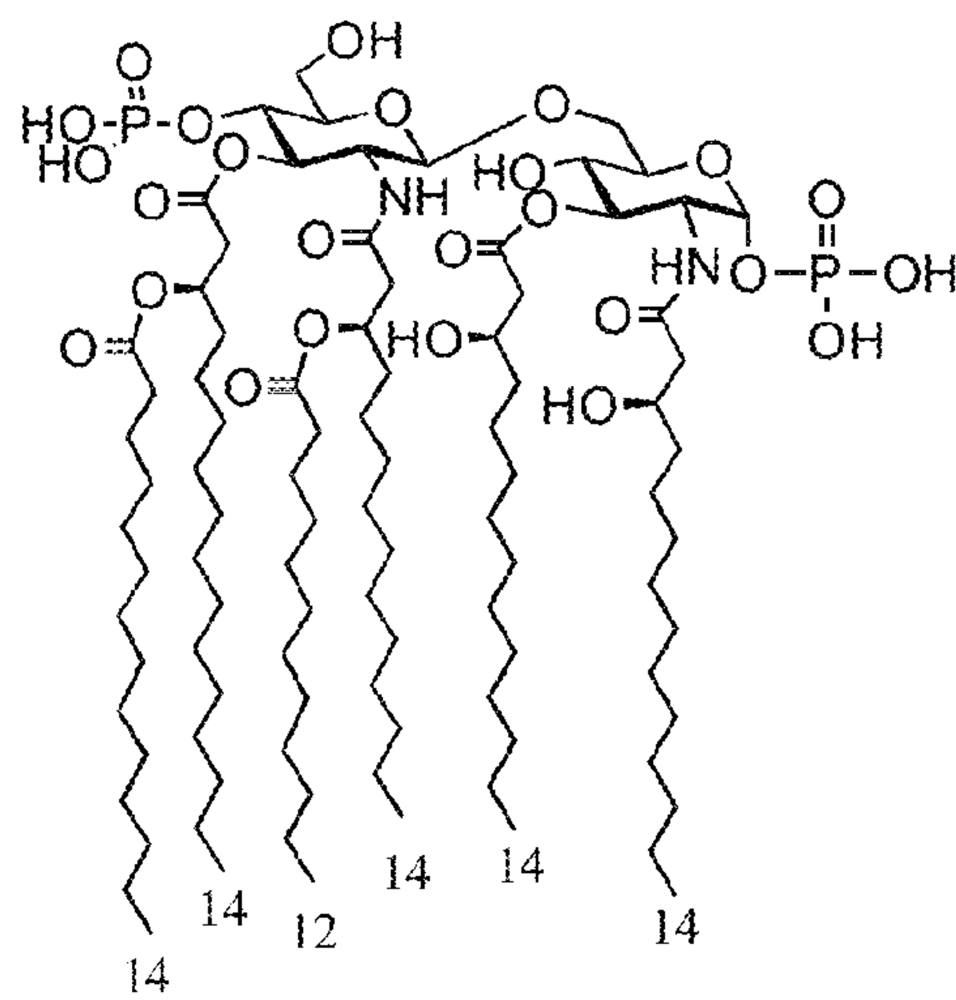
52. hexa-acylated E. coli lipid A
