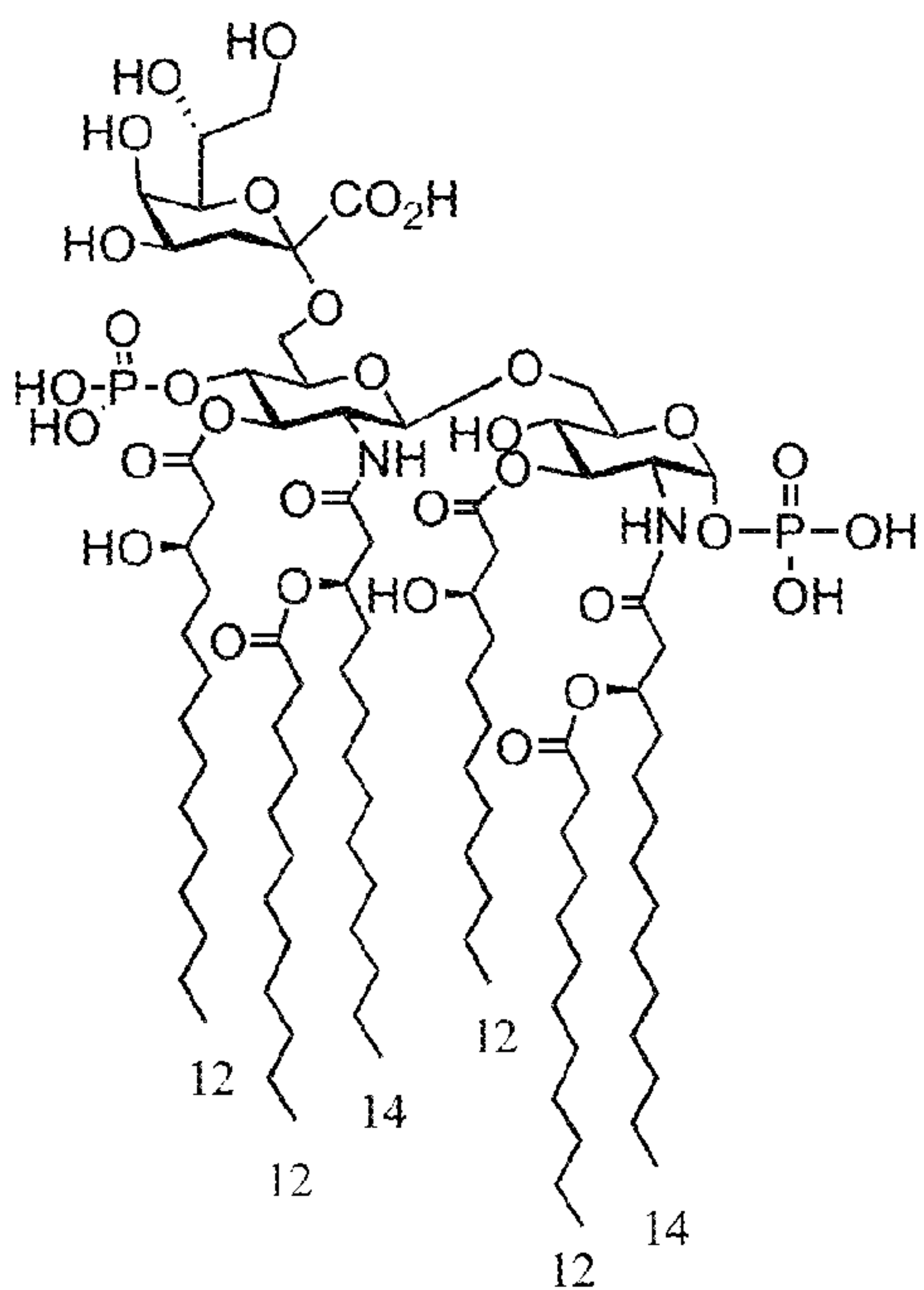
53. N. meningitidis lipid A with KDO
