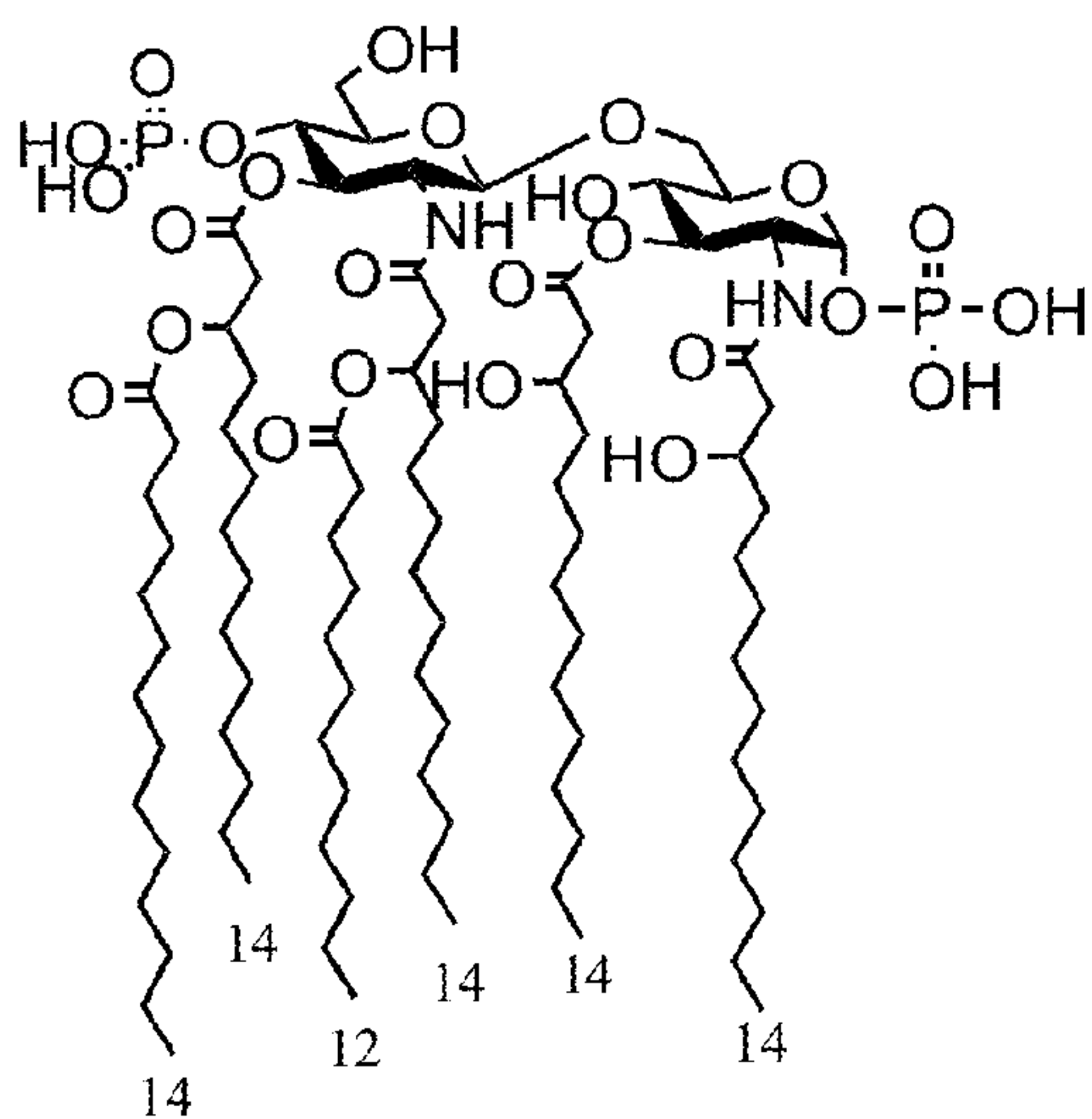
1. hexa-acylated E. coli lipid A
