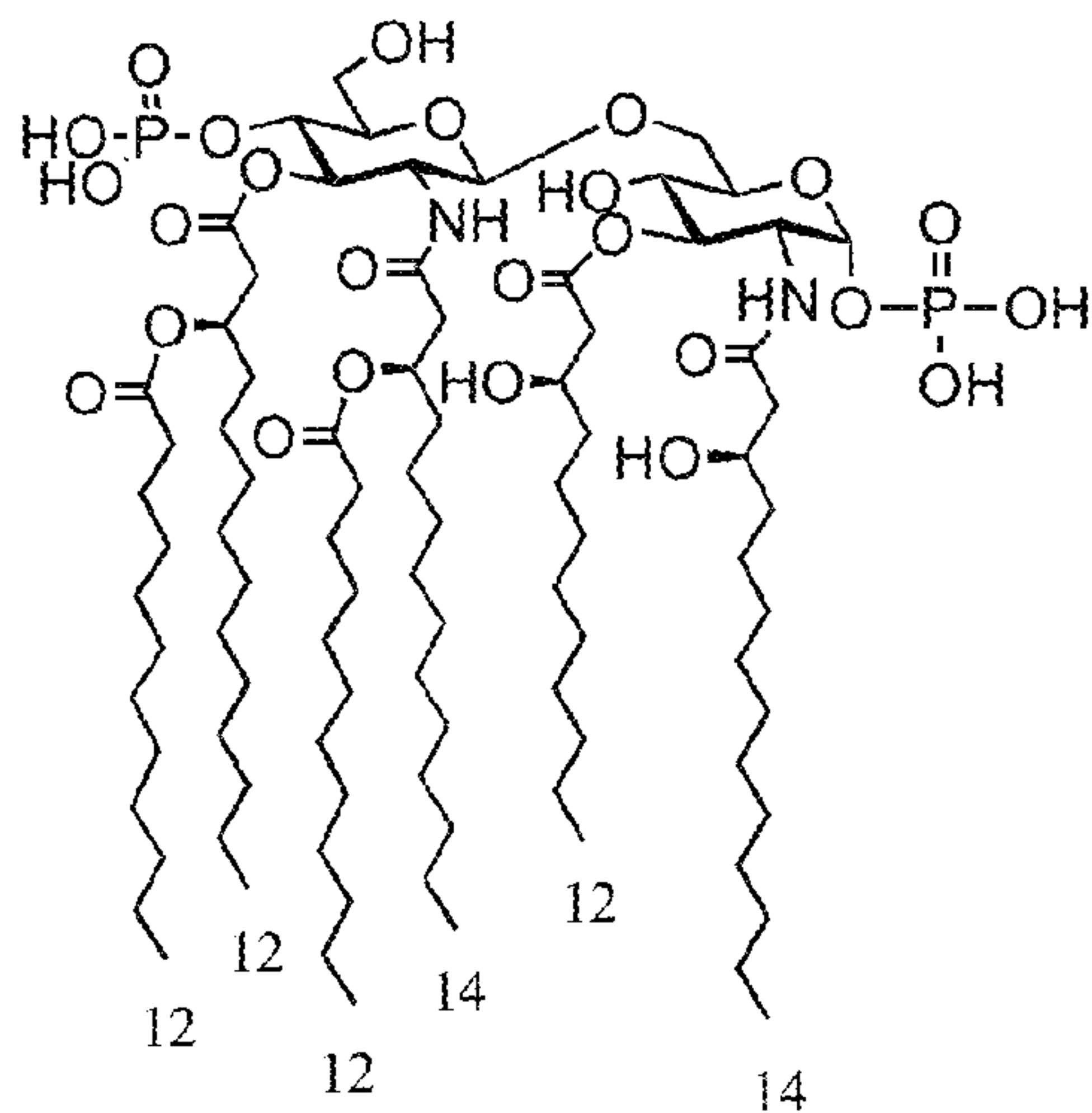
54. E. coli lipid A with shorter lipids
