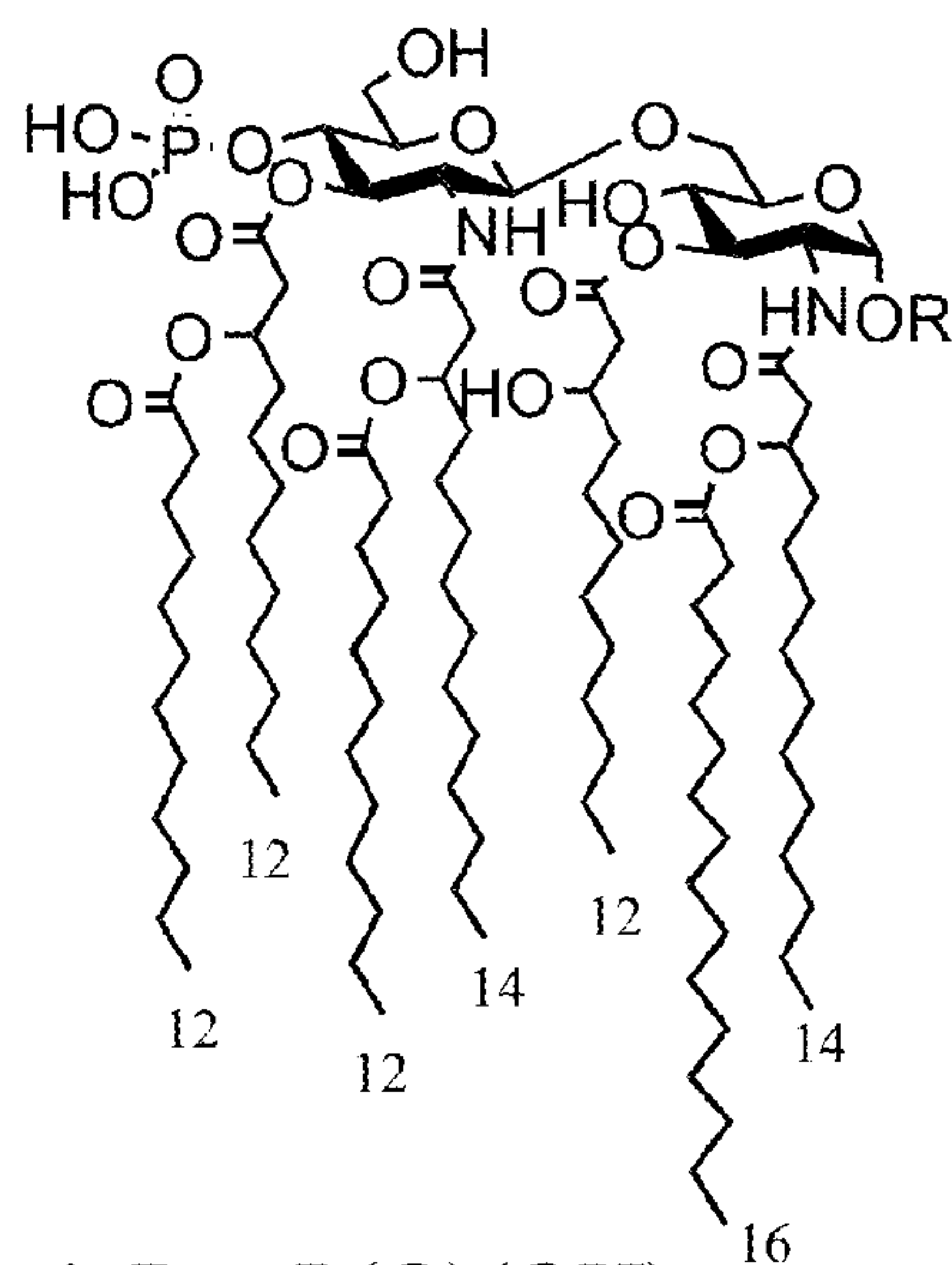
4. R = P(O)(OH) 2 S. typhimurium lipid A w/ shorter lipids
