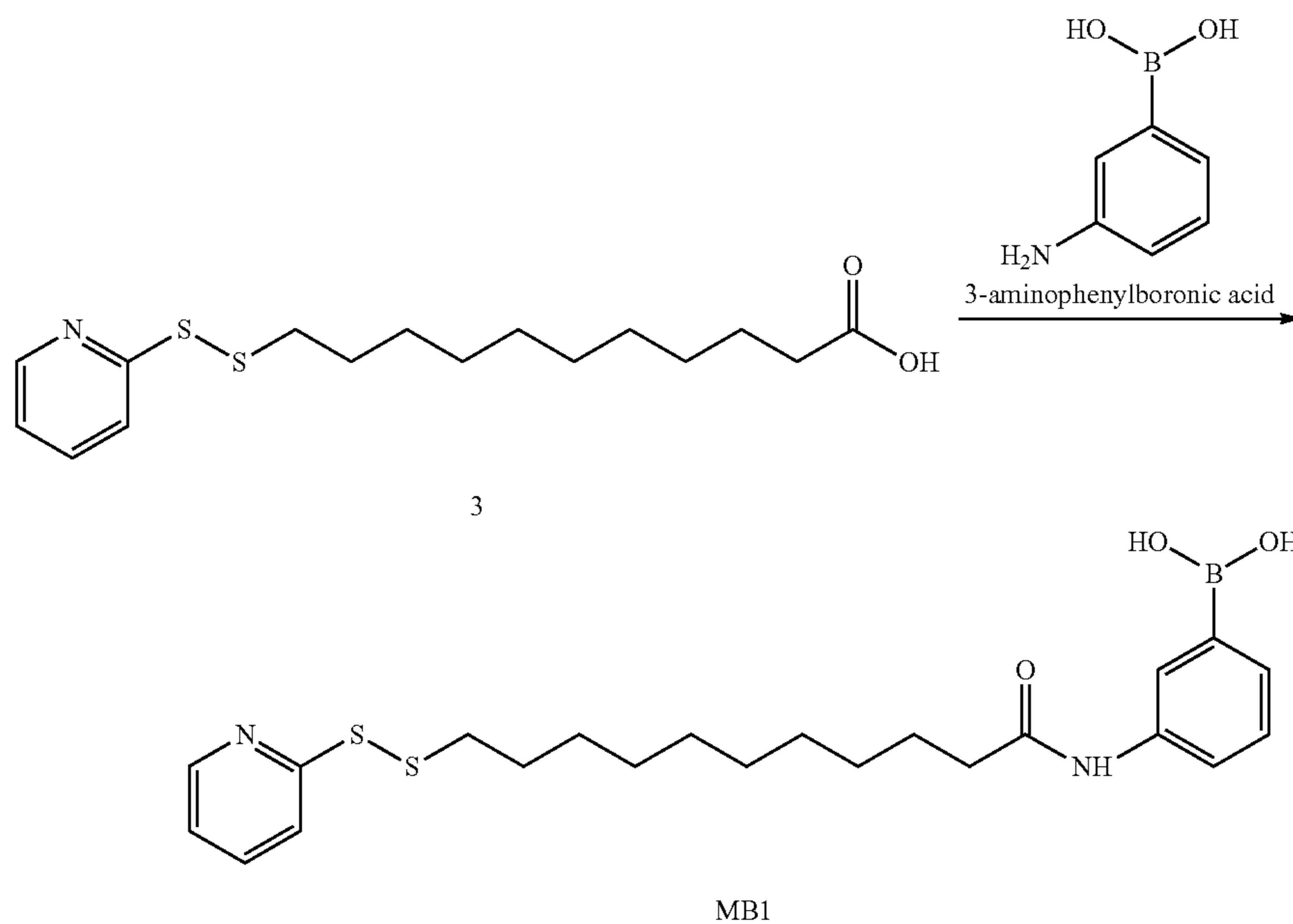
Scheme 3
