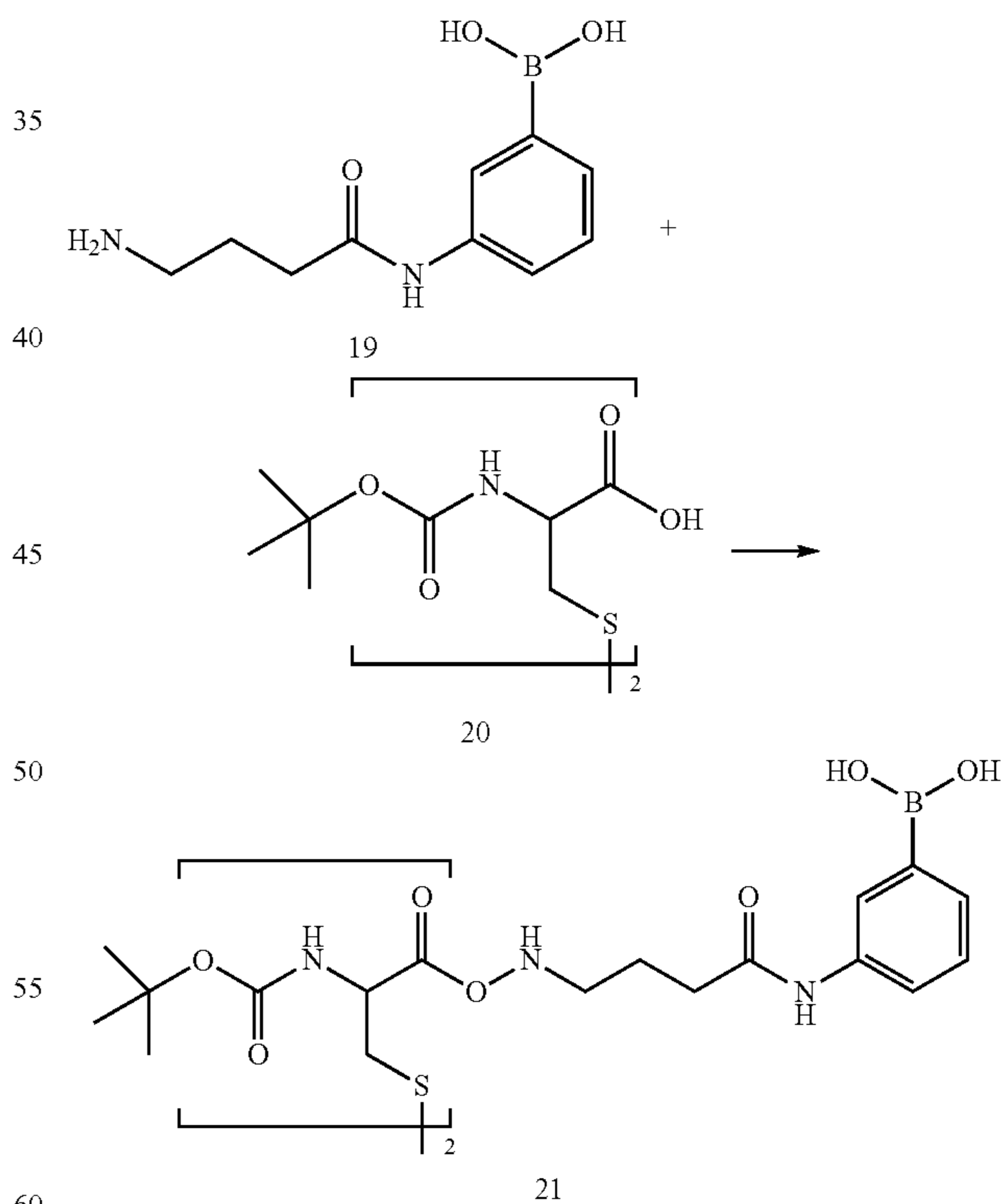
Scheme 18
