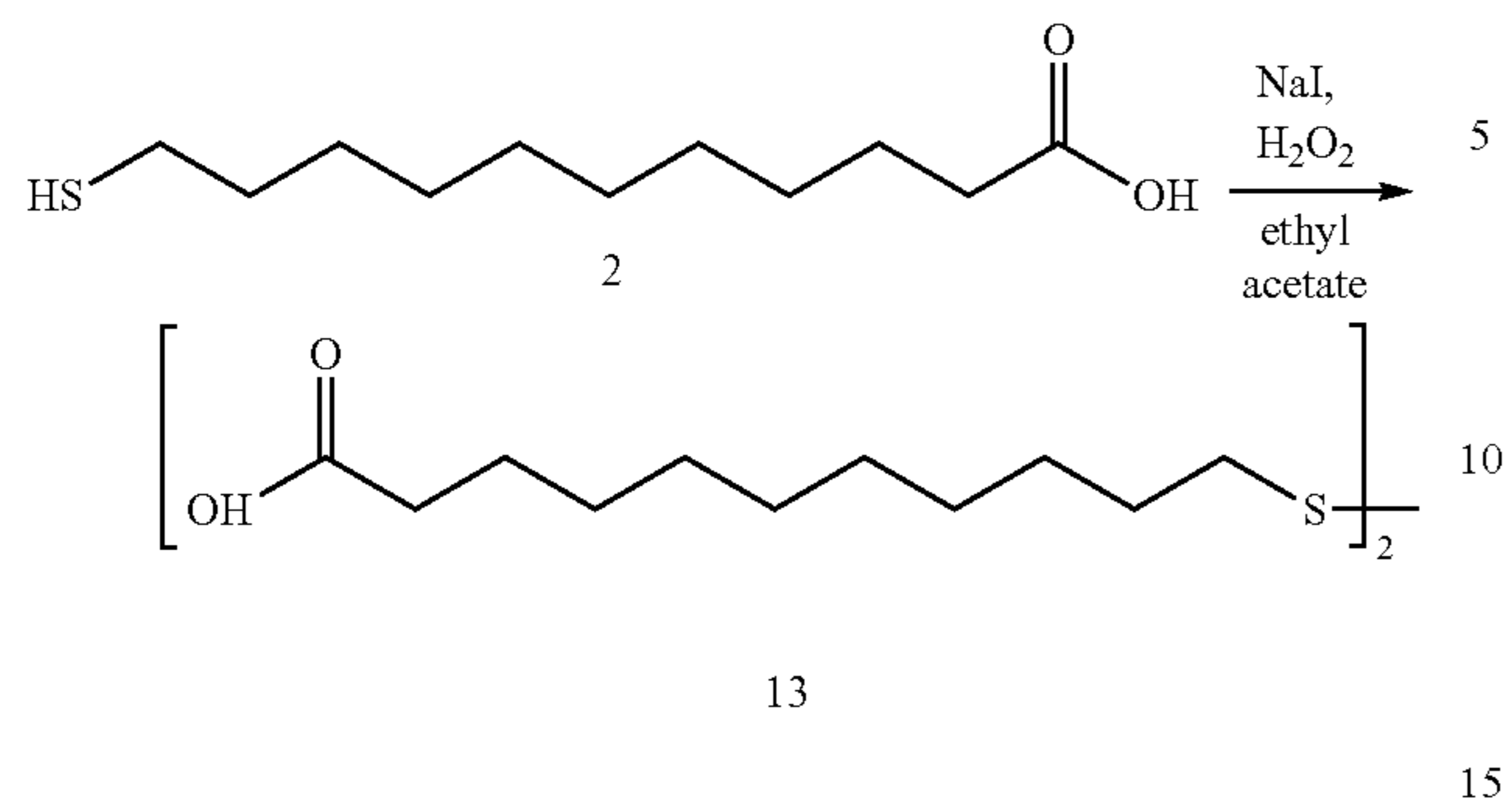
Scheme 12
