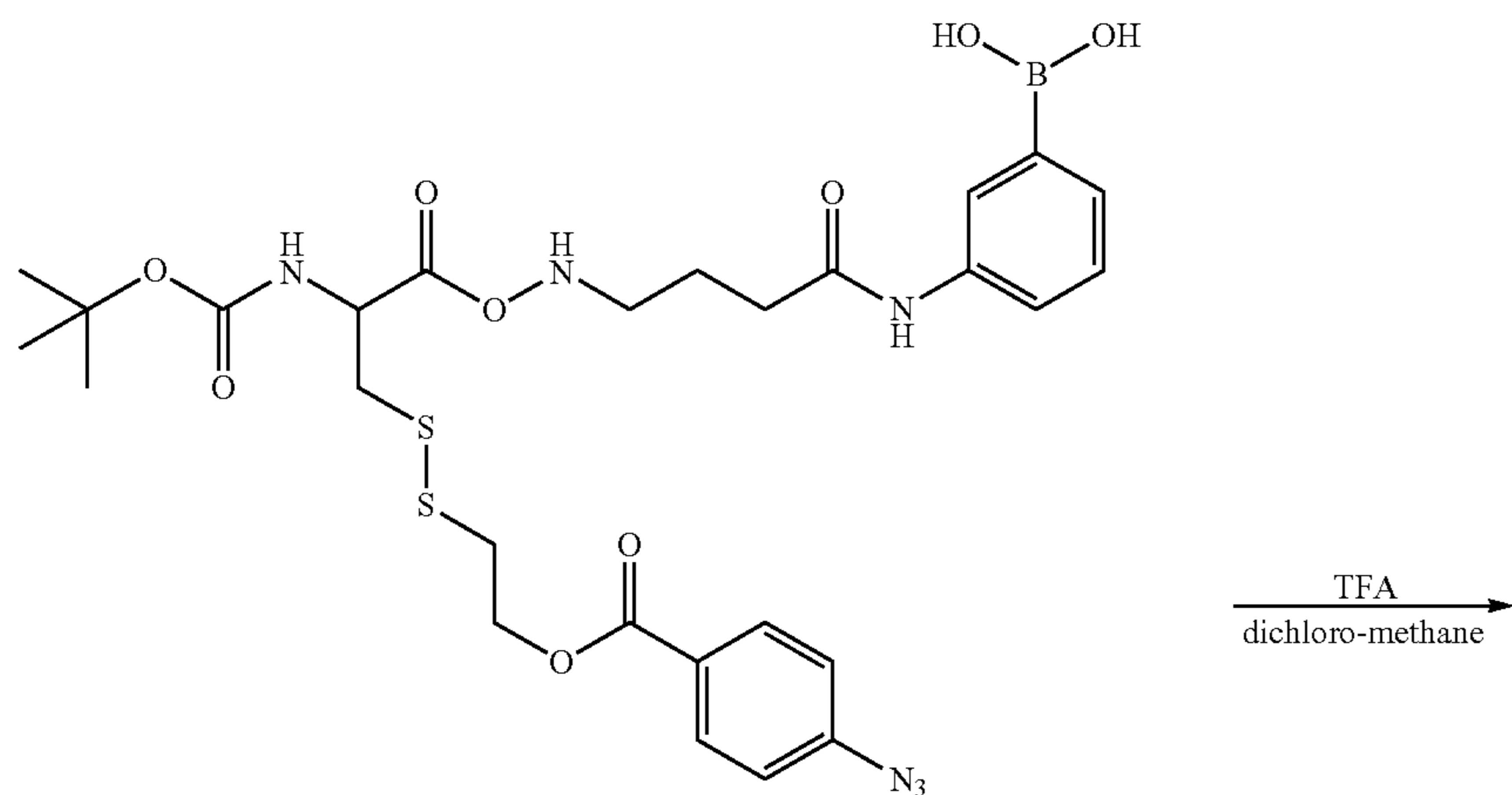
Scheme 21
