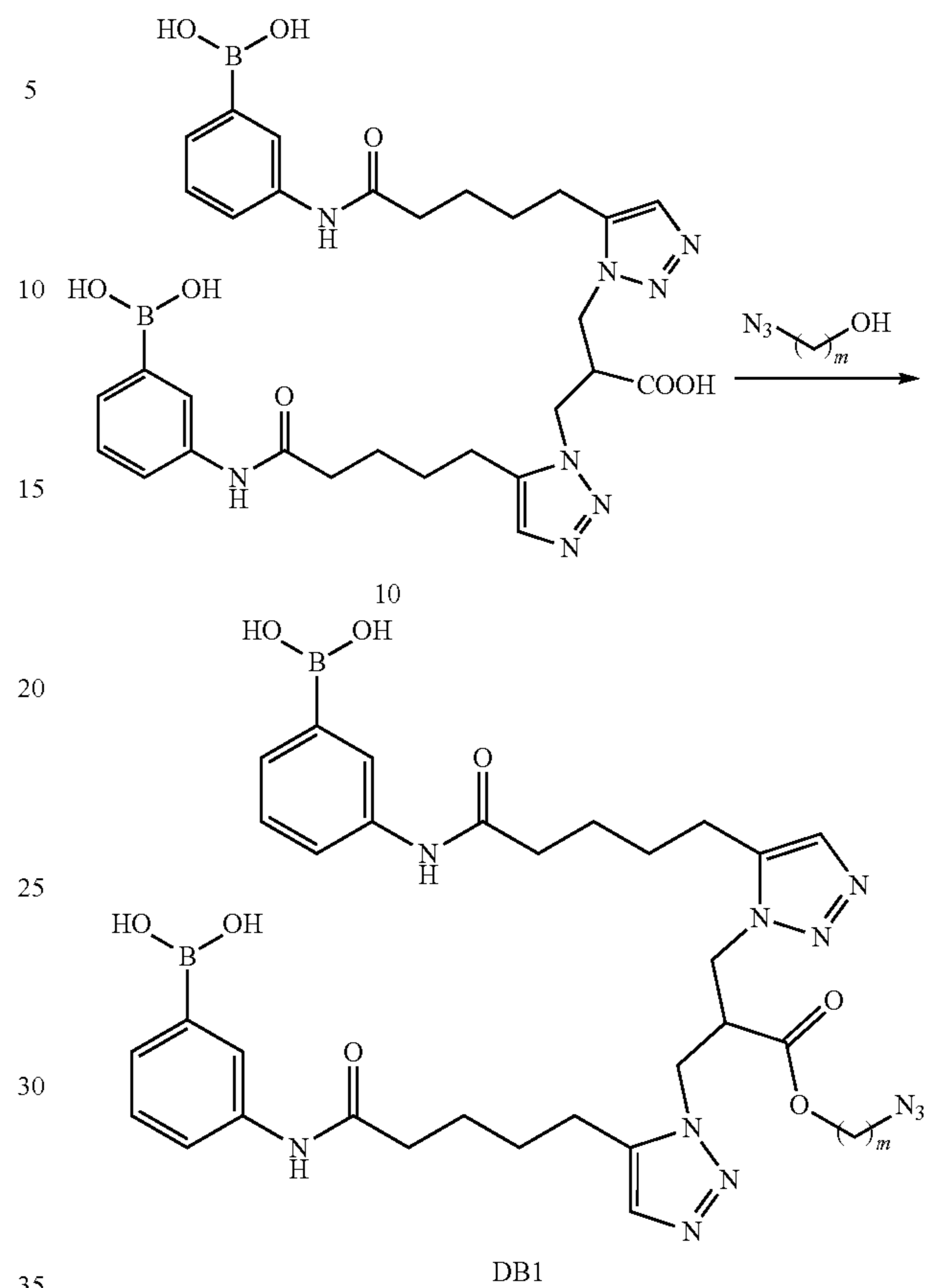
Scheme 9
