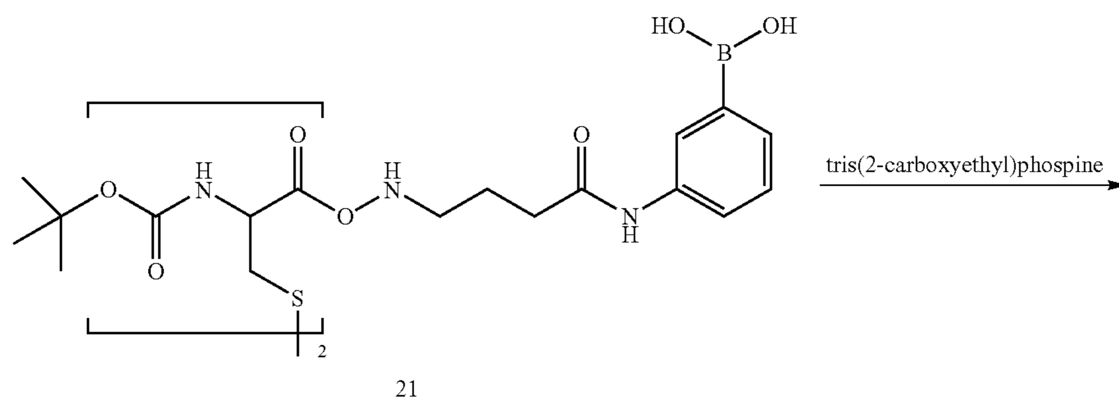
Scheme 19
