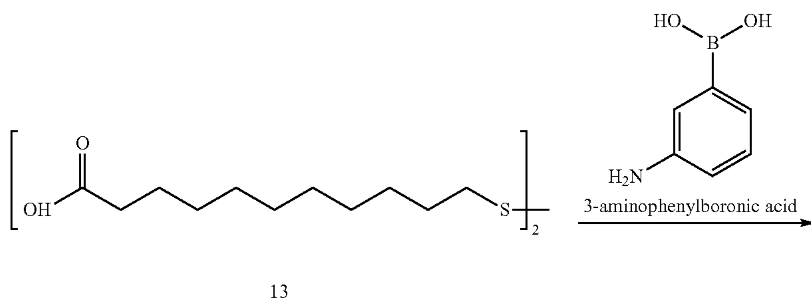
Scheme 13
