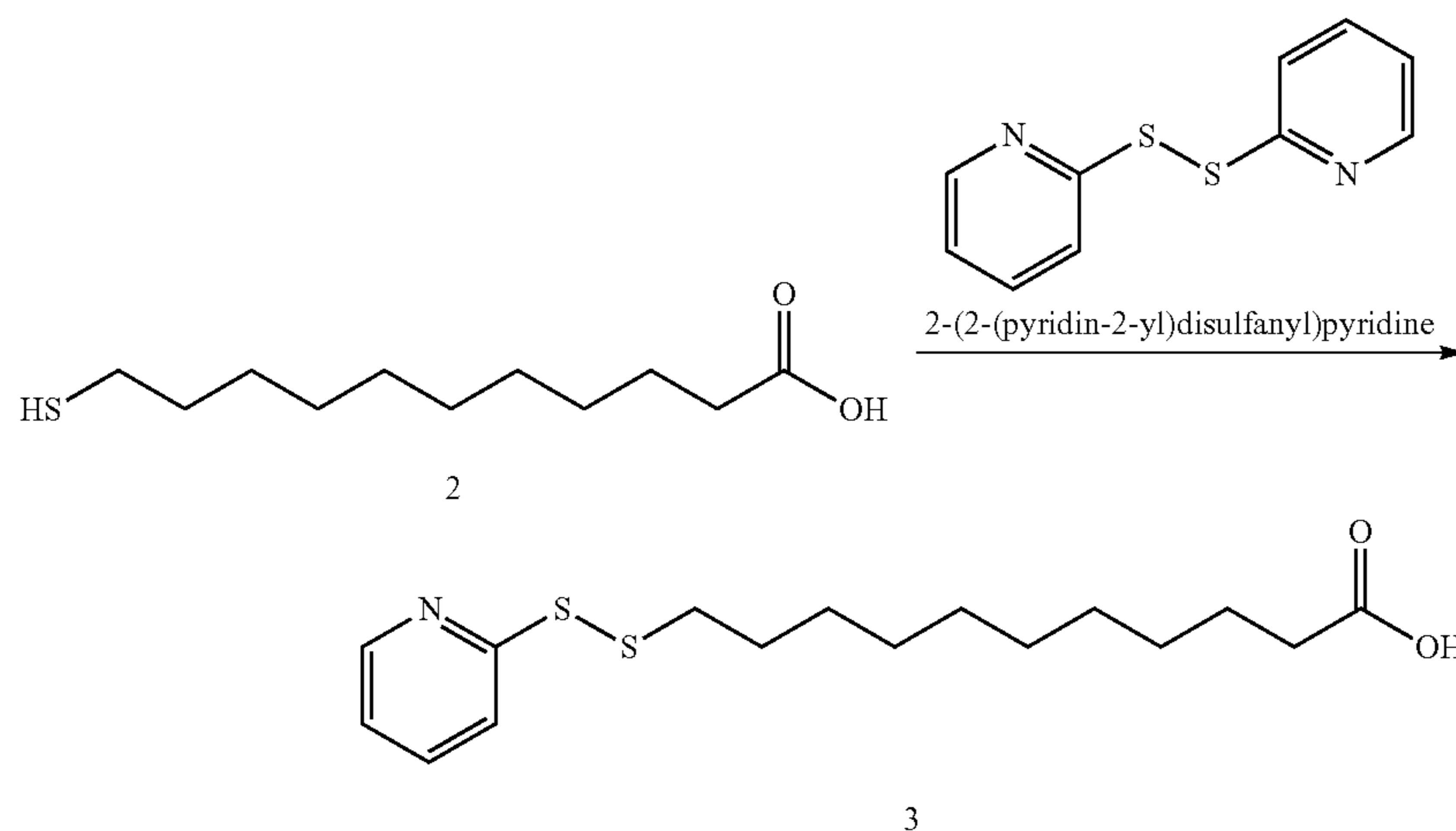
Scheme 2
