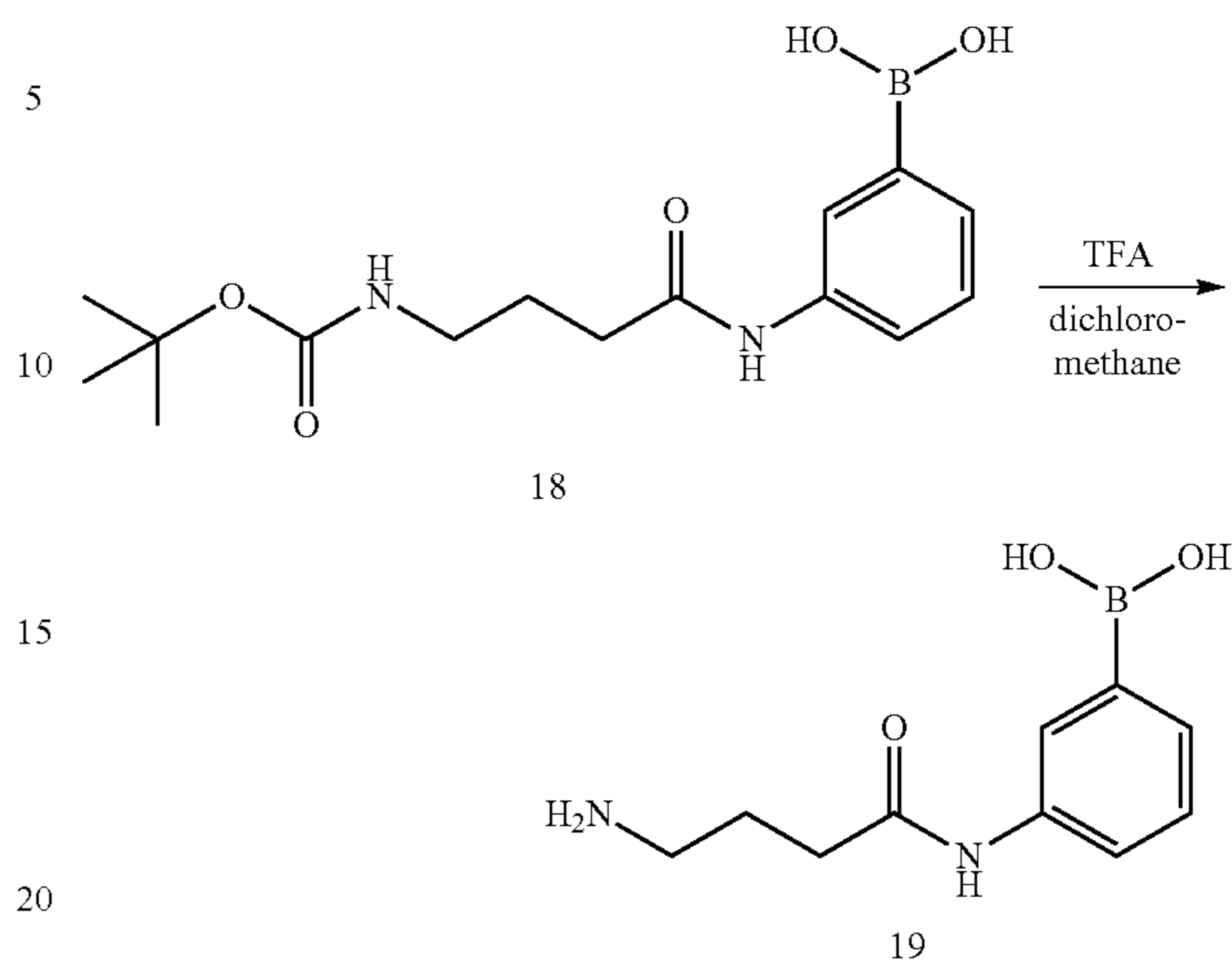
Scheme 17
