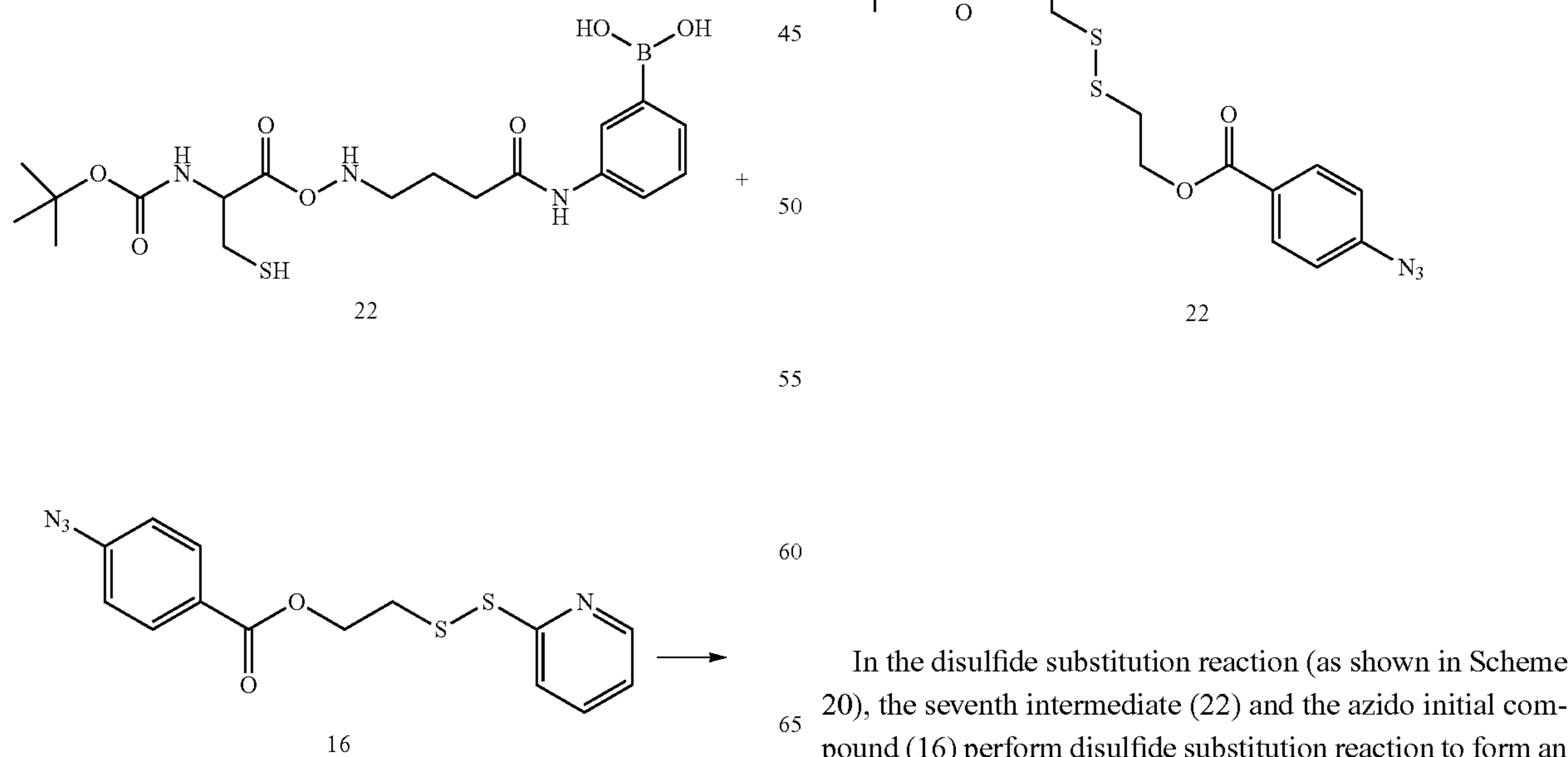
Scheme 20
