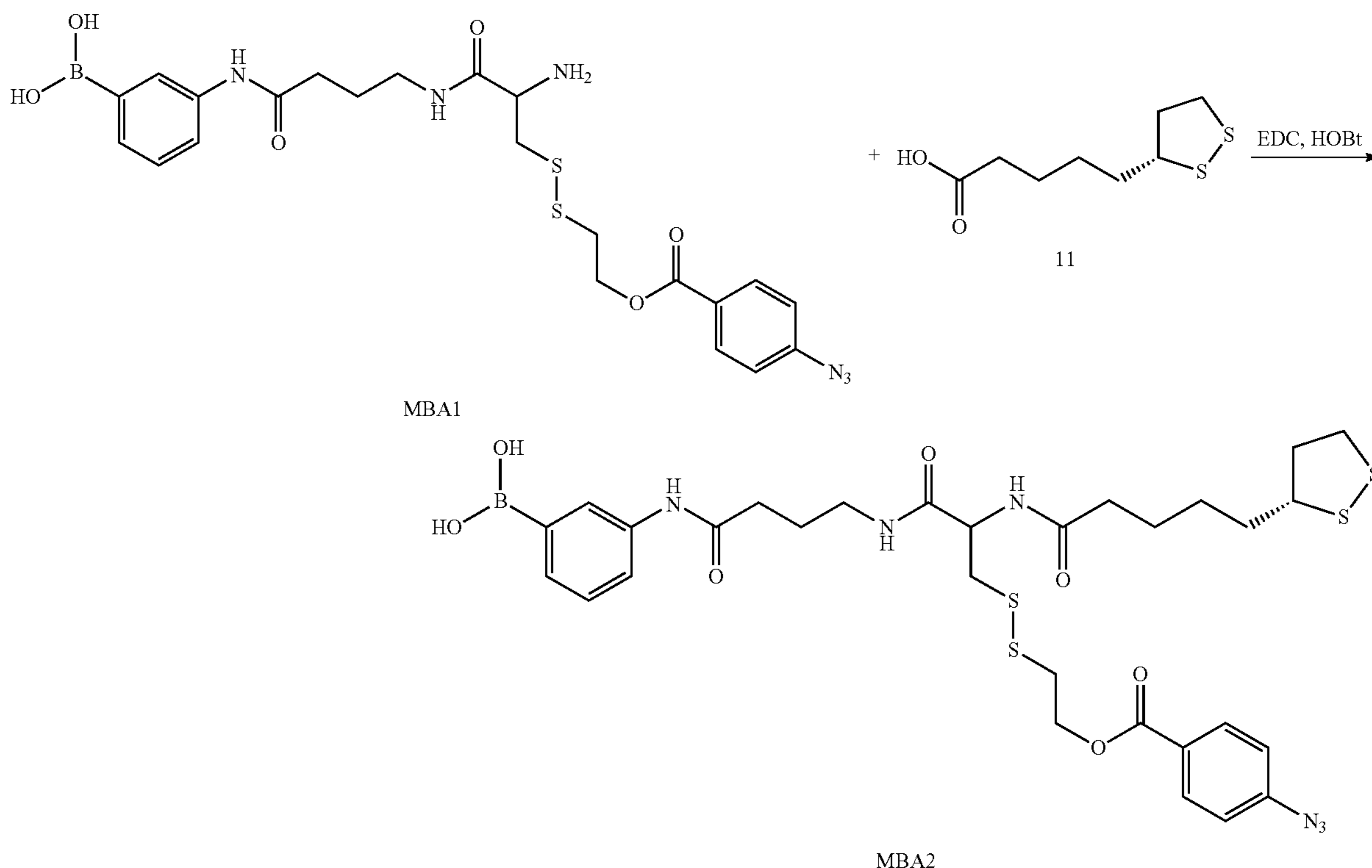
Scheme 22
