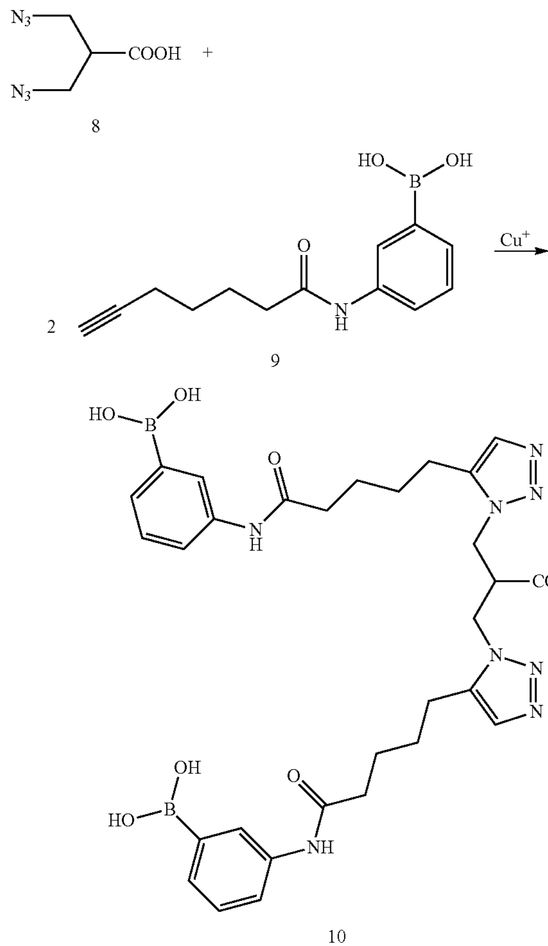
Scheme 8
