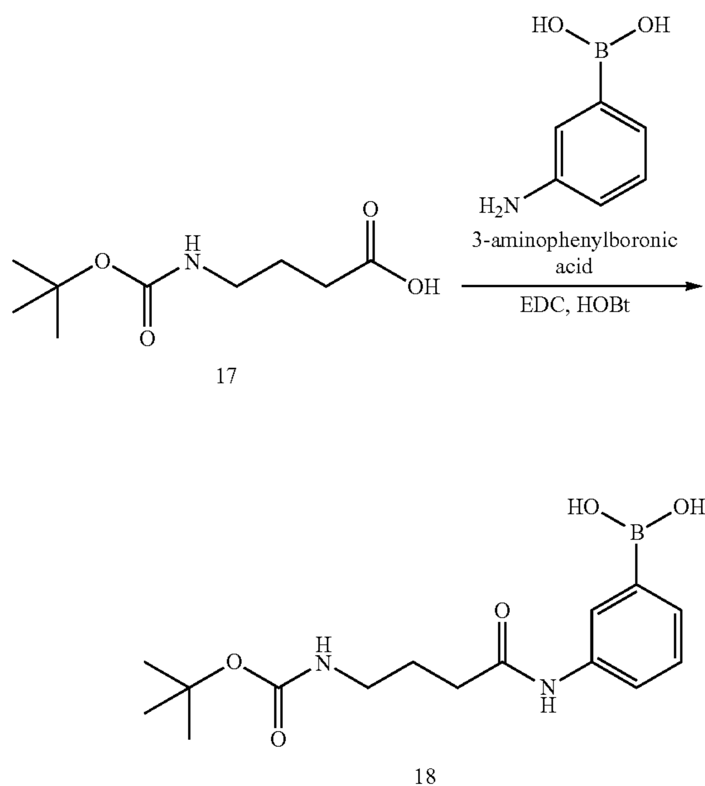
Scheme 16
