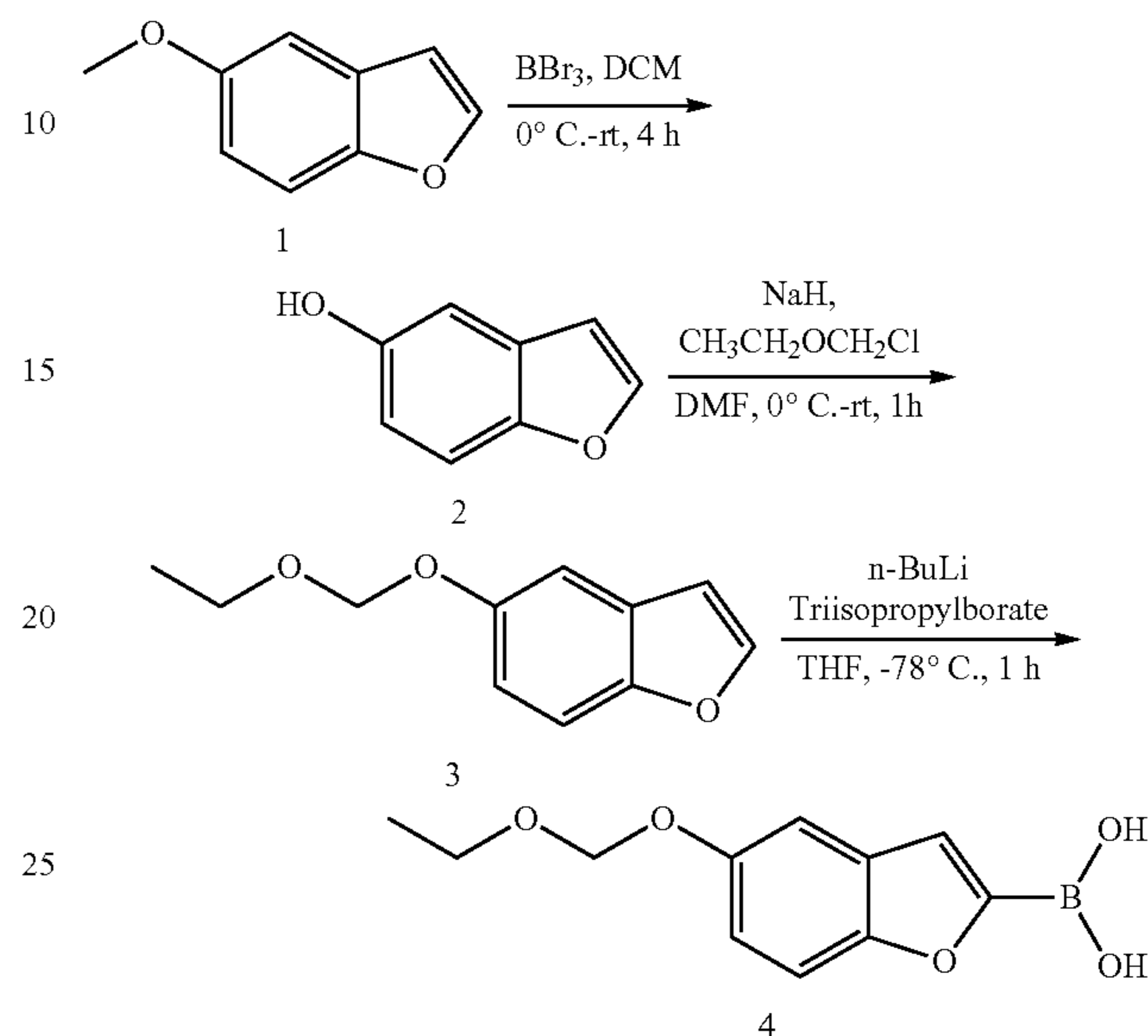
Scheme 1. Synthesis of 5-ethoxymethoxy-benzofuran-2-boronic acid (4)
