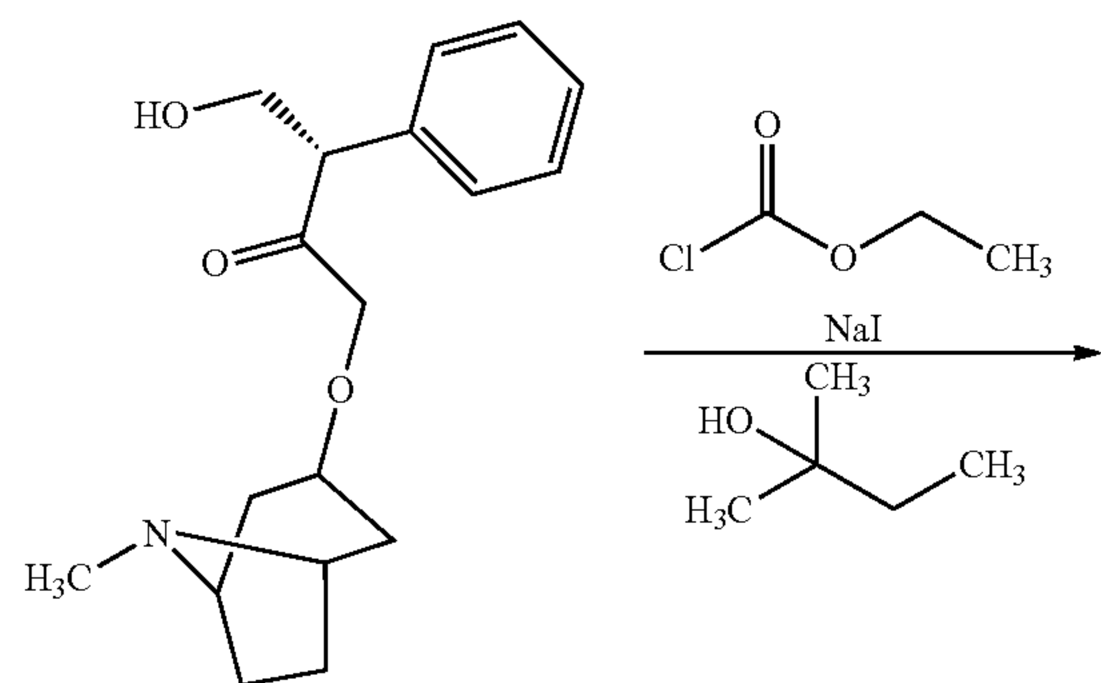
Scheme 15: Atropine
