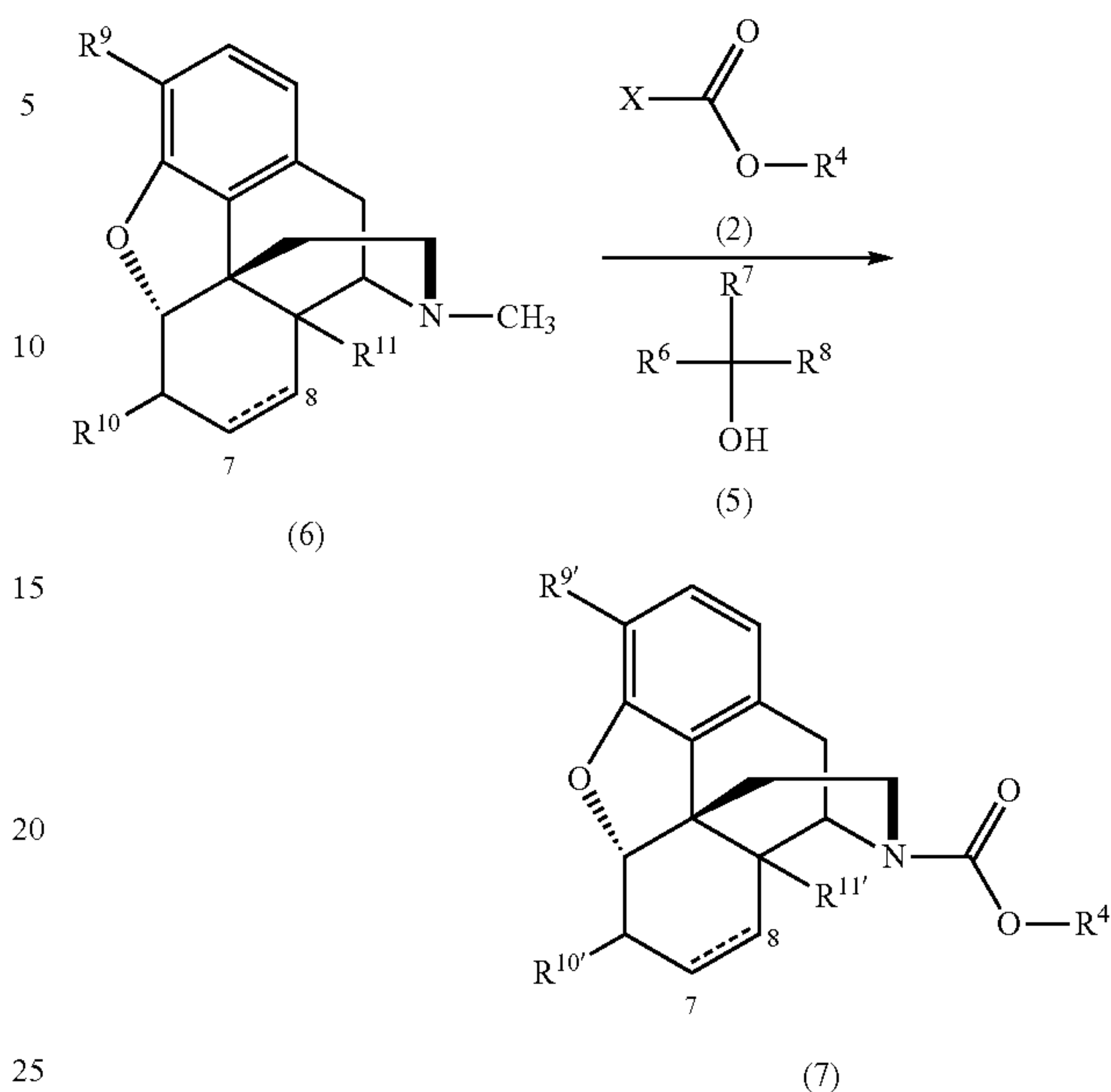
Scheme 4
