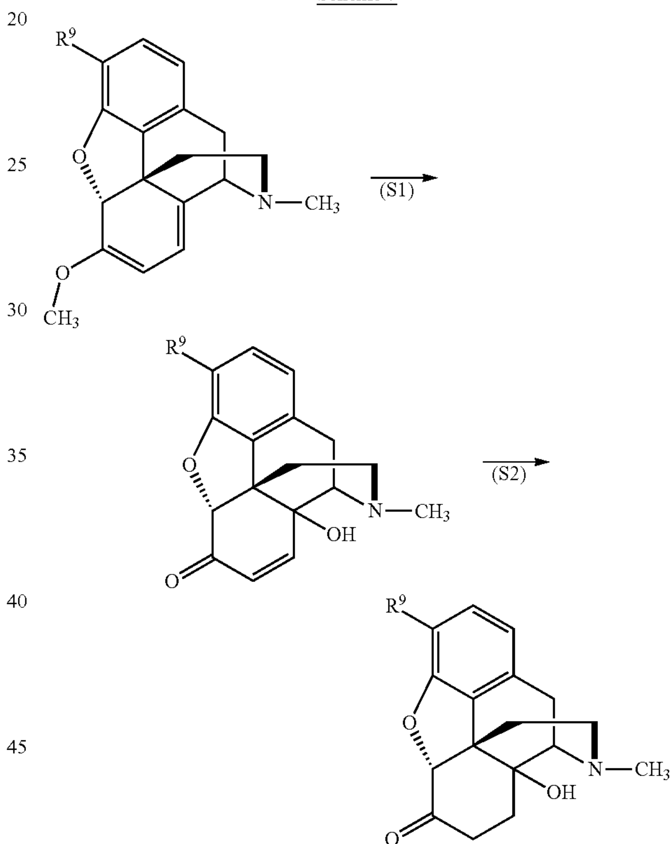
Scheme 7
