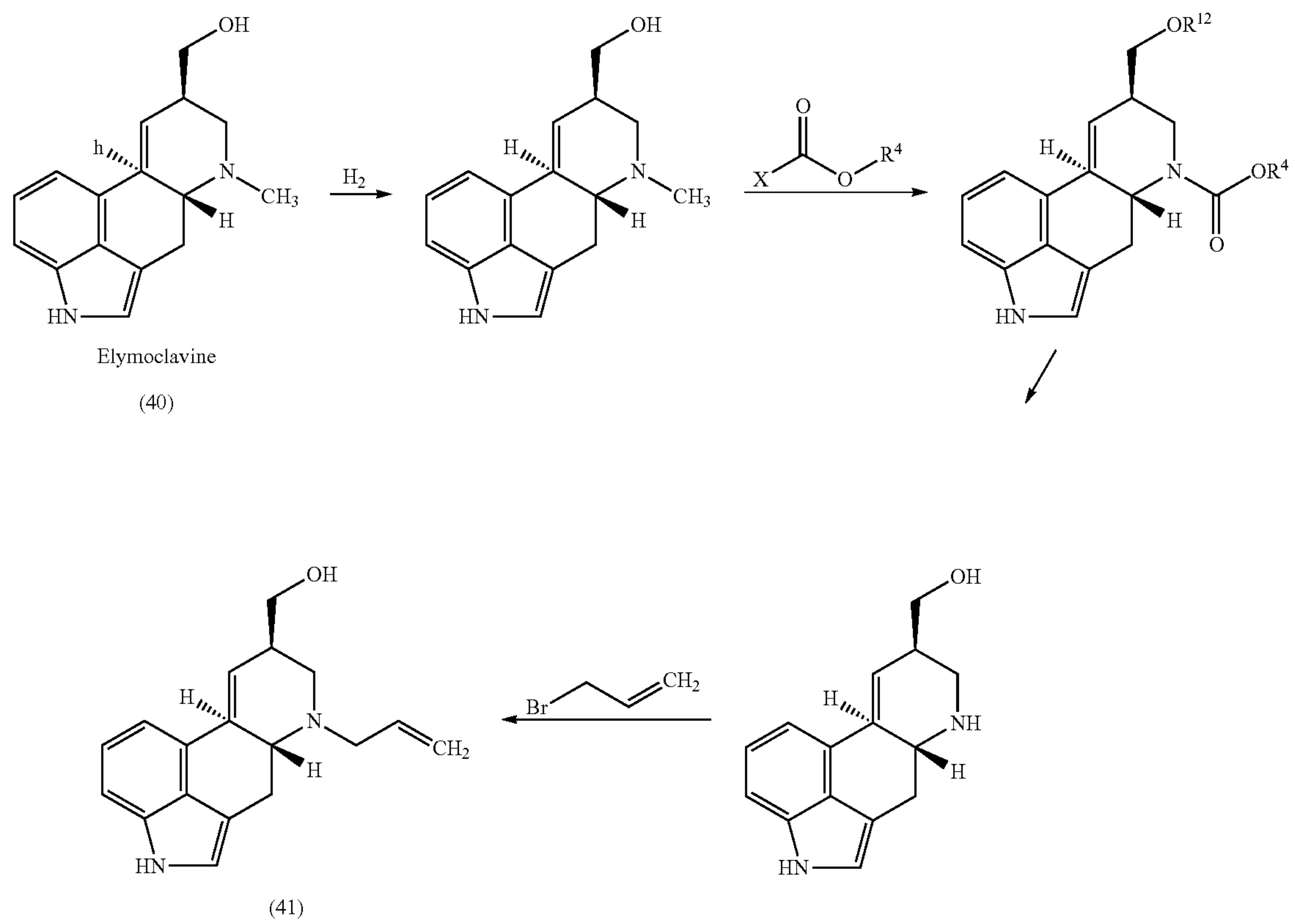
Scheme 14
