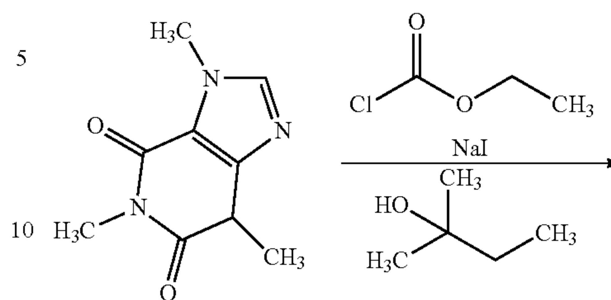
Scheme 16: Caffeine
