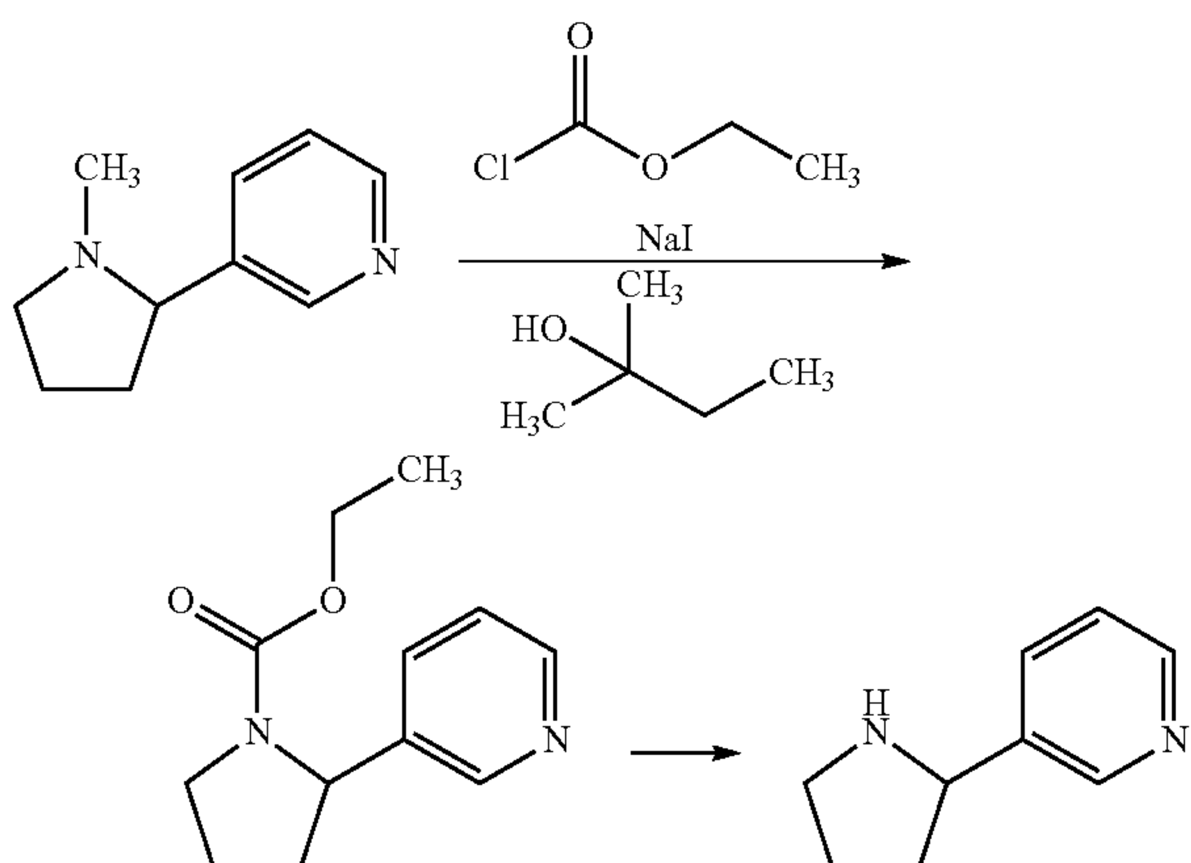
Scheme 19: Nicotine
