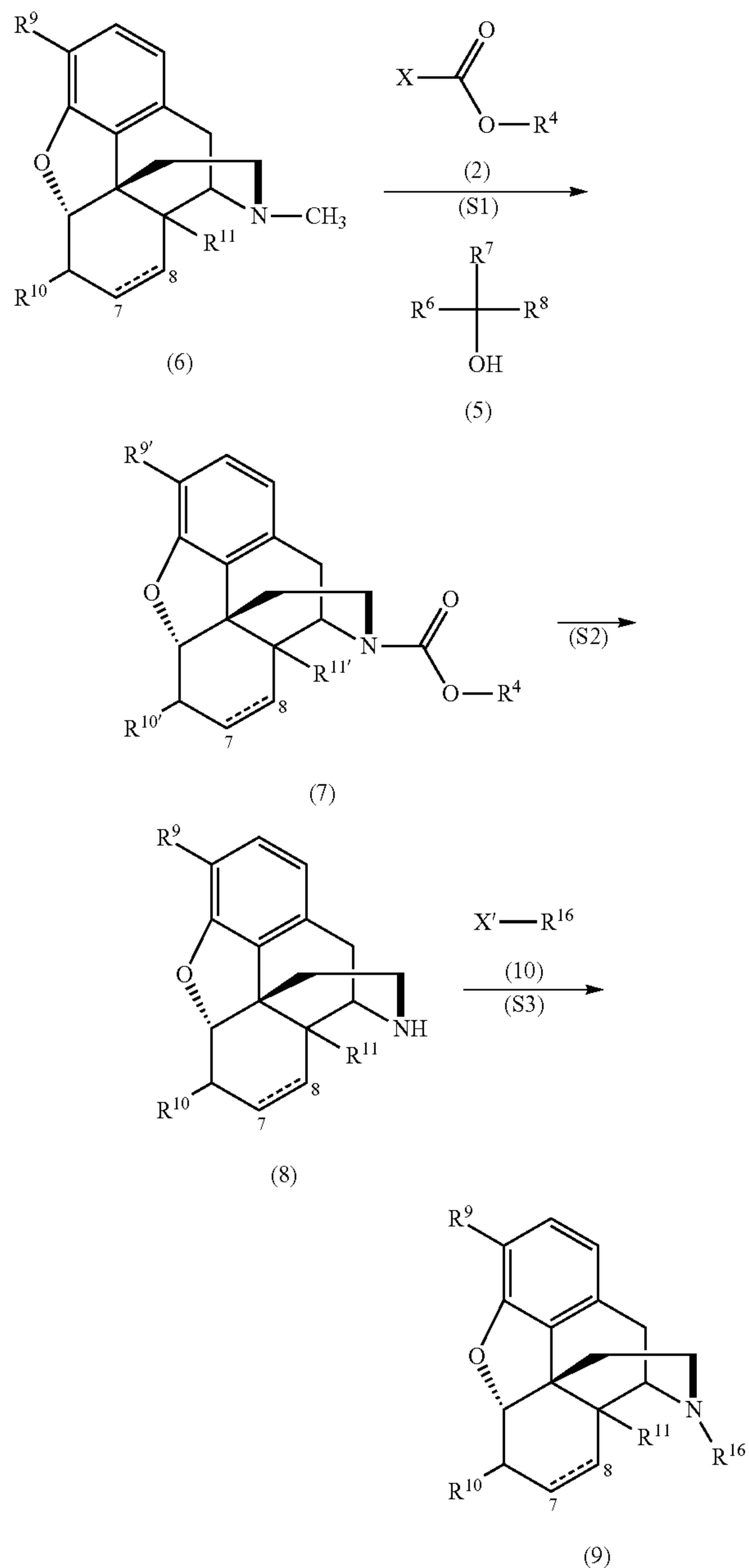
Scheme 6
