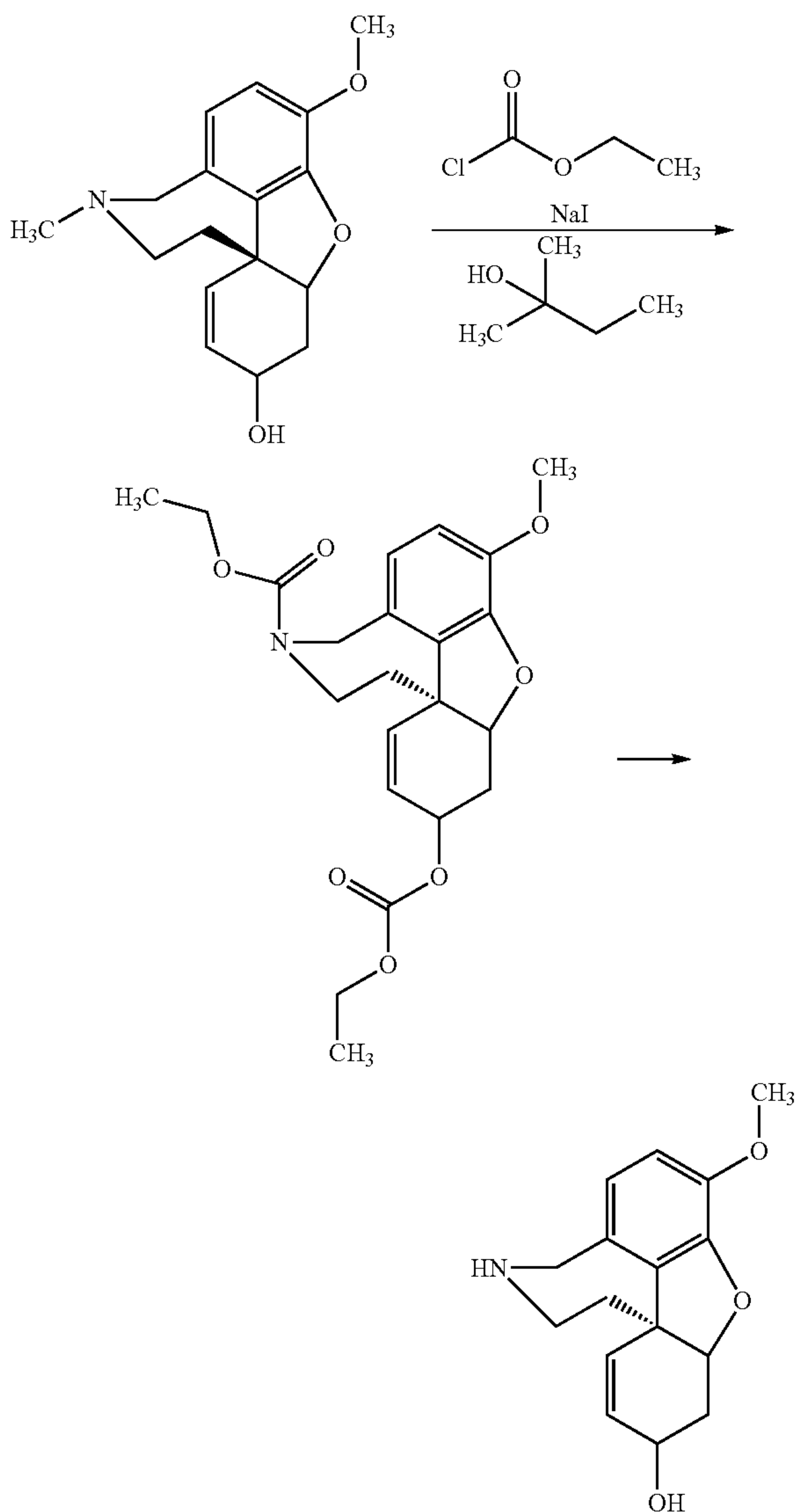
Scheme 18: Galanthamine
