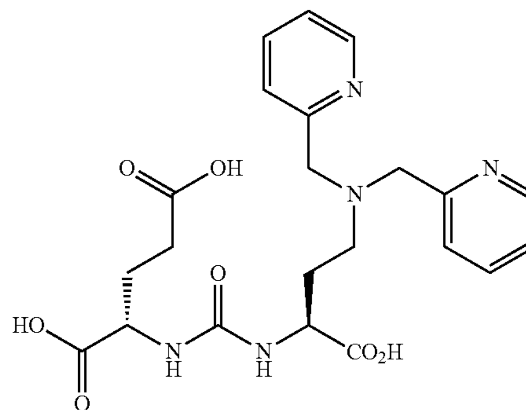
(S,S)-2-[3-[5-(Bis-pyridin-2-ylmethyl-amino)-1-carboxy-pentyl]-ureido]-pentanedioic acid (10) (MIP 1008)
