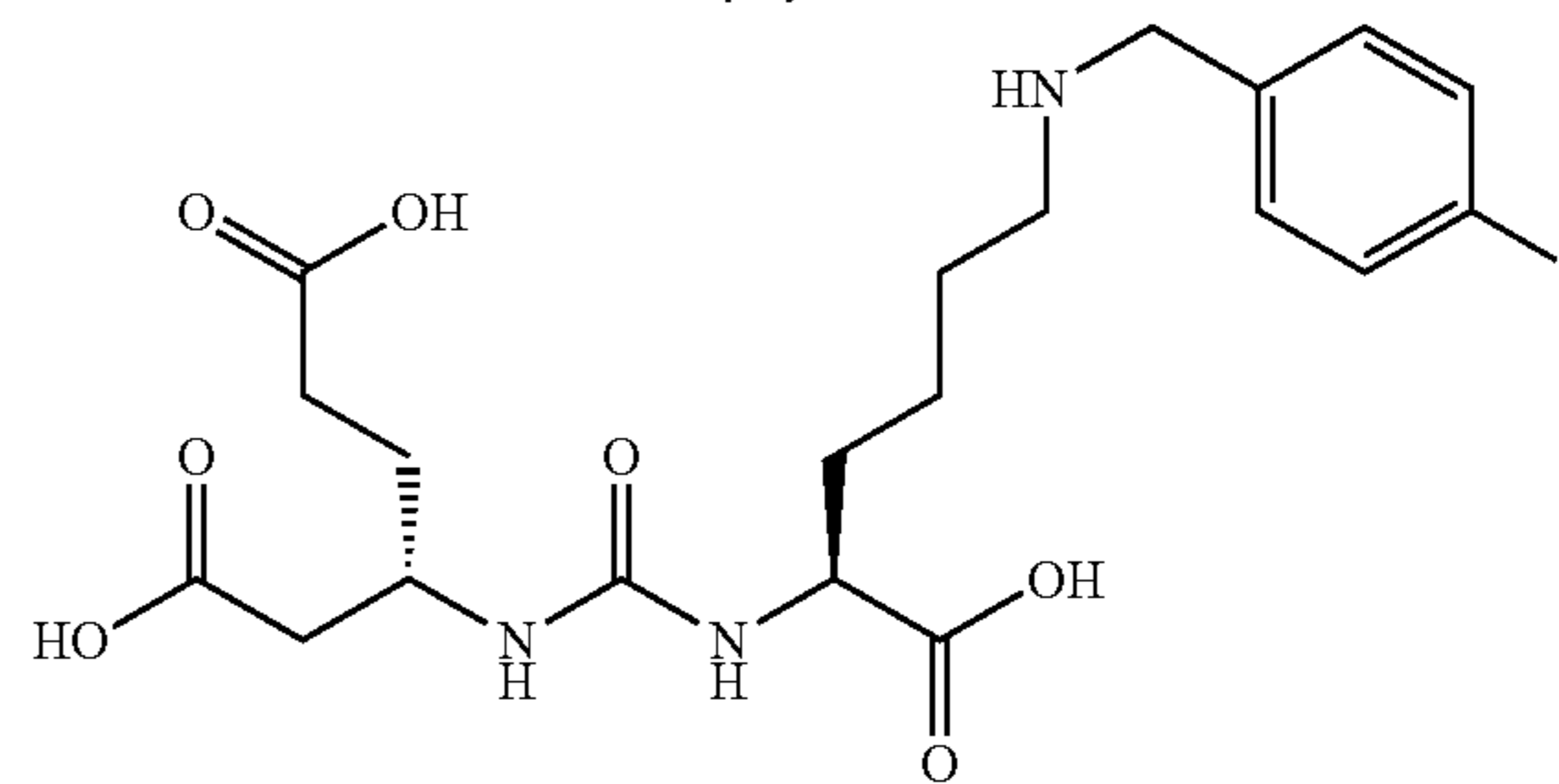
β-glu
