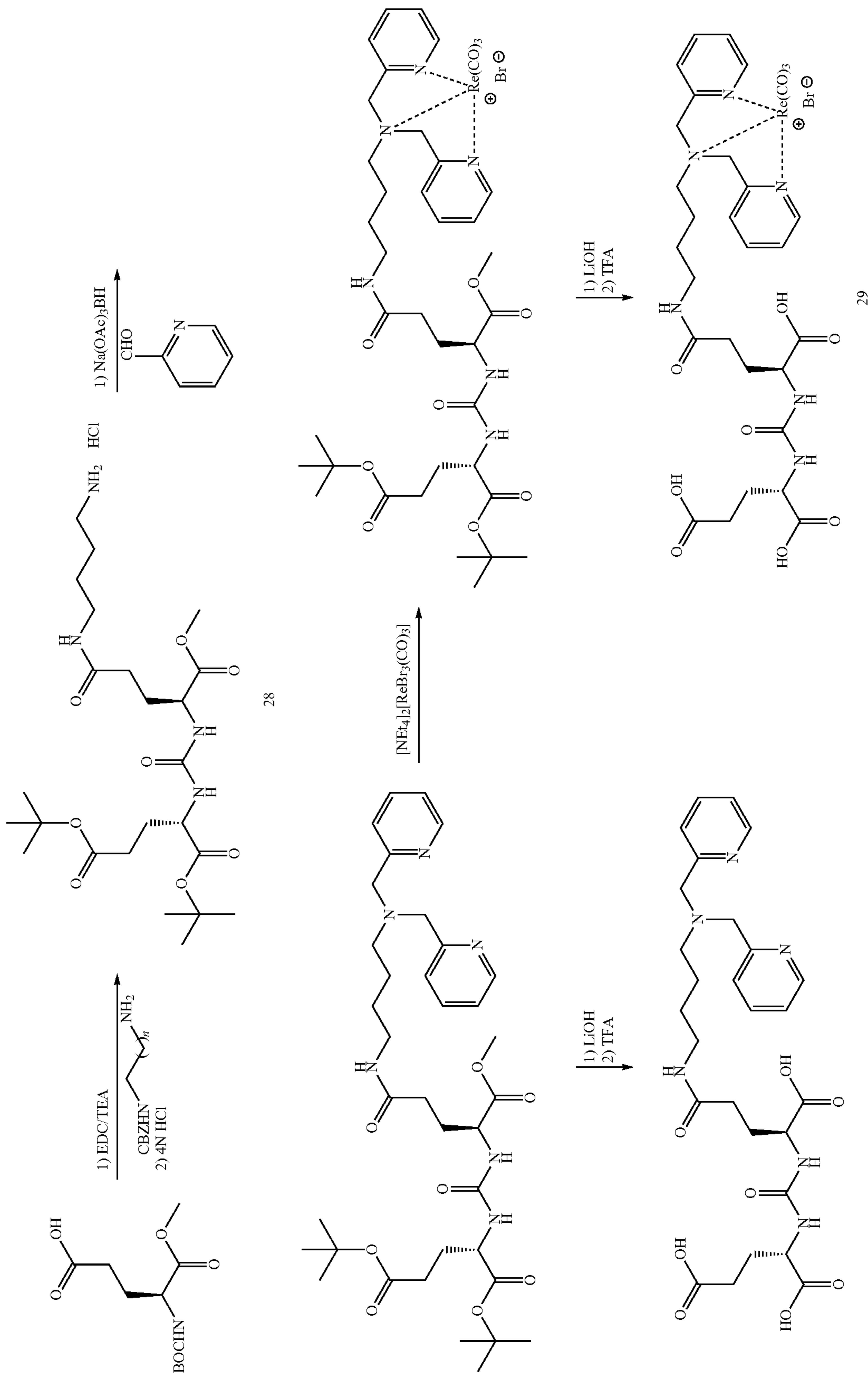
Scheme 4.
