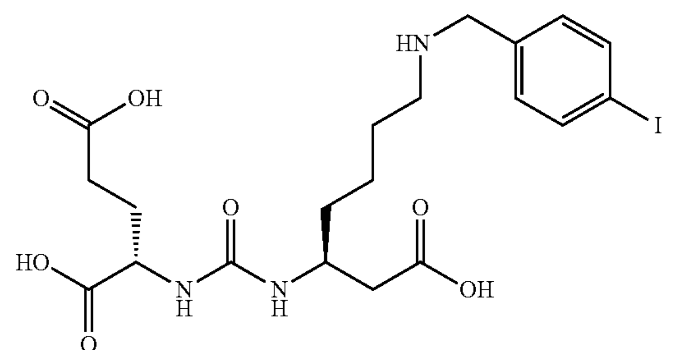
β-lysine
