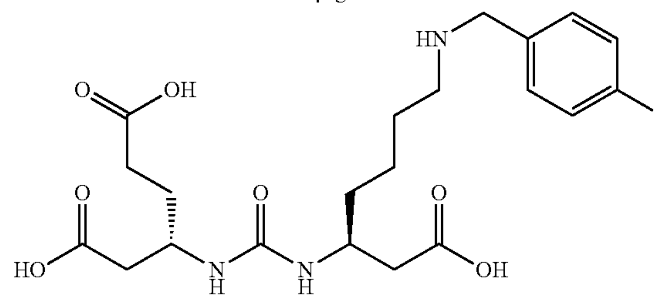
β-lys, β-glu
