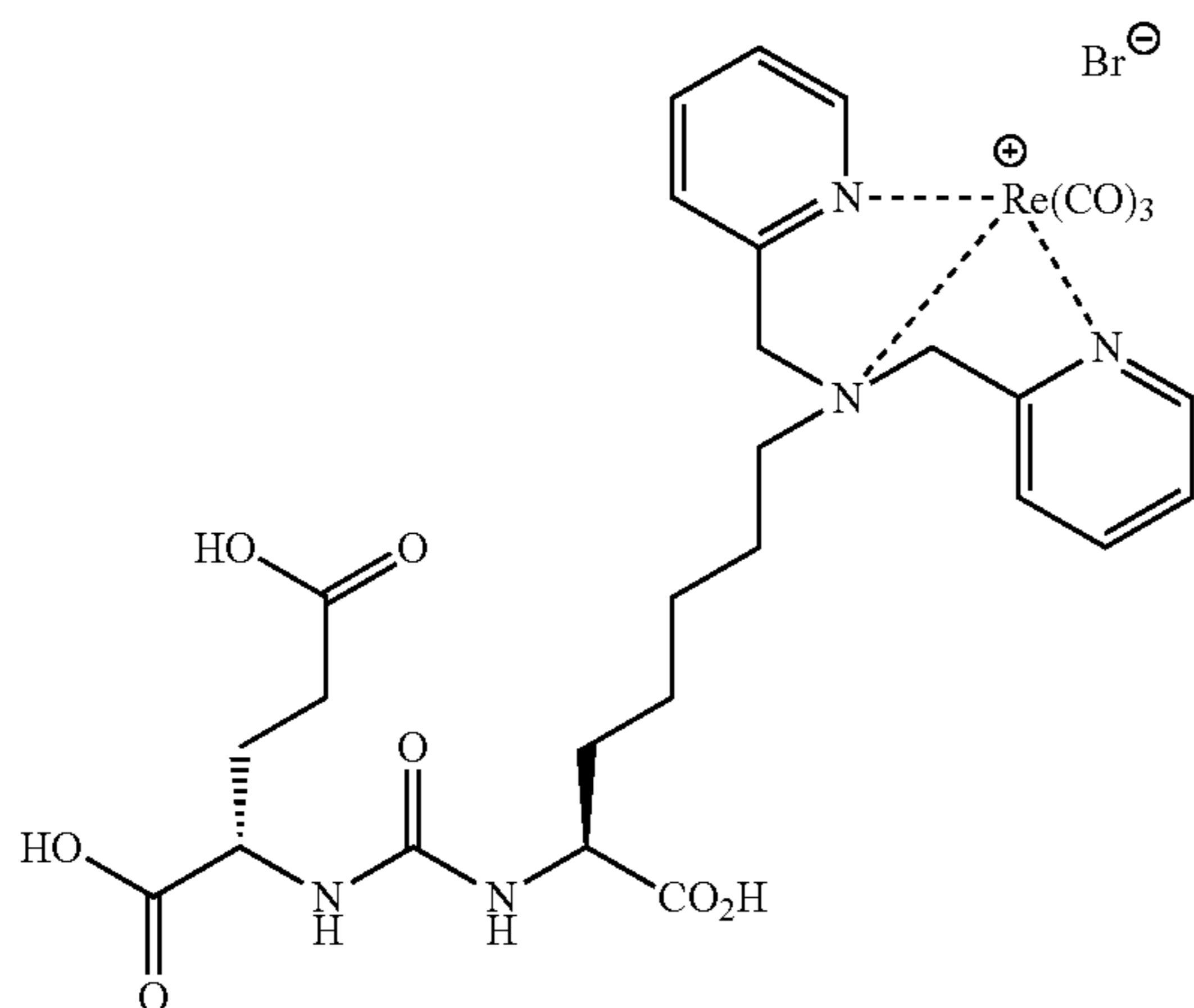
2-{3-[1-Carboxy-5-(carboxymethyl-pyridin-2-ylmethyl-amino)-pentyl]-ureido}-pentanedioic acid (26)
