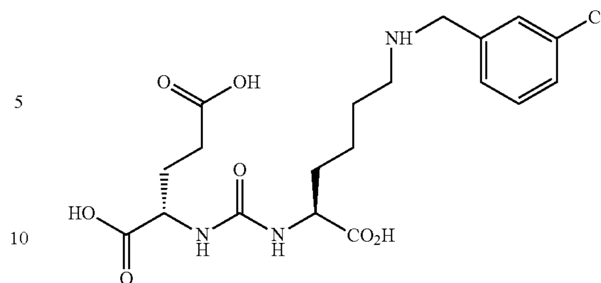
(S,S)-2-{3-[1-Carboxy-5-(4-chloro-benzylamino)-pentyl]-ureido}-pentanedioic acid (9) (MIP 1135)
