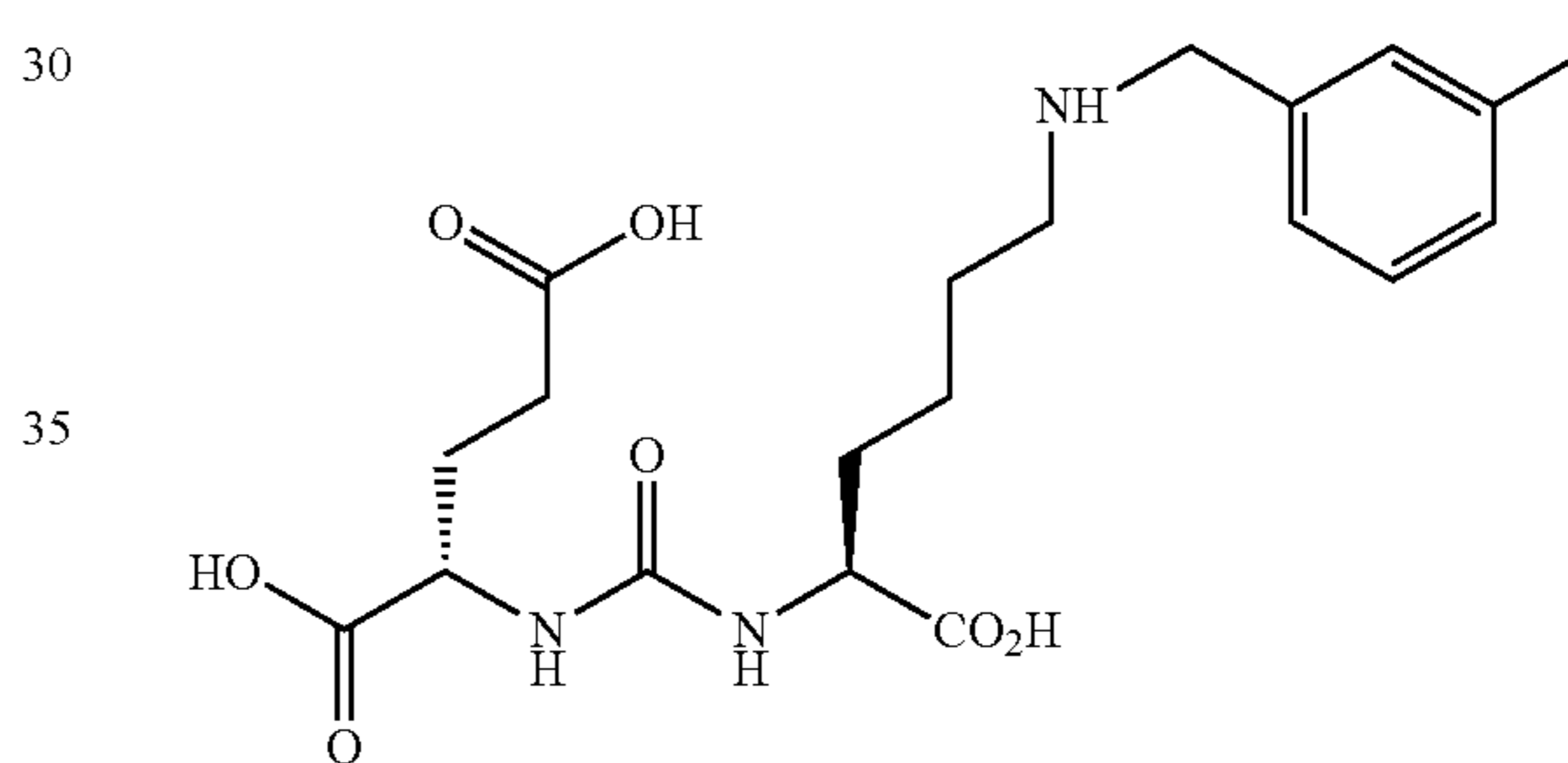
(S,S)-2-{3-[1-Carboxy-5-(4-iodo-benzylamino)-pentyl]-ureido}-pentanedioic (14) (MIP 1072)
