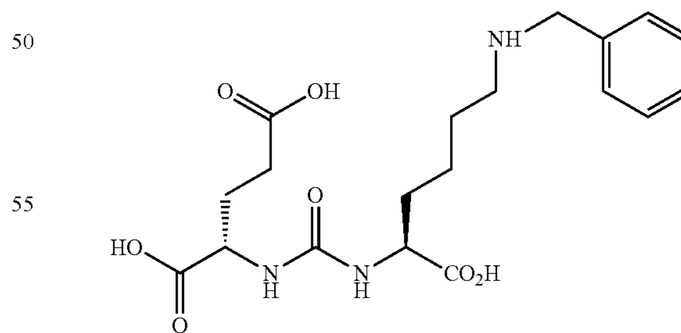
2-(3-{1-Carboxy-5-[3-(phenyl)-ureido]-pentyl}-ureido)-pentanedioic acid (11) (MIP 1111)
