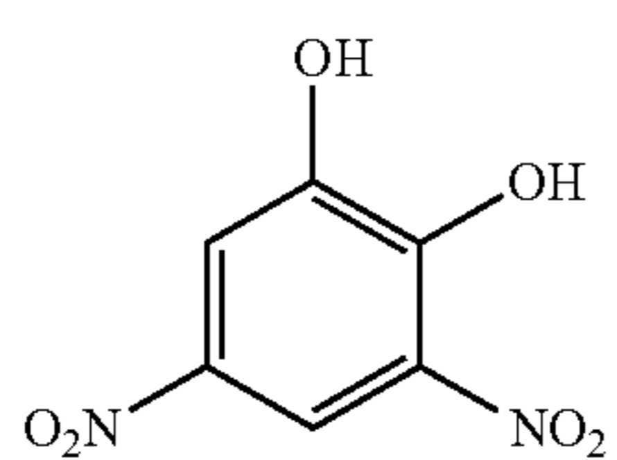
3,5-dinitrocatechol
