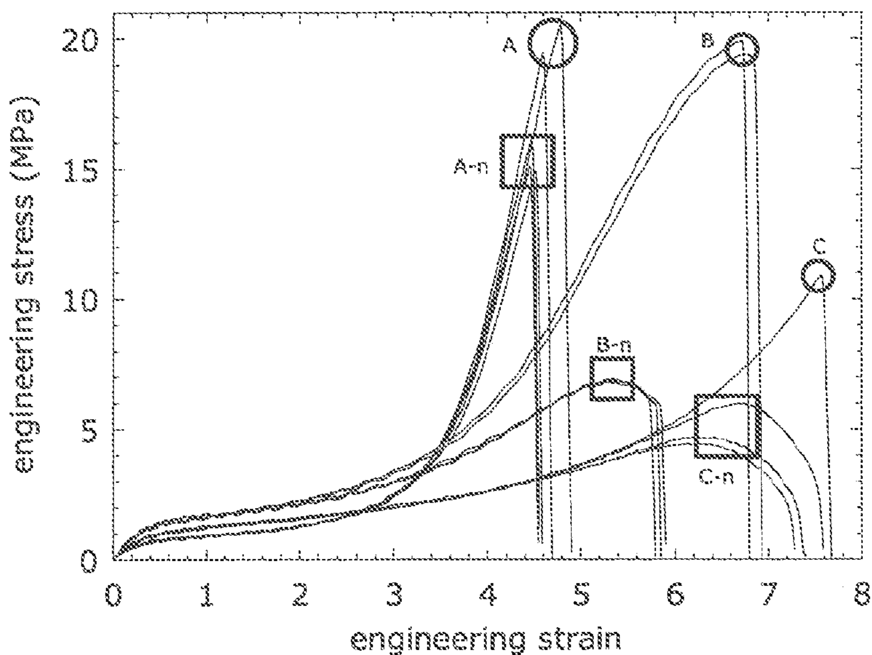
High Speed Tensile Results: Three Films
