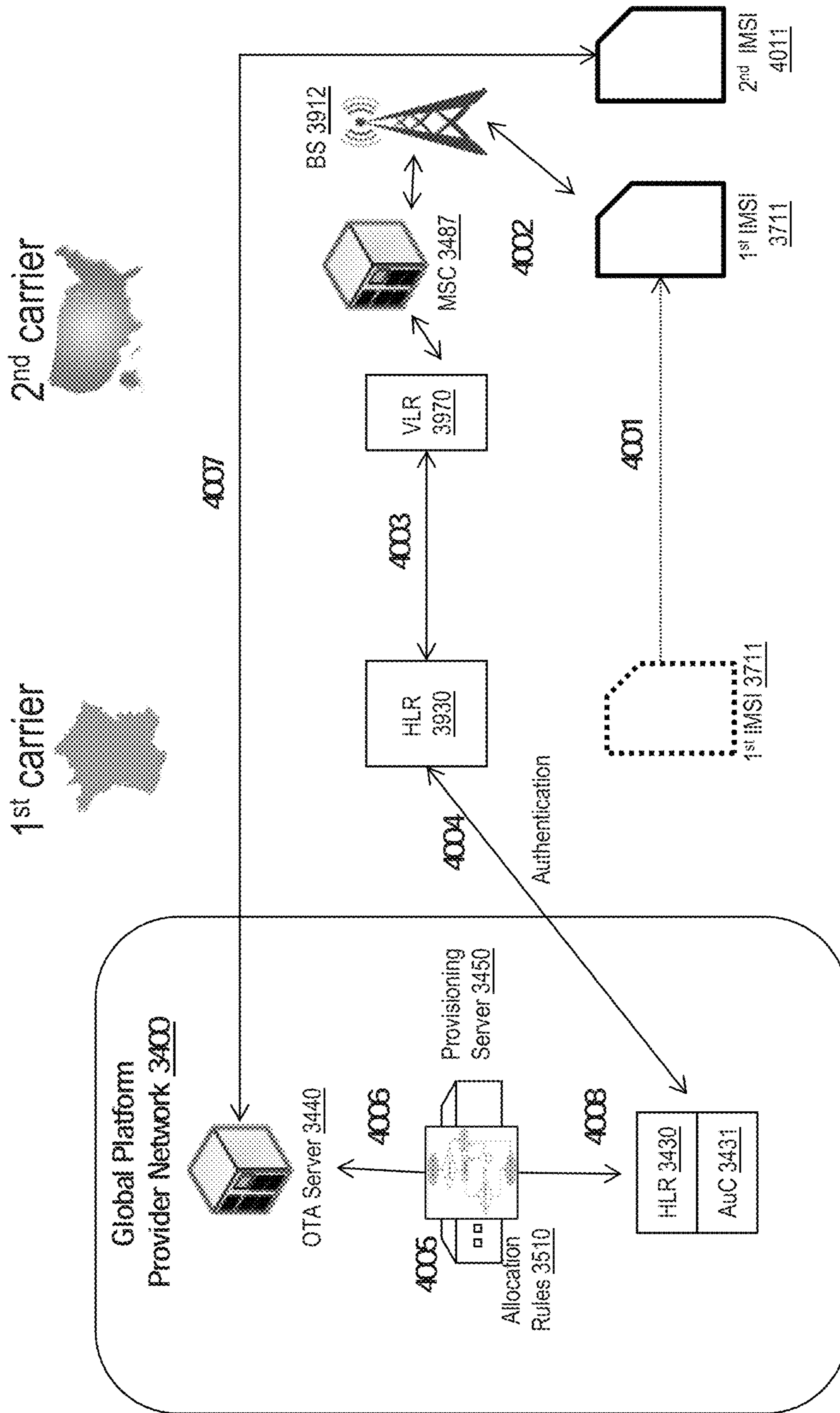
FIG. 40 IMSI Reallocation
