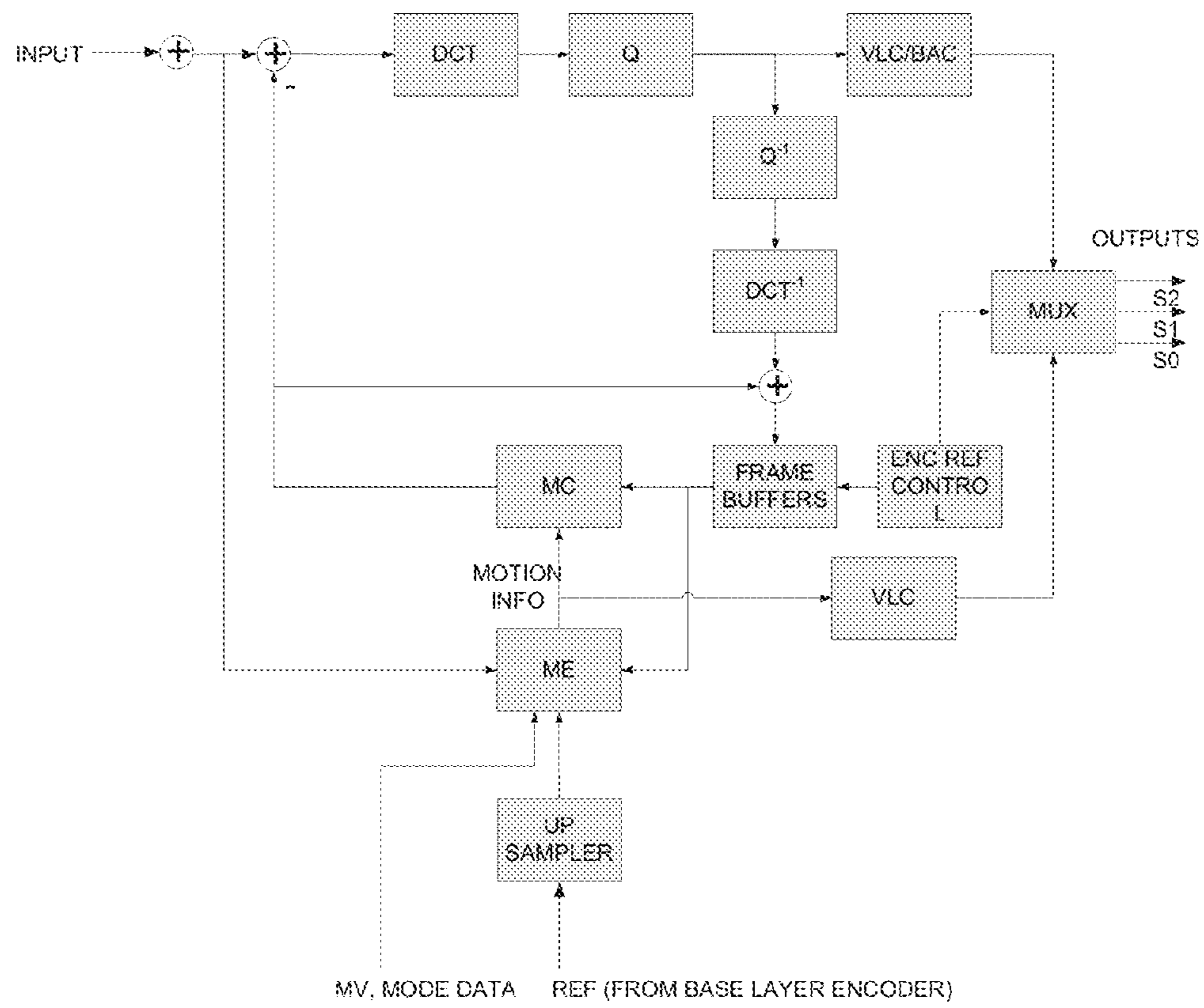
FIG. 6: SPATIAL SCALABILITY ENHANCEMENT LAYER CODEC
