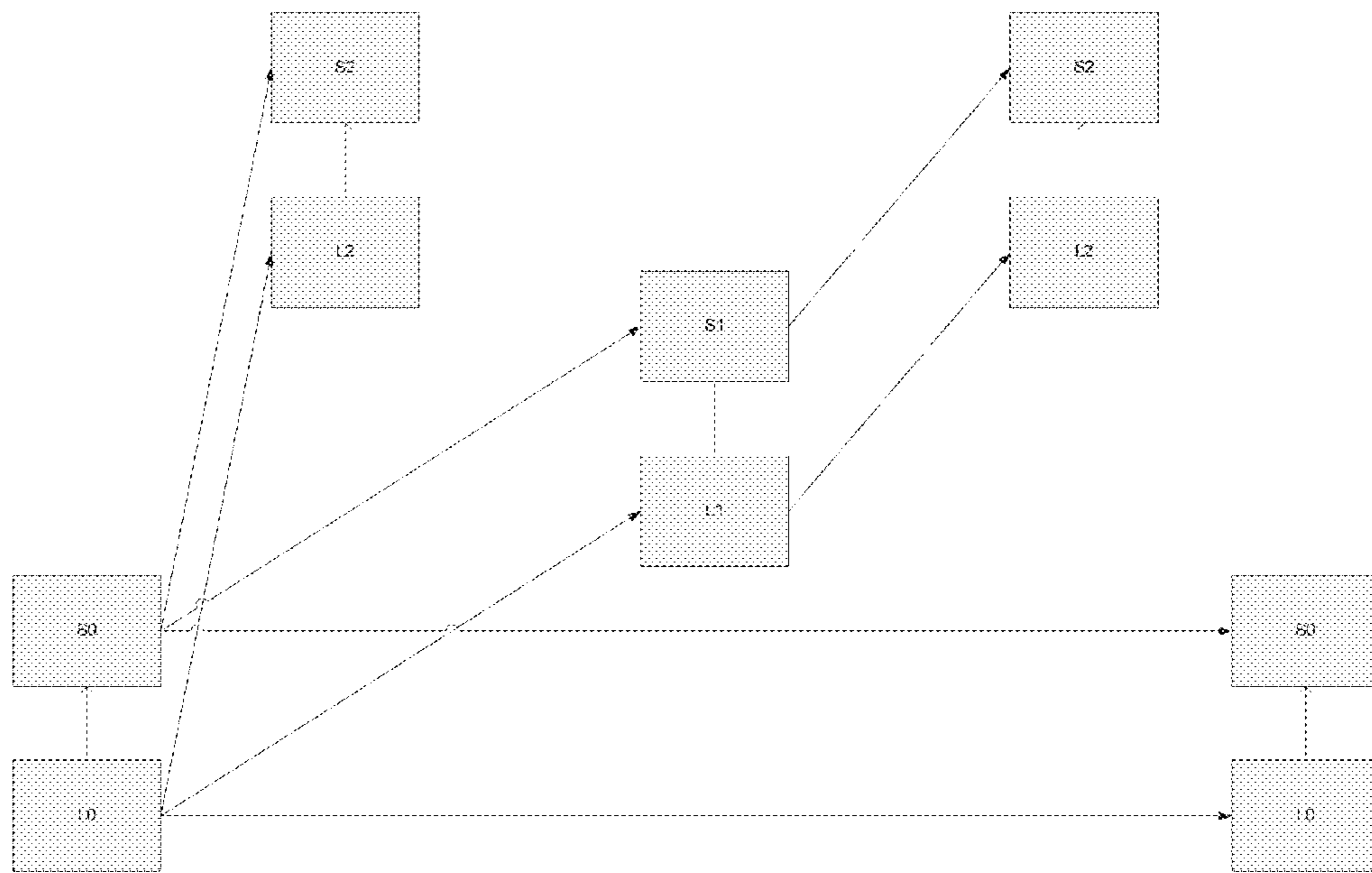
FIG. 7: PICTURE CODING STRUCTURE FOR SPATIAL SCALABILITY
