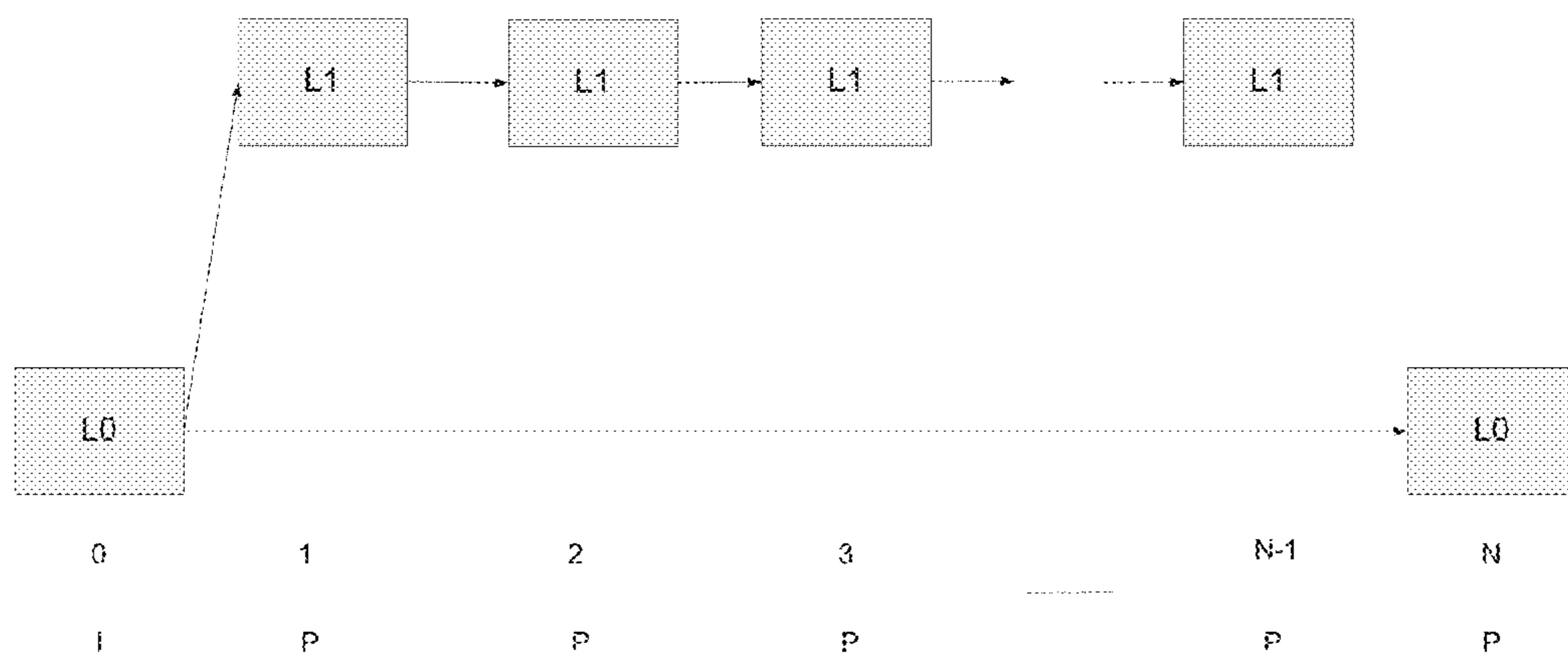
FIG. 5: ALTERNATIVE PICTURE CODING STRUCTURE EXAMPLE
