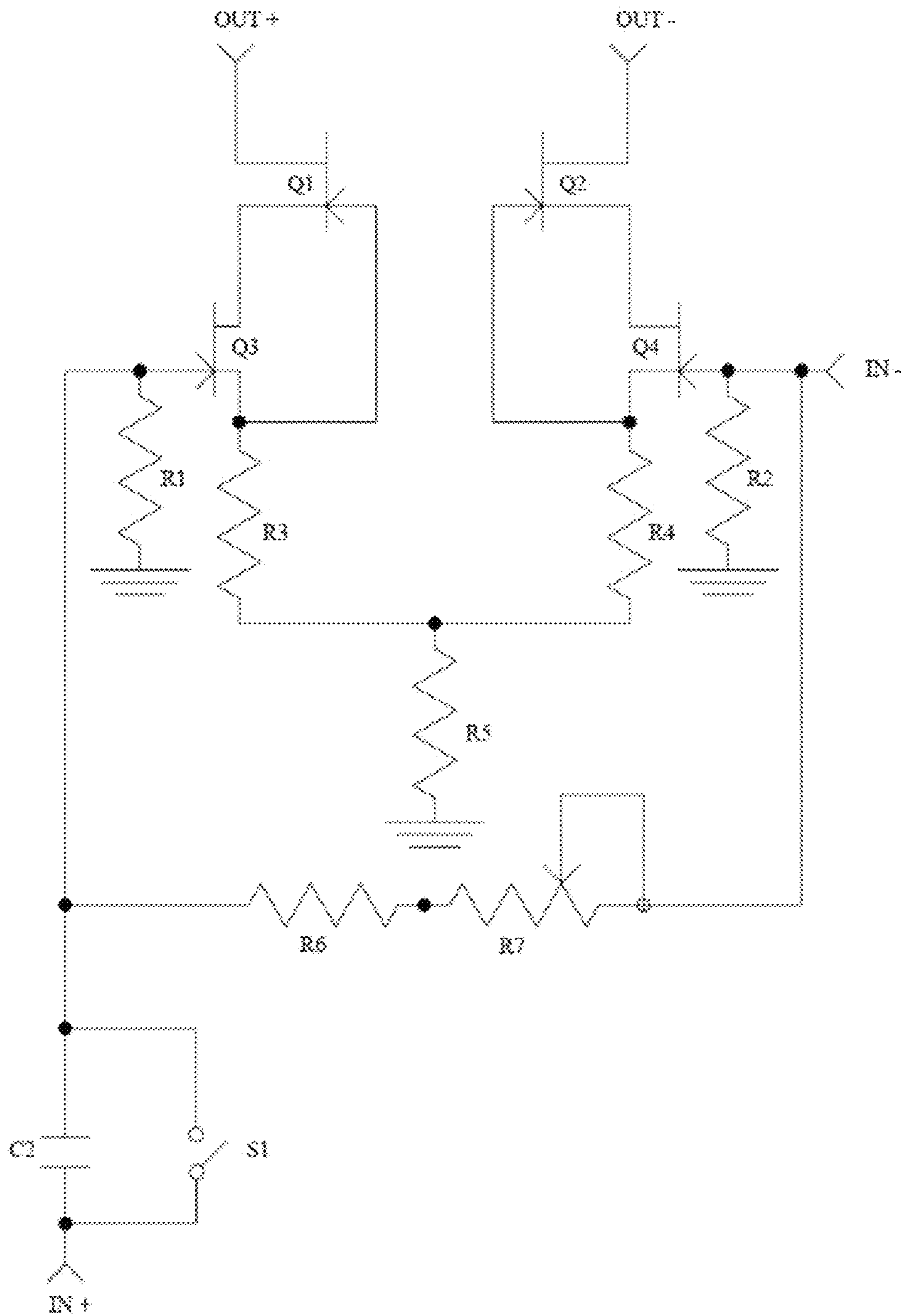
Preamp Circuit without C1
