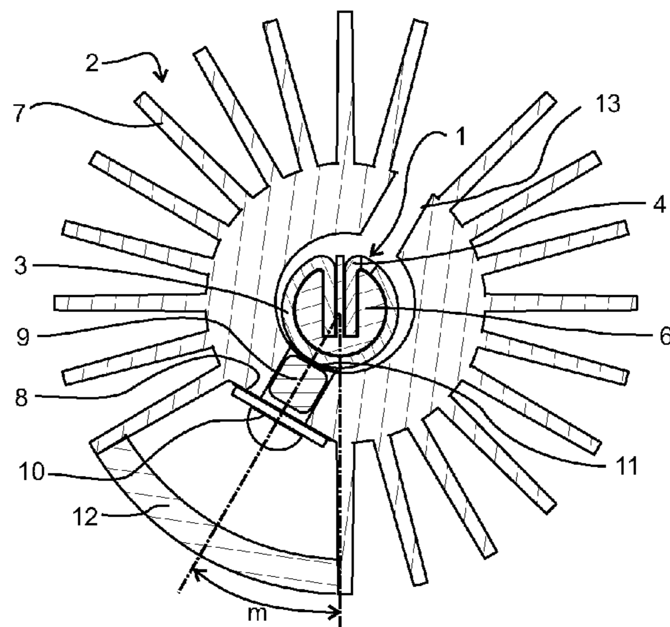
FIG. 4 (SECTION B-B OF FIG. 3)
