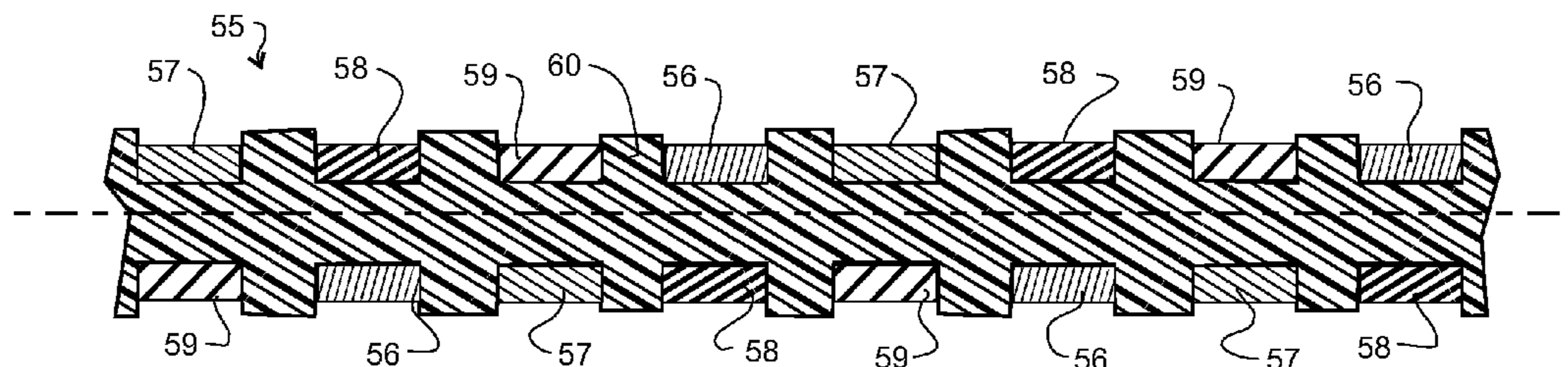
FIG. 26 (SECTION A-A OF FIG. 25)
