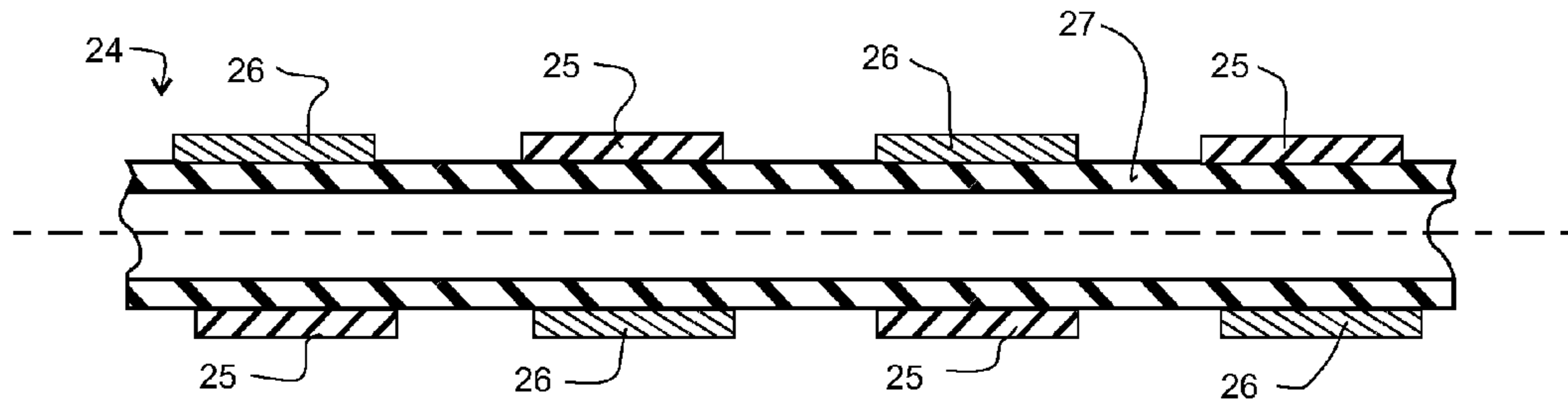
FIG. 12 (SECTION A-A OF FIG. 11)
