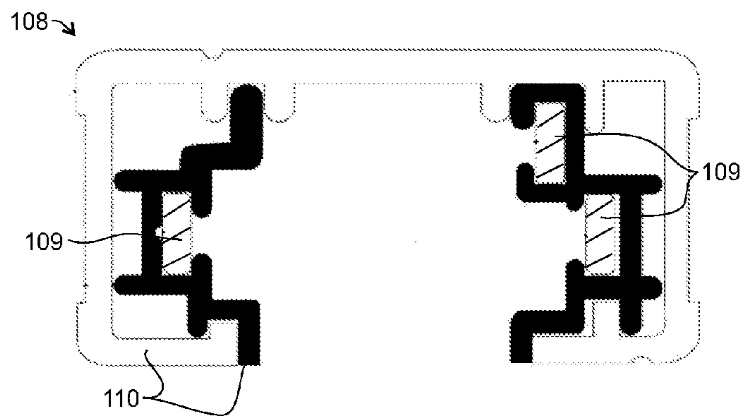
FIG. 38 (PRIOR ART)
