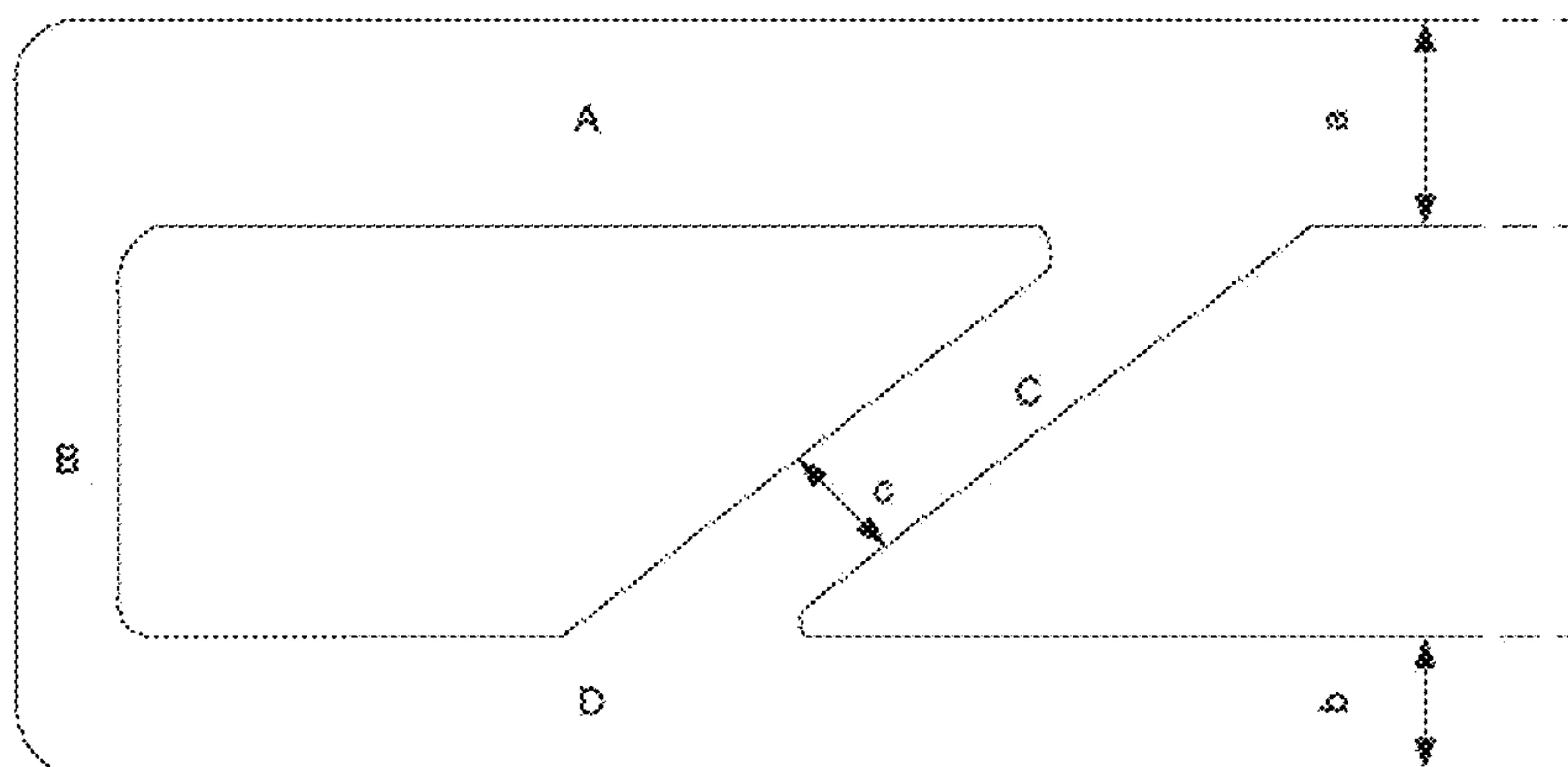
A: runway, B: exit, C: rapid exit, D: taxiway a ≈ 40m, b ≈ 20m and c ≈ 30m
