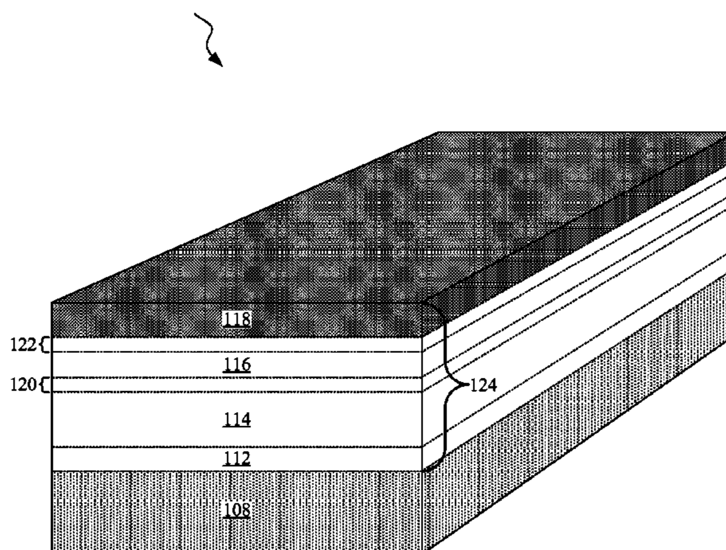
Alumina-Based Layer Structure On Stainless Steel Substrate
