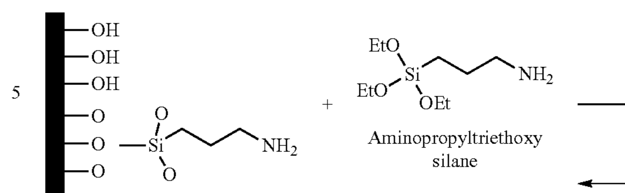
Step 1: Conversion of Glass to Amine-Terminated Glass
