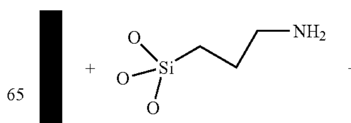
Step 2: Preparation of Active Ester
