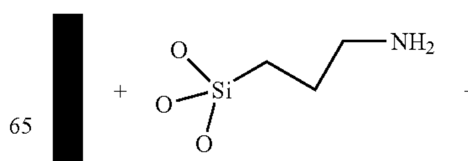
Step 2: Preparation of Active Ester
