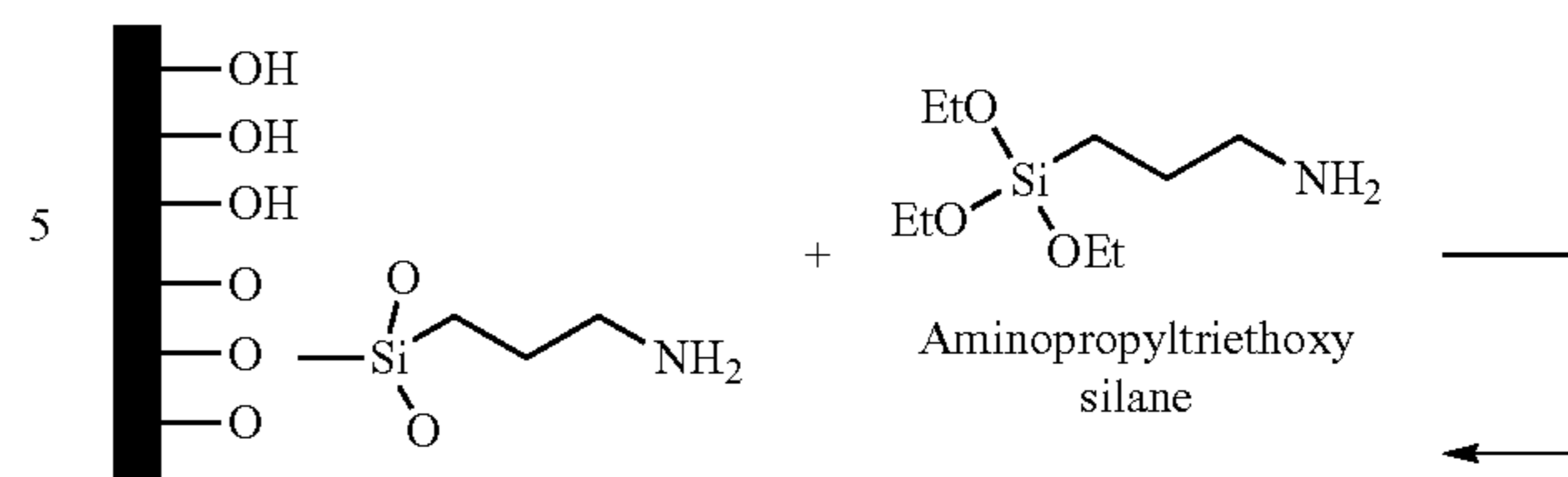
Step 1: Conversion of Glass to Amine-Terminated Glass
