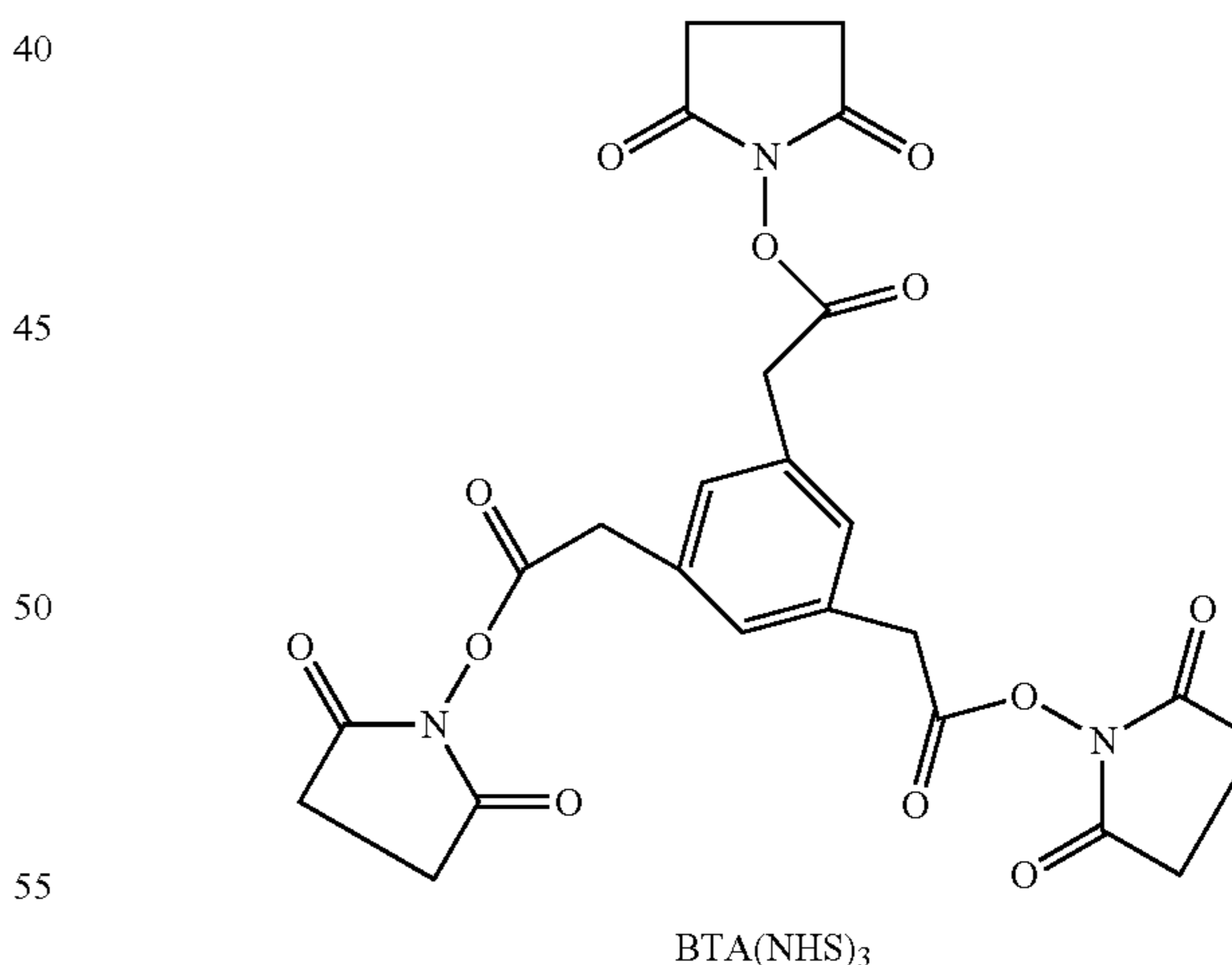
Step 2: Preparation of Active Ester
