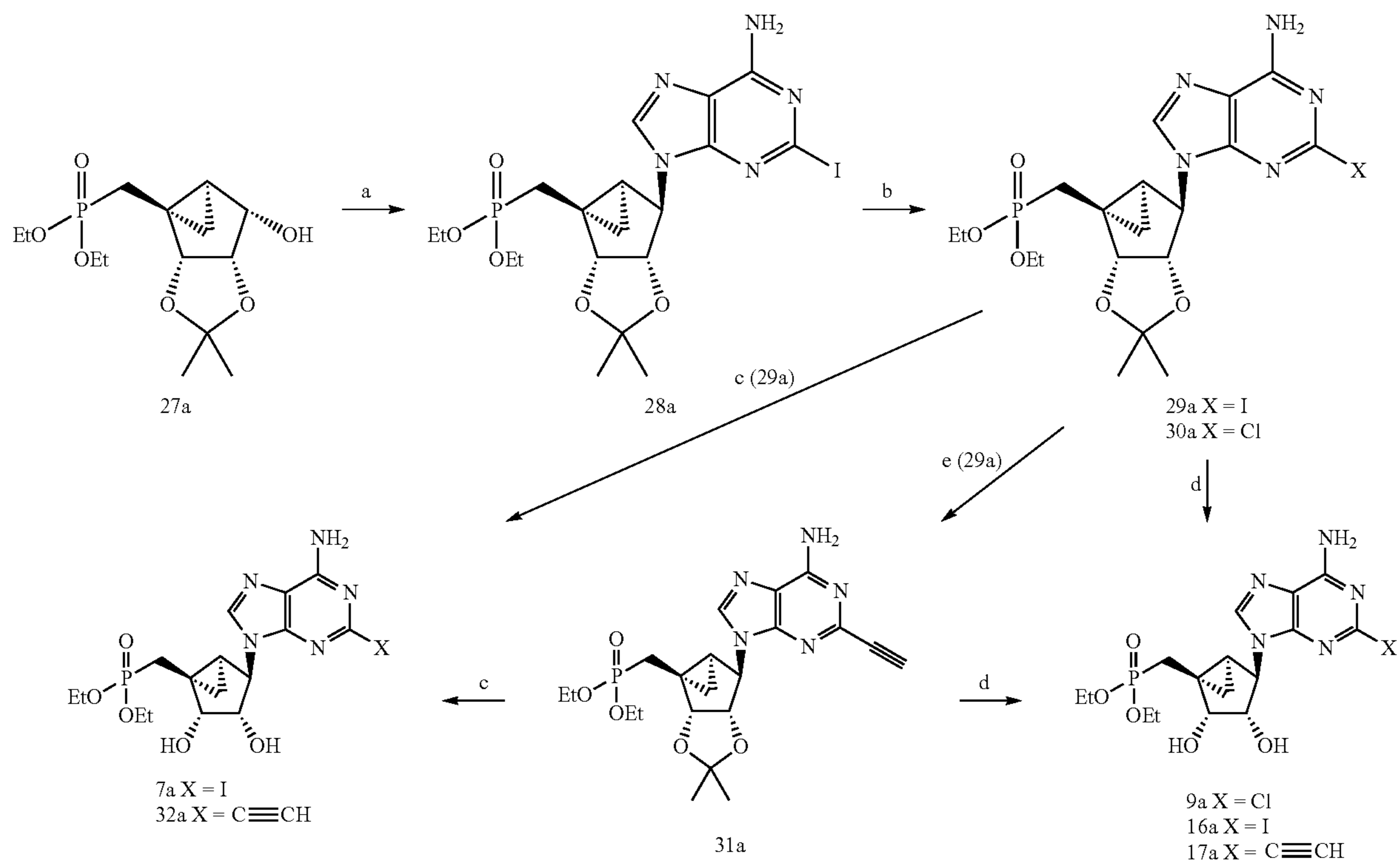
Scheme 3a
