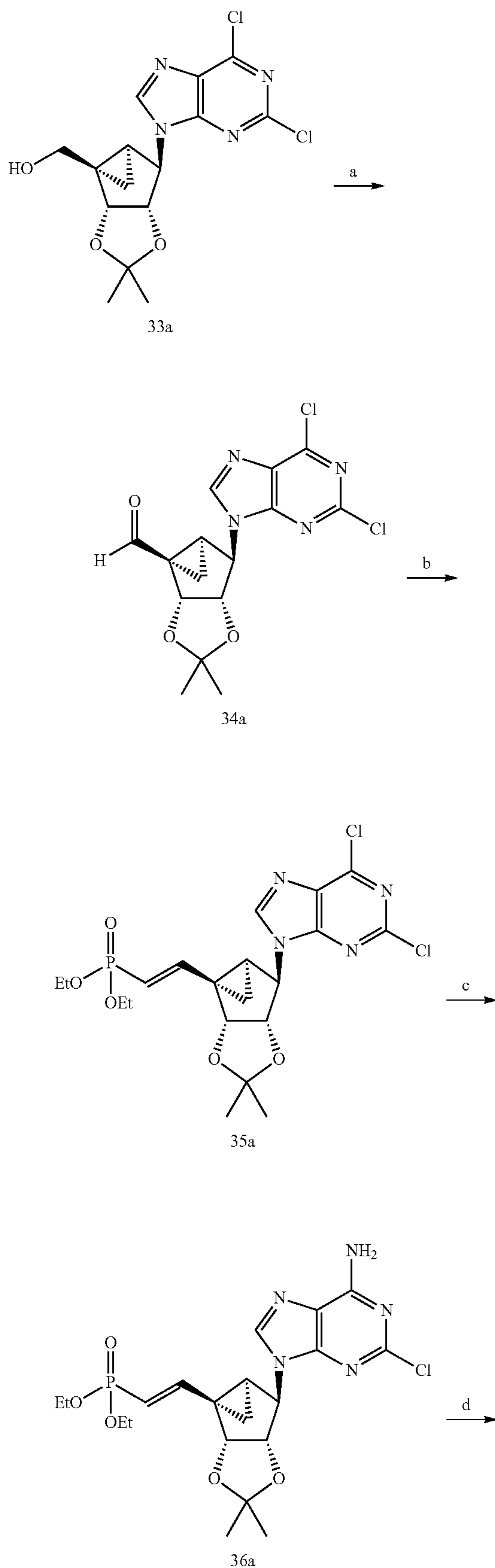
Scheme 4a
