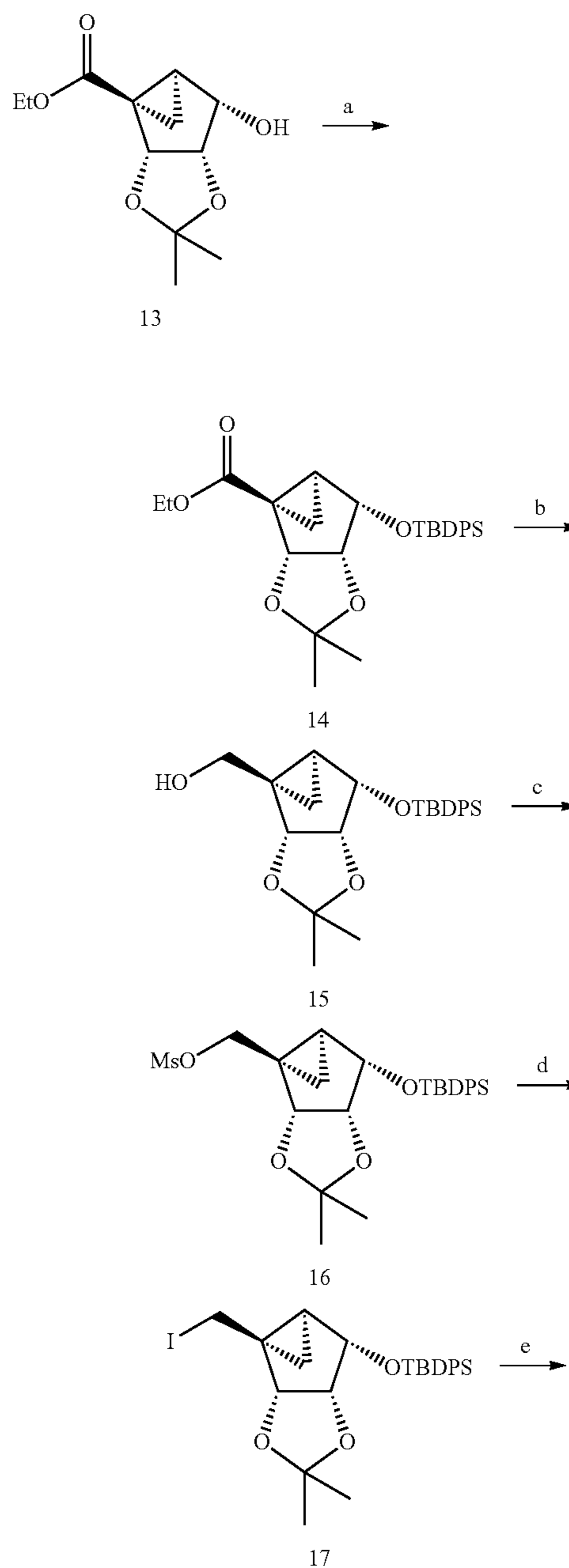
Scheme 1
