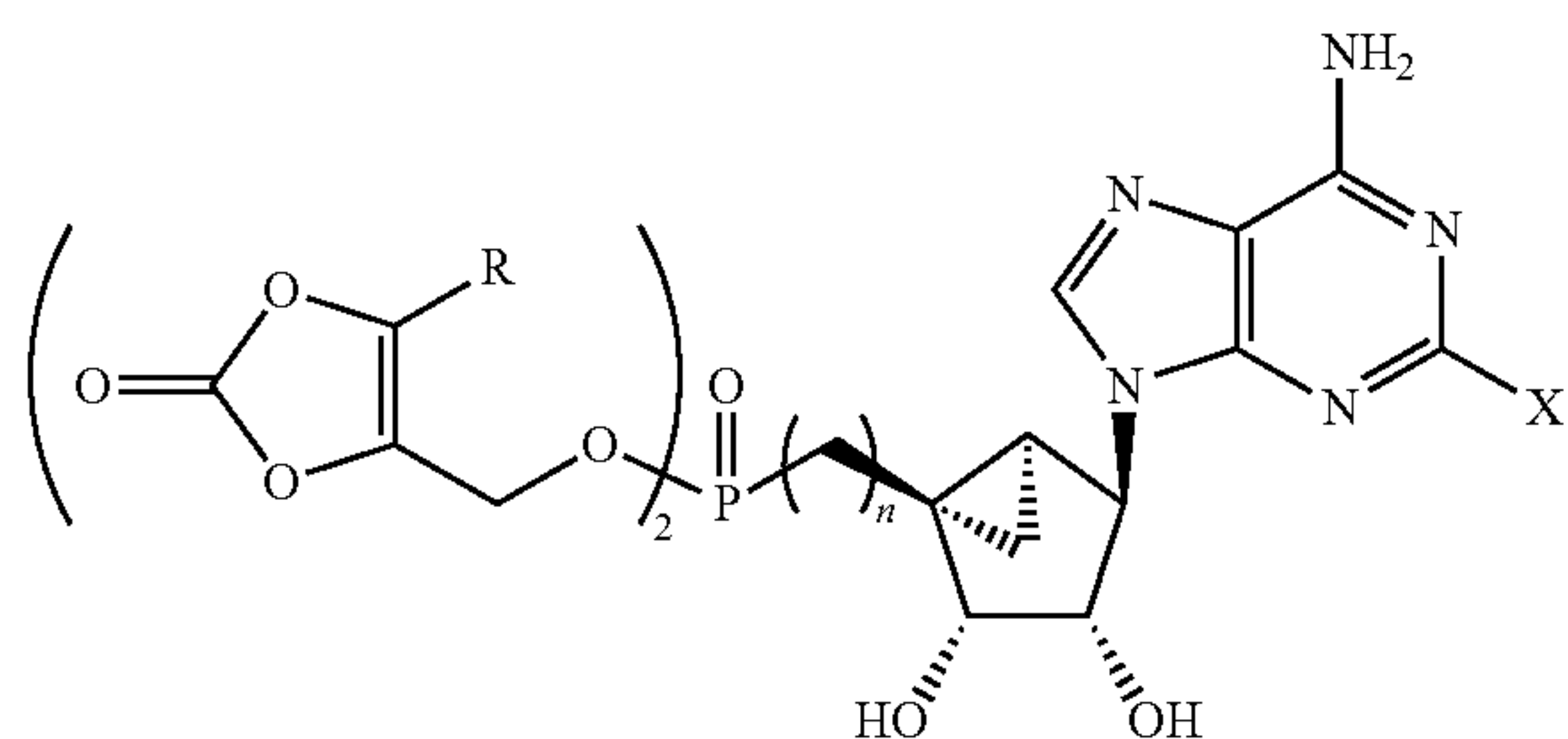
Dioxolenone Prodrugs 9 n = 1 or 2; X = any halogen R = alkyl or aryl
