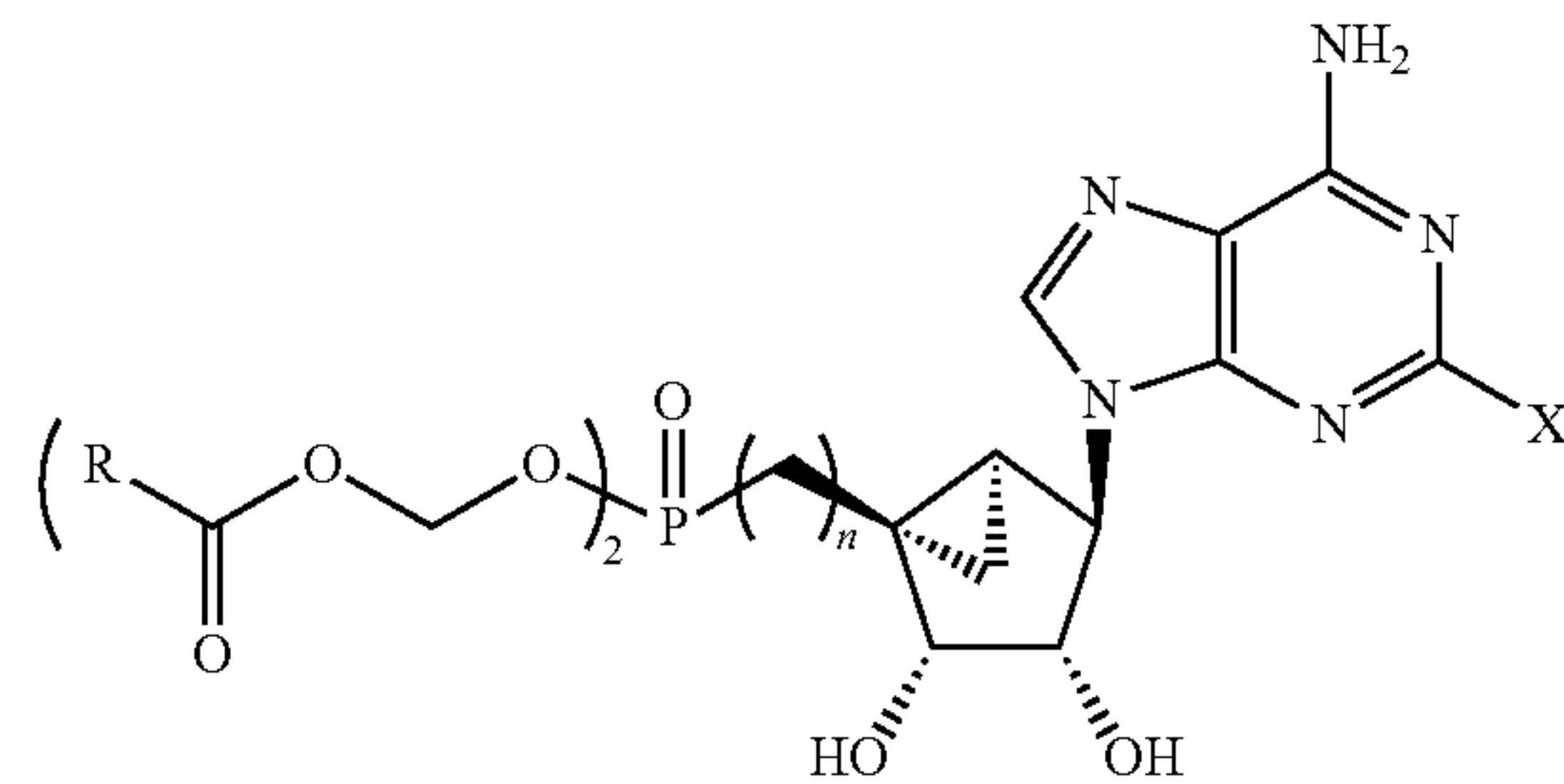
Acyloxyalkyl esters 4,5
