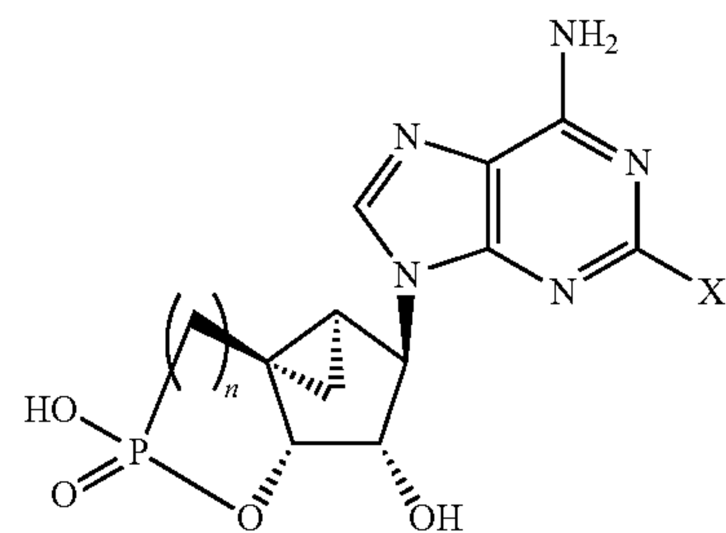
Cyclic prodrugs 6
