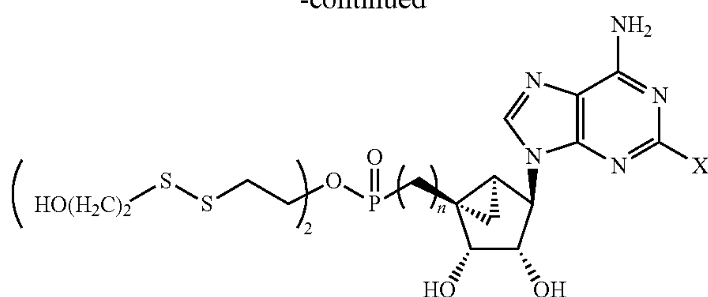
DTE (Dithioethanol) esters 8 n = 1 or 2; X = any halogen
