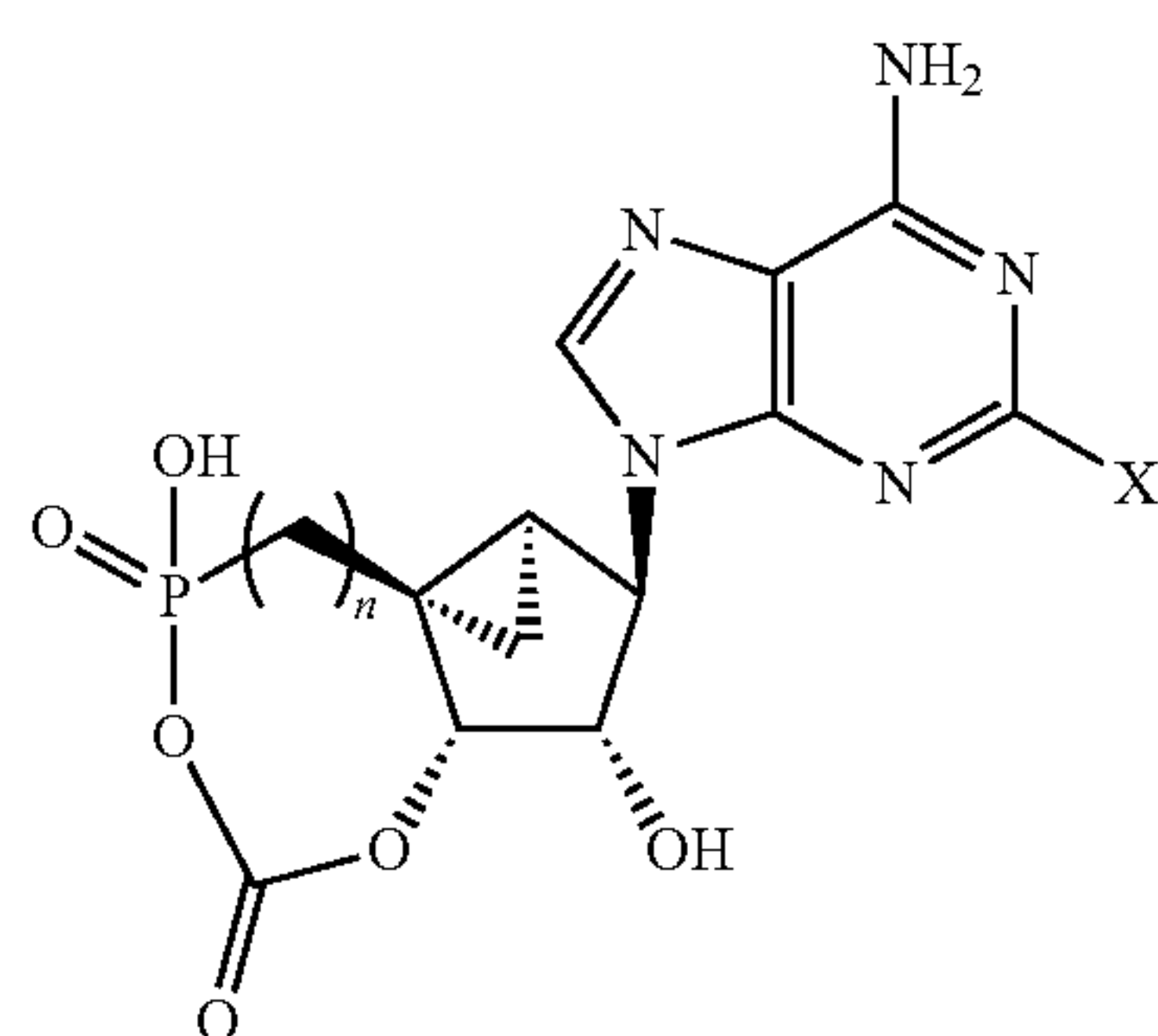
Cyclic prodrugs n = 1 or 2; X = any halogen
