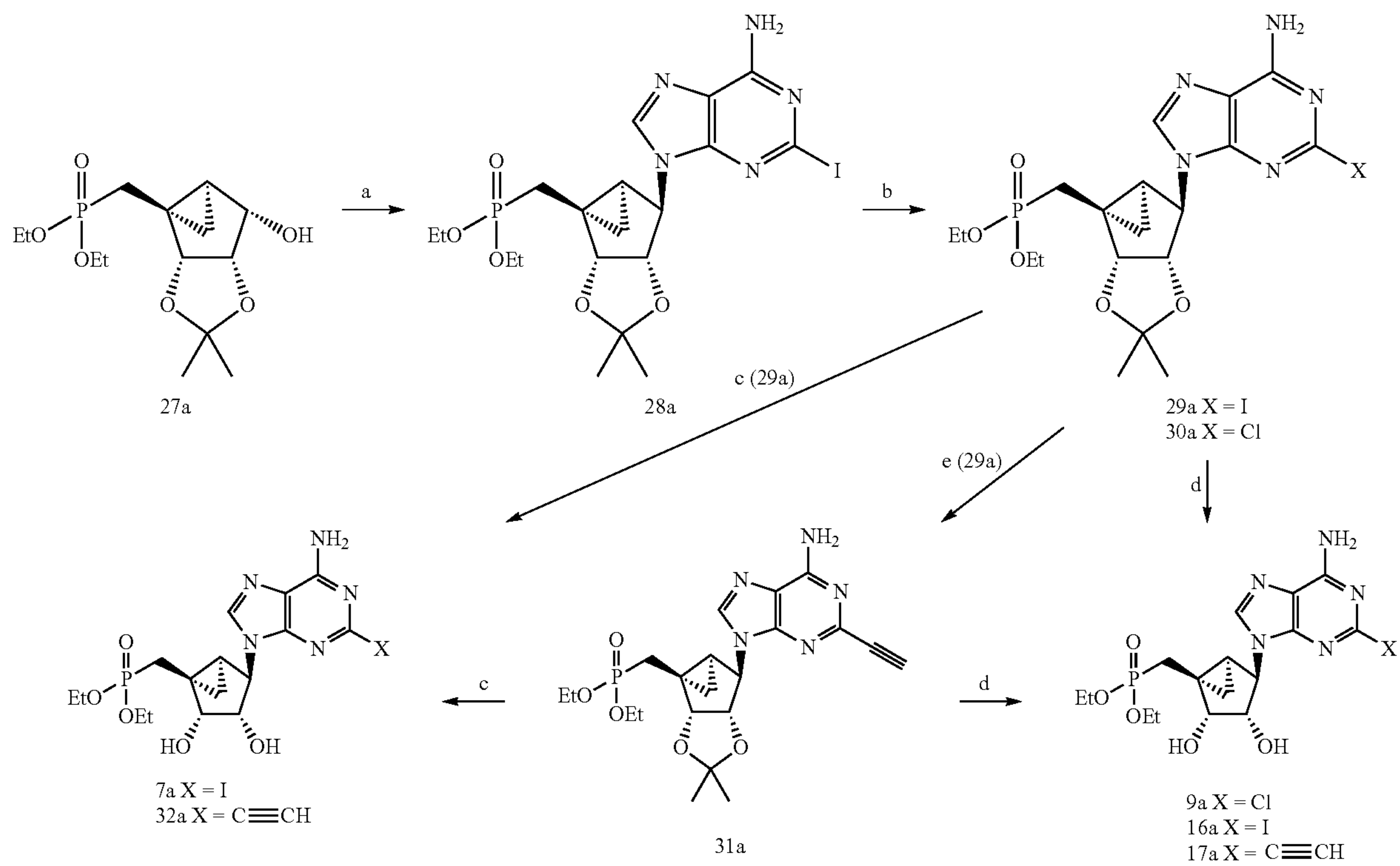
Scheme 3a
