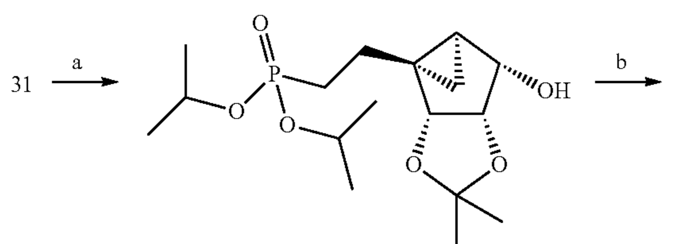
Scheme 5
