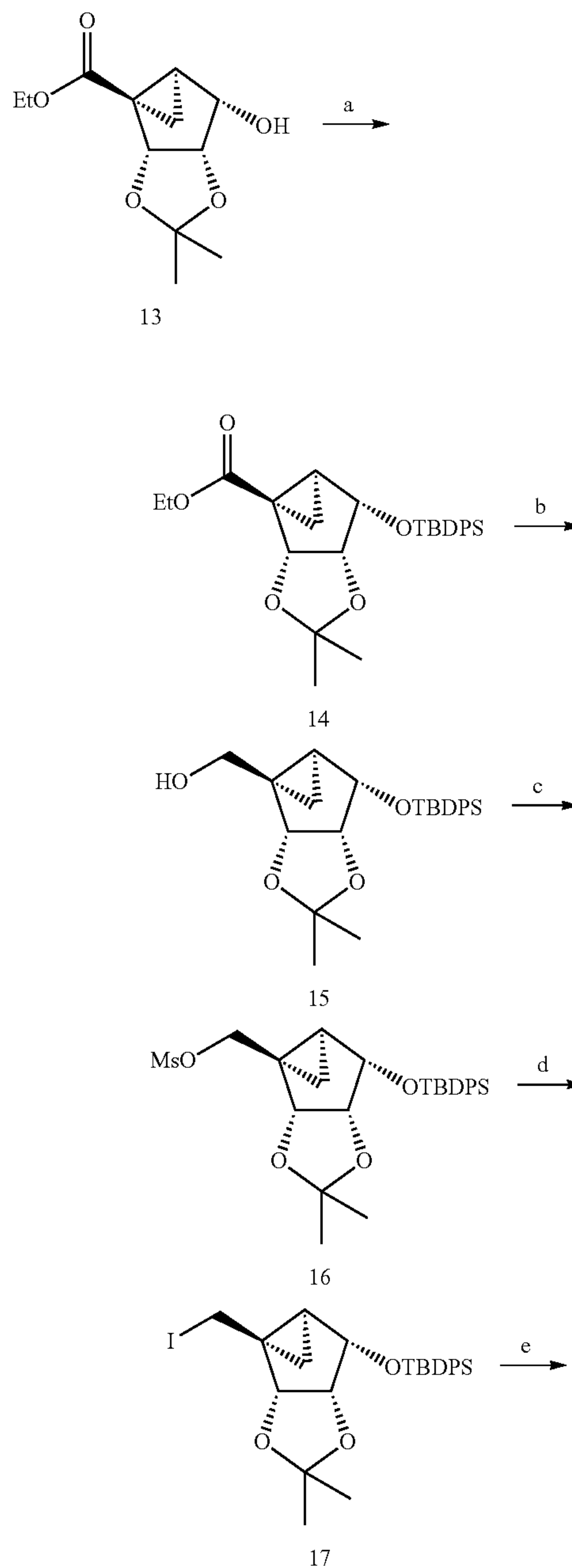
Scheme 1
