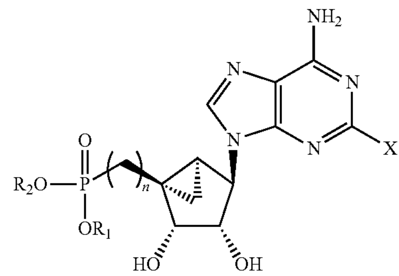
Alkyl or aryl ester prodrugs 1-3 n = 1 or 2; X = any halogen R 1 = R 2 = any alkyl or aryl groups R 1 = any alkyl or aryl groups; R 2 = H
