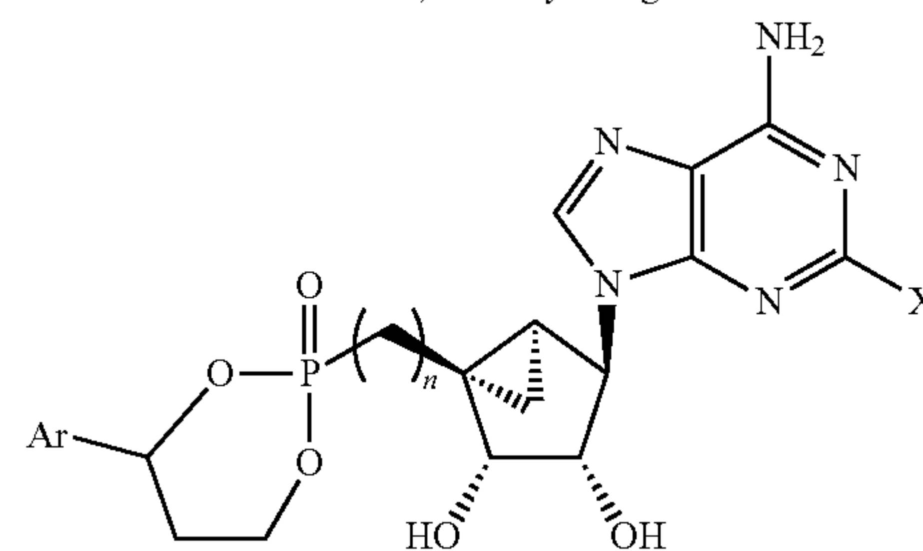
Cyclic 1-Ary-1,3-propanyl Ester 12 n = 1 or 2; X = any halogen
