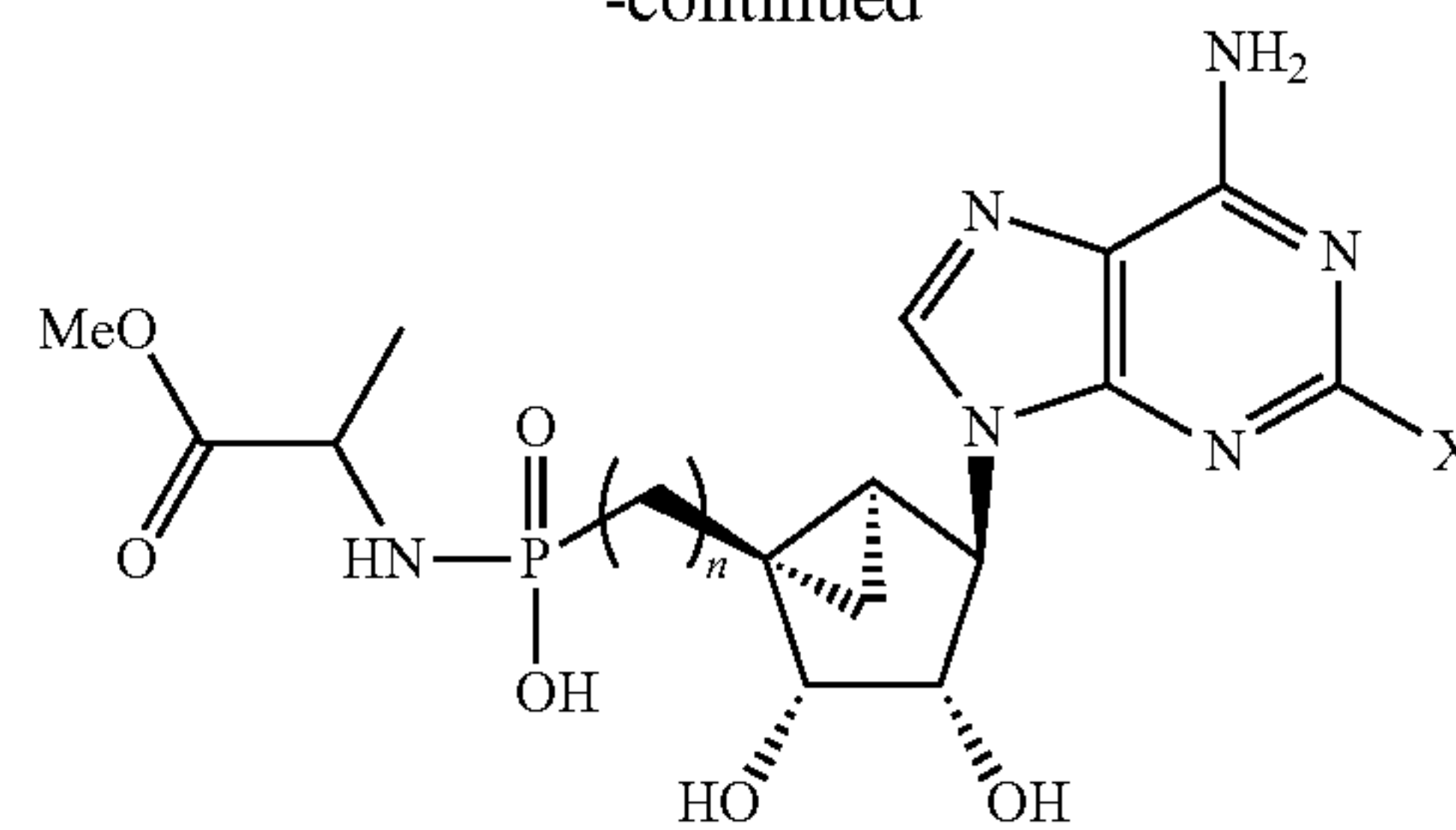
Phosphoramidate Monoesters 11 n = 1 or 2; X = any halogen
