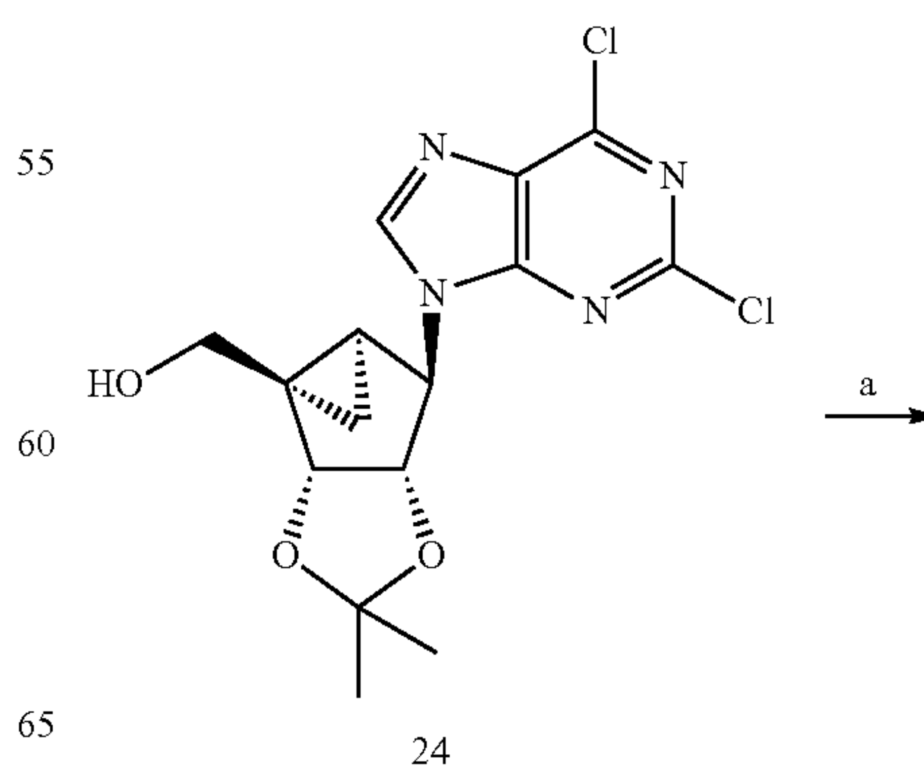
Scheme 3
