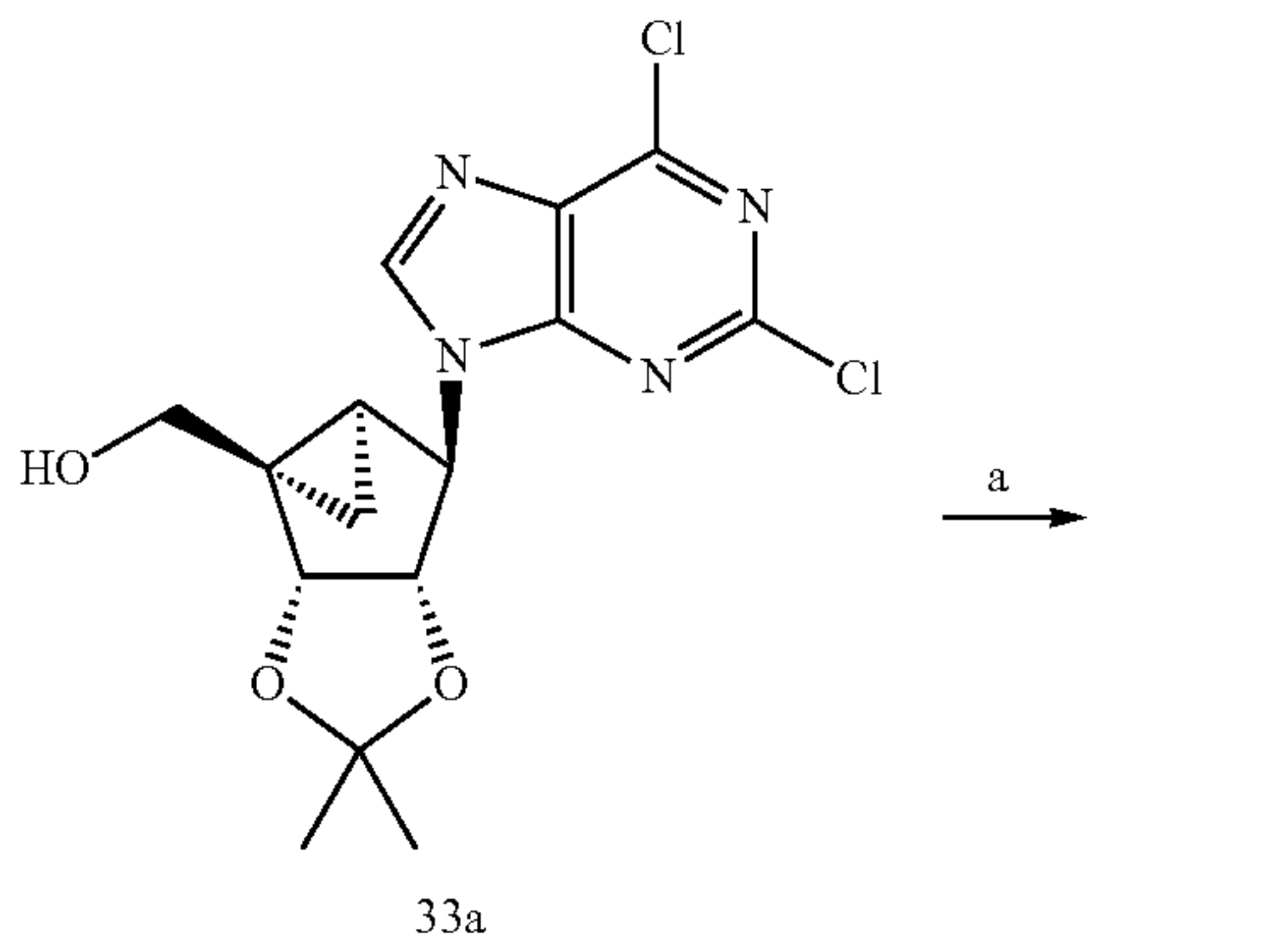
Scheme 4a
