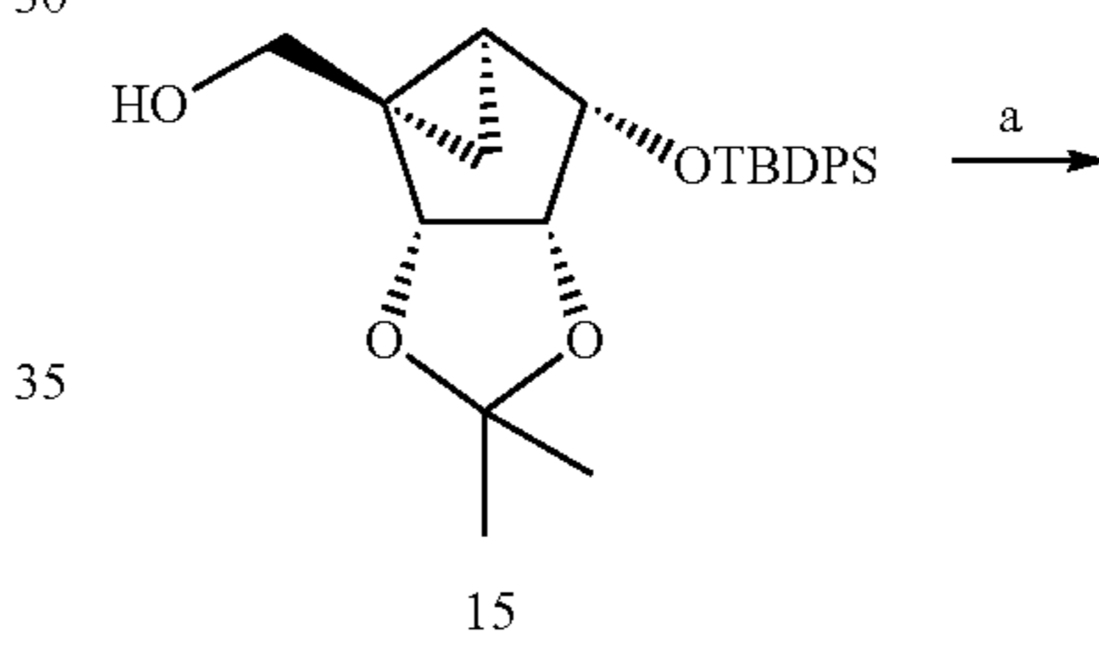
Scheme 6
