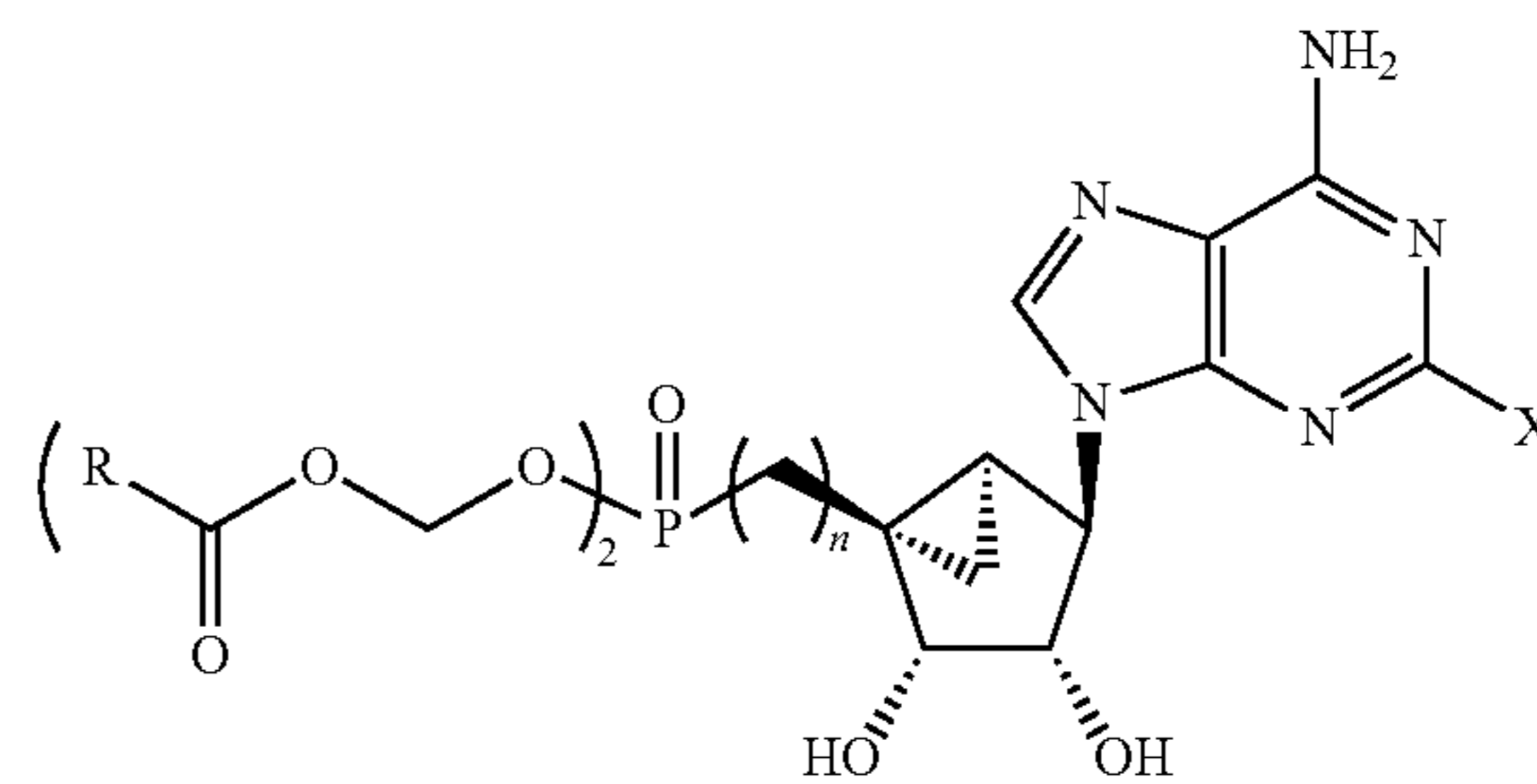
Acyloxyalkyl esters 4,5 n = 1 or 2; X = any halogen R = any alkyl or aryl groups
