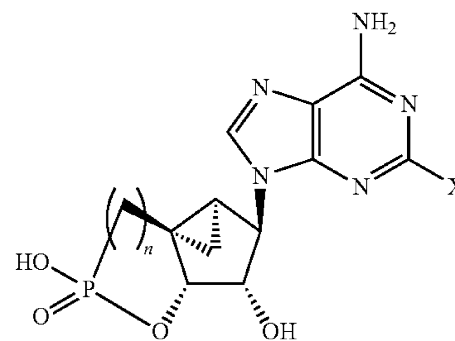
Cyclic prodrugs 6 n = 1 or 2; X = any halogen
