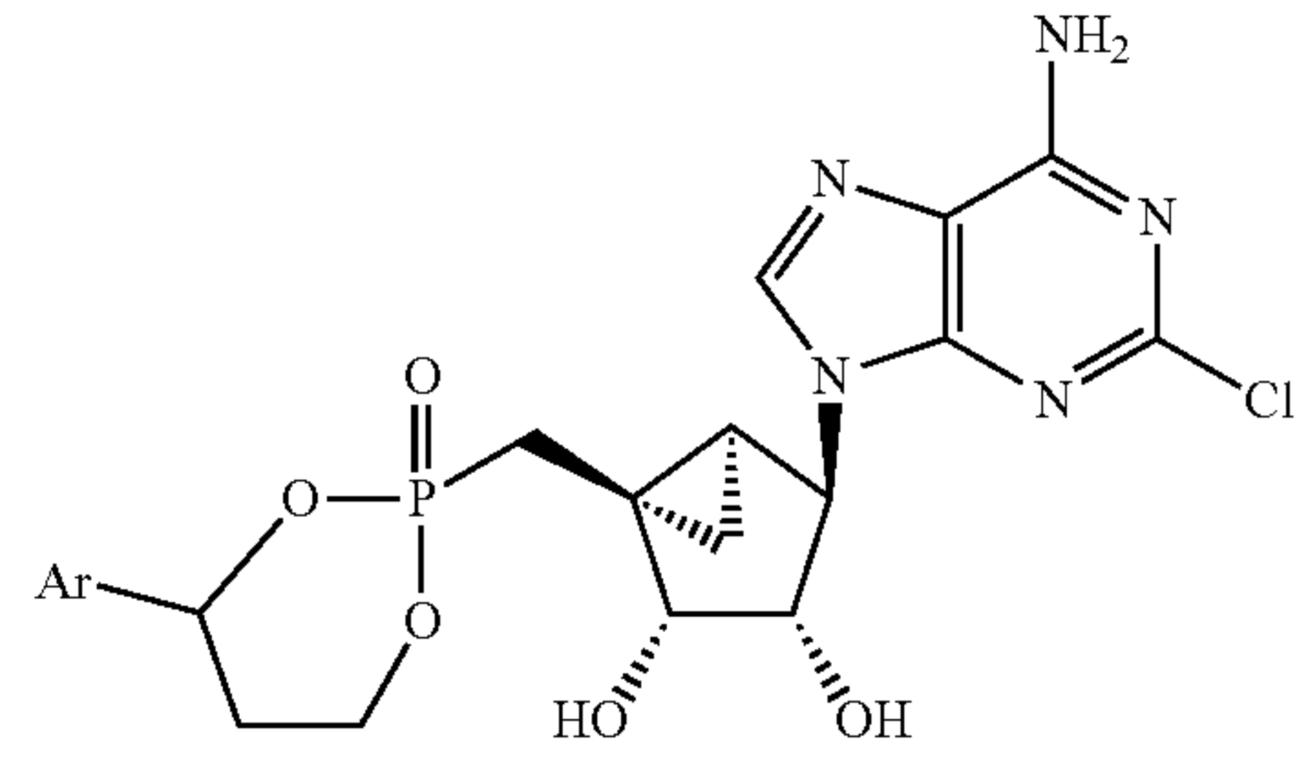
Cyclic 1-Ary-1,3-propanyl Ester
