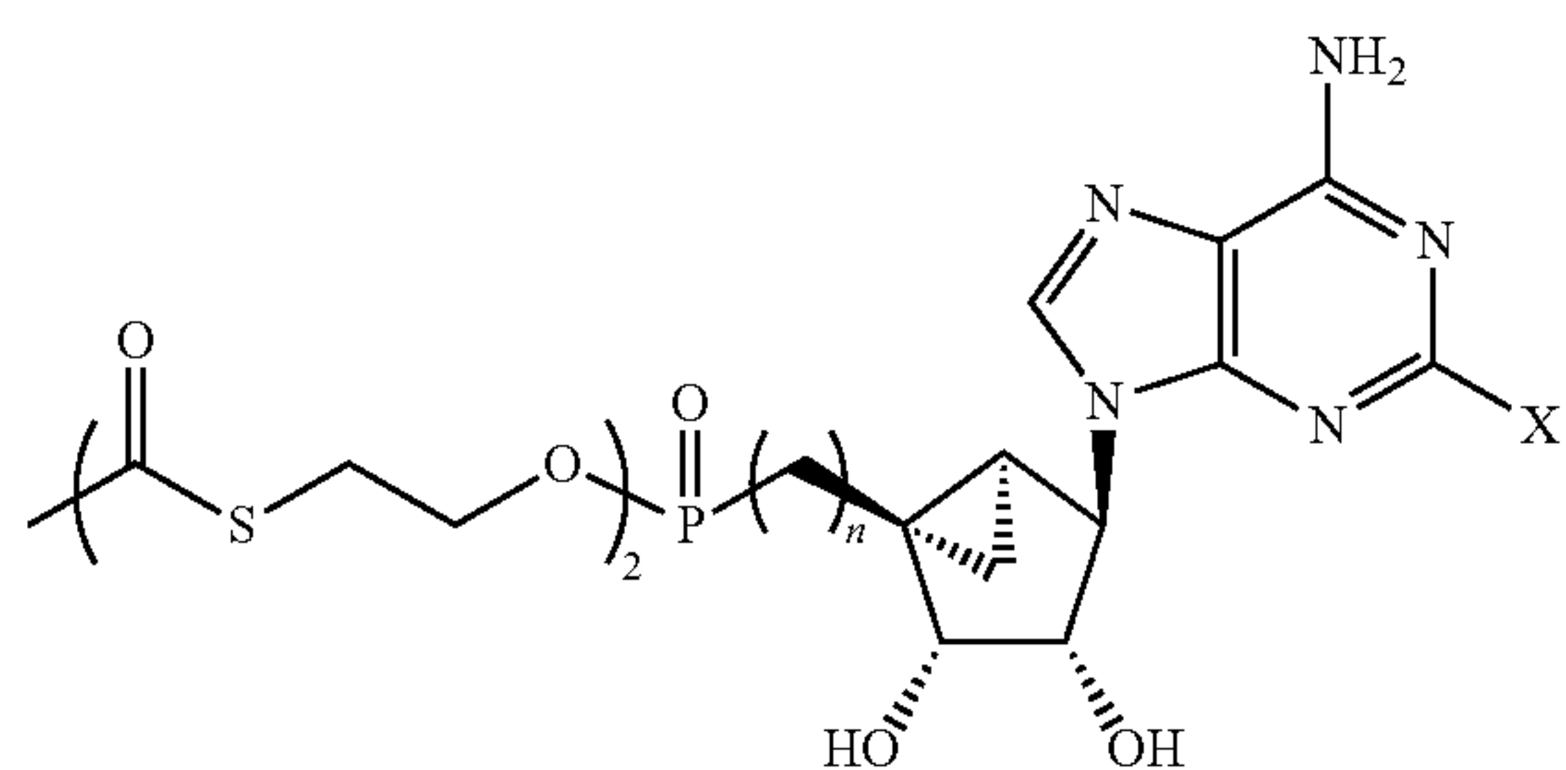
SATE (S-acetylthiethanol) esters 7,8 n = 1 or 2; X = any halogen
