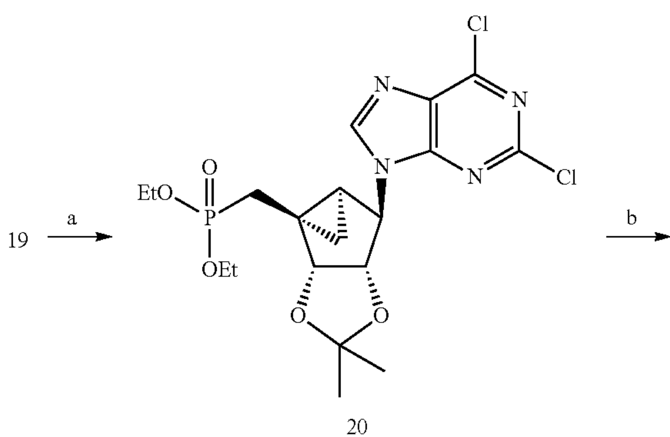
Scheme 2
