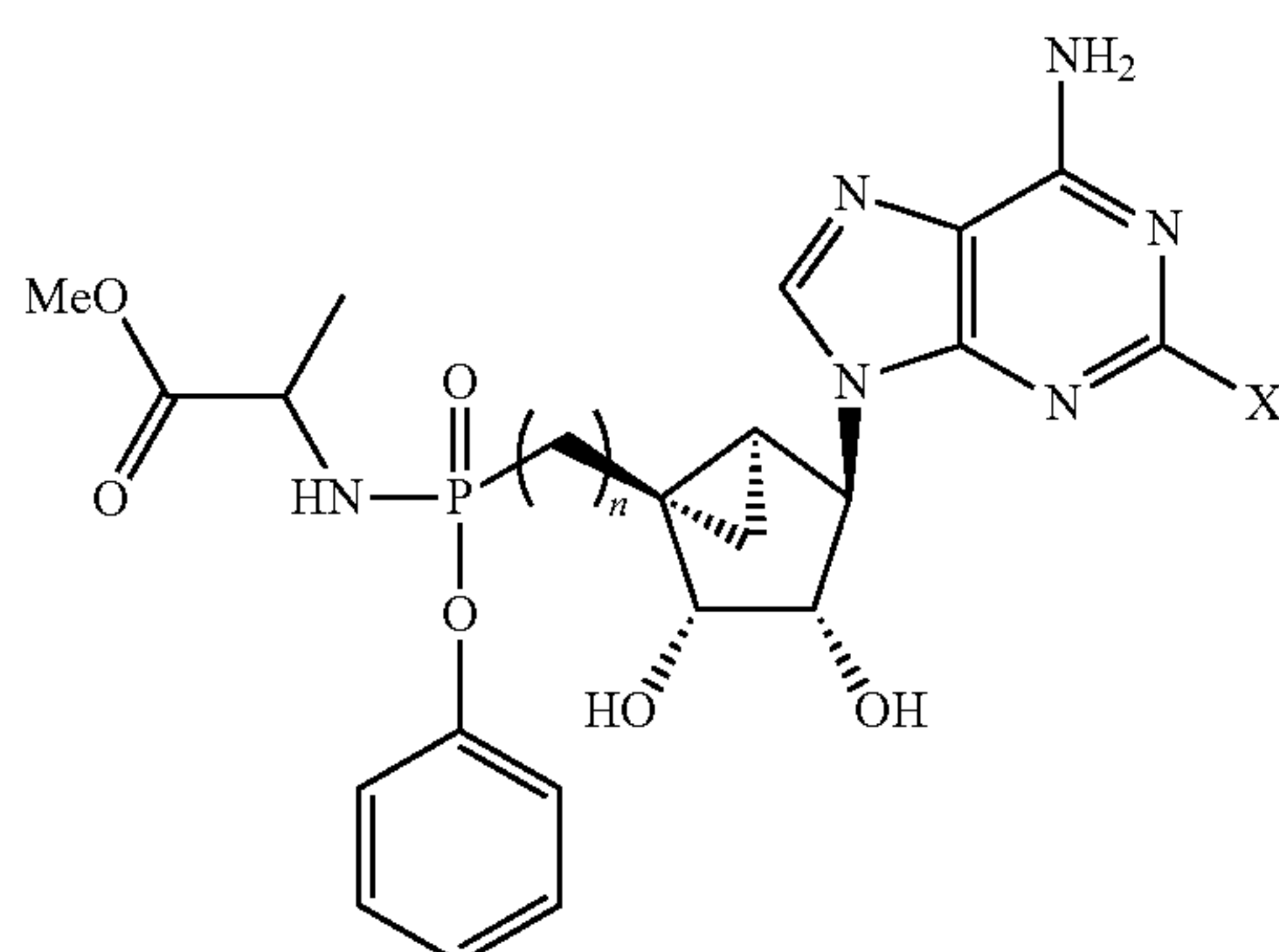
Aryl phosphoramidates 10 n = 1 or 2; X = any halogen
