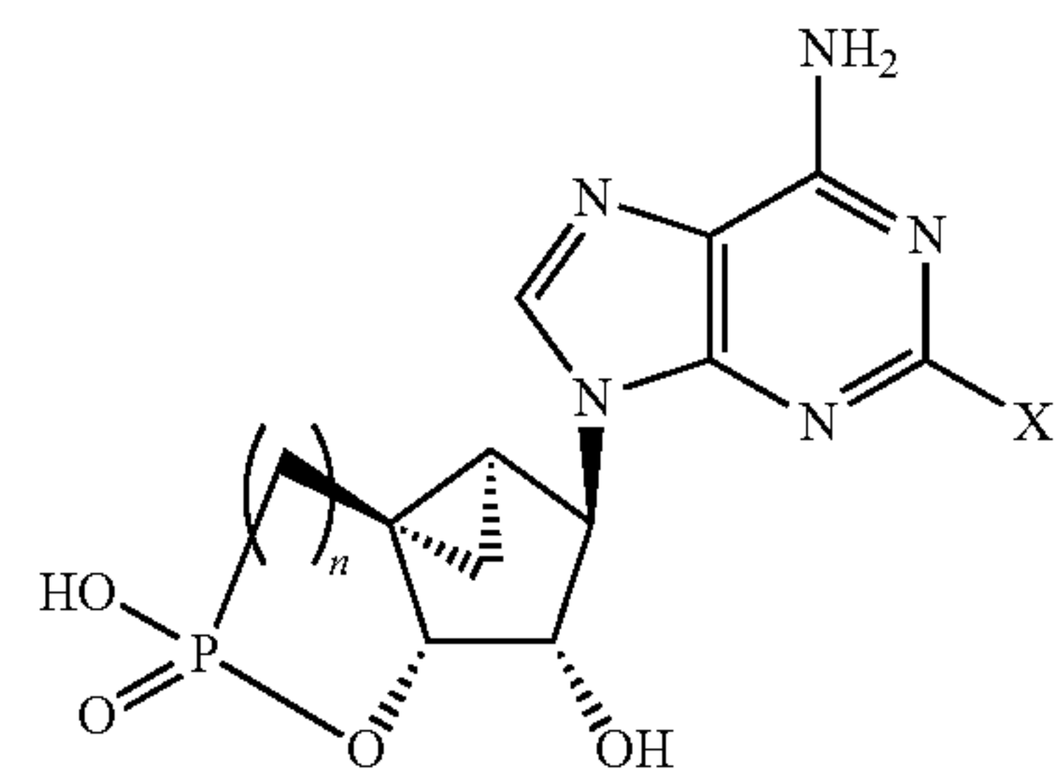
Cyclic prodrugs 6 n = 1 or 2; X = any halogen
