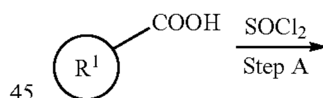
Scheme 7. Alternative route for the preparation of triazolopyrimidine compounds.
