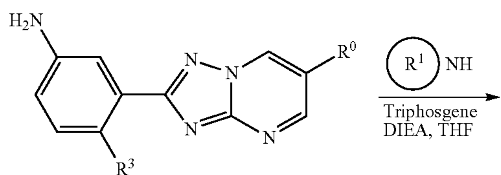
Scheme 4. Coupling of \text{—C(O)—R}^1 where \text{R}^1 is N-linked \text{C}_{4-6} heterocycloalkyl to the phenyl-triazolopyrimidine
