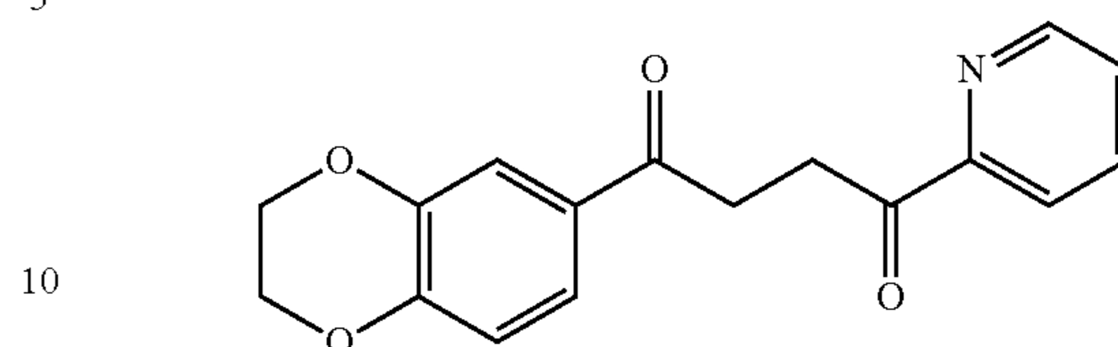
1-(2,3-dihydrobenzo[b][1,4]dioxin-6-yl)-4-(pyridin-2-yl)butane-1,4-dione 2
