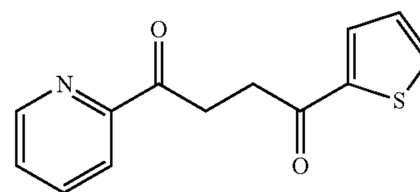
1-(pyridin-2-yl)-4-(thiophen-2-yl)butane-1,4-dione 5
