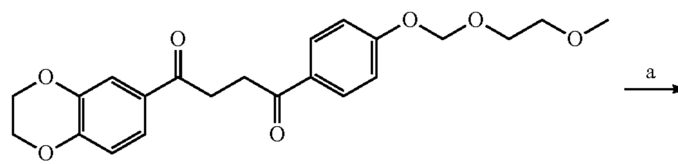
Scheme 6
