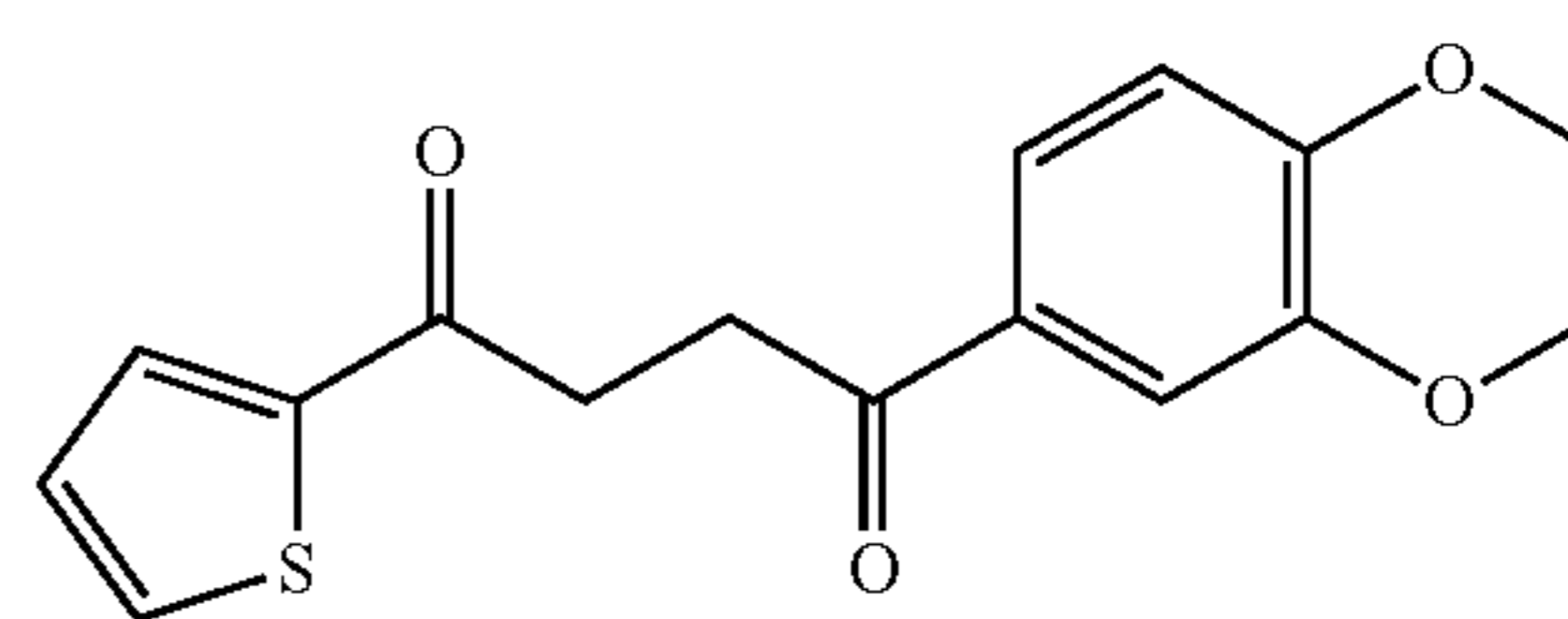
1-(2,3-dihydrobenzo[b][1,4]dioxin-6-yl)-4-(thiophen-2-yl)butane-1,4-dione 3
