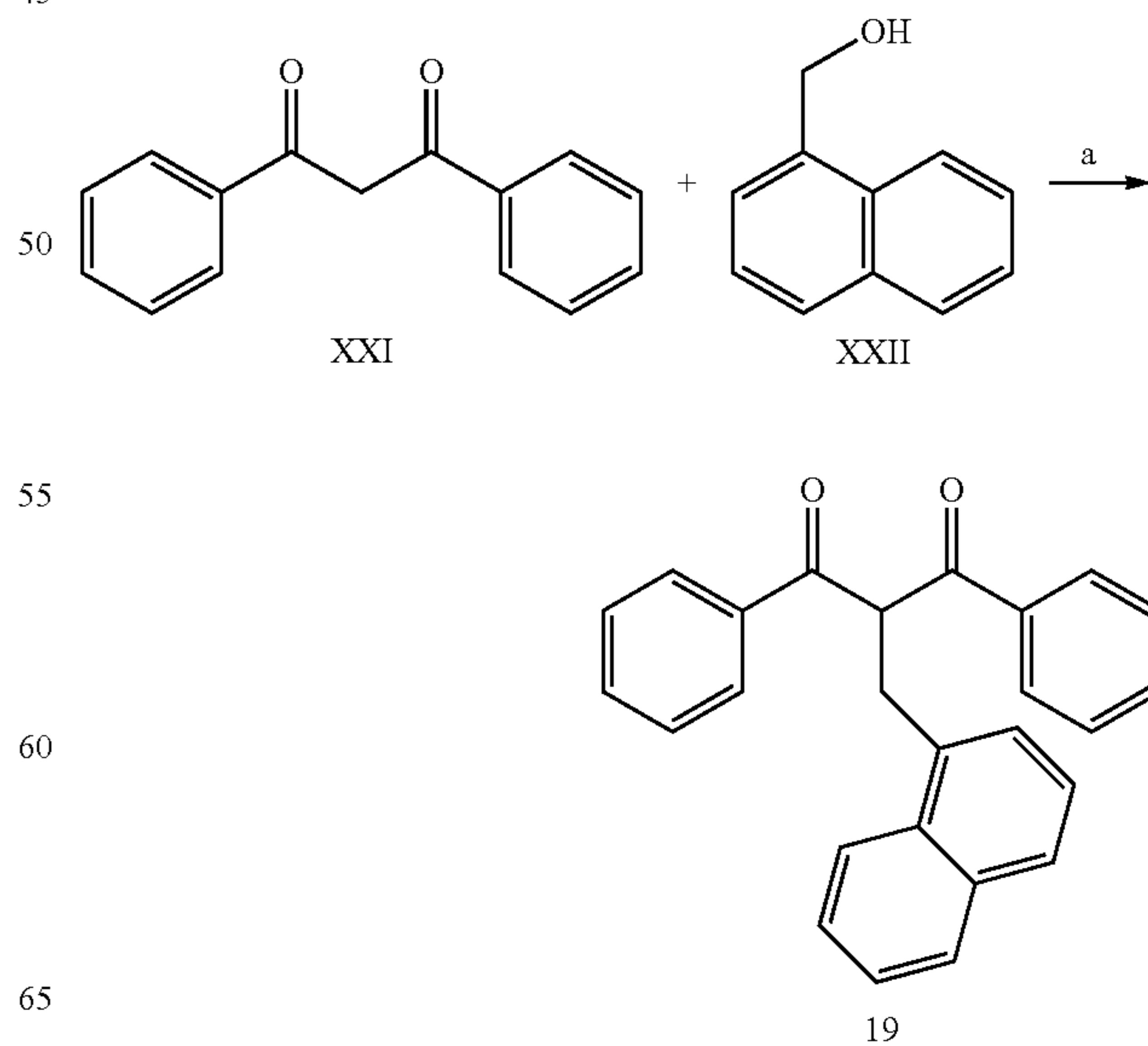
Scheme 10
