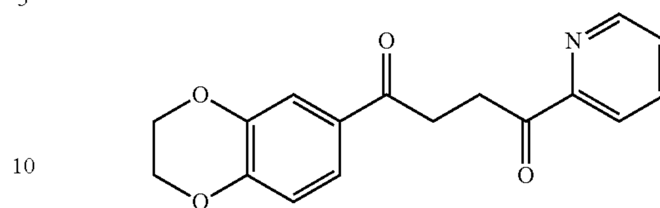
1-(2,3-dihydrobenzo[b][1,4]dioxin-6-yl)-4-(pyridin-2-yl)butane-1,4-dione 2
