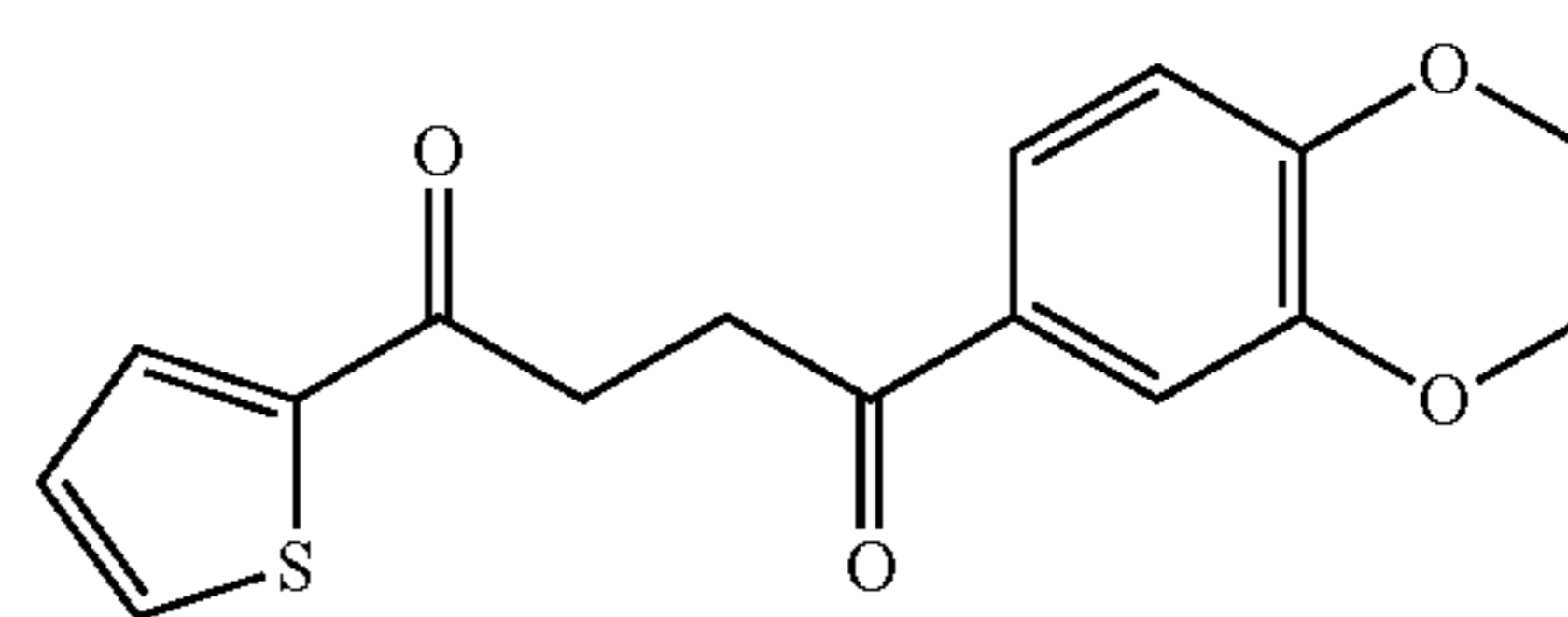
1-(2,3-dihydrobenzo[b][1,4]dioxin-6-yl)-4-(thiophen-2-yl)butane-1,4-dione 3
