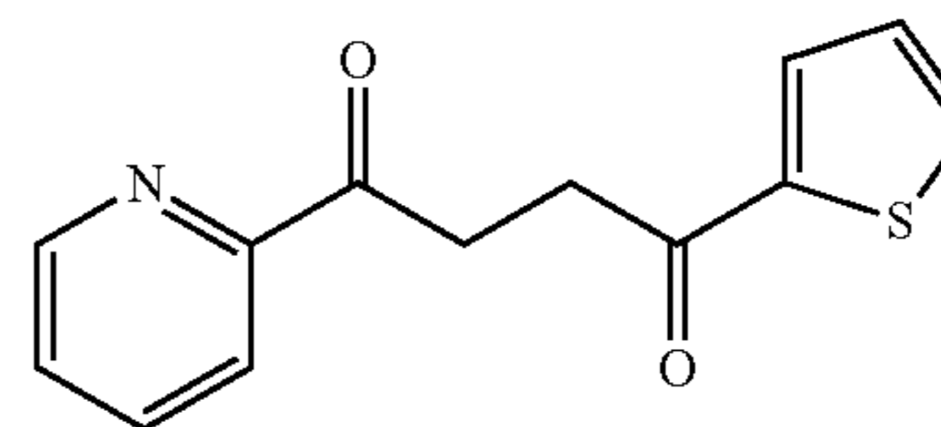
1-(pyridin-2-yl)-4-(thiophen-2-yl)butane-1,4-dione 5
