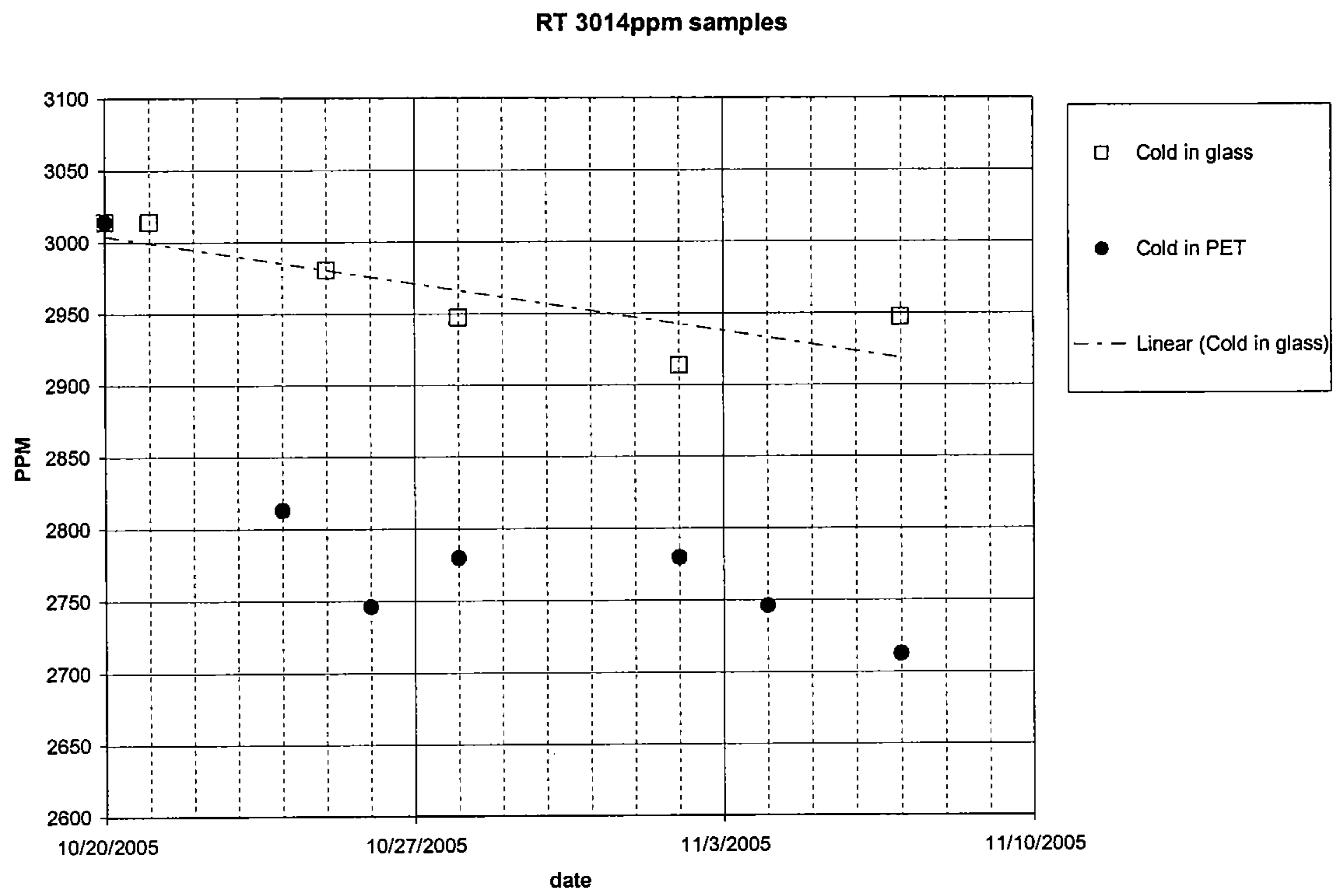
Figure 6 – Solutions Stored In PET Bottles
