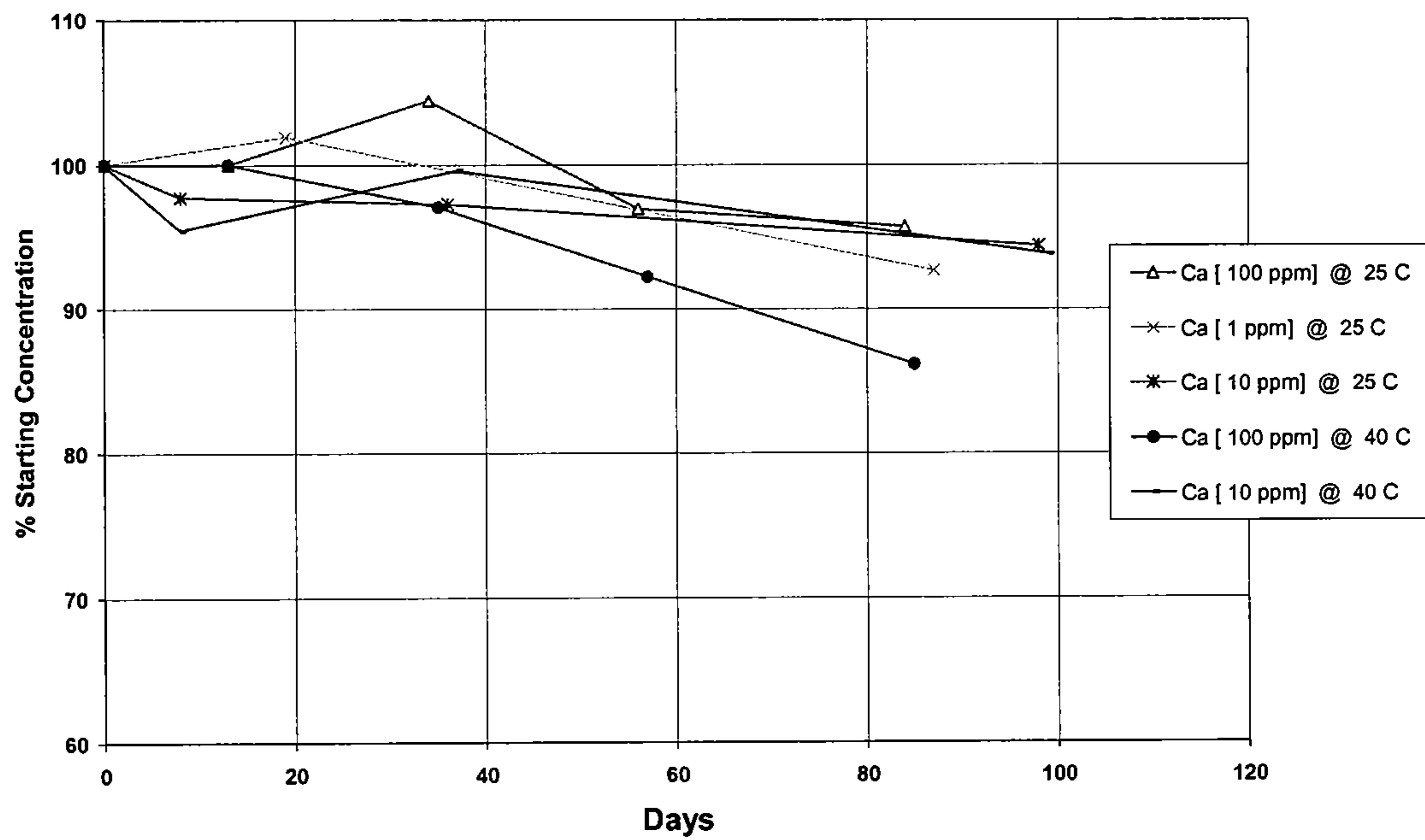
Figure 8 - Low Levels of CaCl2 in Deionized Water
