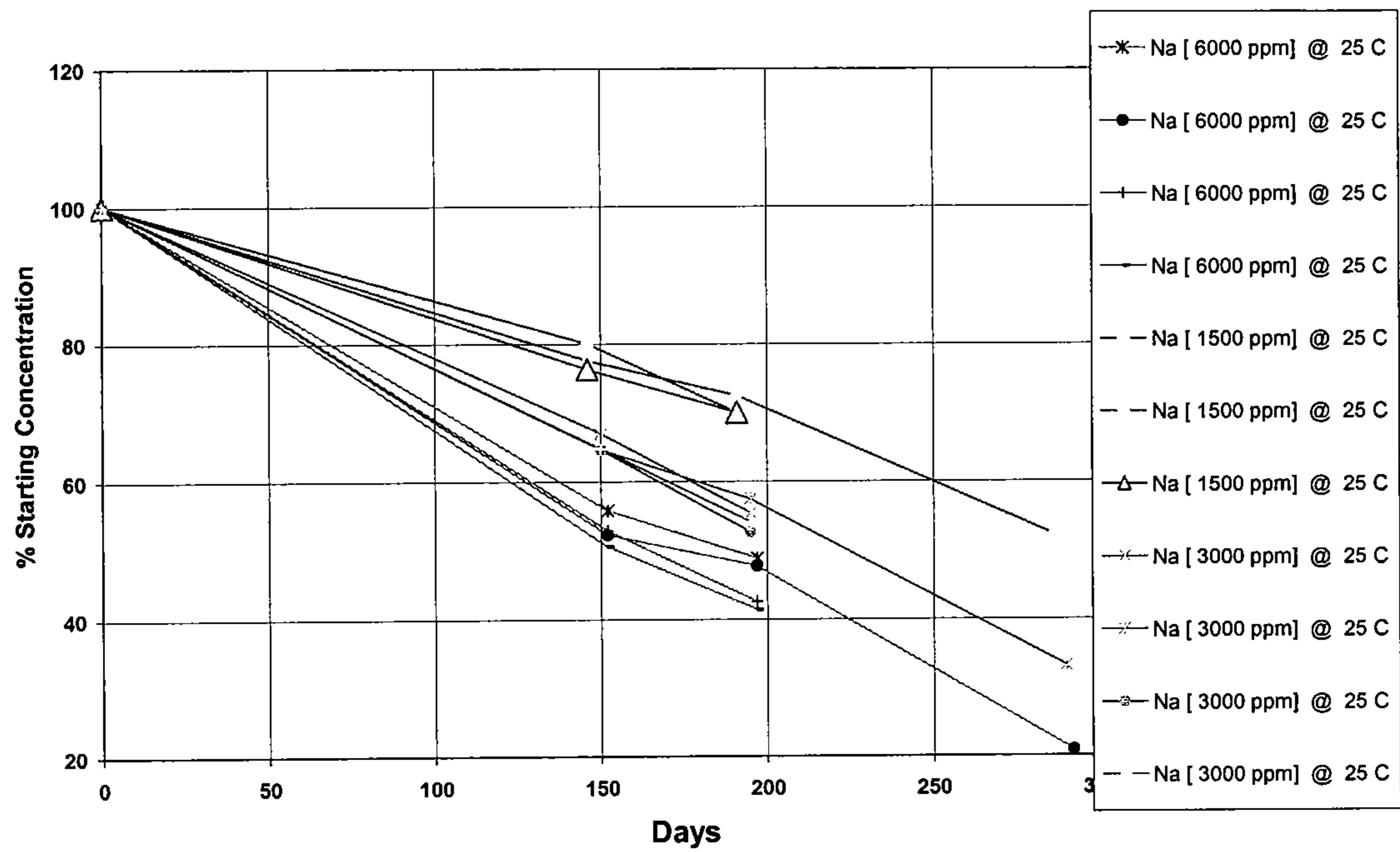
Figure 4 - High Levels of NaCl in Deionized Water
