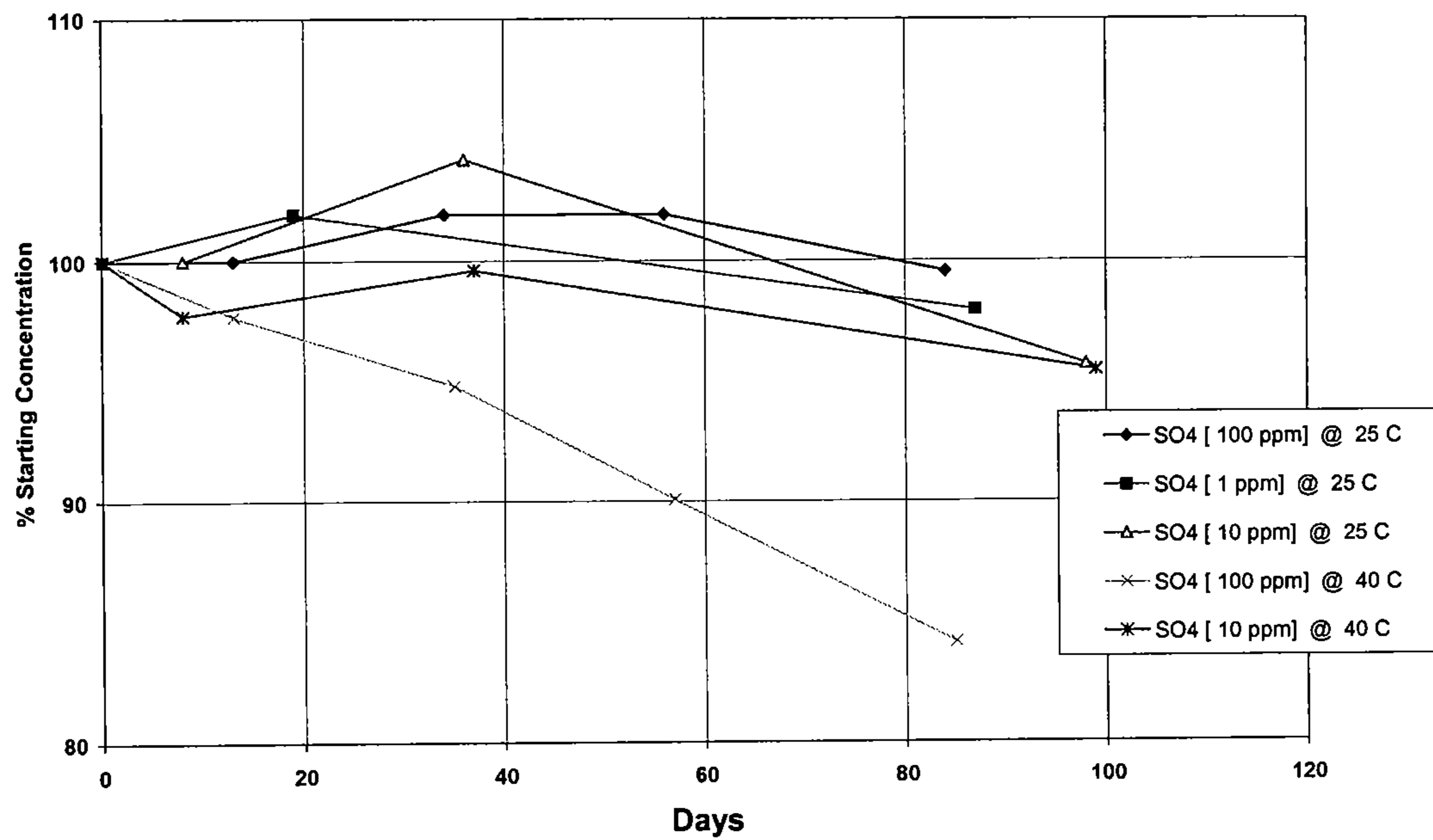
Figure 9 -Low Levels of Na 2 SO 4 in Deionized Water
