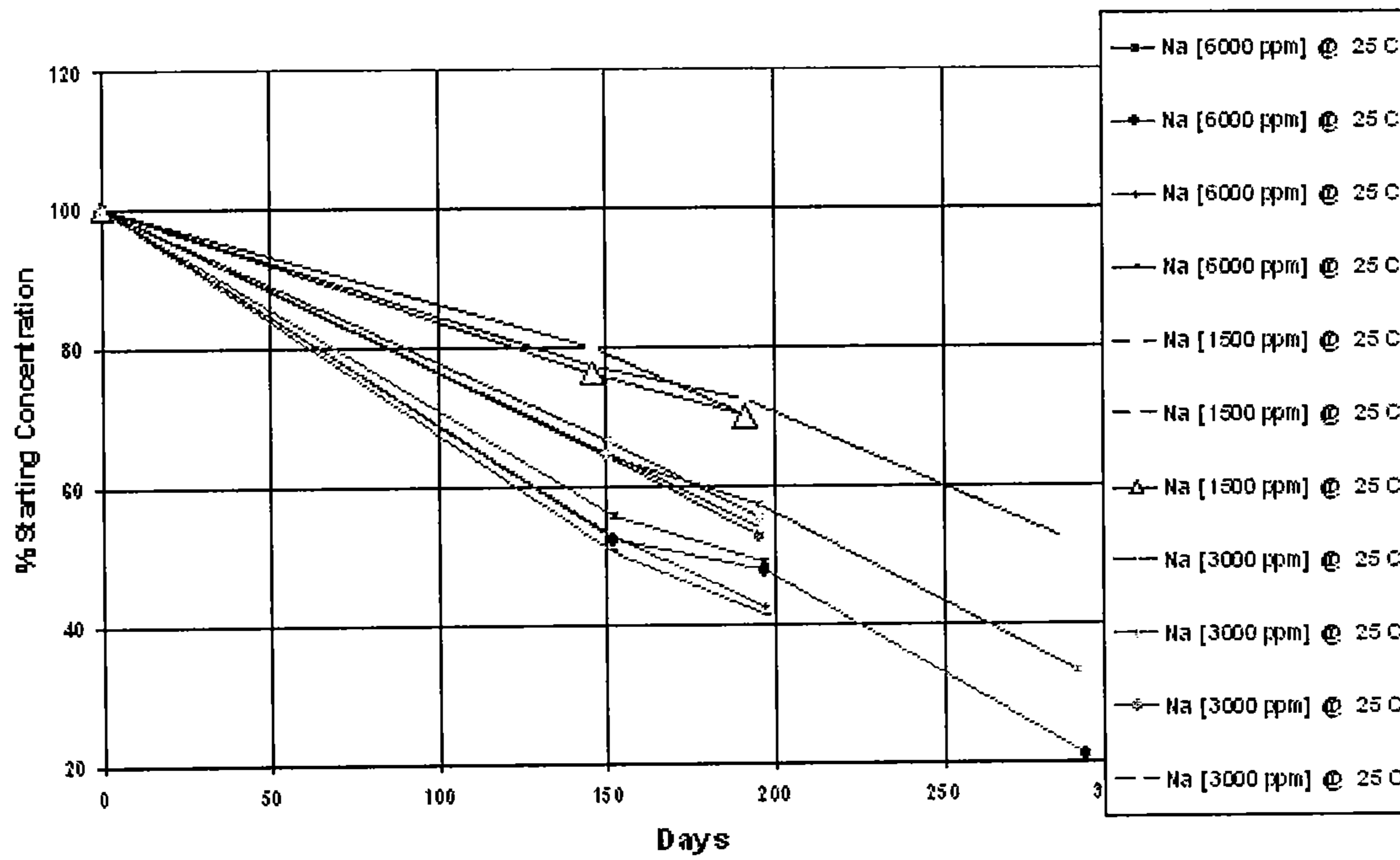
Figure 3: ClO 2 Stability In Glass Bottles Beginning At 3000 ppm
