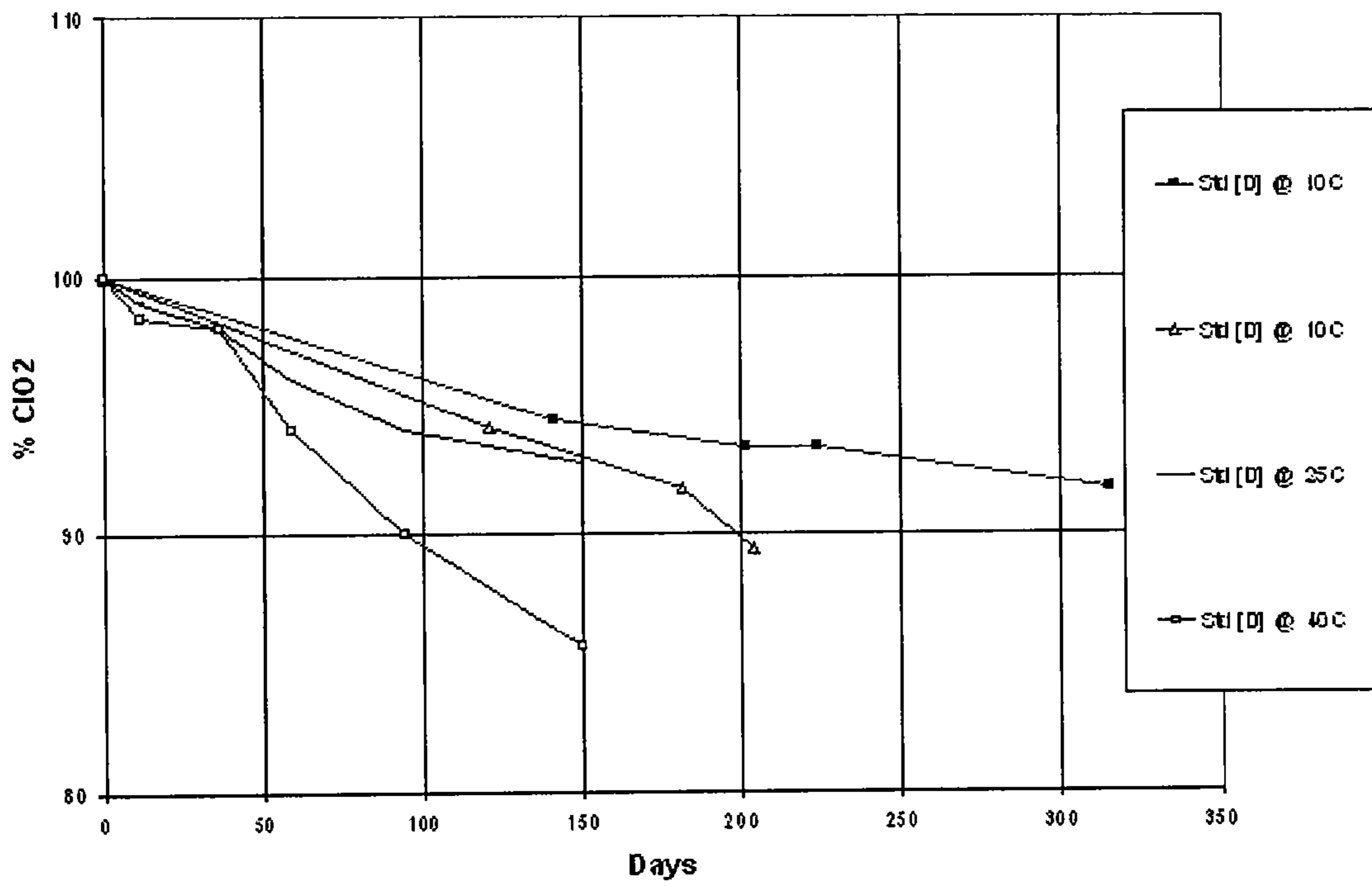
Figure 2: ClO 2 Stability In Glass Bottles Beginning At 4500 ppm
