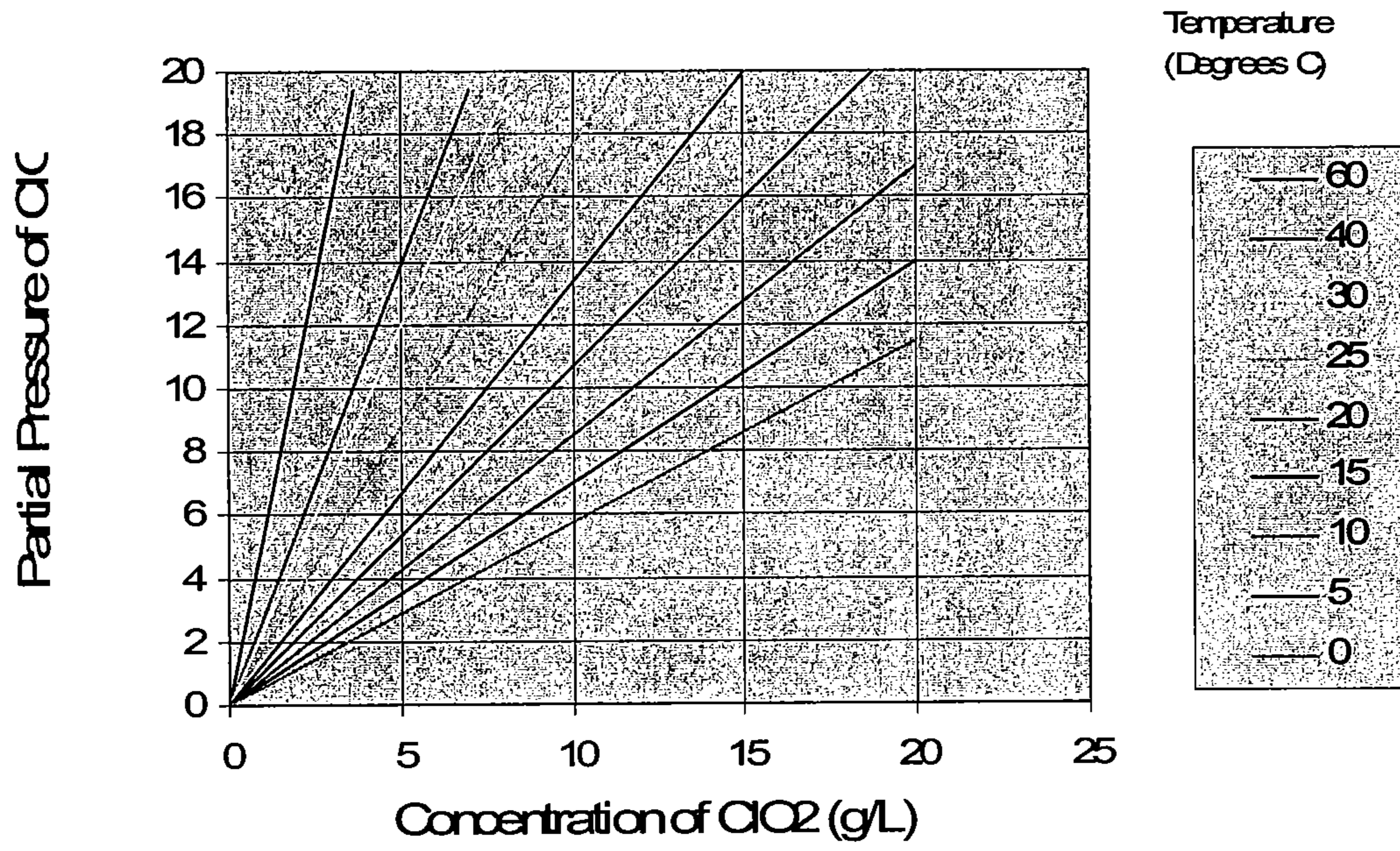
Figure 1 - Solubility of Chlorine Dioxide in Water
