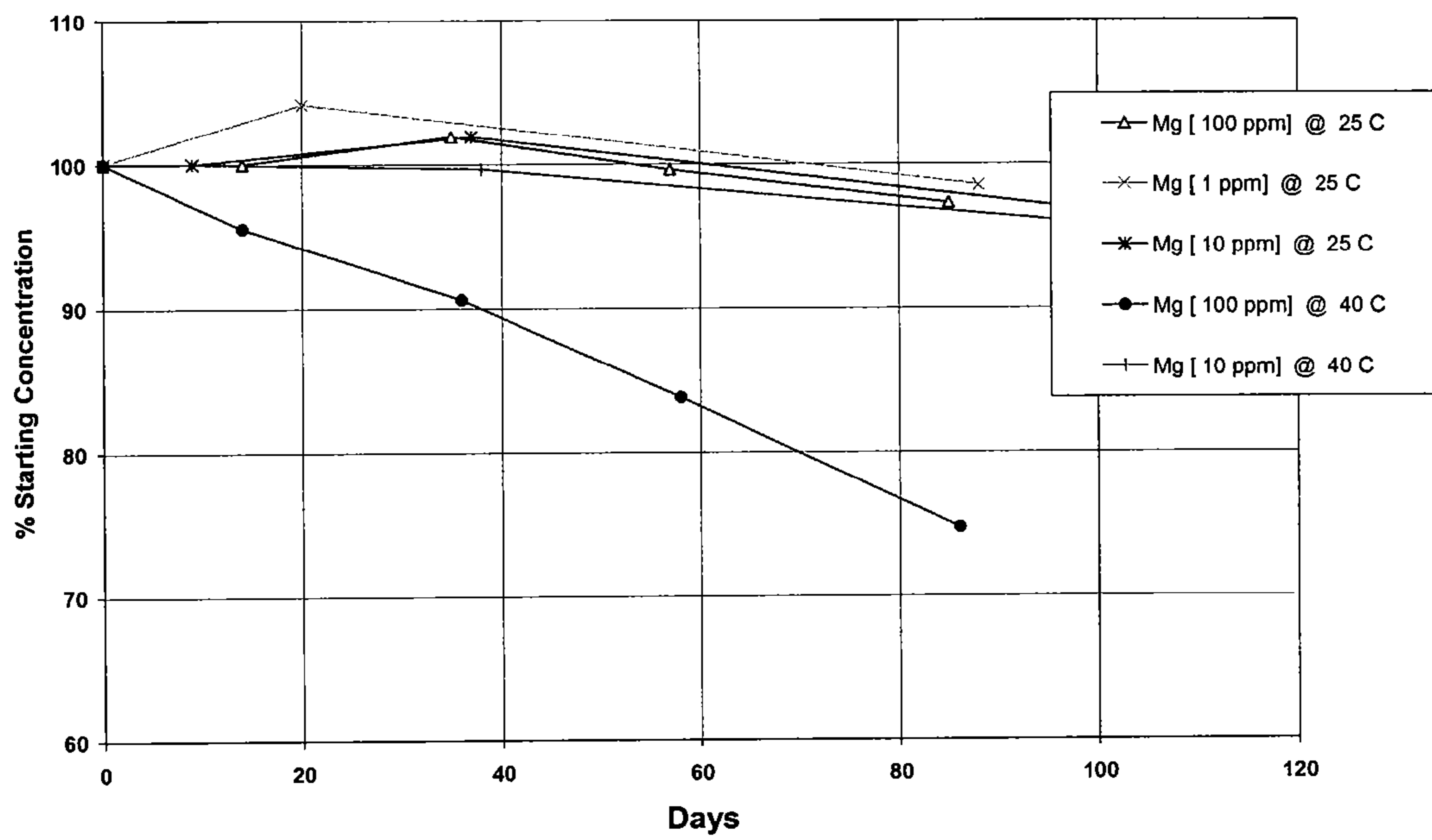
Figure 7 - Low Levels of MgCl2 in Deionized Water
