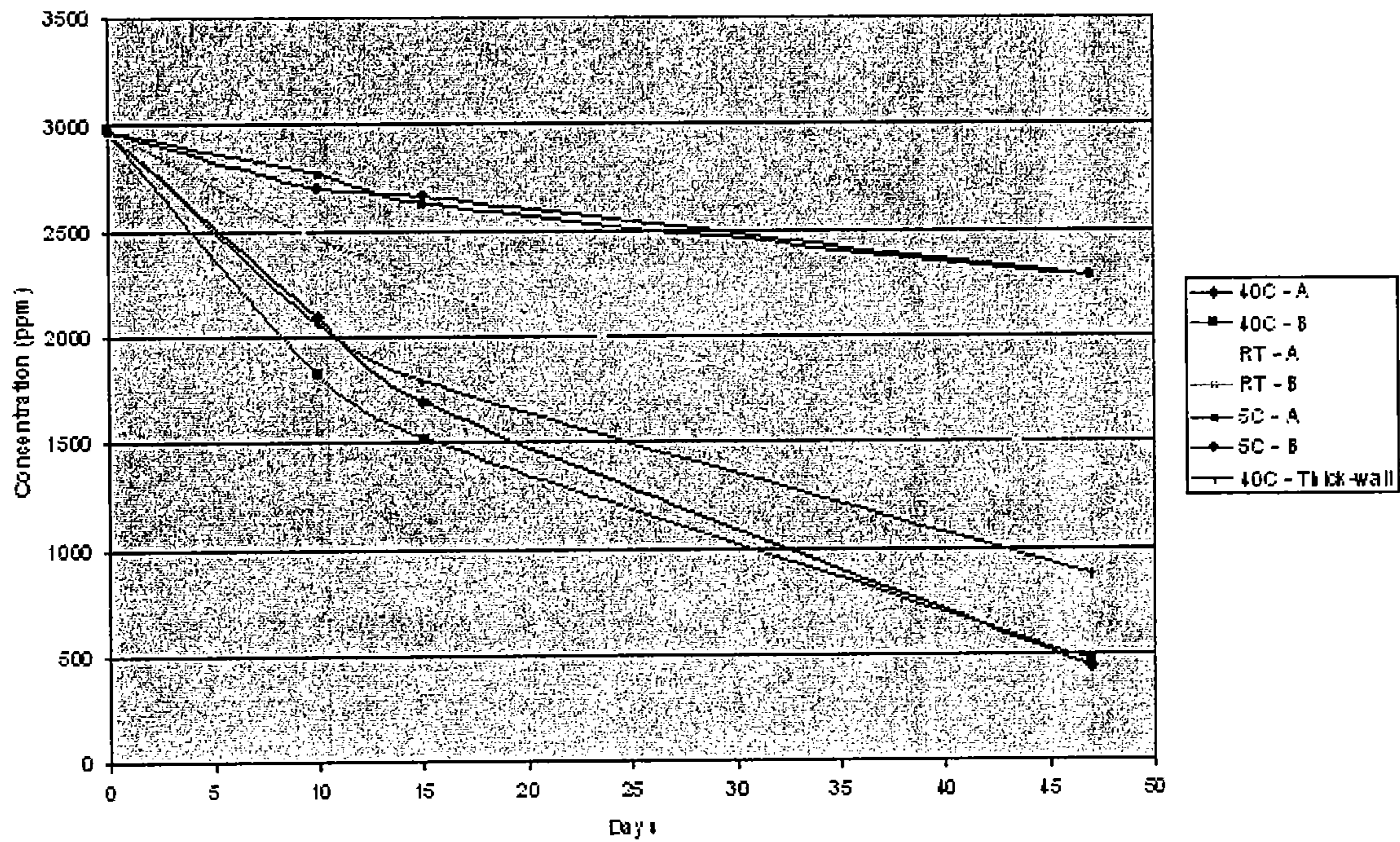
Figure 5: Solutions Stored In HDPE Bottles
