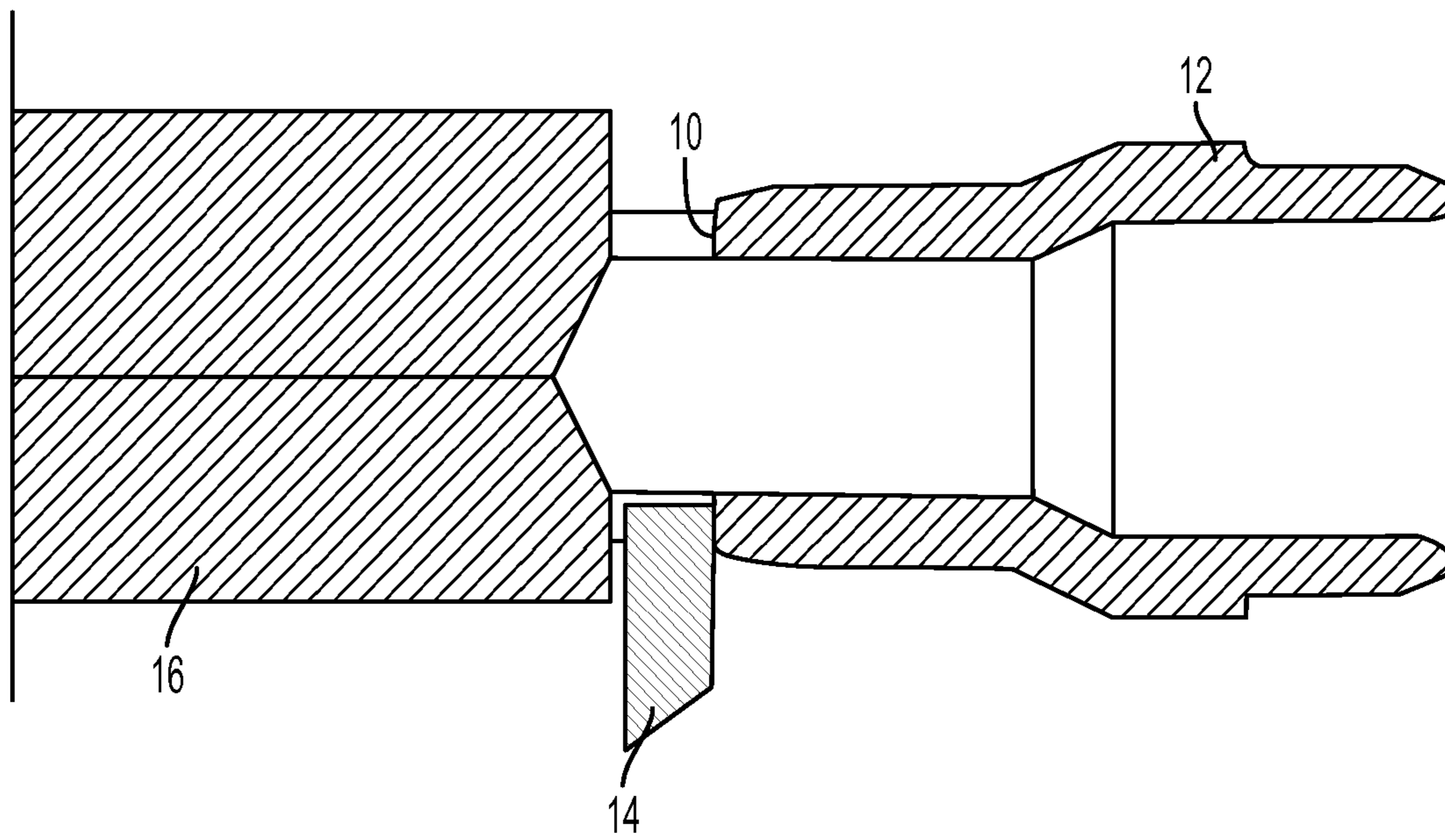
FIG. 2 PRIOR ART
