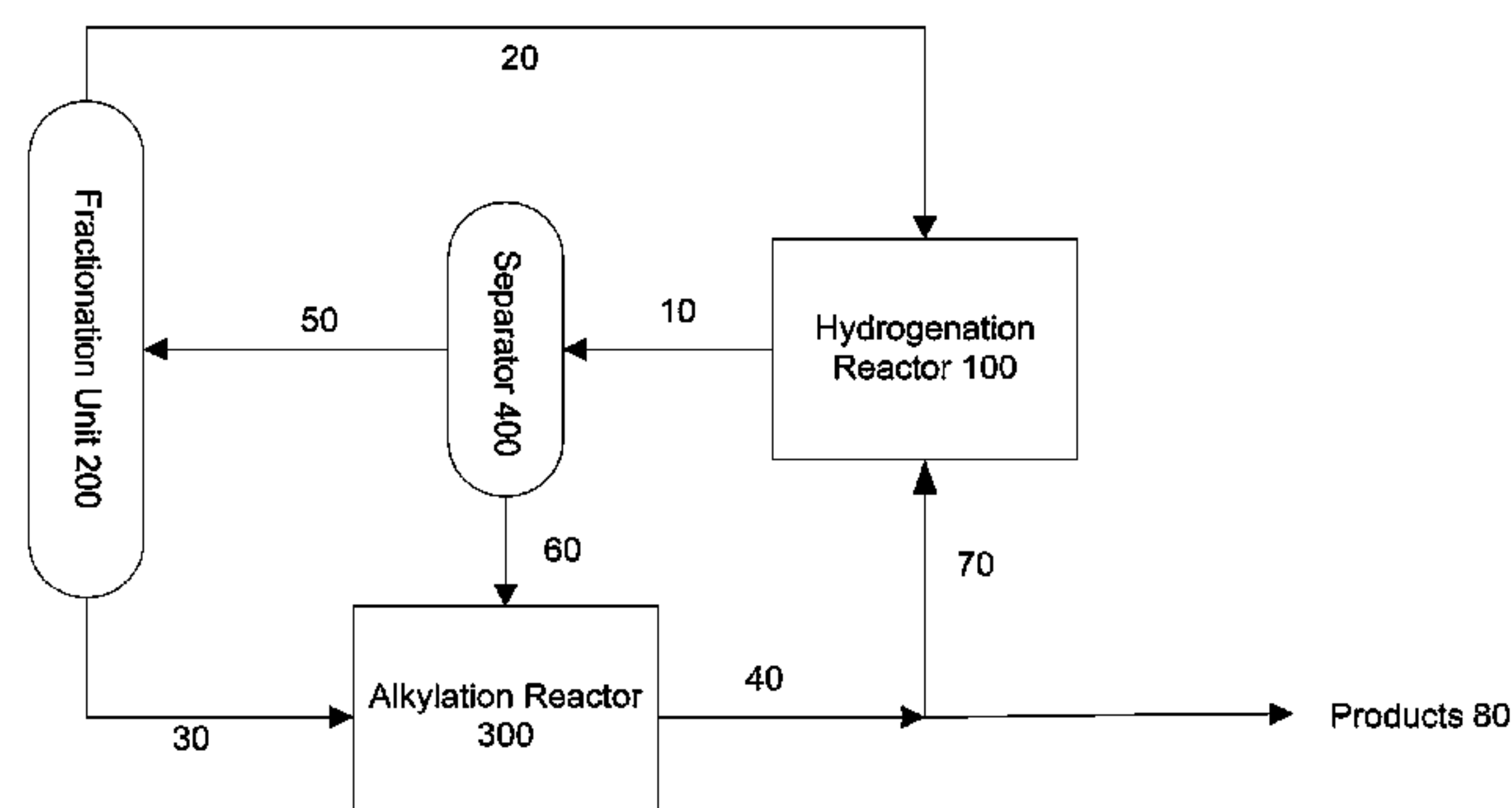
An Alkylation Unit with Catalyst Hydro-Regeneration, Hydrogen Recycle, and Hydrogen Chloride Recovery
