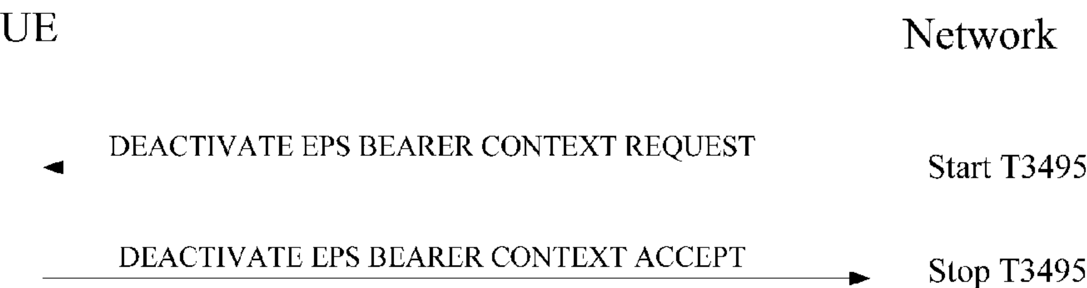
Figure 6.4.4.2.1: EPS bearer context deactivation procedure
