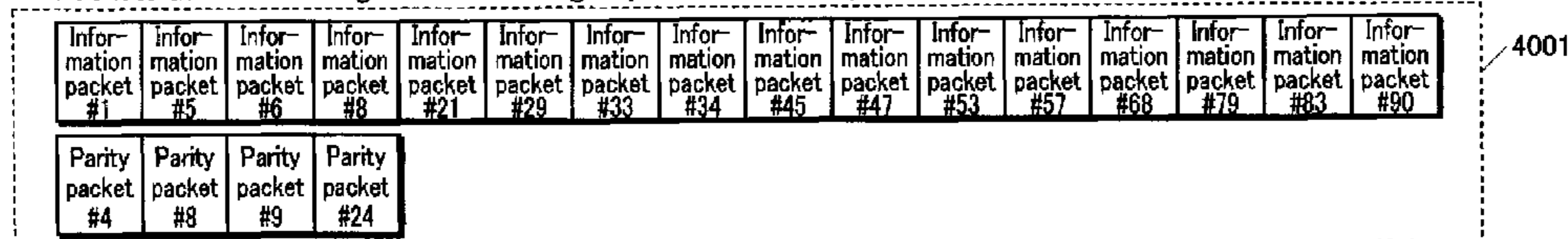
Packets that are missing before decoding at packet level in repeater
