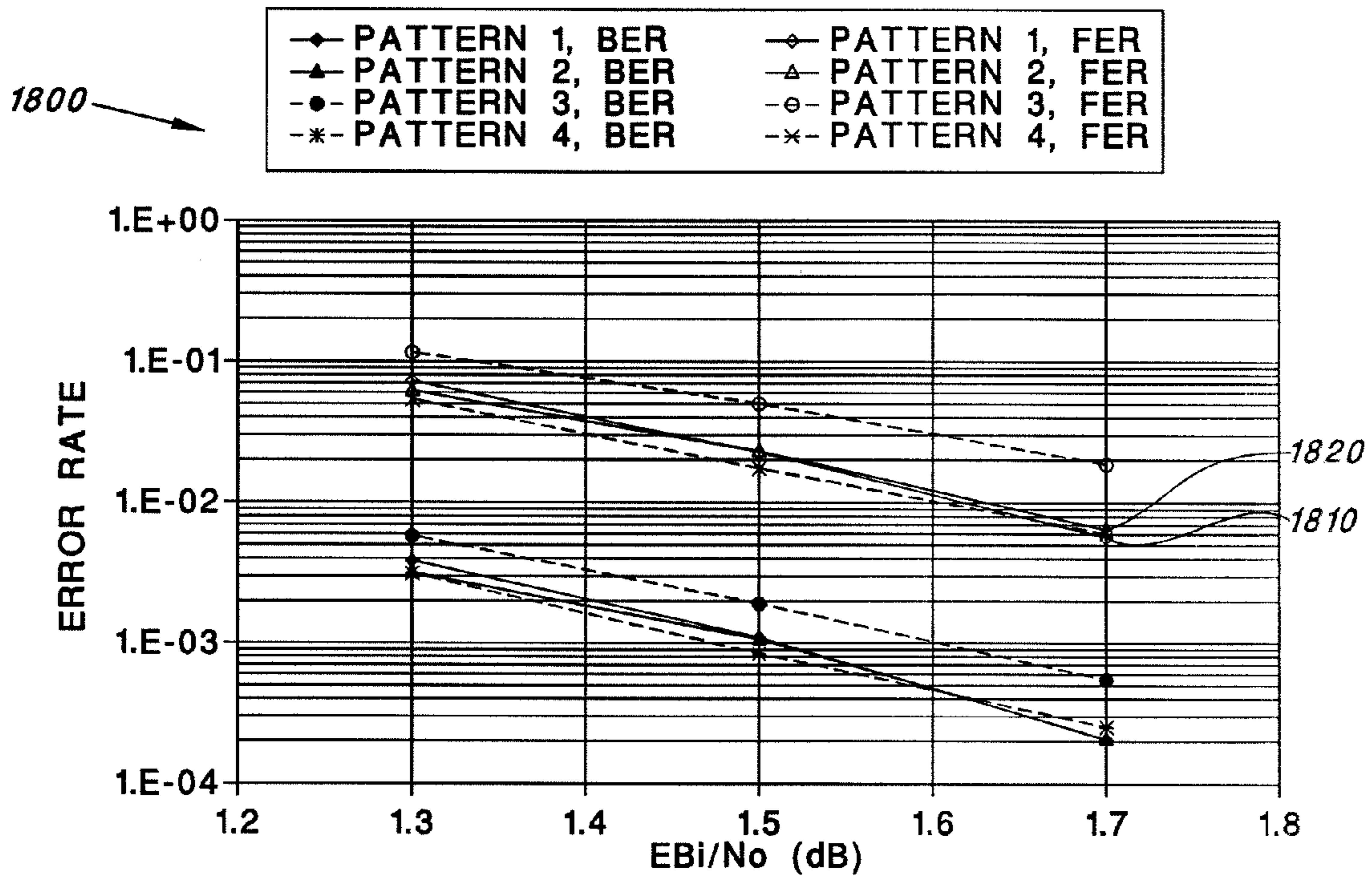
FIG. 18 RATE 1/2 PUNCTURING COMPARISON, FRAME=512
