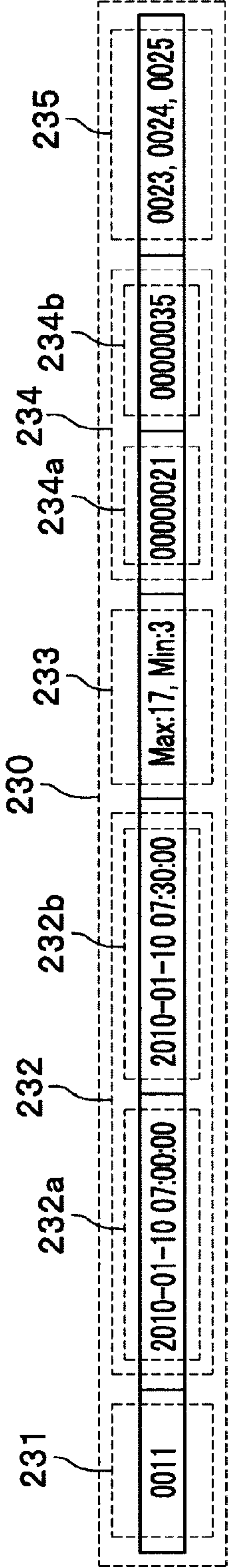
(b) DATA STRUCTURE OF TIME-SERIES INDEX NODE
