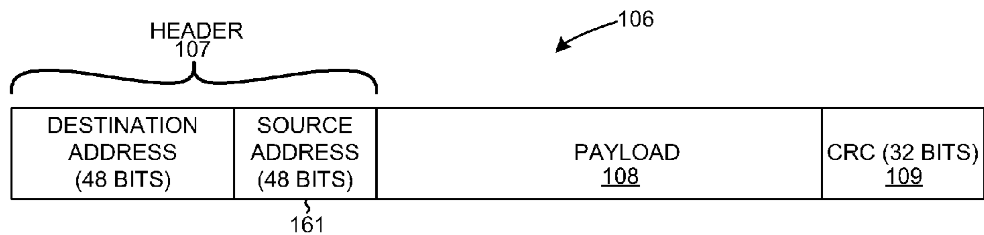
ETHERNET PACKET FIG. 15
