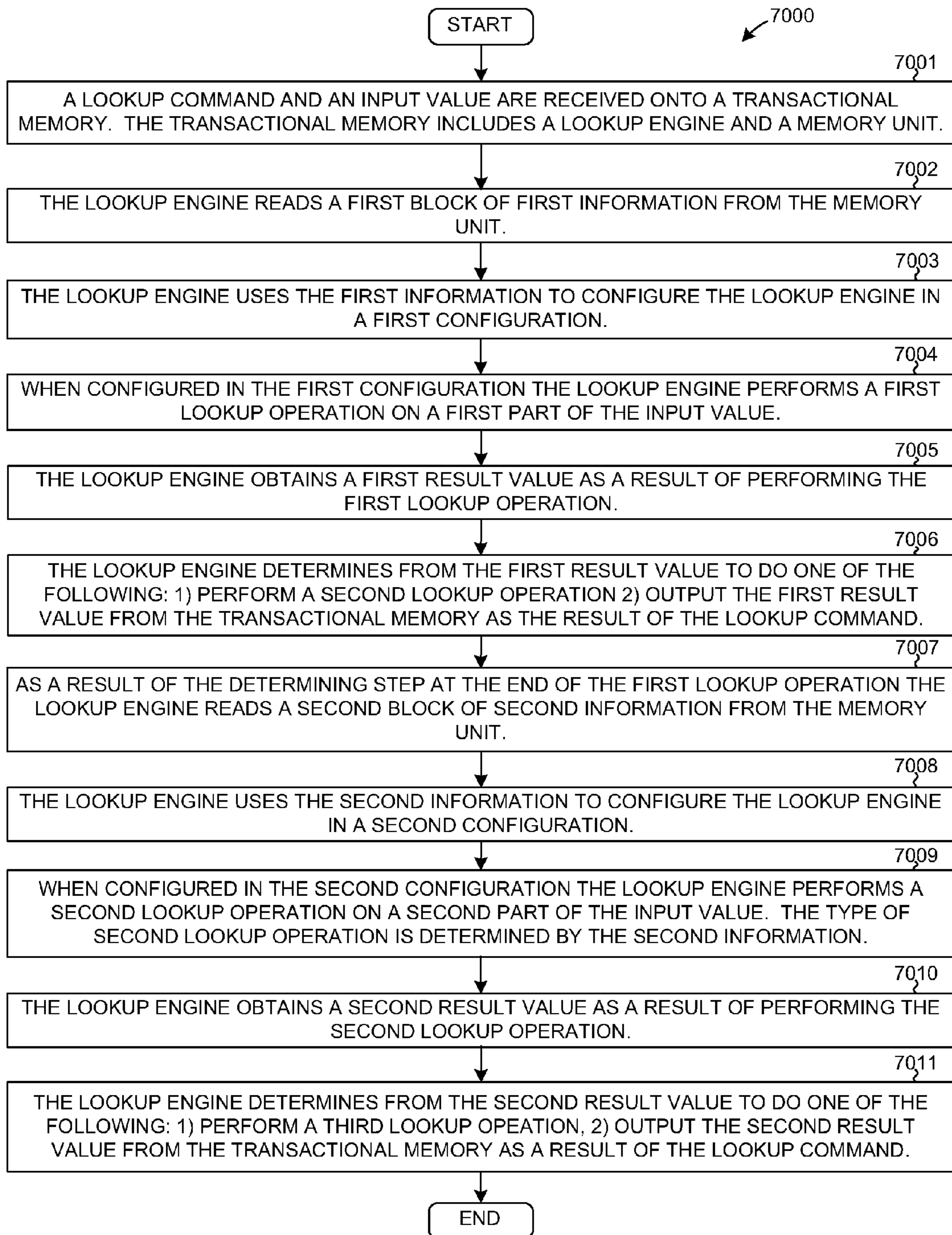
RECURSIVE USE OF MULTIPLE HARDWARE LOOKUP STRUCTURES
