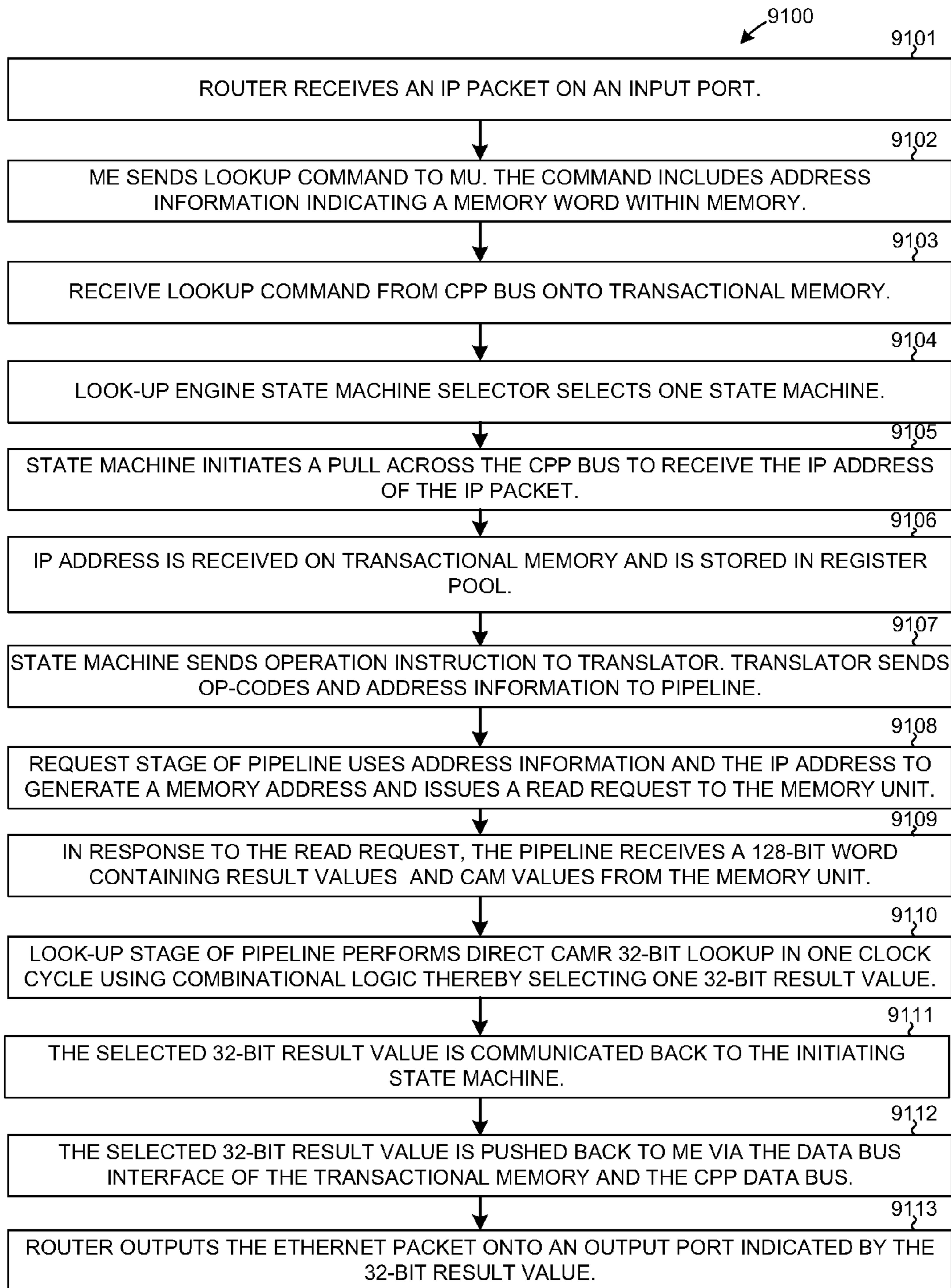
CAMR 32-BIT LOOKUP FLOWCHART
