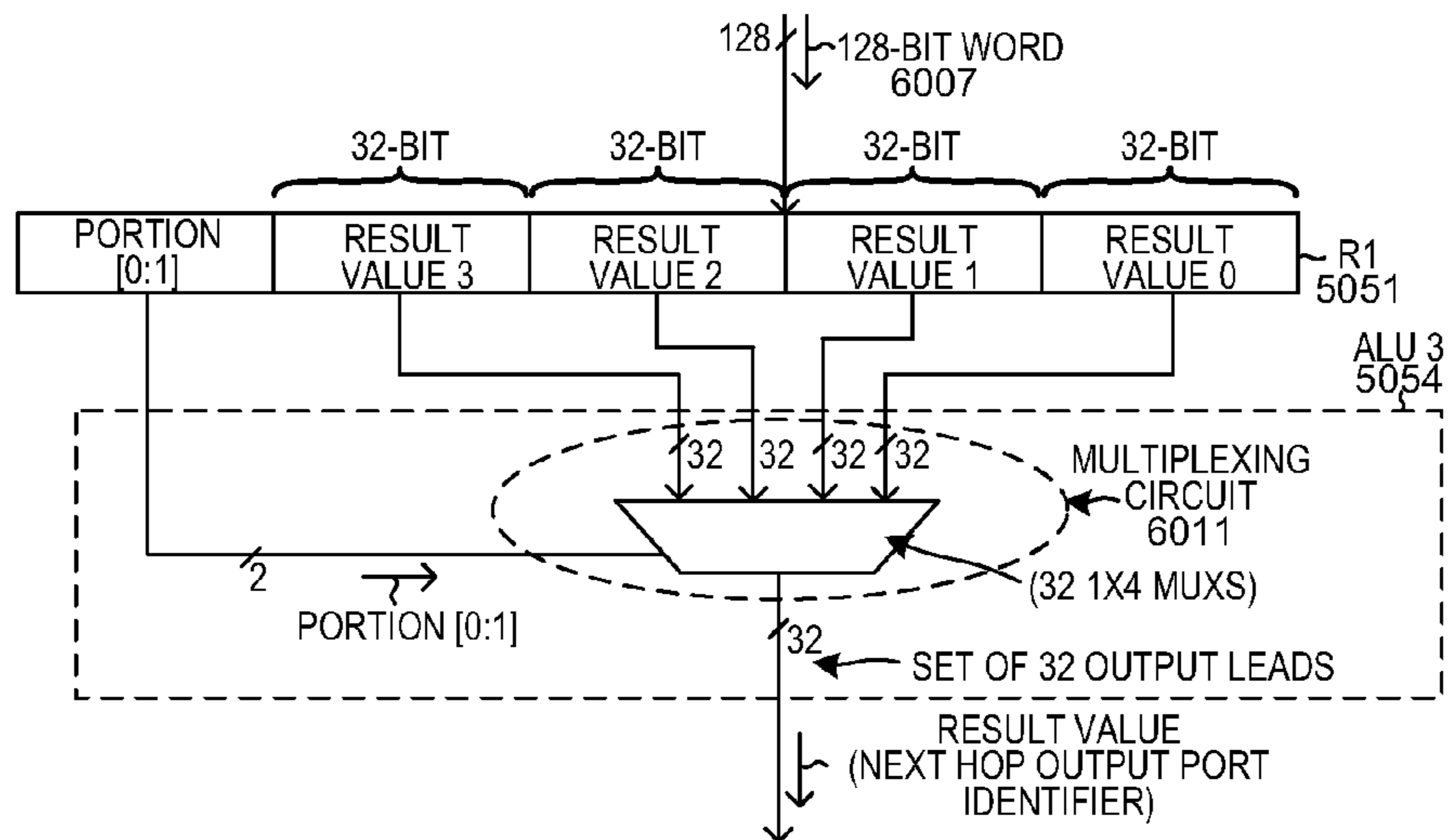
DIRECT 32-BIT LOOKUP STAGE FIG. 42
