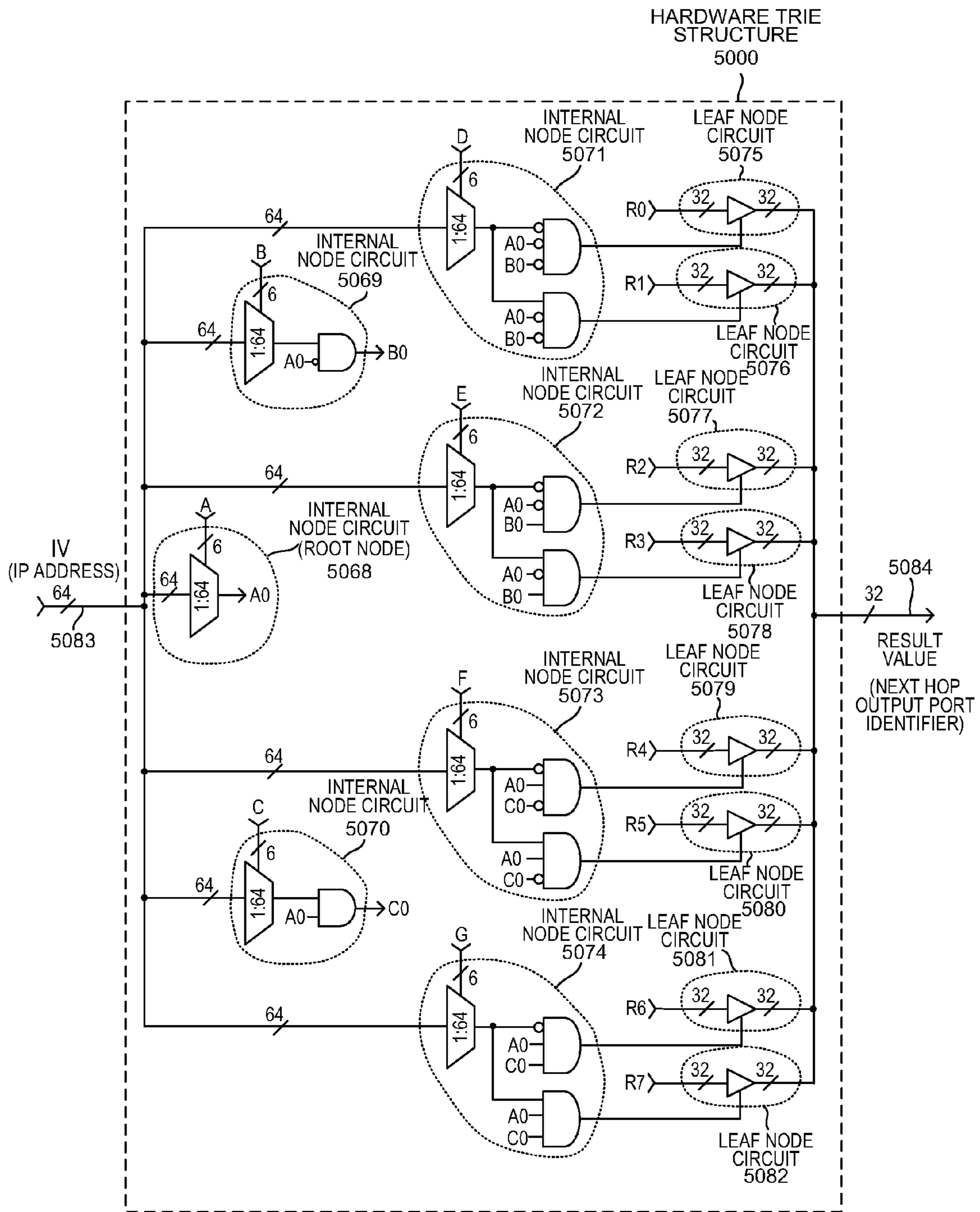
HARDWARE TRIE STRUCTURE
