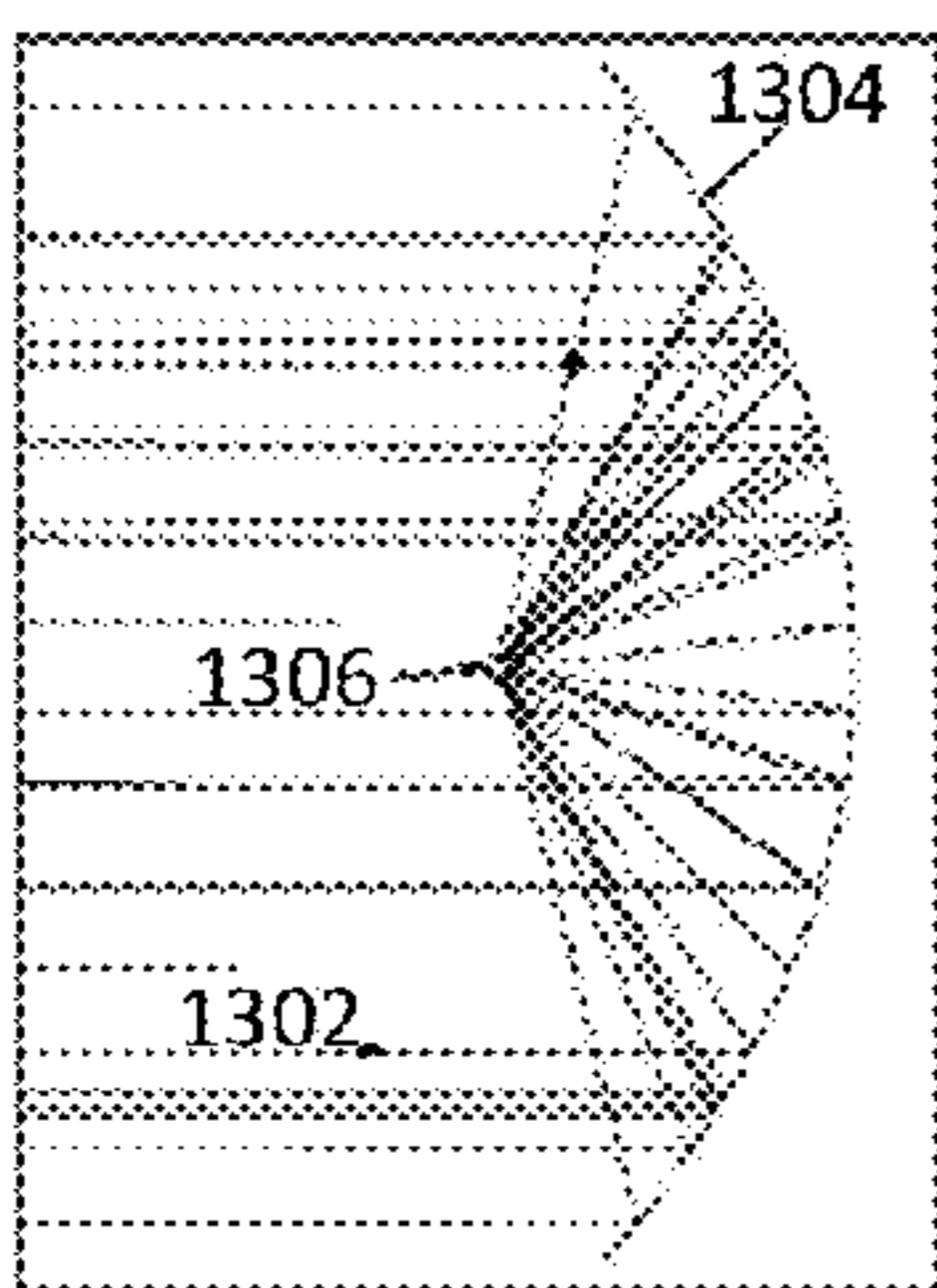
Receiver/Collector Layout
