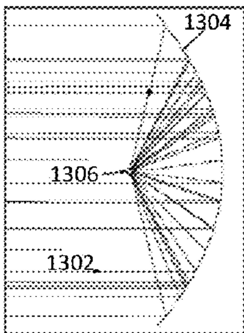
Receiver/Collector Layout
