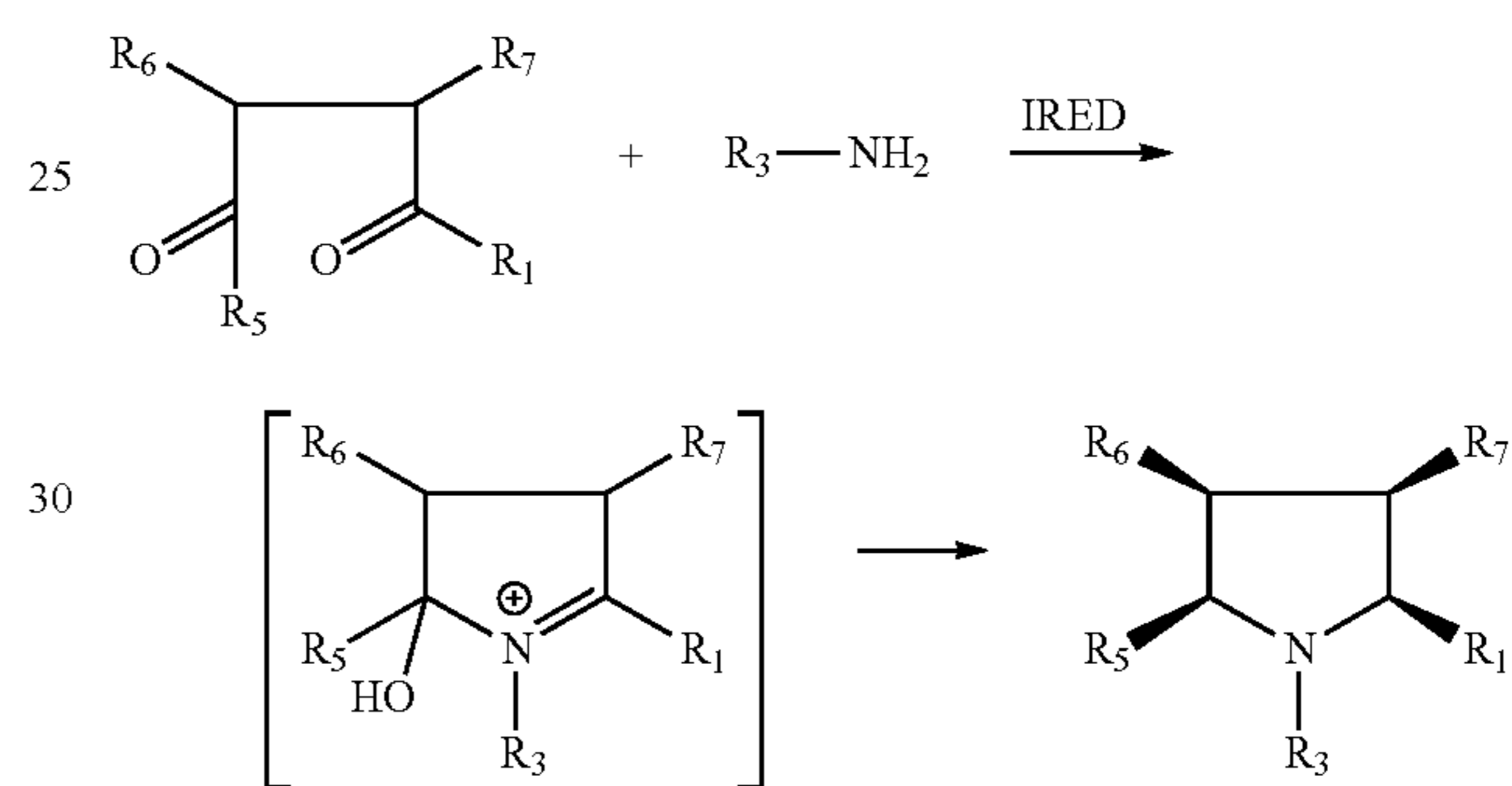
Scheme 9
