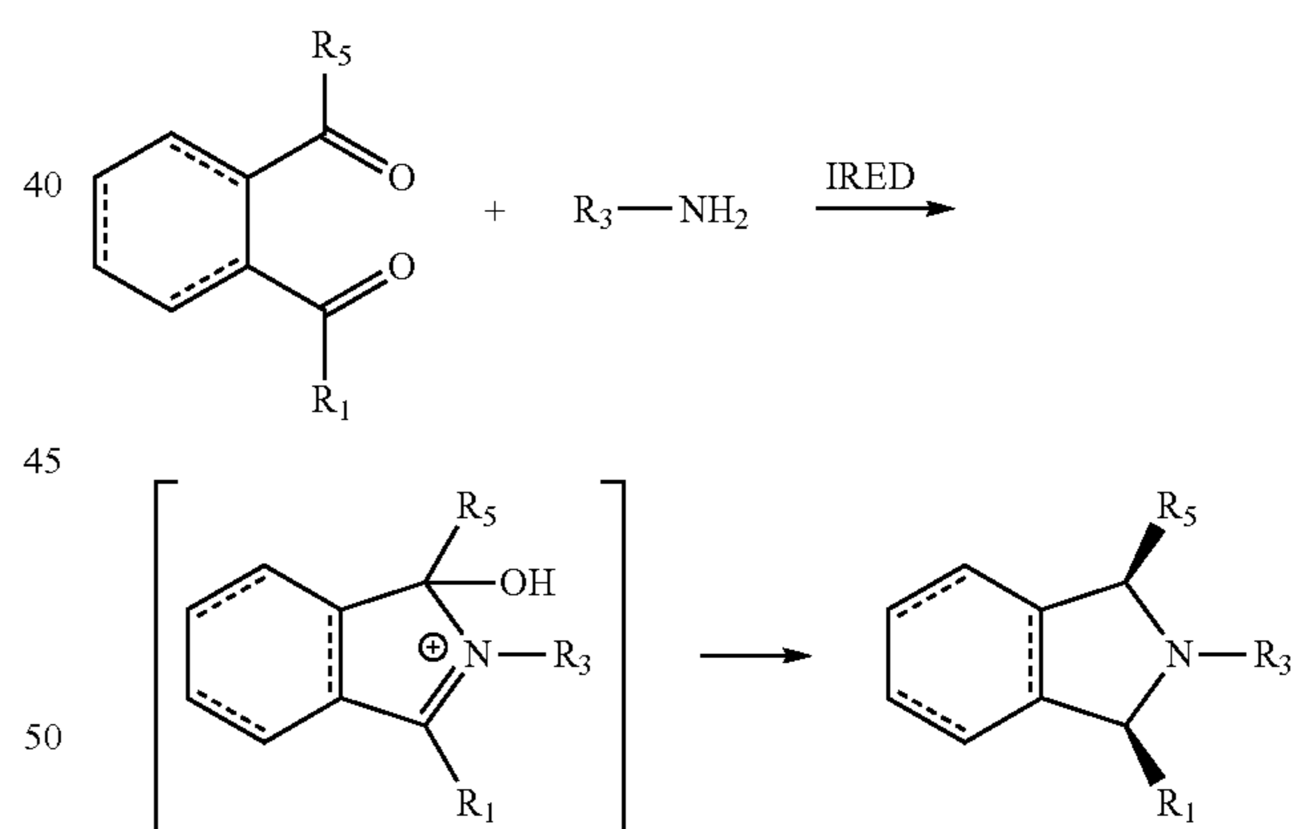
Scheme 9
