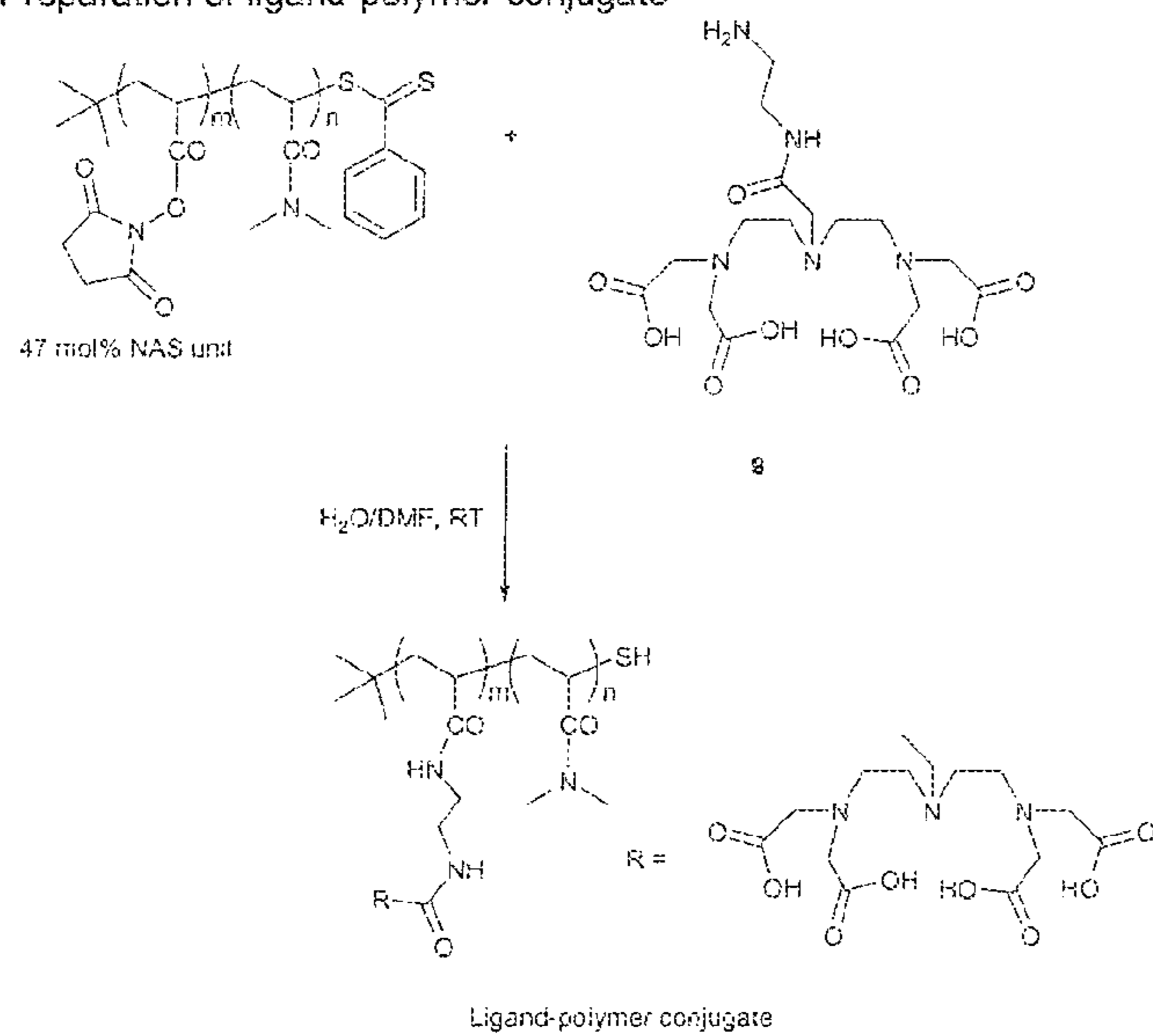
Scheme 10. Preparation of ligand-polymer conjugate
