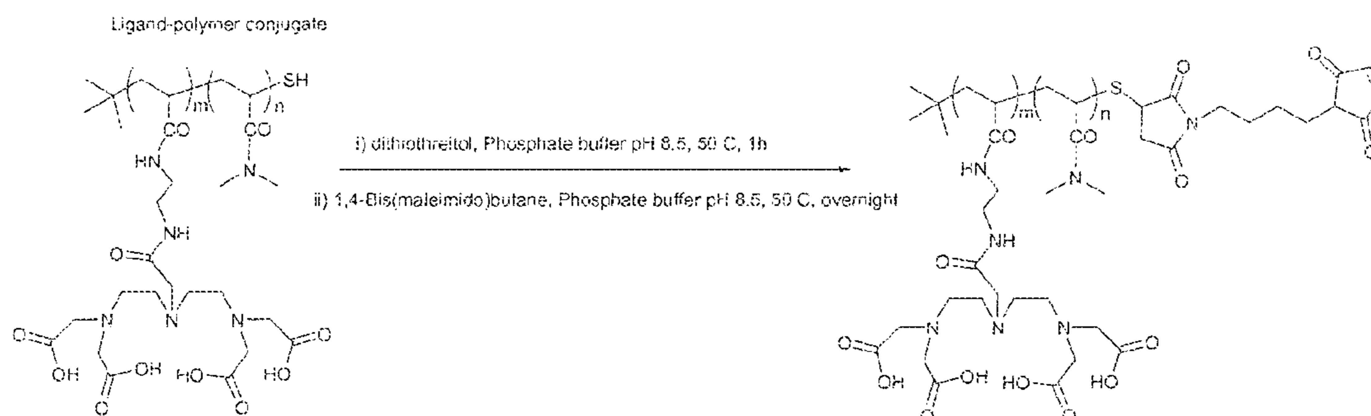
Scheme 11. Reaction of ligand-polymer conjugate with 1,4-bis(maleimido)butane
