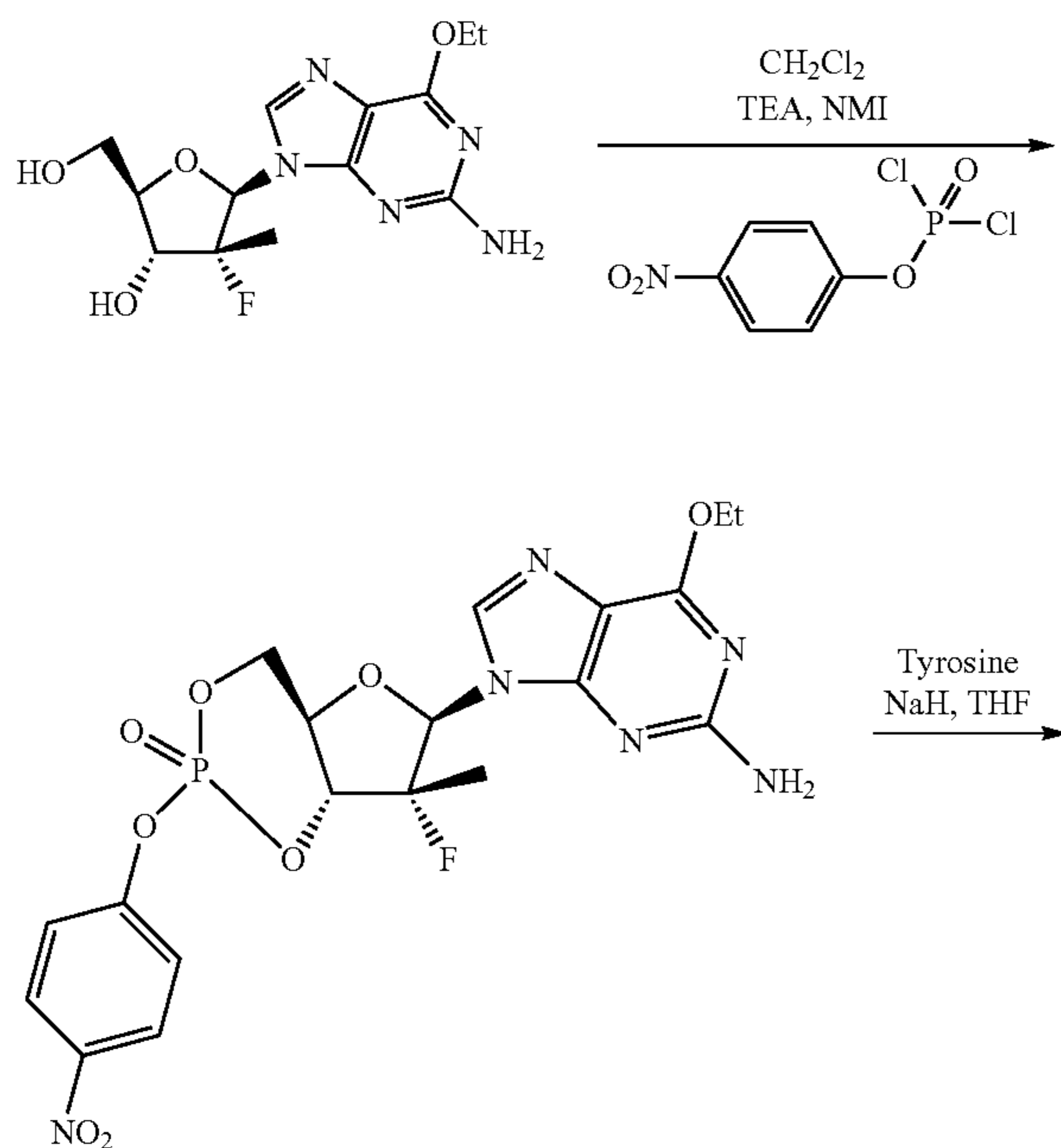
Scheme 5
