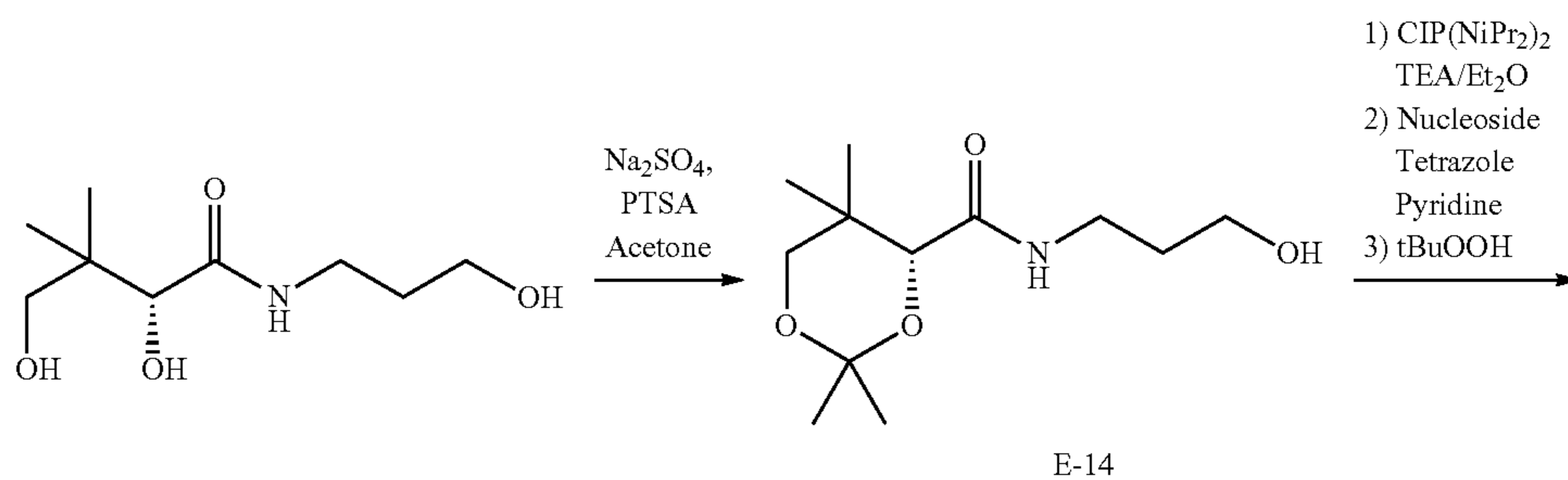
Scheme 4
