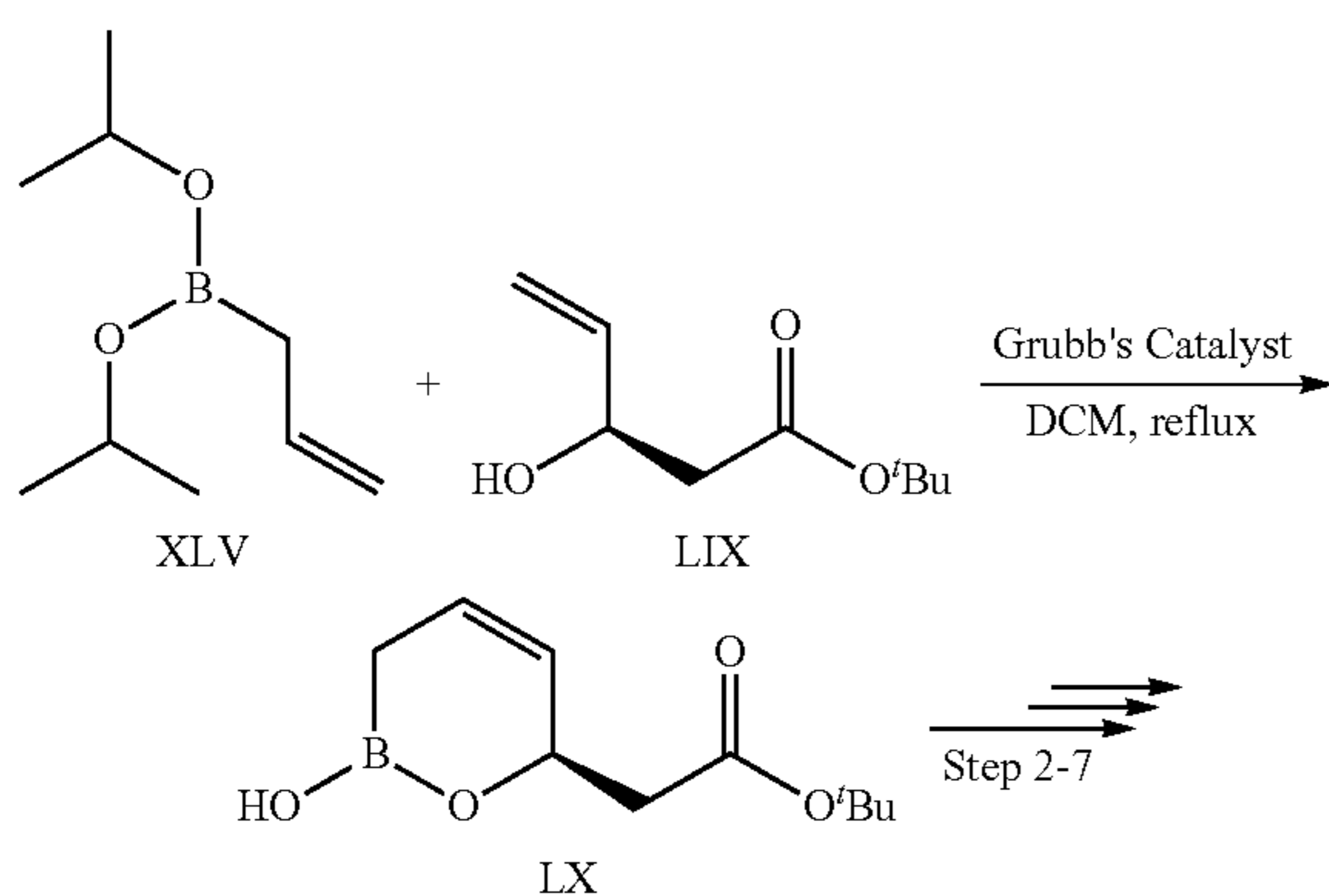
Scheme 14
