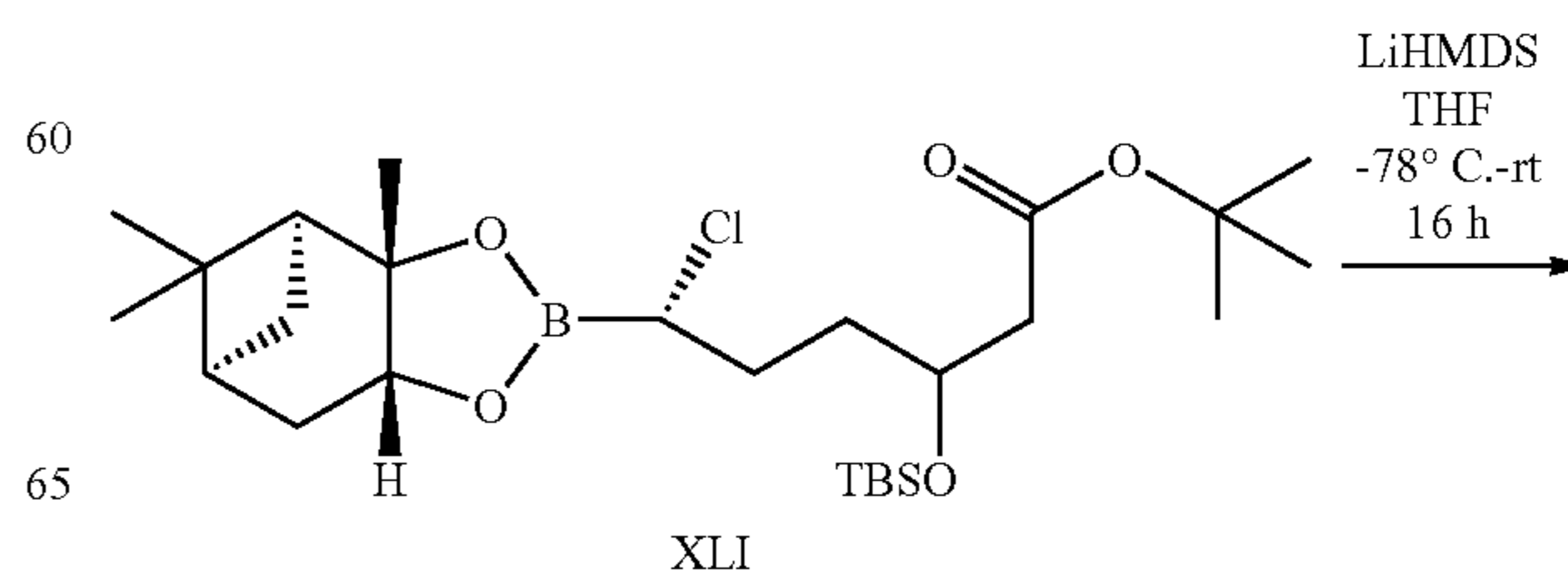
Scheme 10
