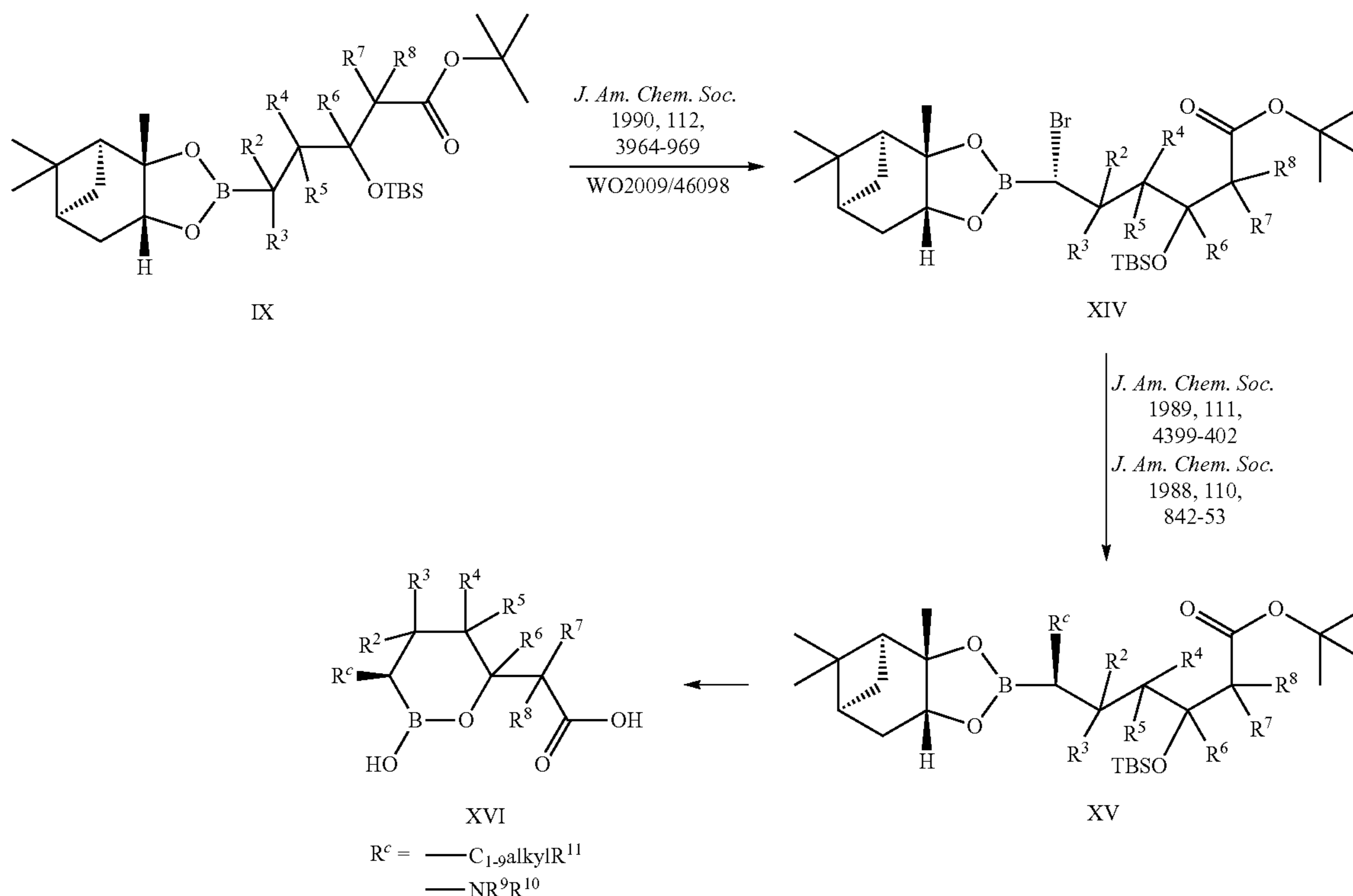
Scheme 2
