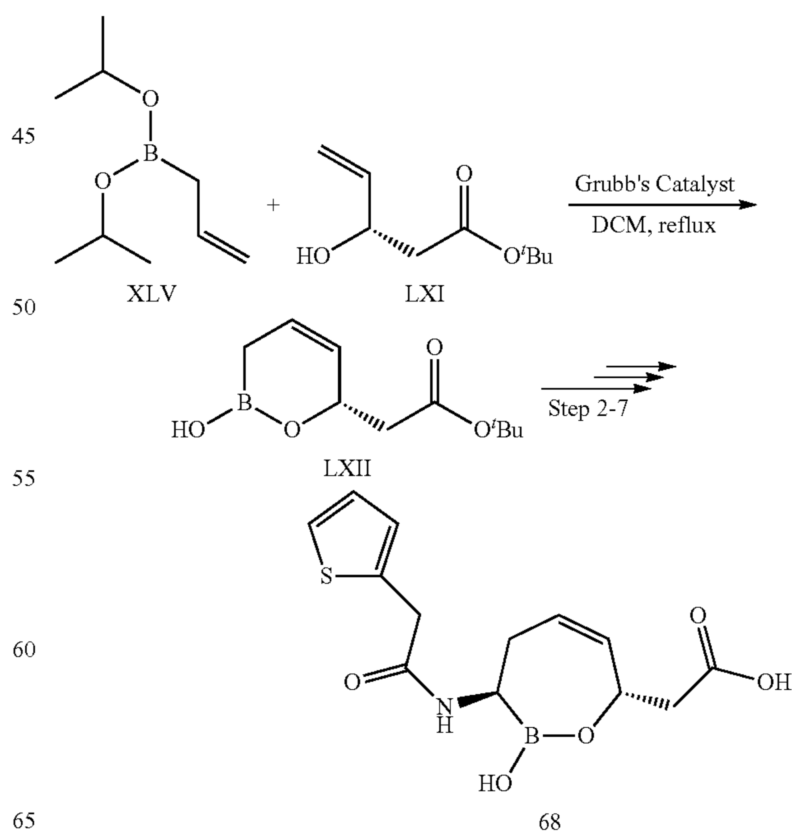
Scheme 15
