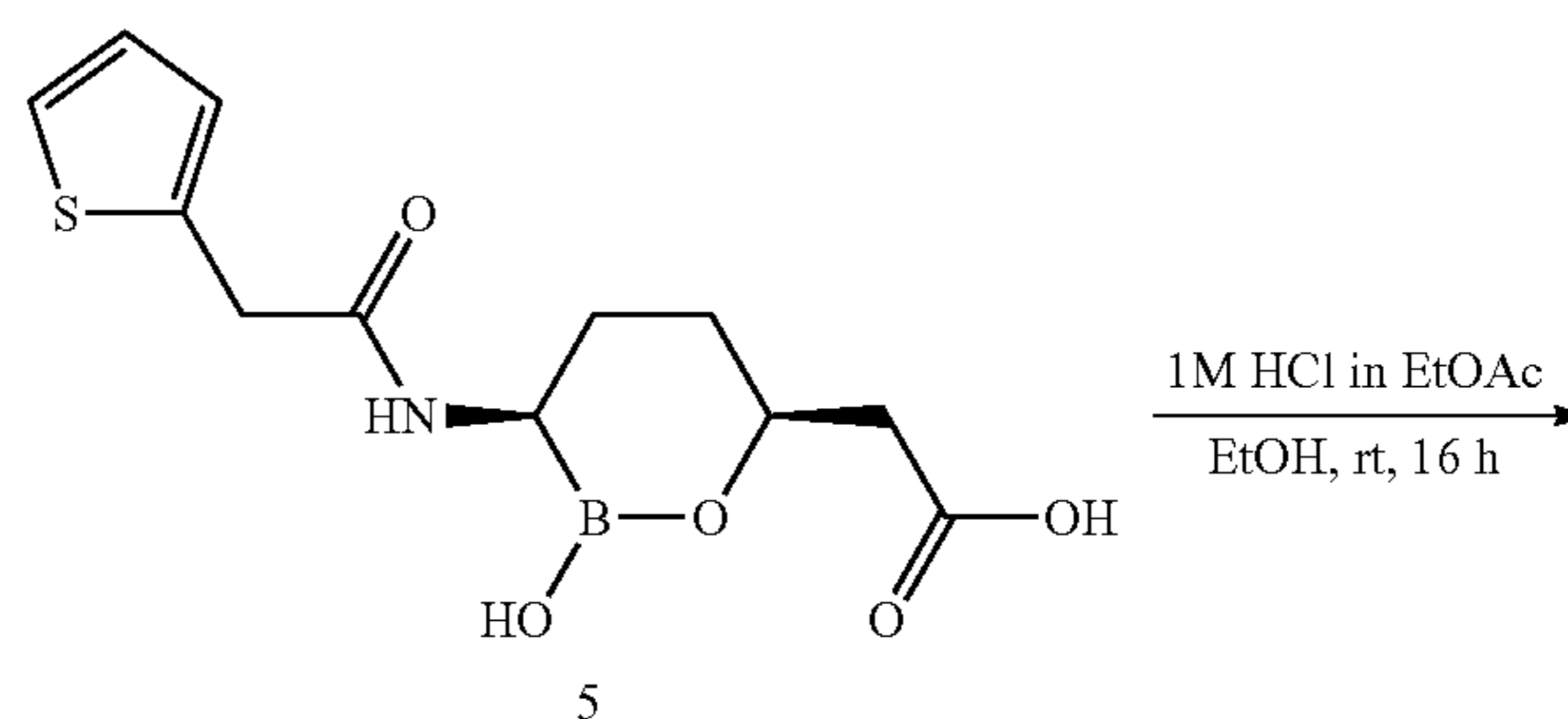
Scheme 13
