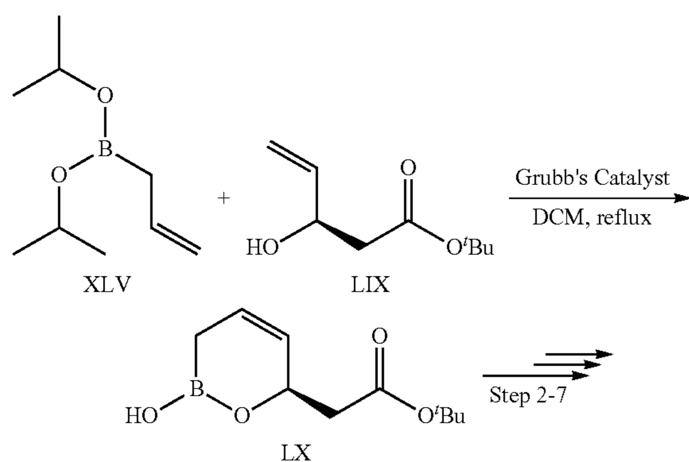
Scheme 14
