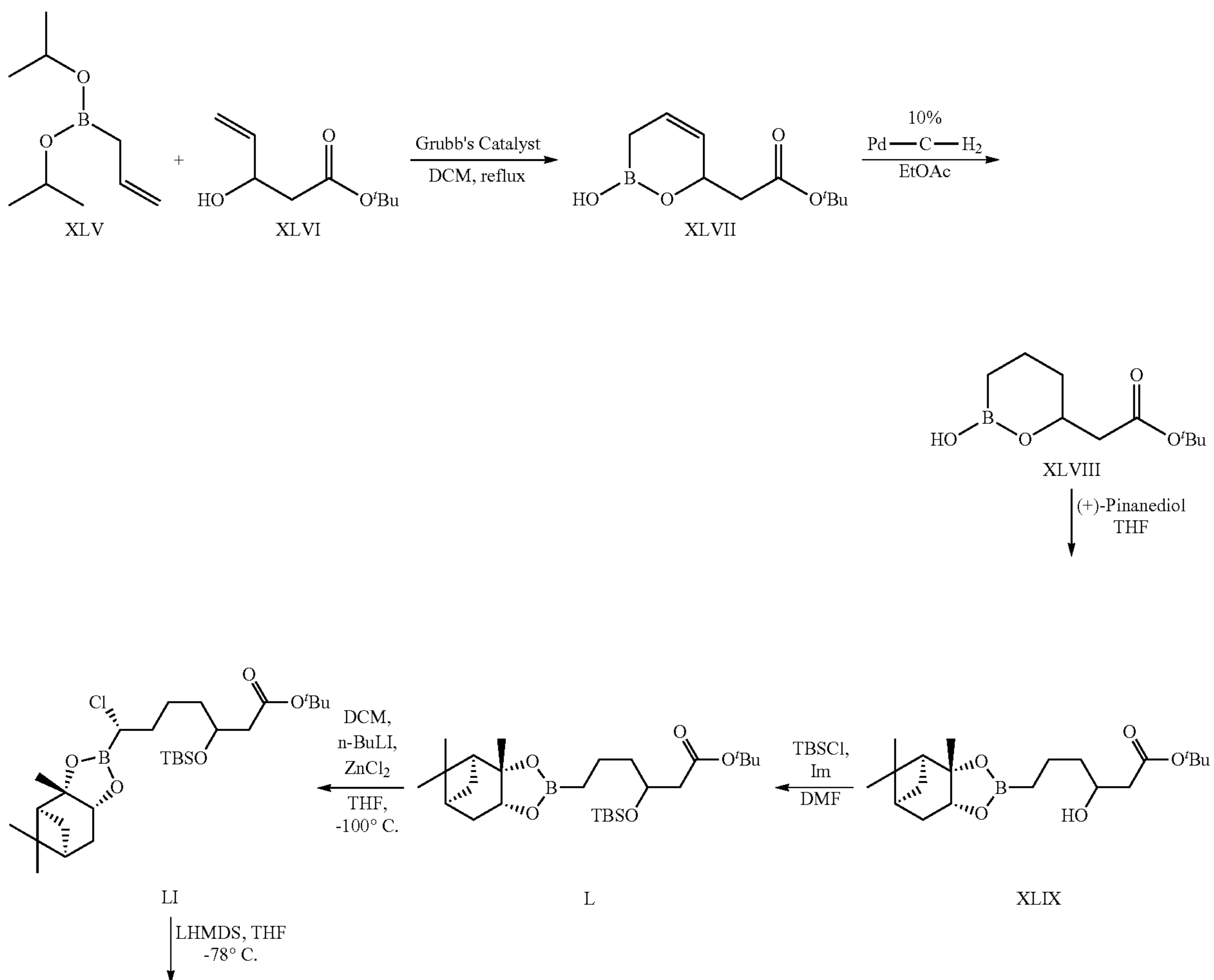
Scheme 11
