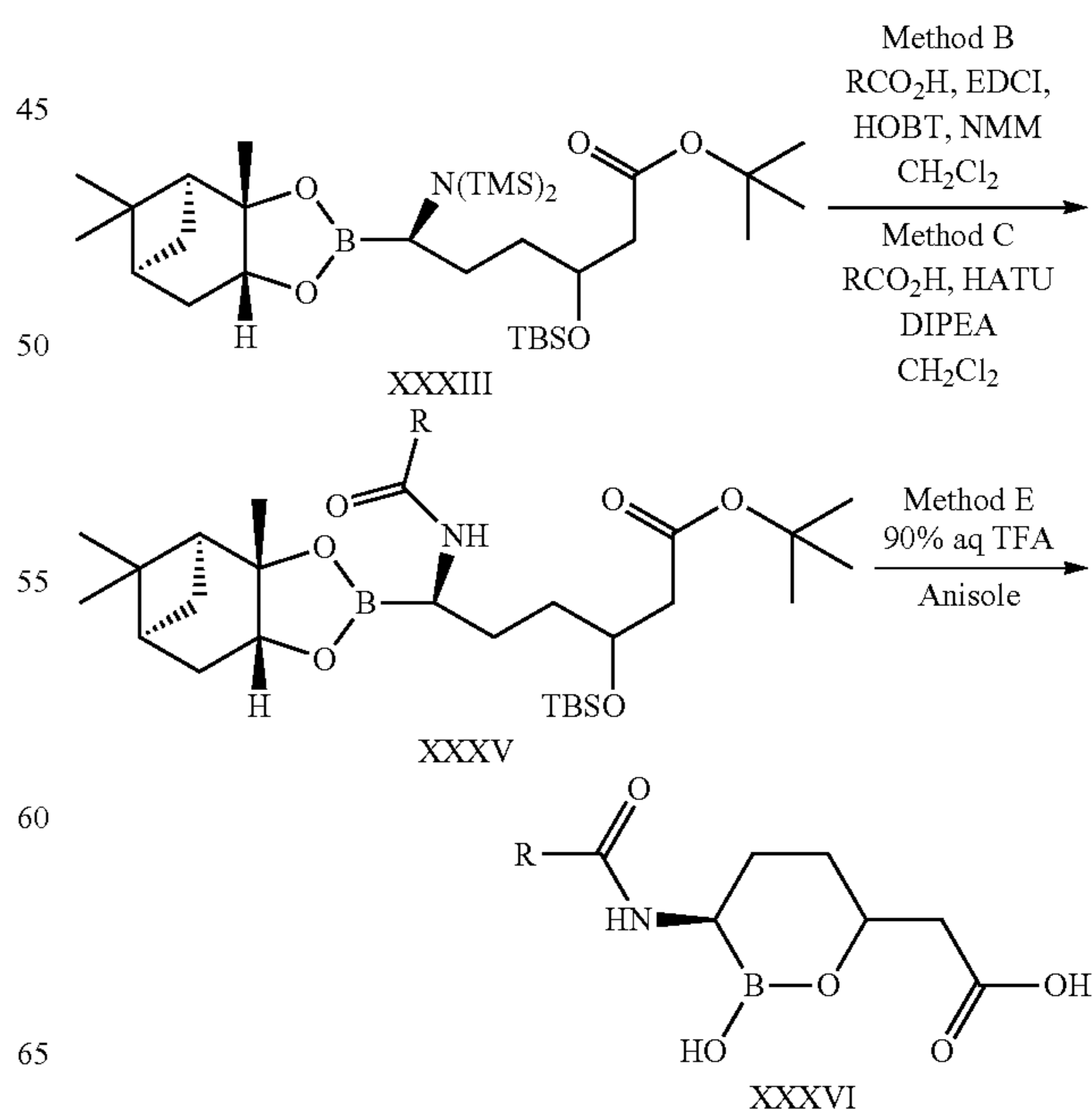
Scheme 9
