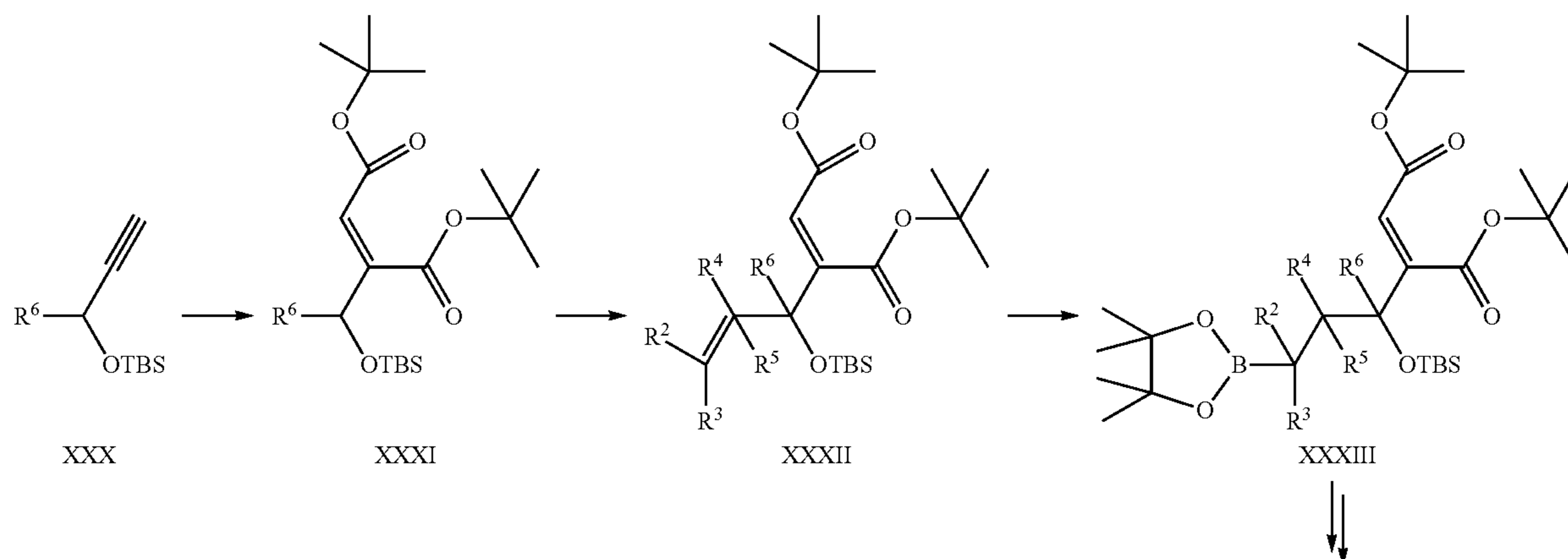
Scheme 7
