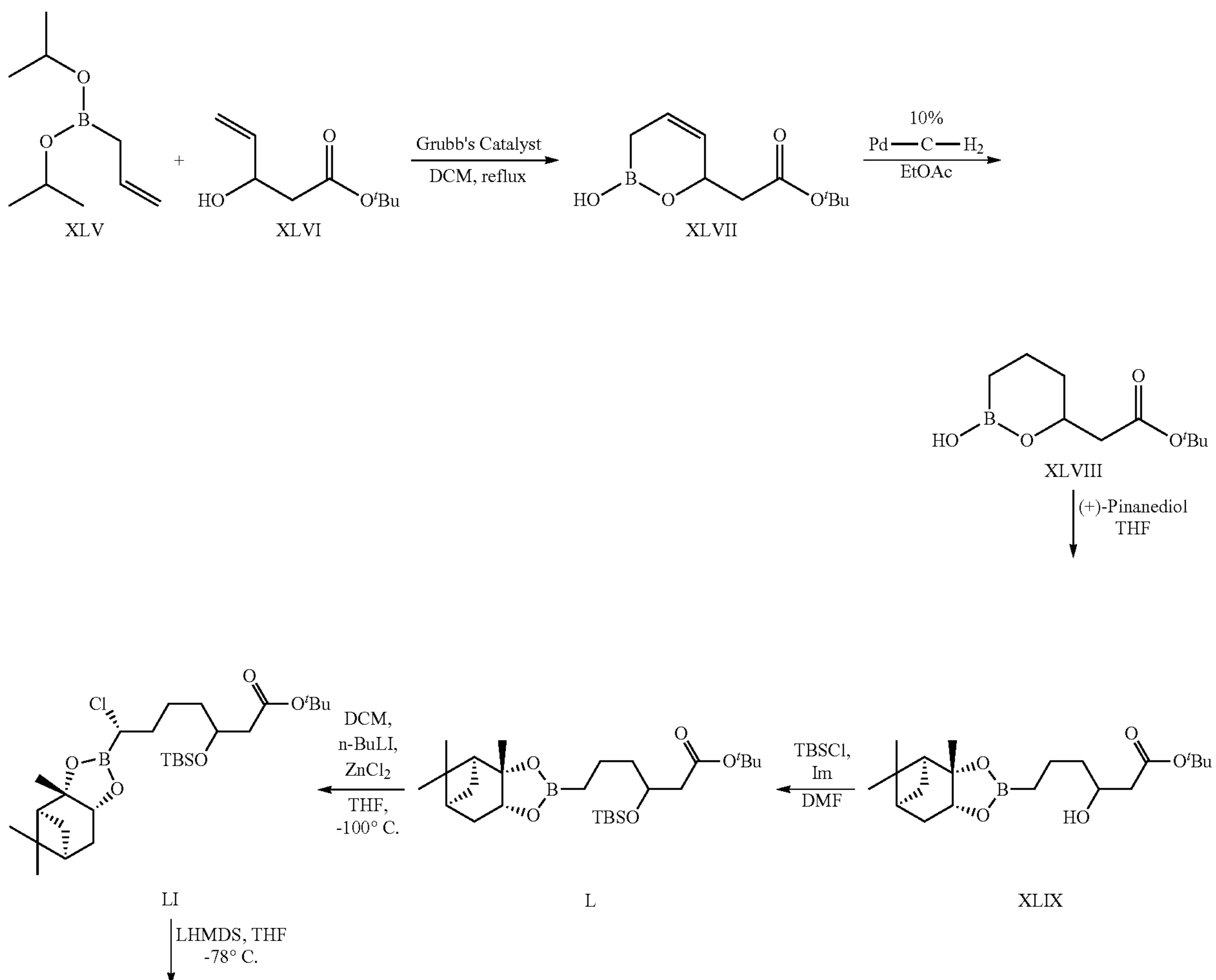
Scheme 11
