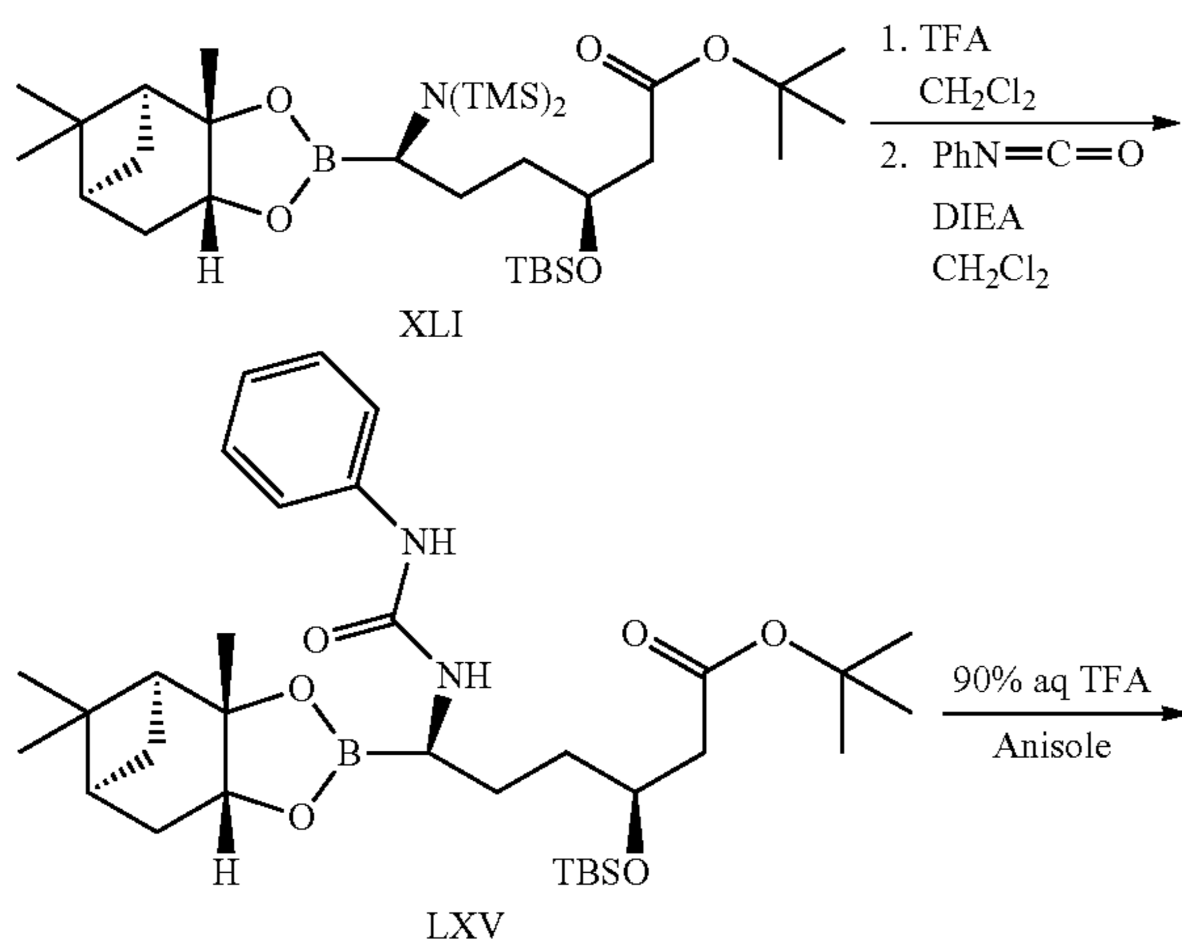
Scheme 18
