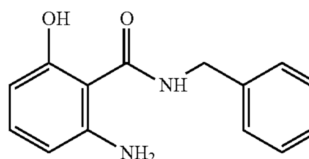
2-Amino-N-benzyl-6-hydroxybenzamide
