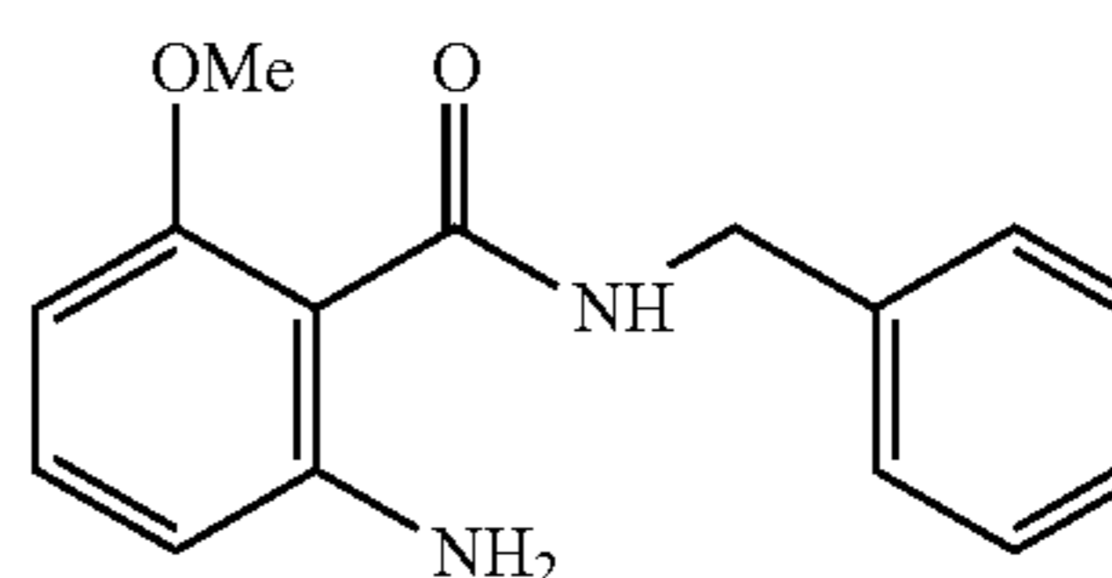
2-Amino-N-benzyl-6-methoxybenzamide
