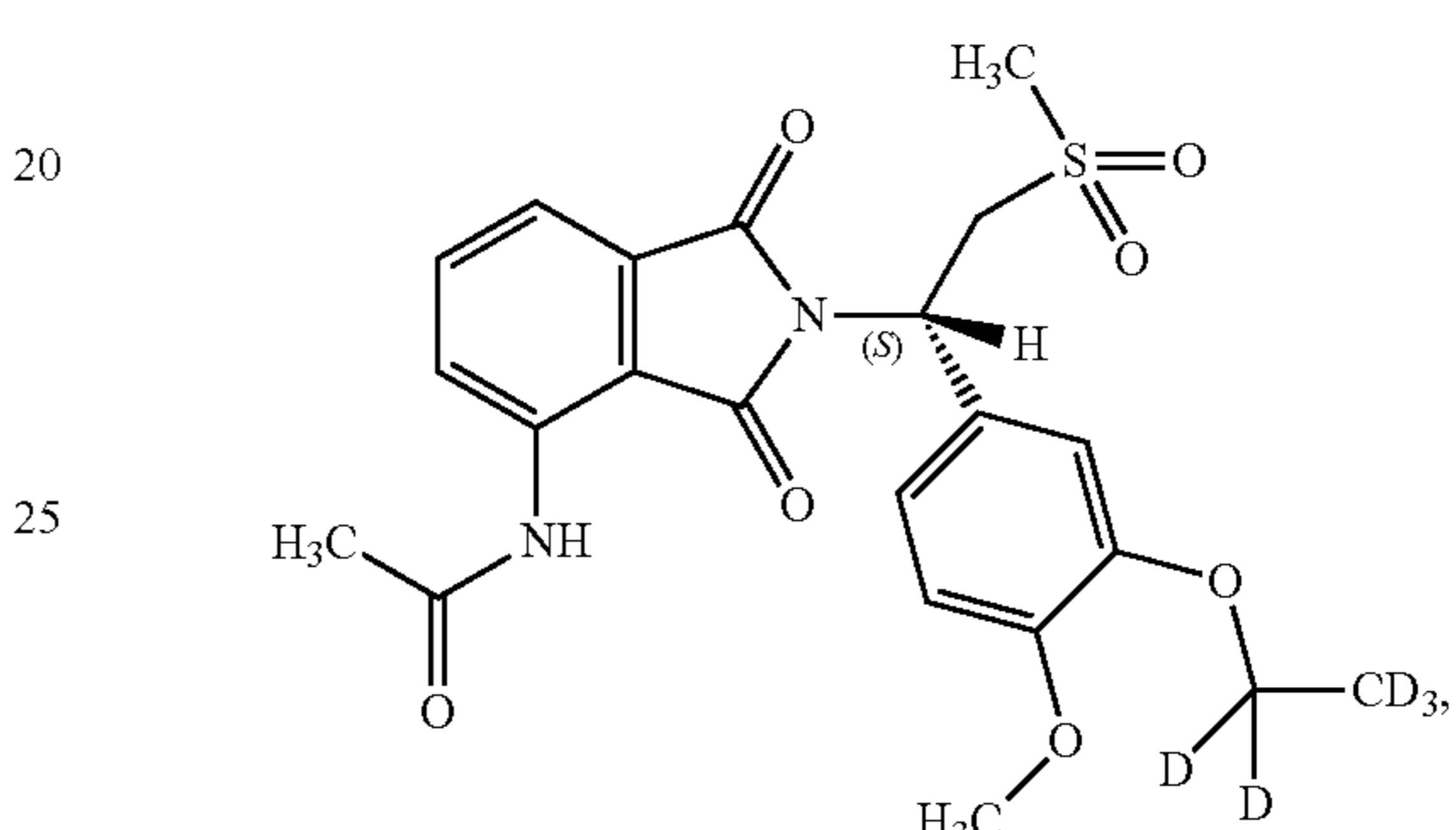
Compound 114a
