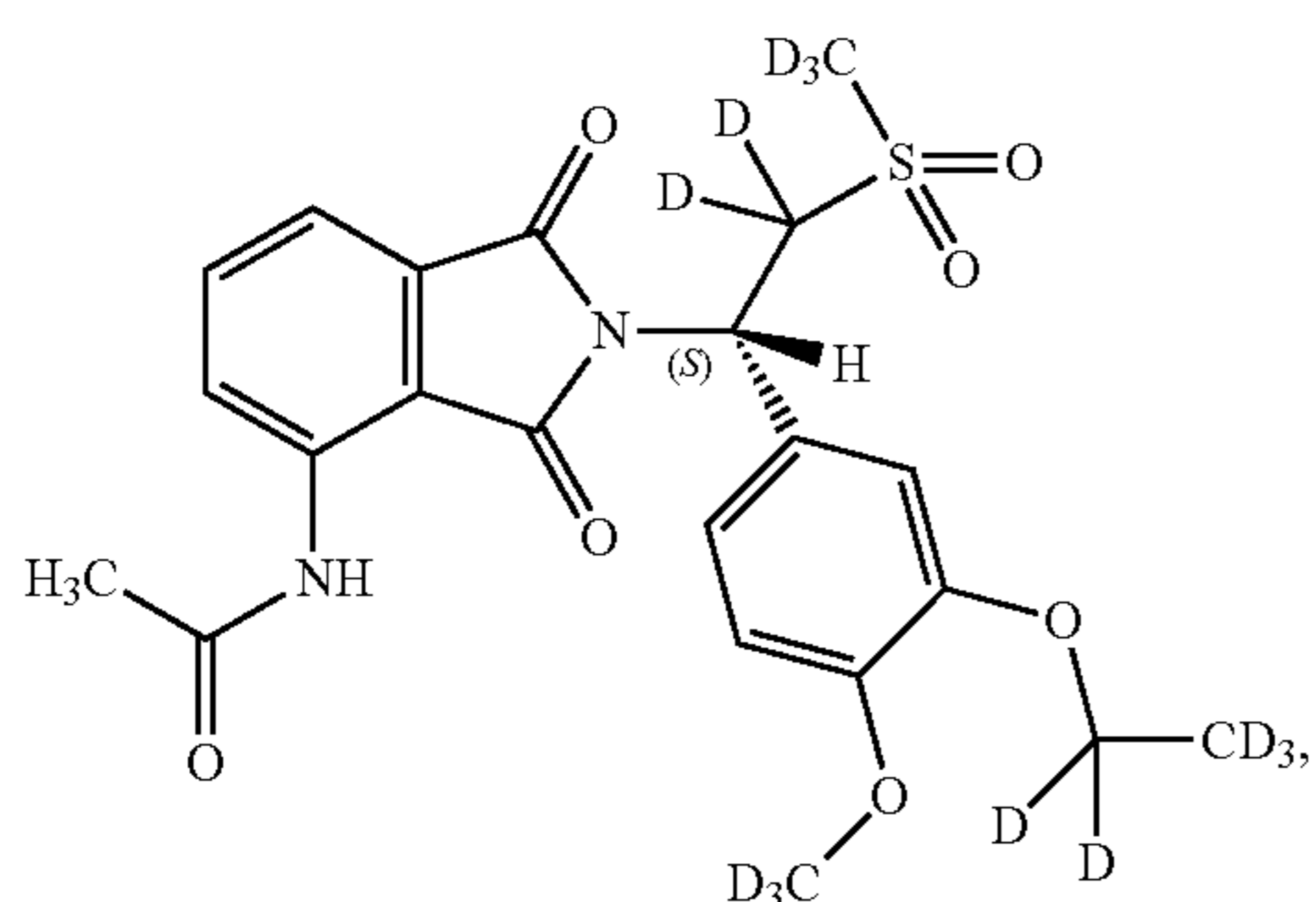
Compound 116a
