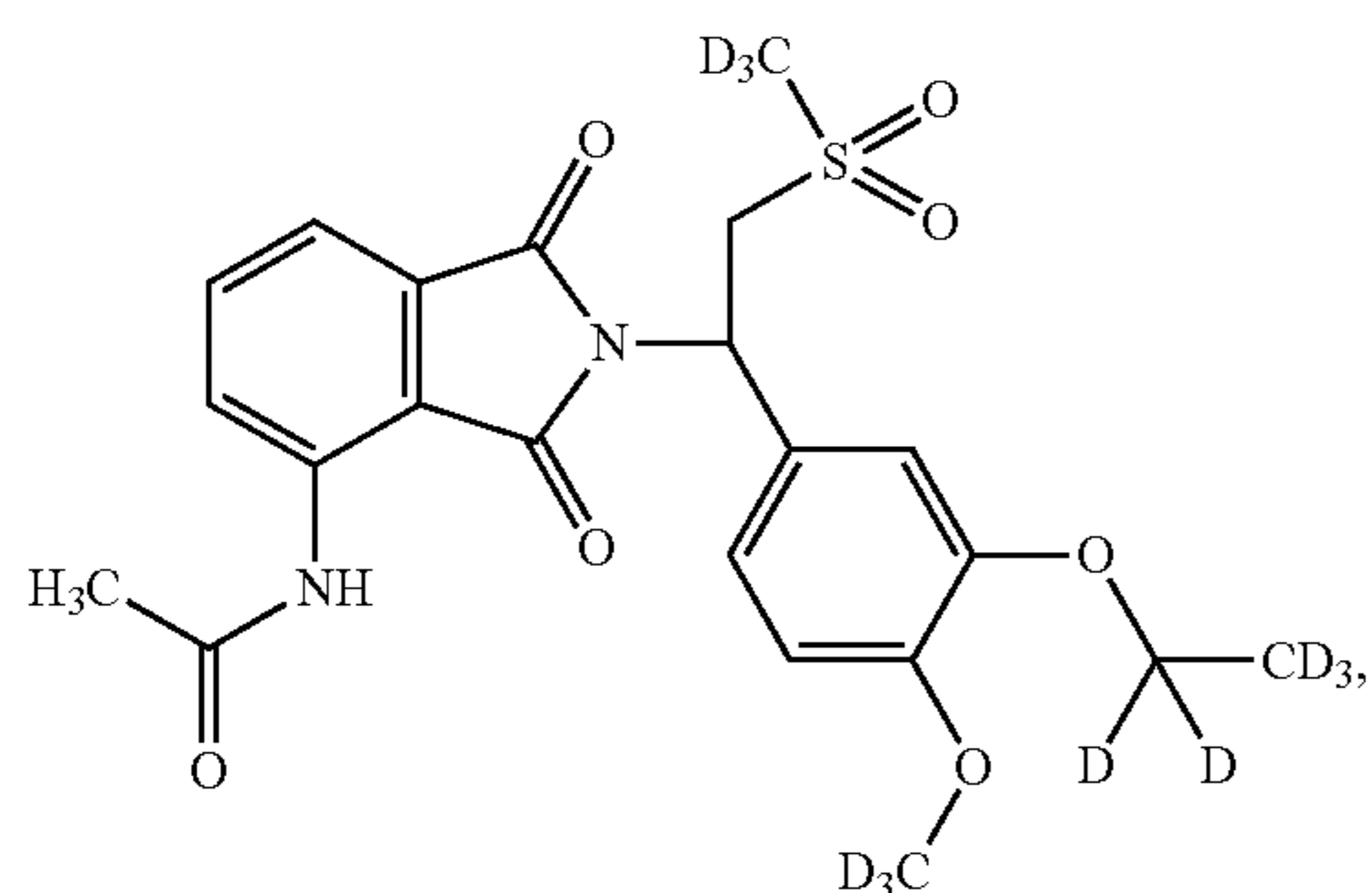
Compound 106
