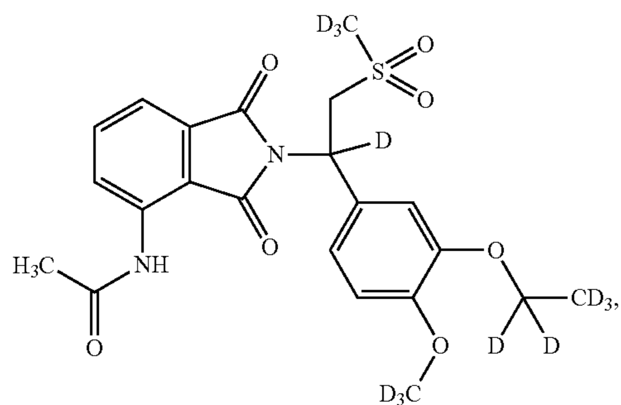
Compound 105
