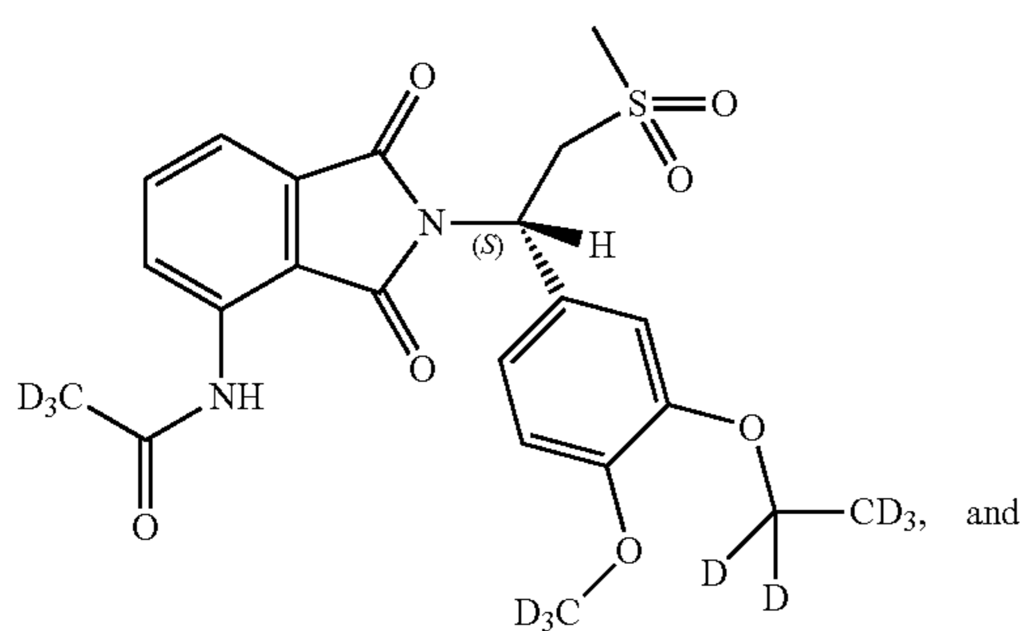
Compound 115a
