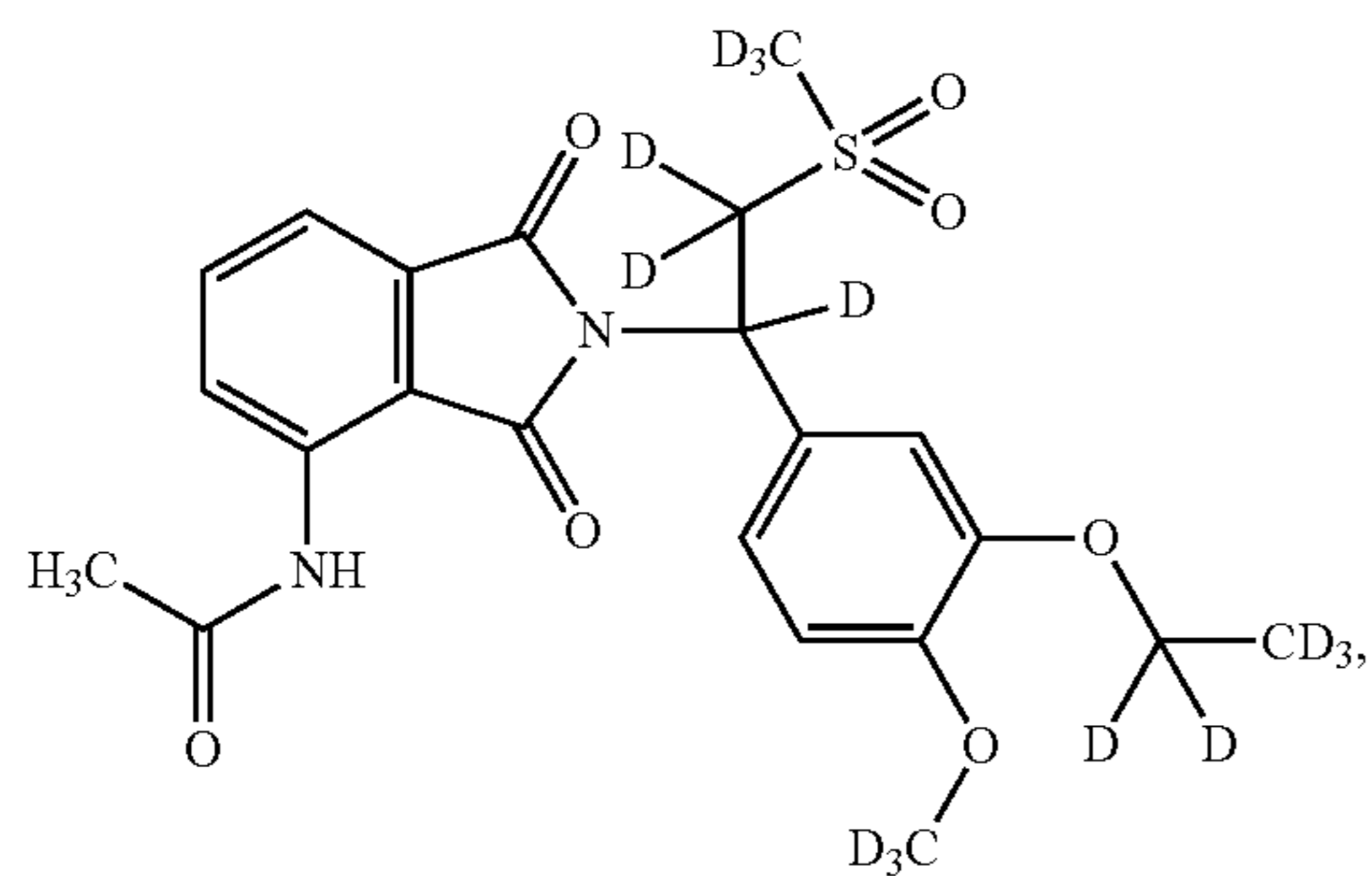
Compound 104
