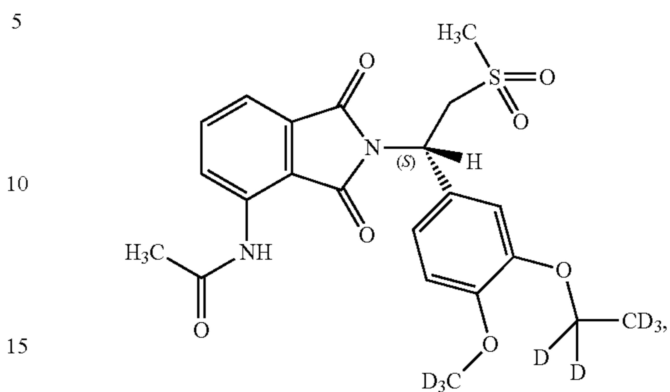
Compound 110a
