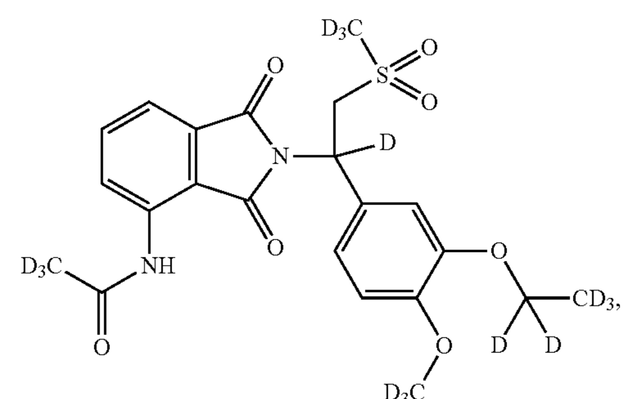
Compound 102
