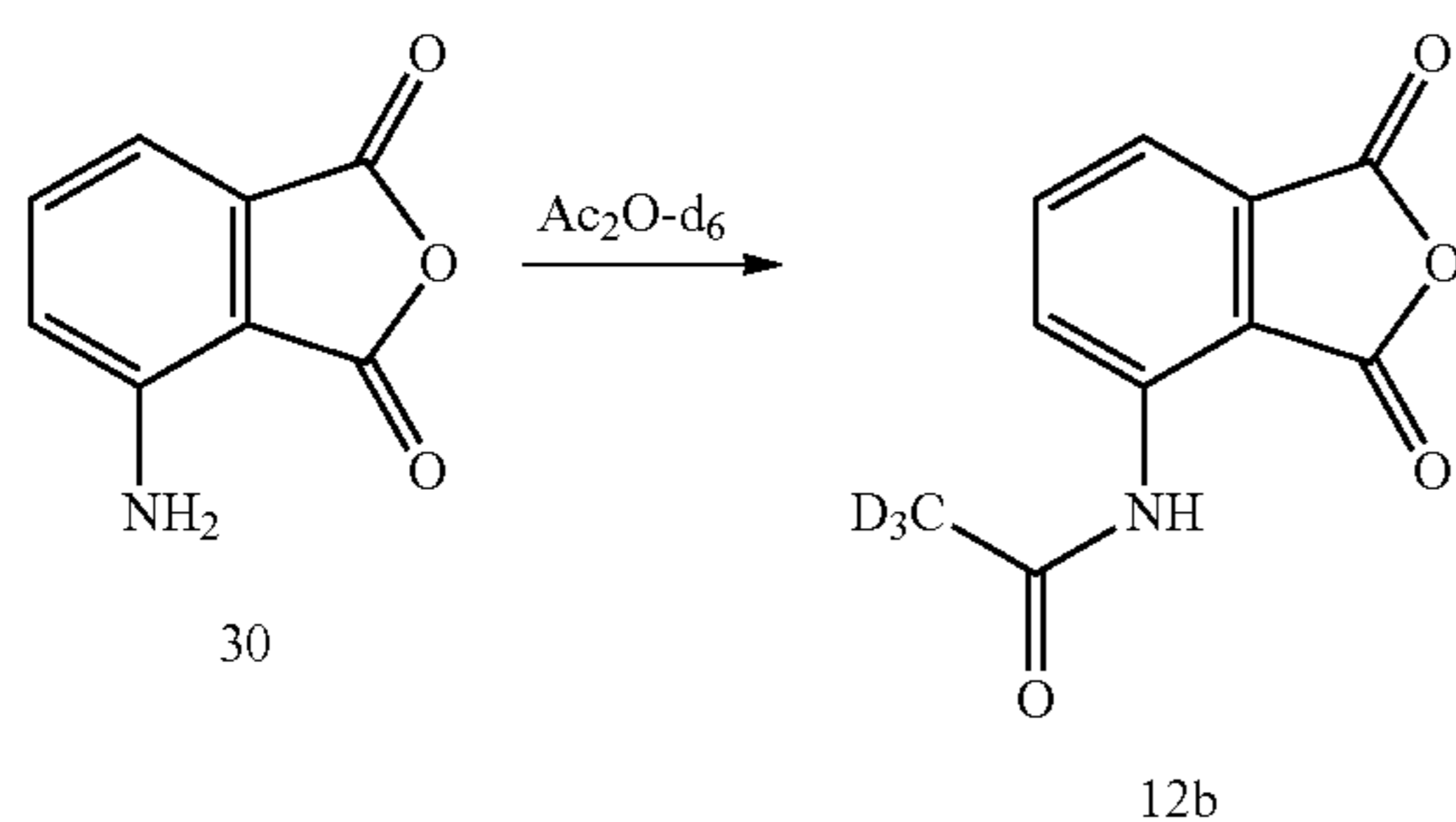
Scheme 8. Preparation of 12b.
