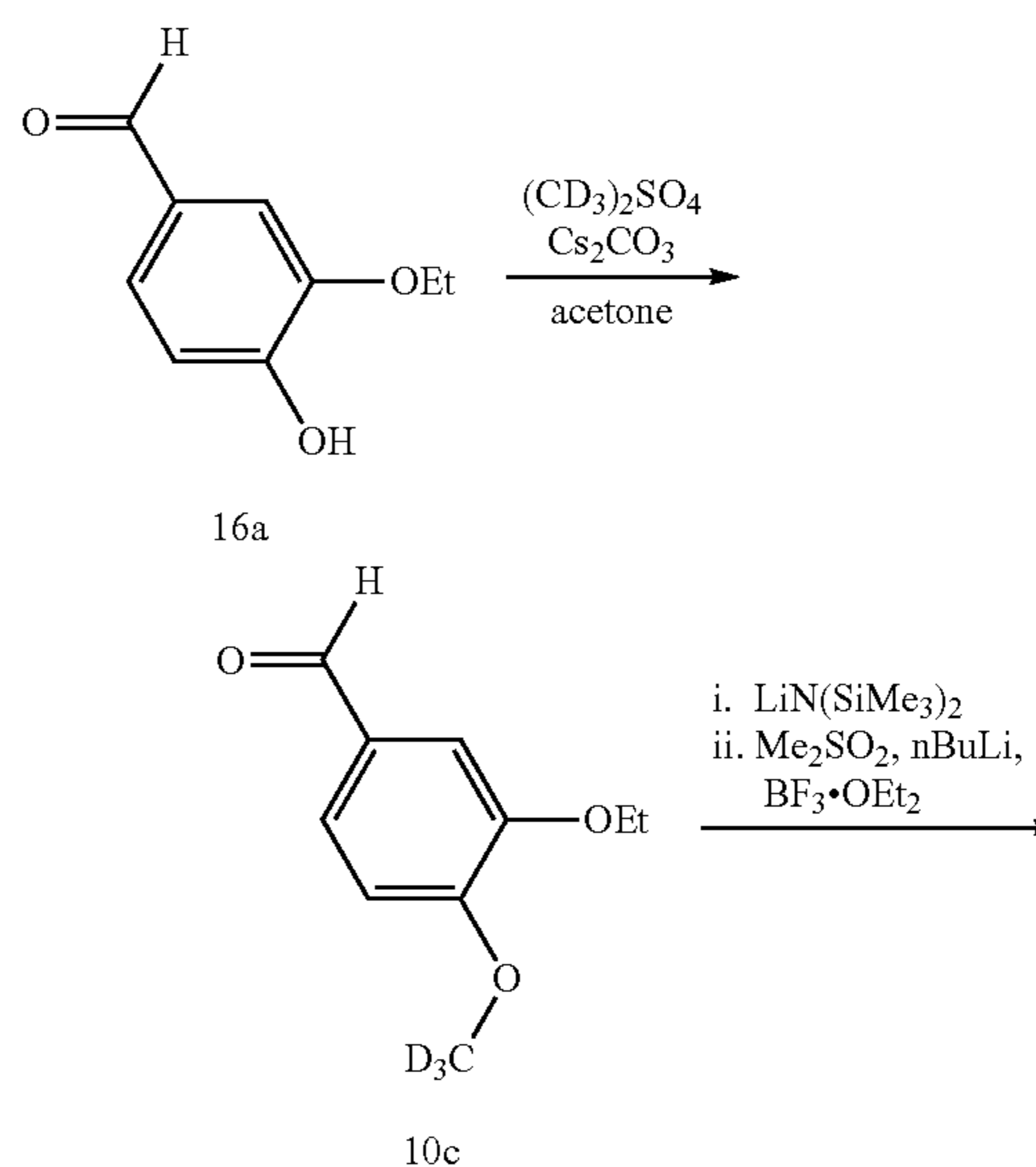
Scheme 6. Preparation of Compound 114a.
