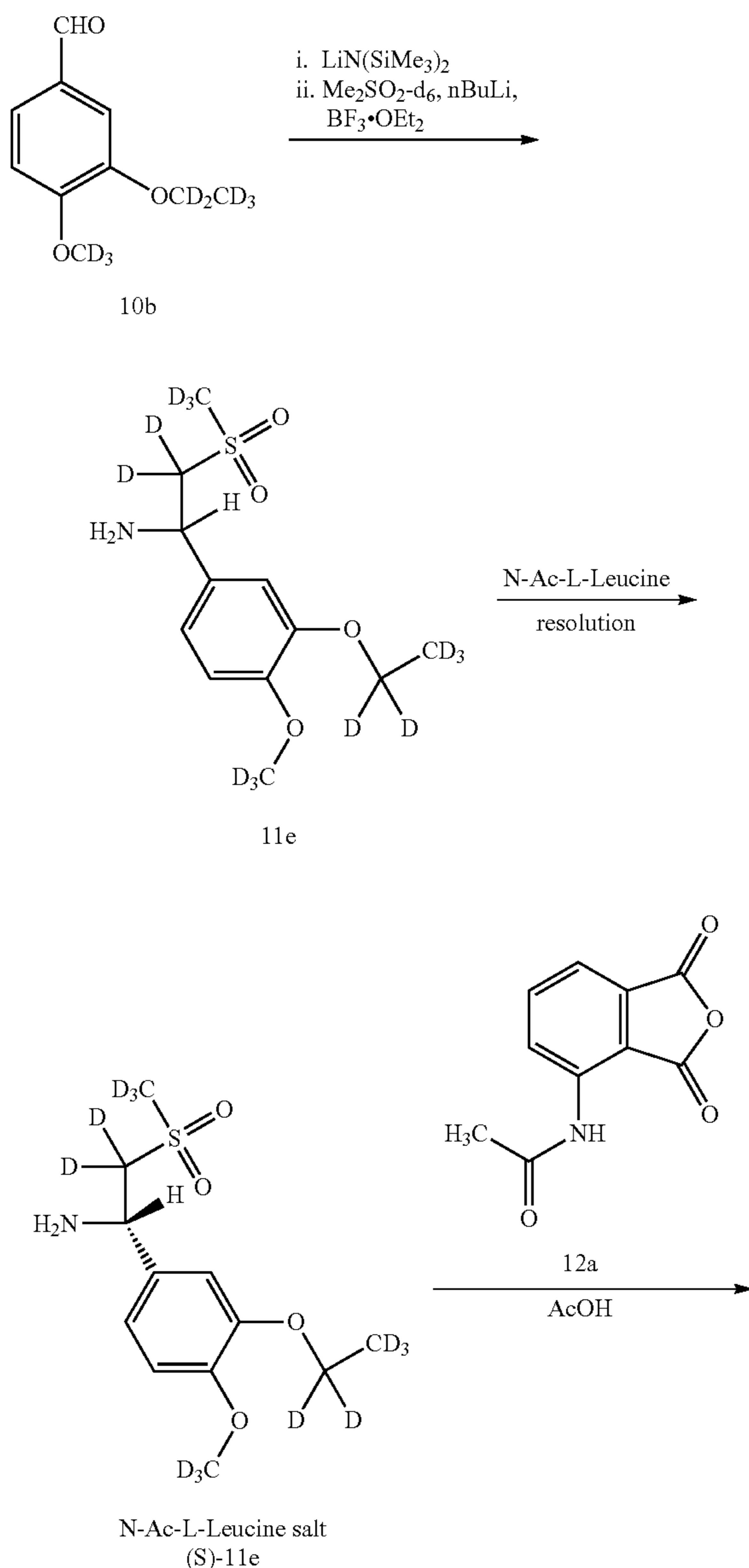
Scheme 9. Preparation of Compound 116a.
