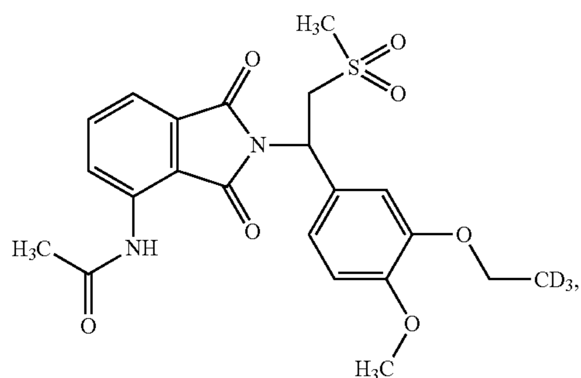
Compound 112
