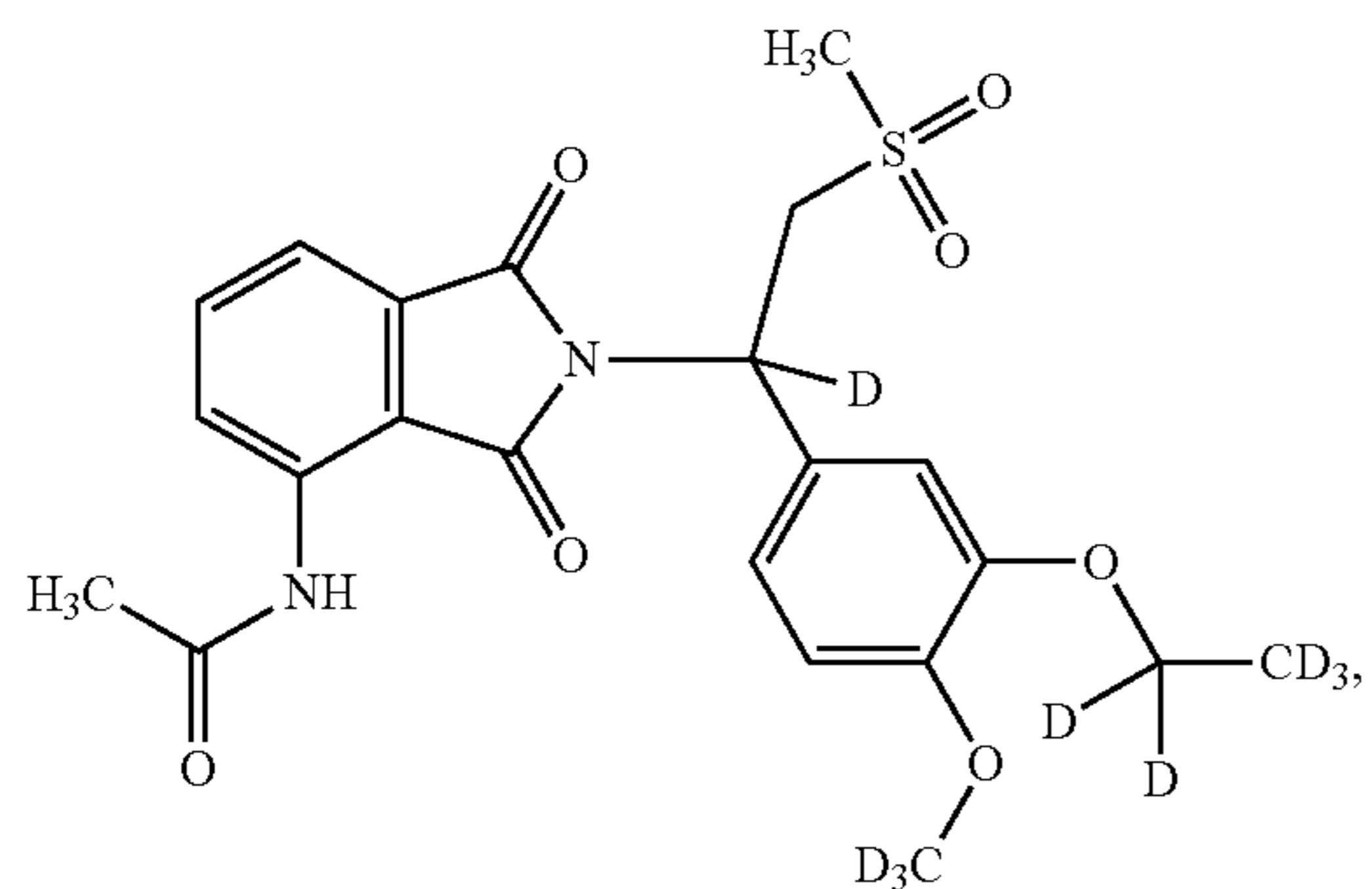
Compound 113
