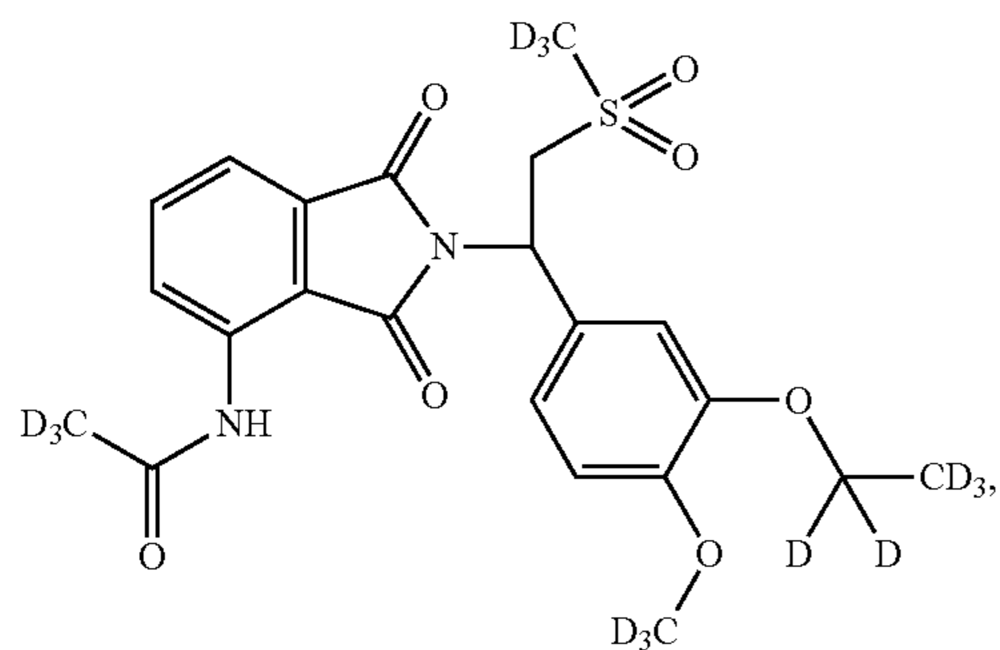
Compound 103
