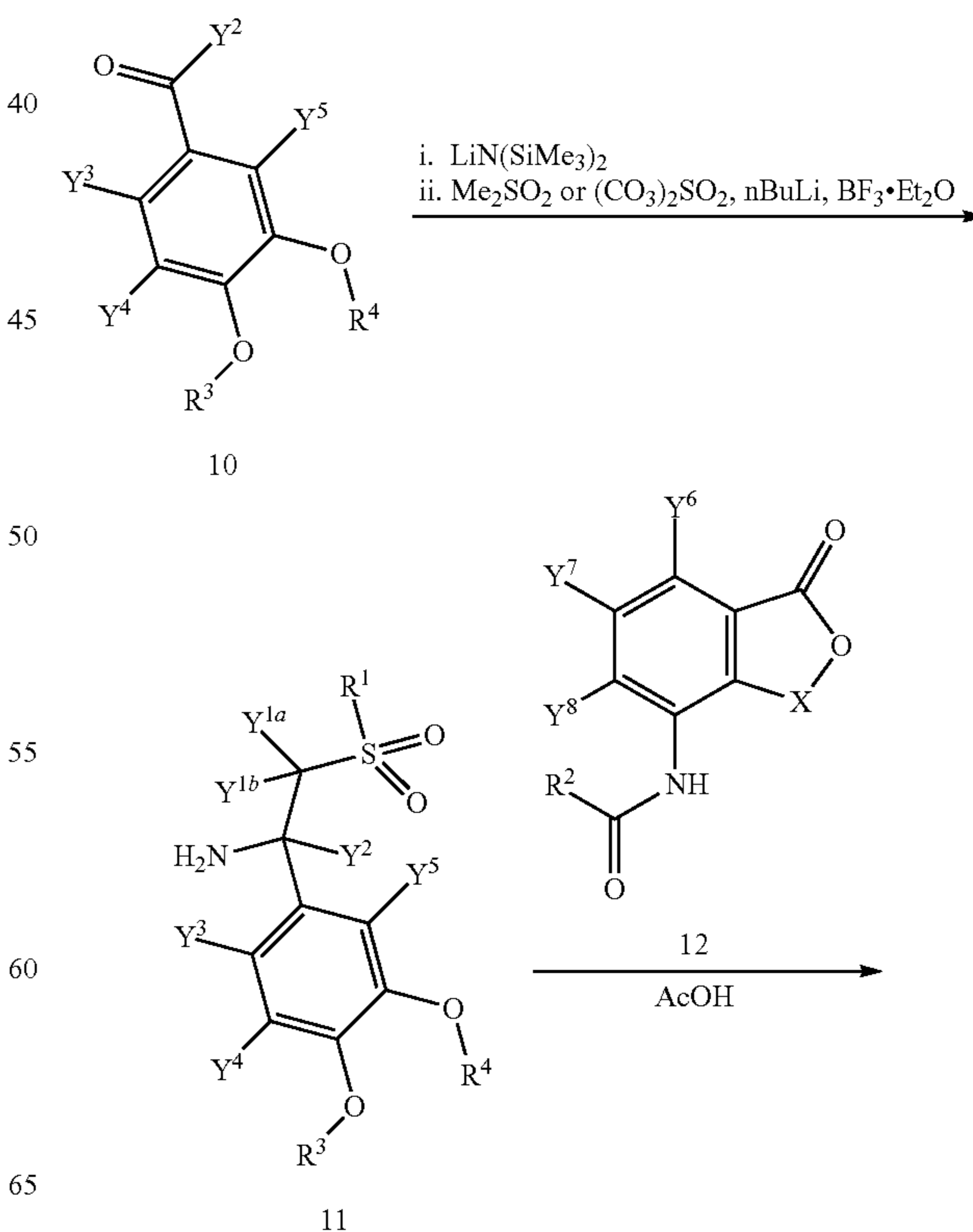
Scheme 1: General Route to Compounds of Formula I.
