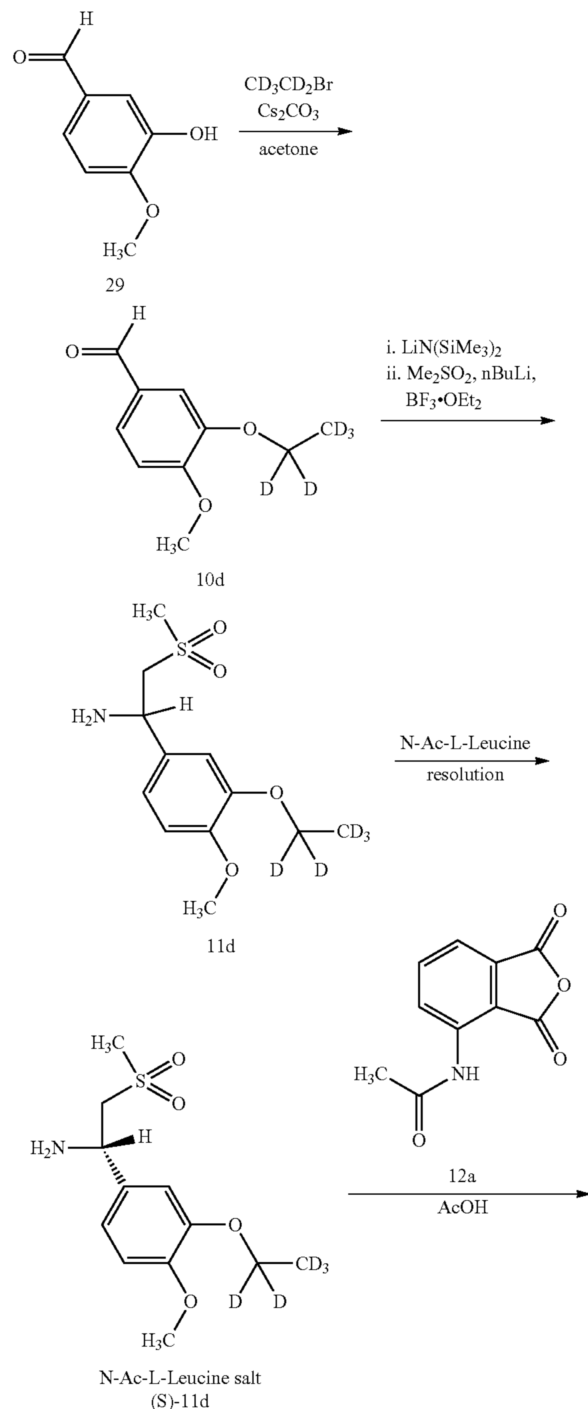
Scheme 7. Preparation of Compound 110a.
