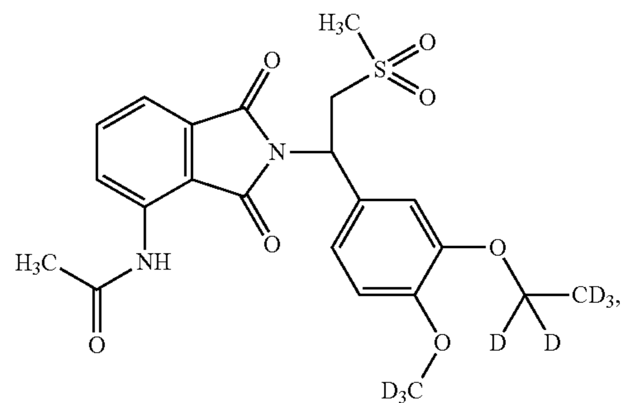
Compound 107
