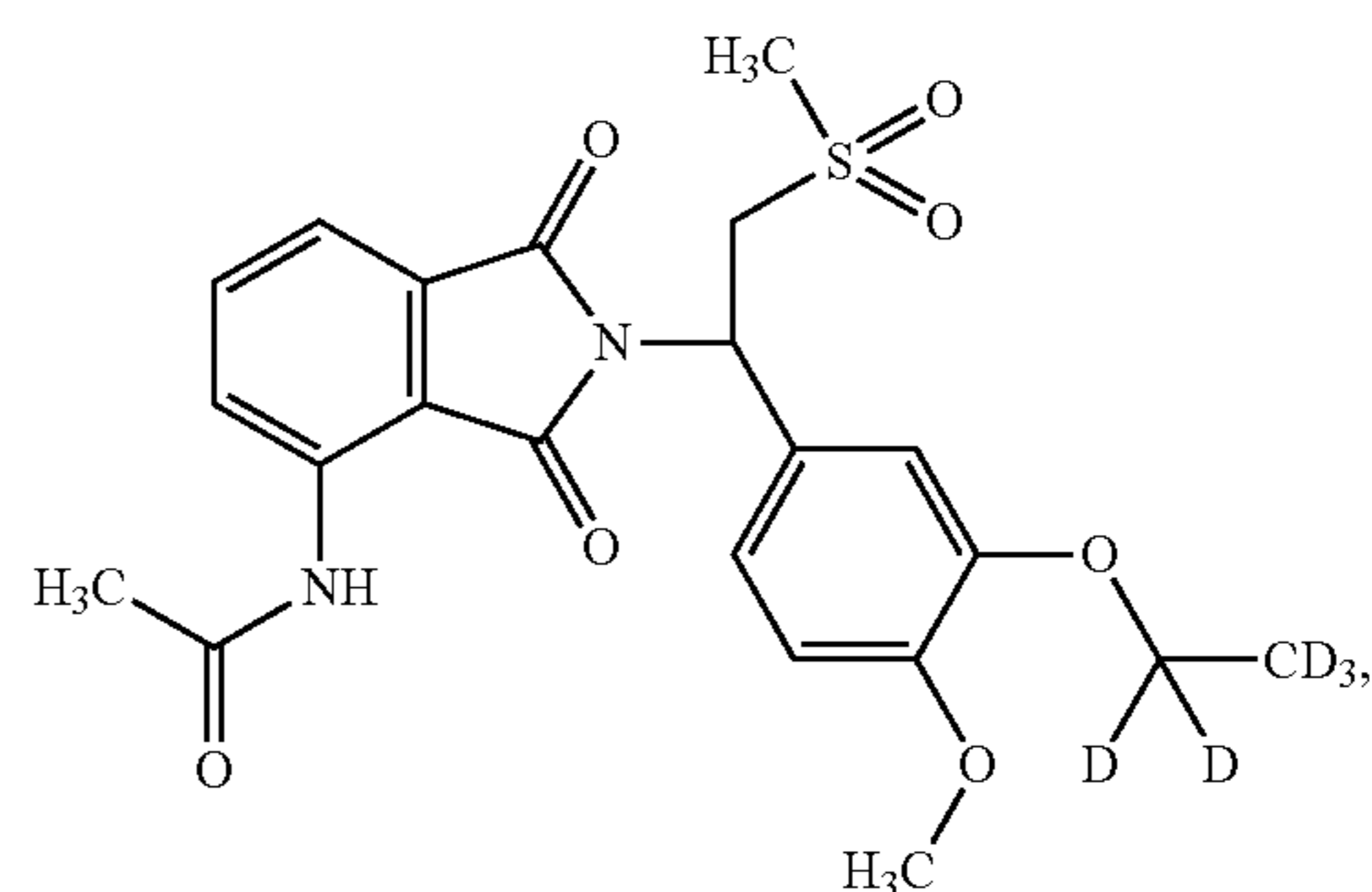
Compound 110
