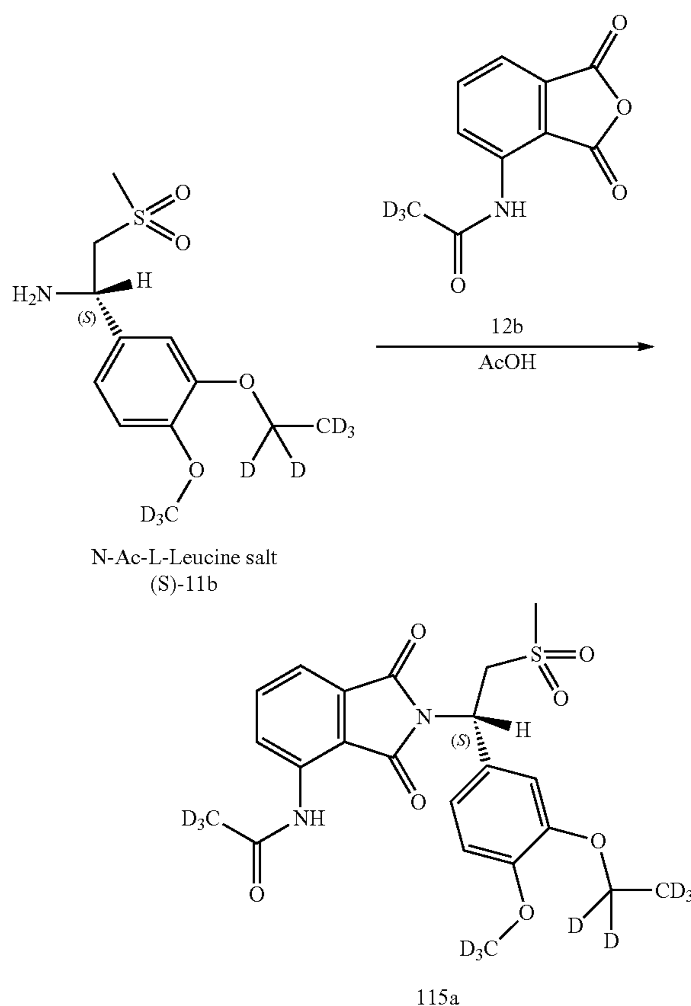
Scheme 8. Preparation of 115a.
