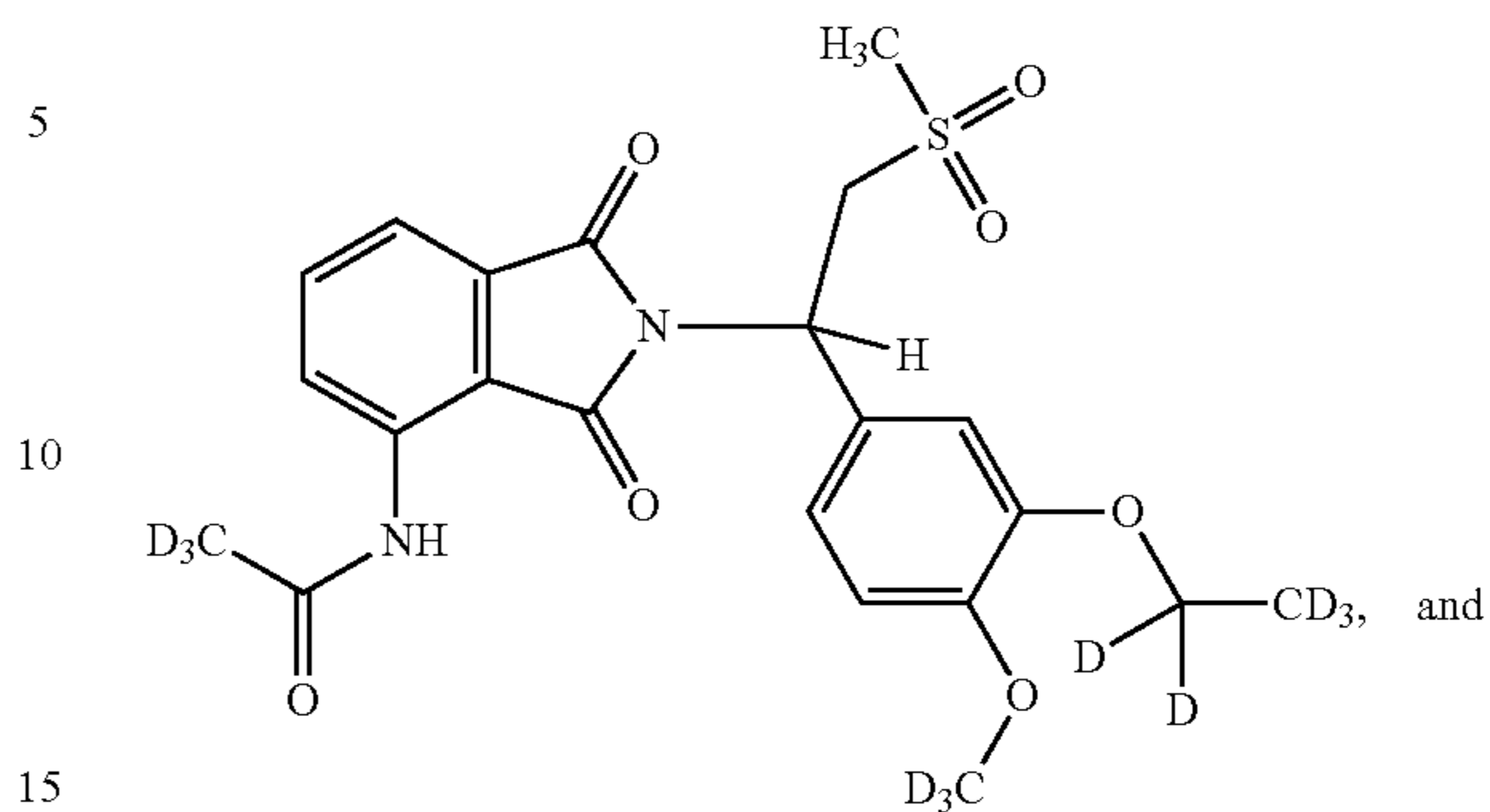
Compound 115
