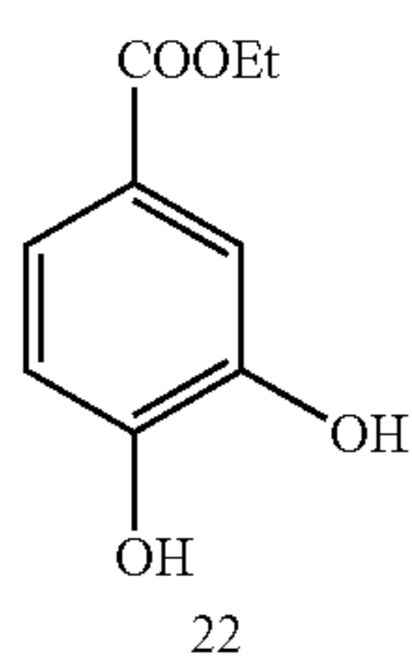
Scheme 4. Preparation of Compound 113a.
