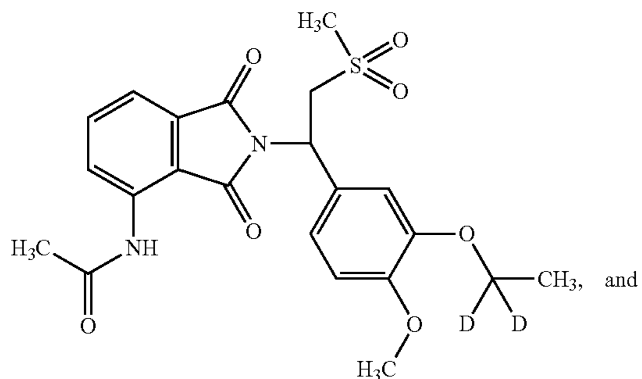
Compound 111
