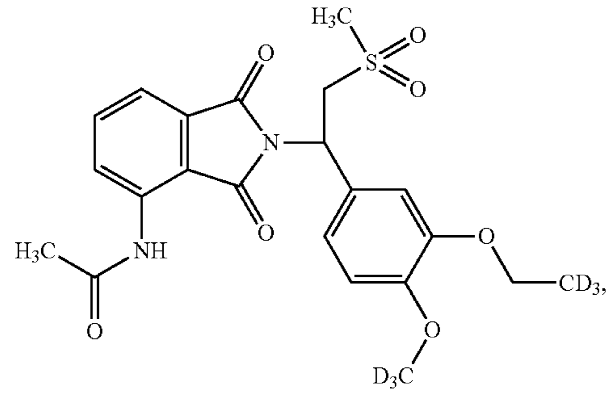
Compound 109
