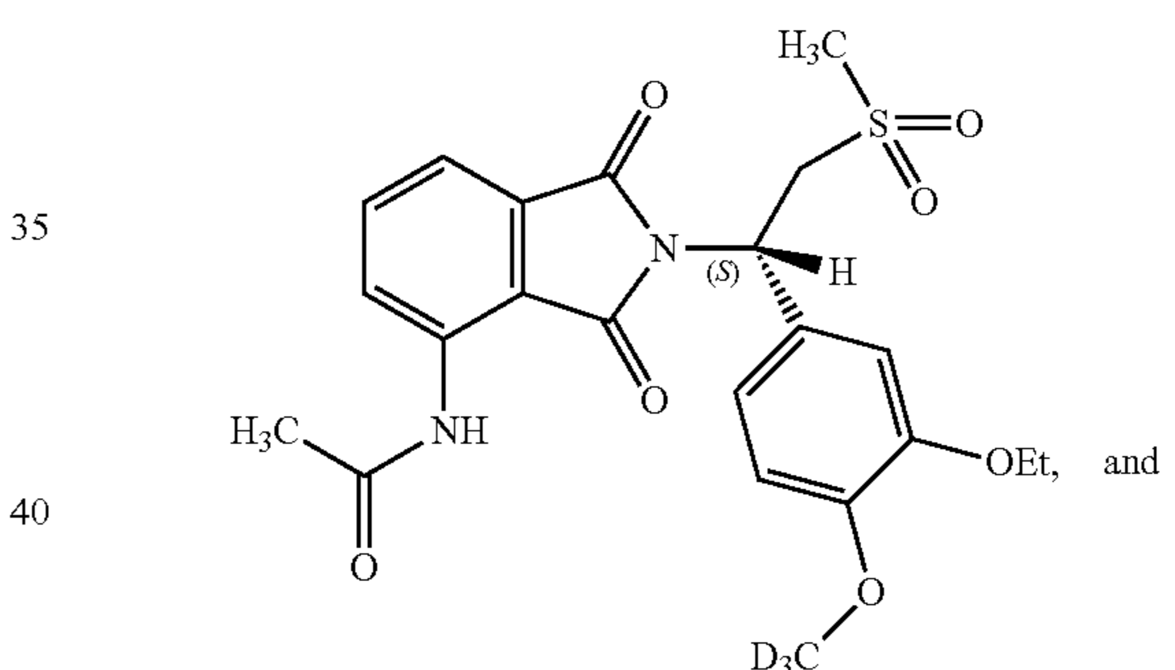
Compound 115a
