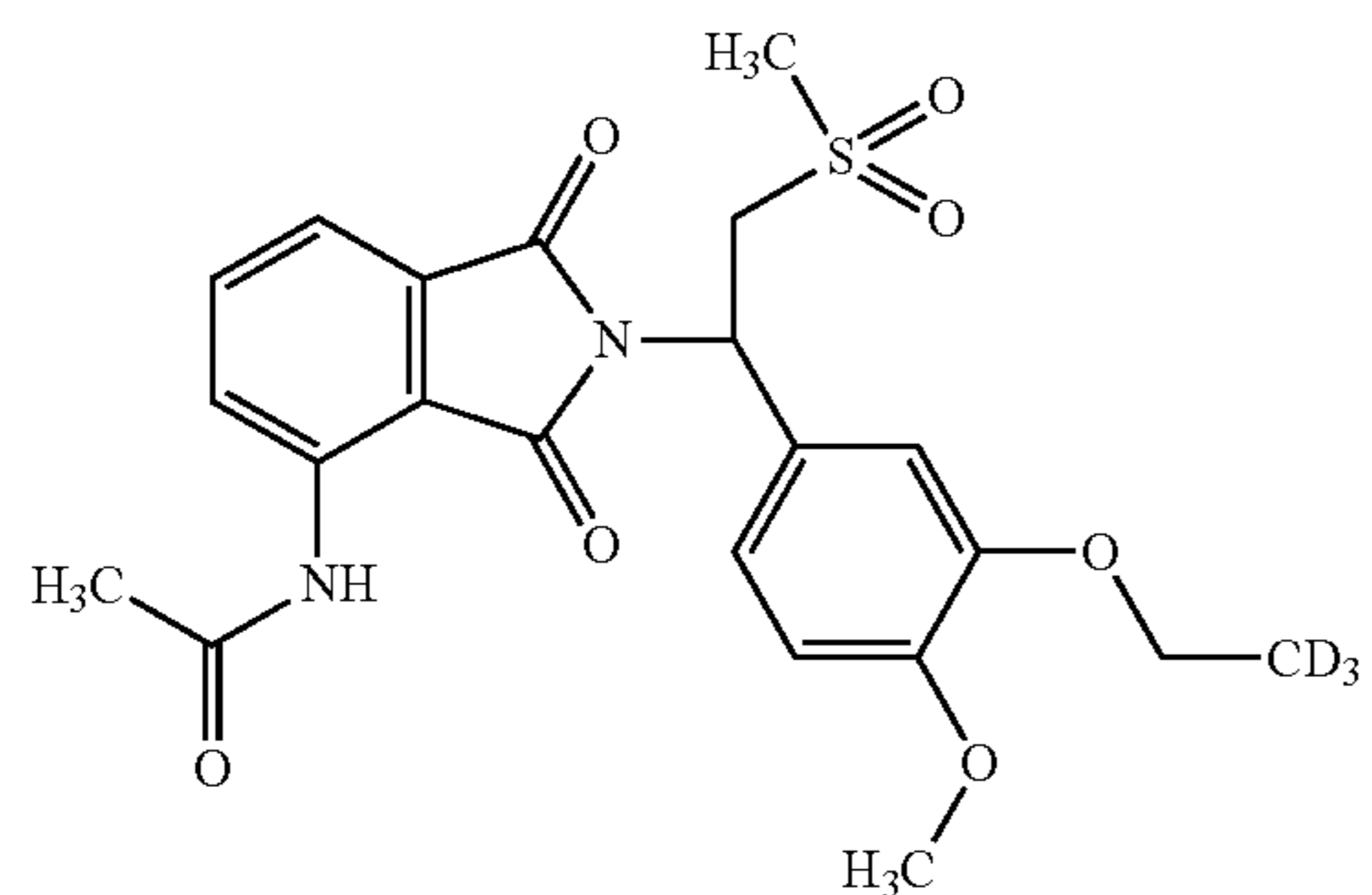
Compound 112
