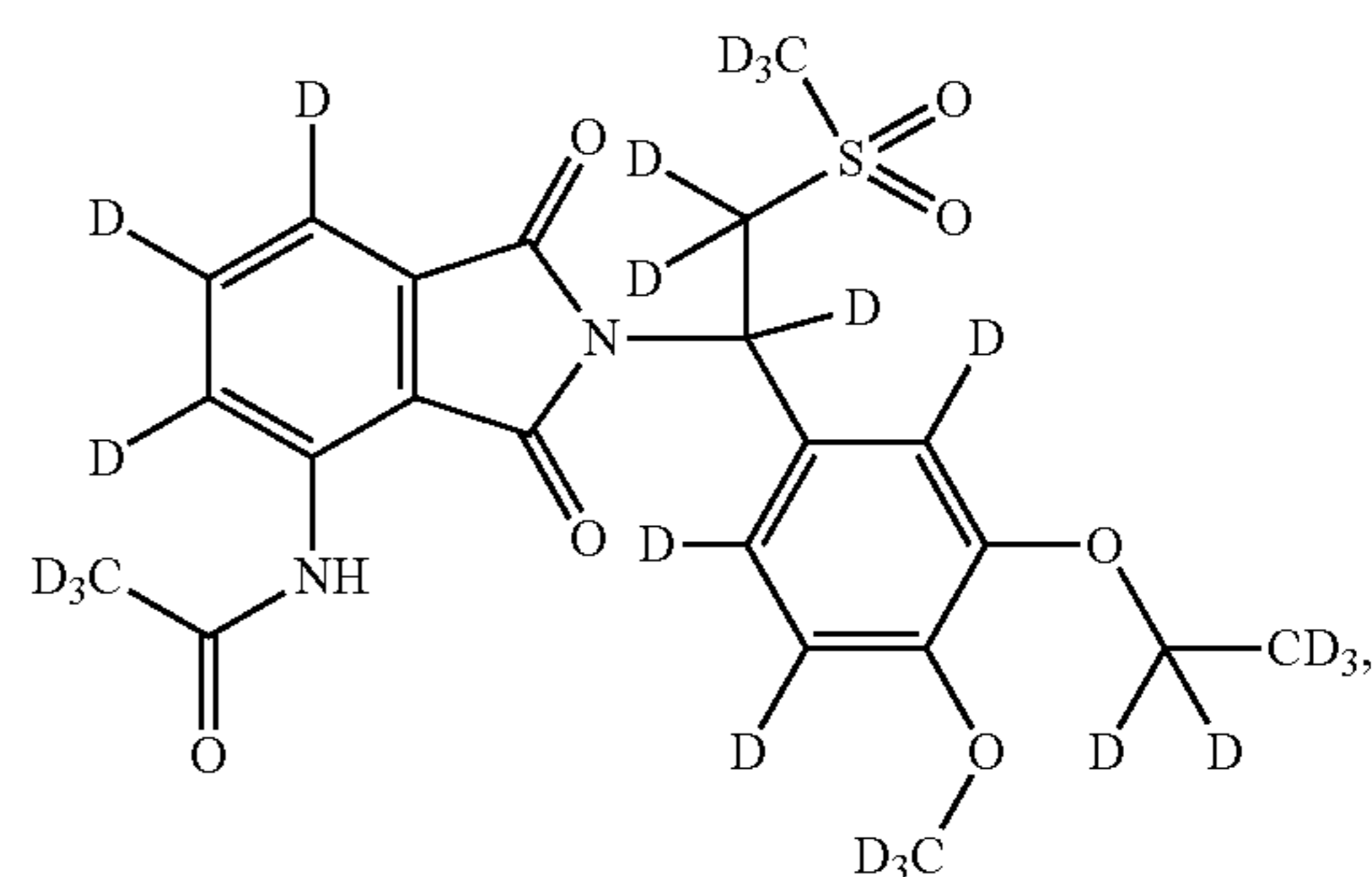
Compound 101
