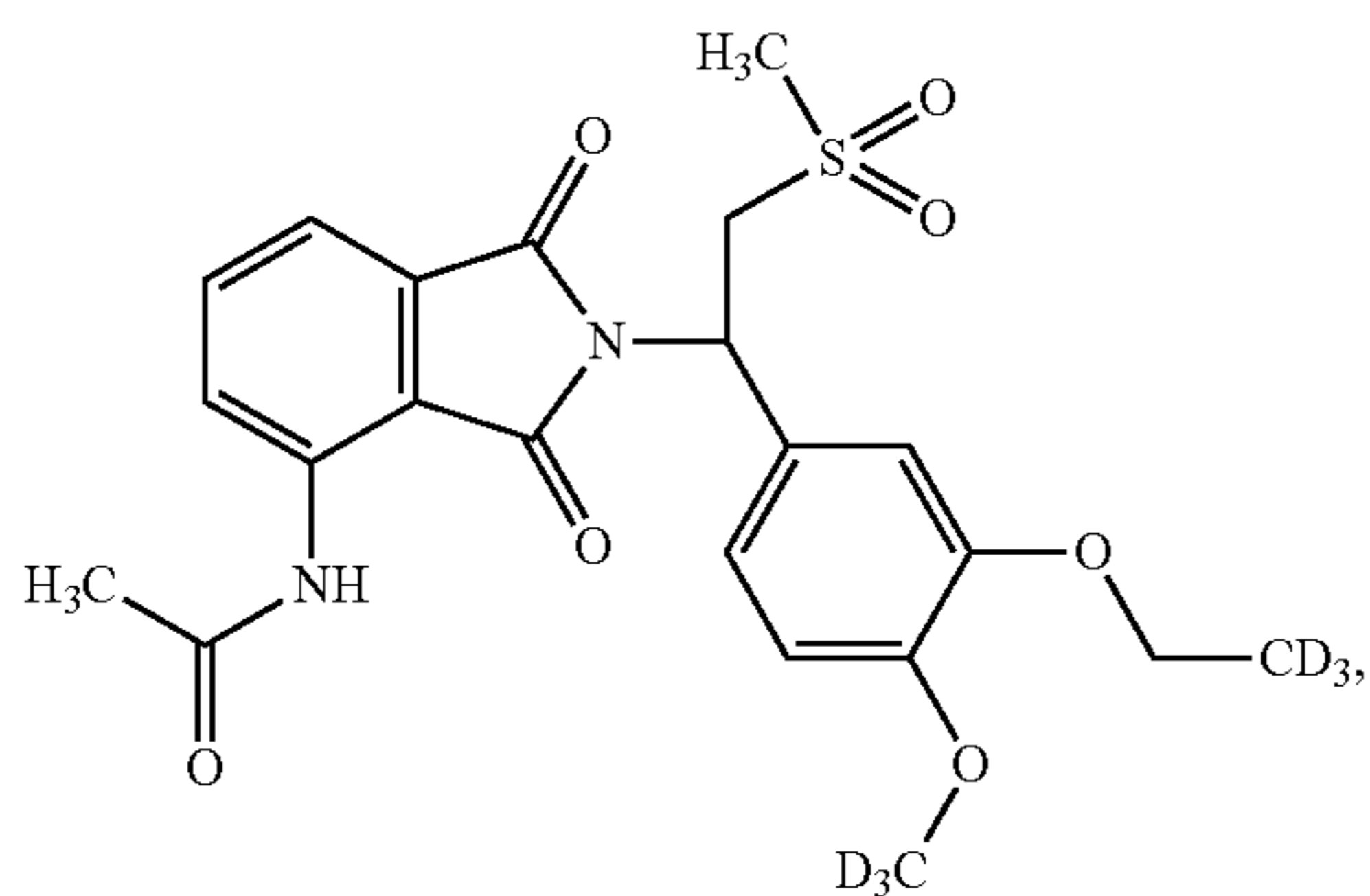
Compound 109
