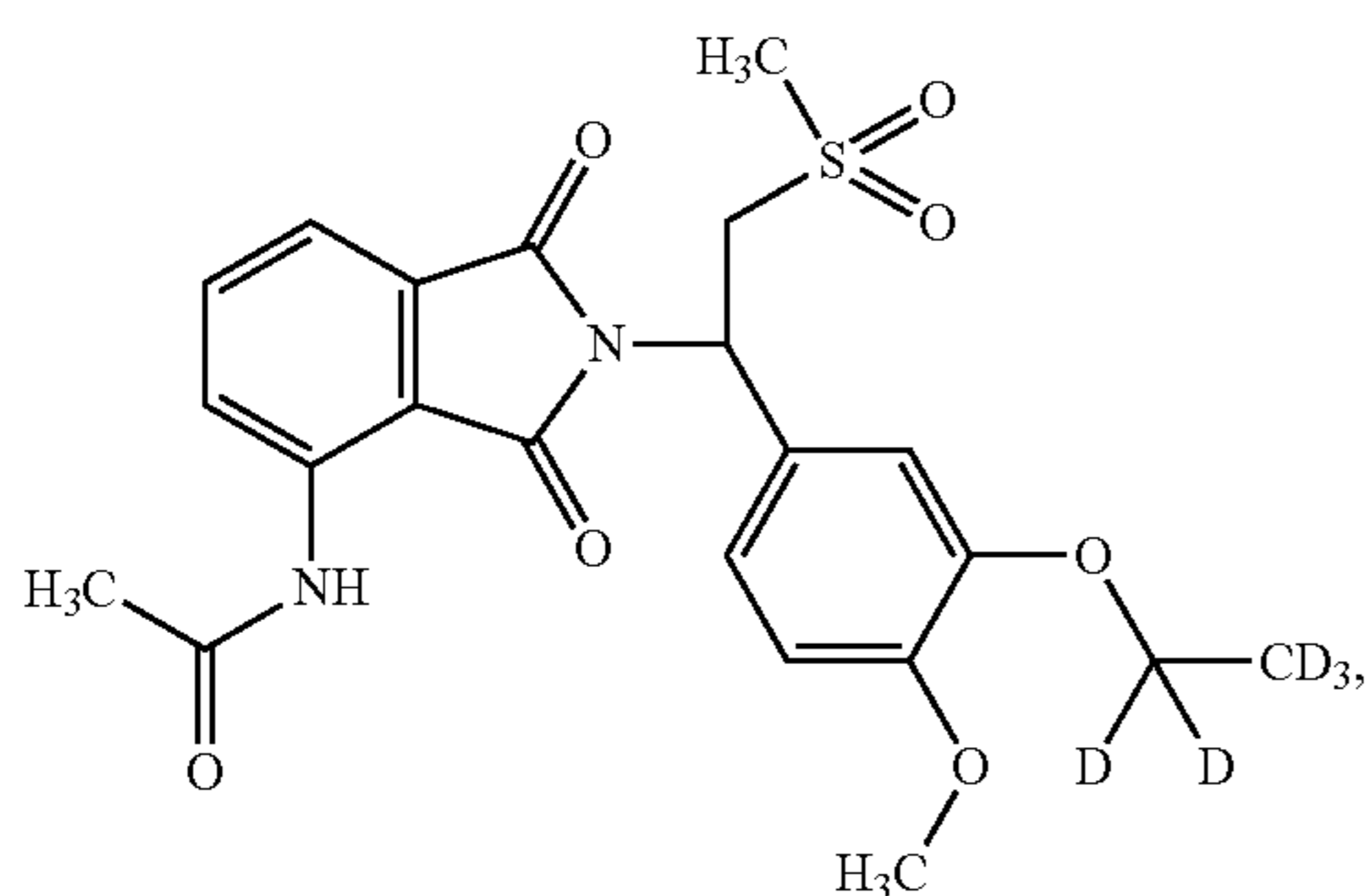
Compound 110
