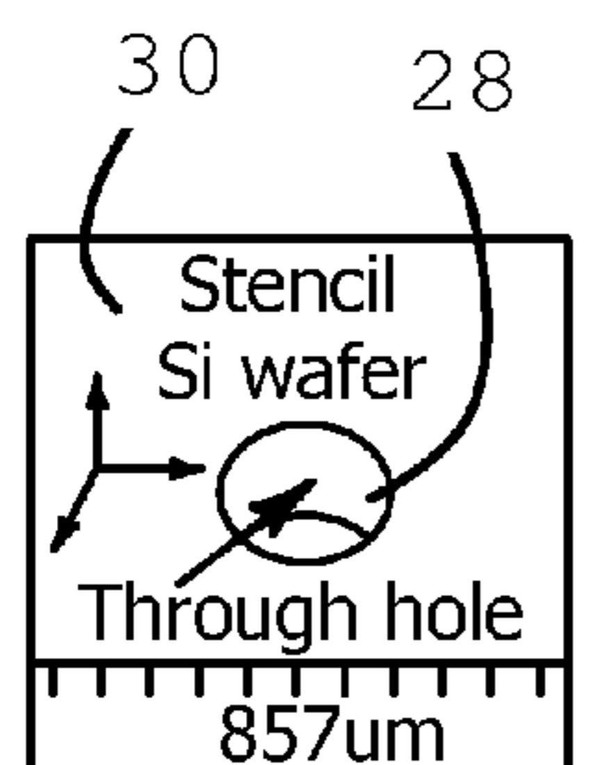
Initial step. Glass wafer underneath the stencil silicon wafer.
