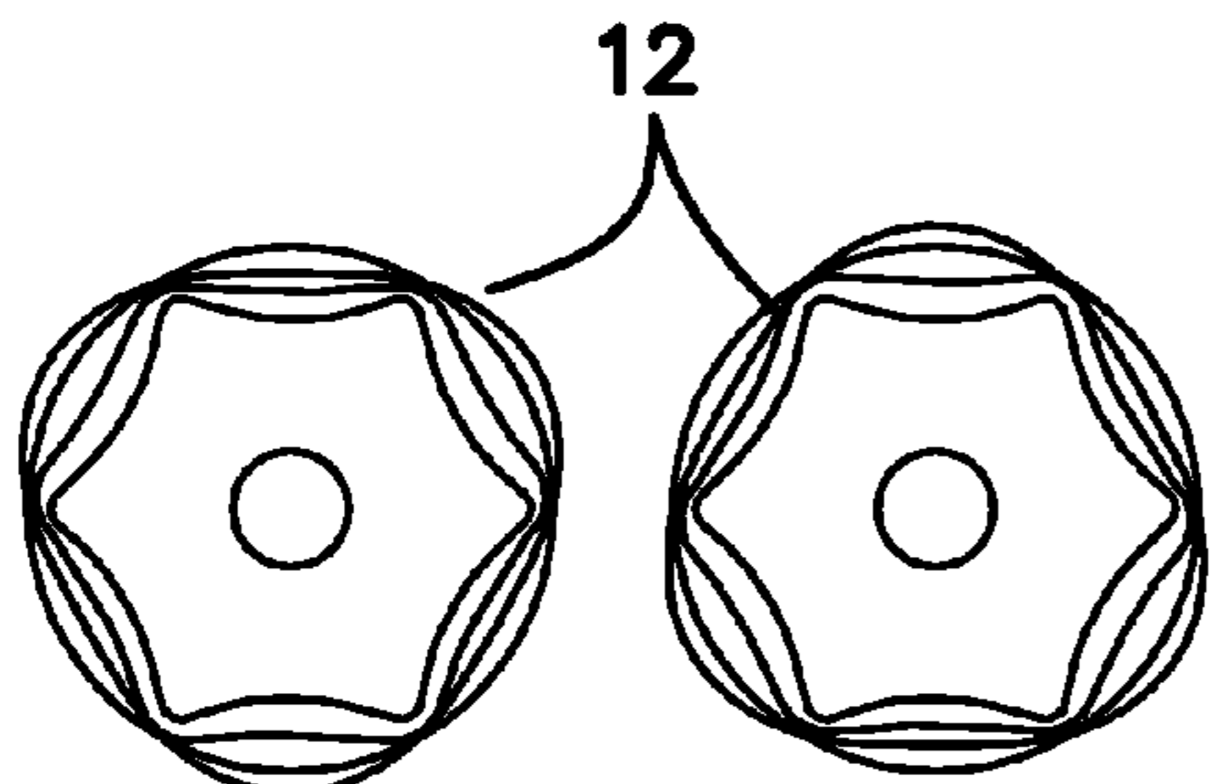
Half-periods of vibration: third mode
