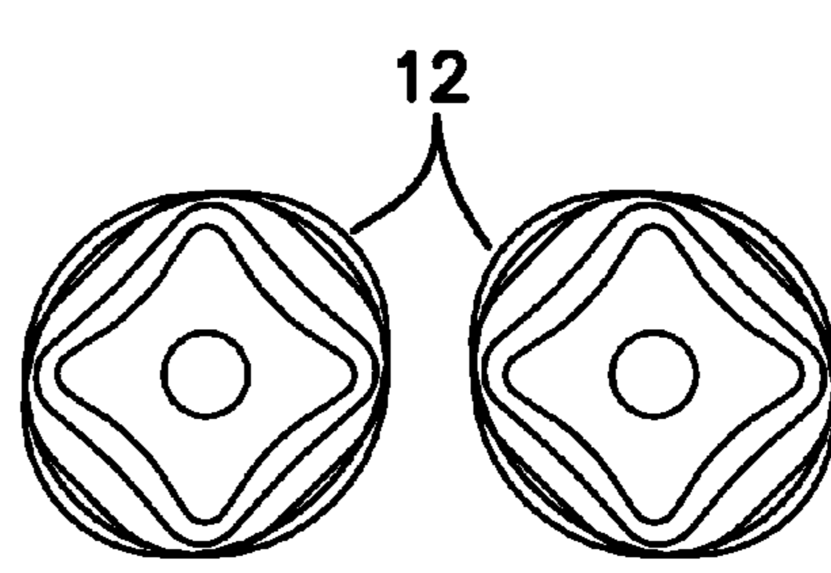
Half-periods of vibration: second mode
