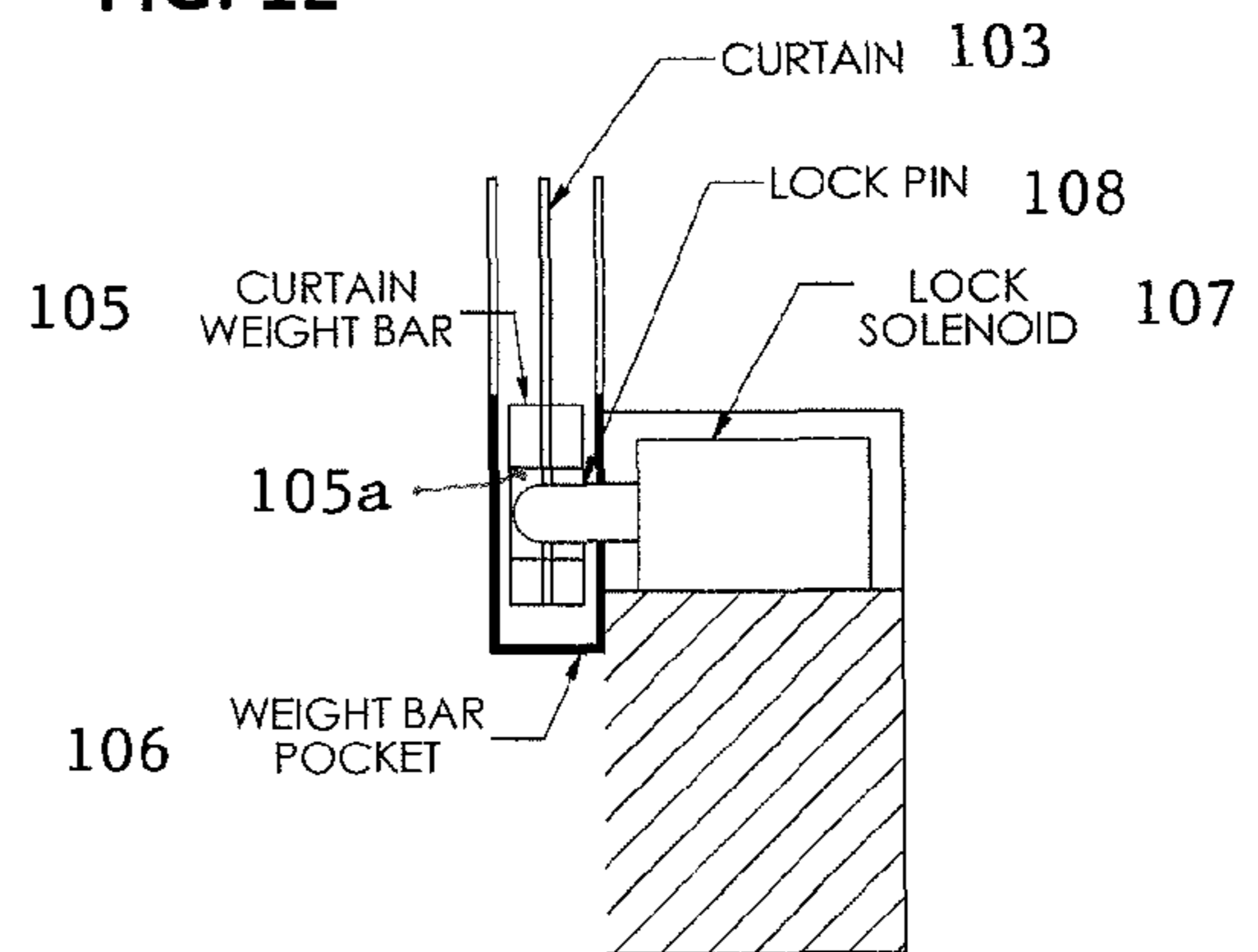
DETAIL "C"
