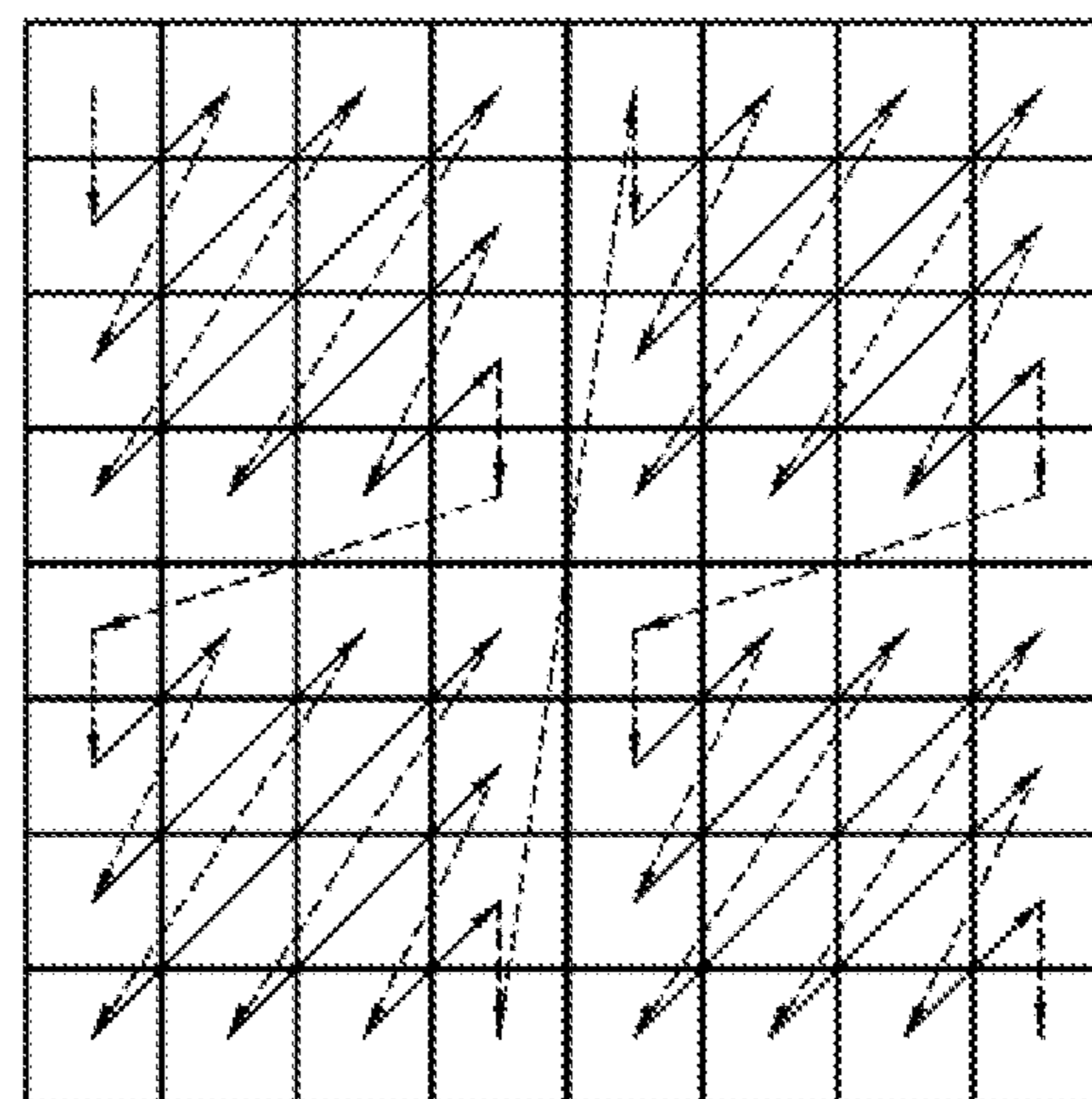
diagonal scanning (860)
