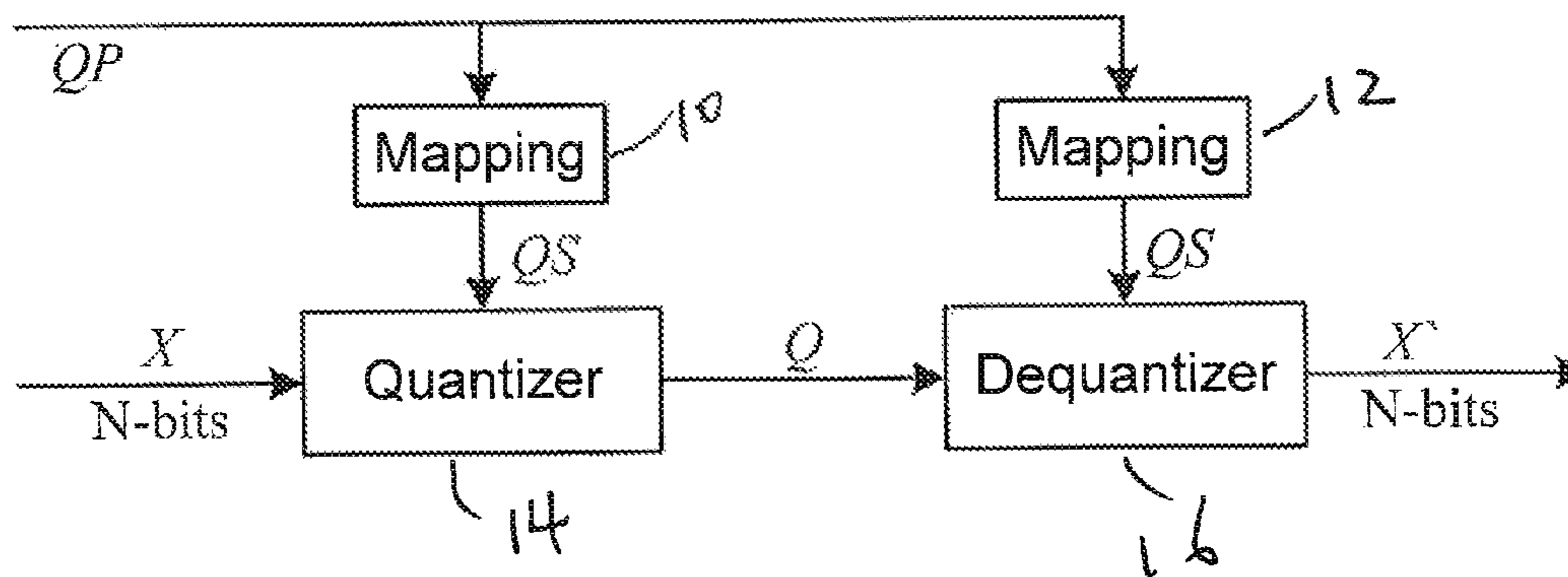
FIG. 4 Prior Art
