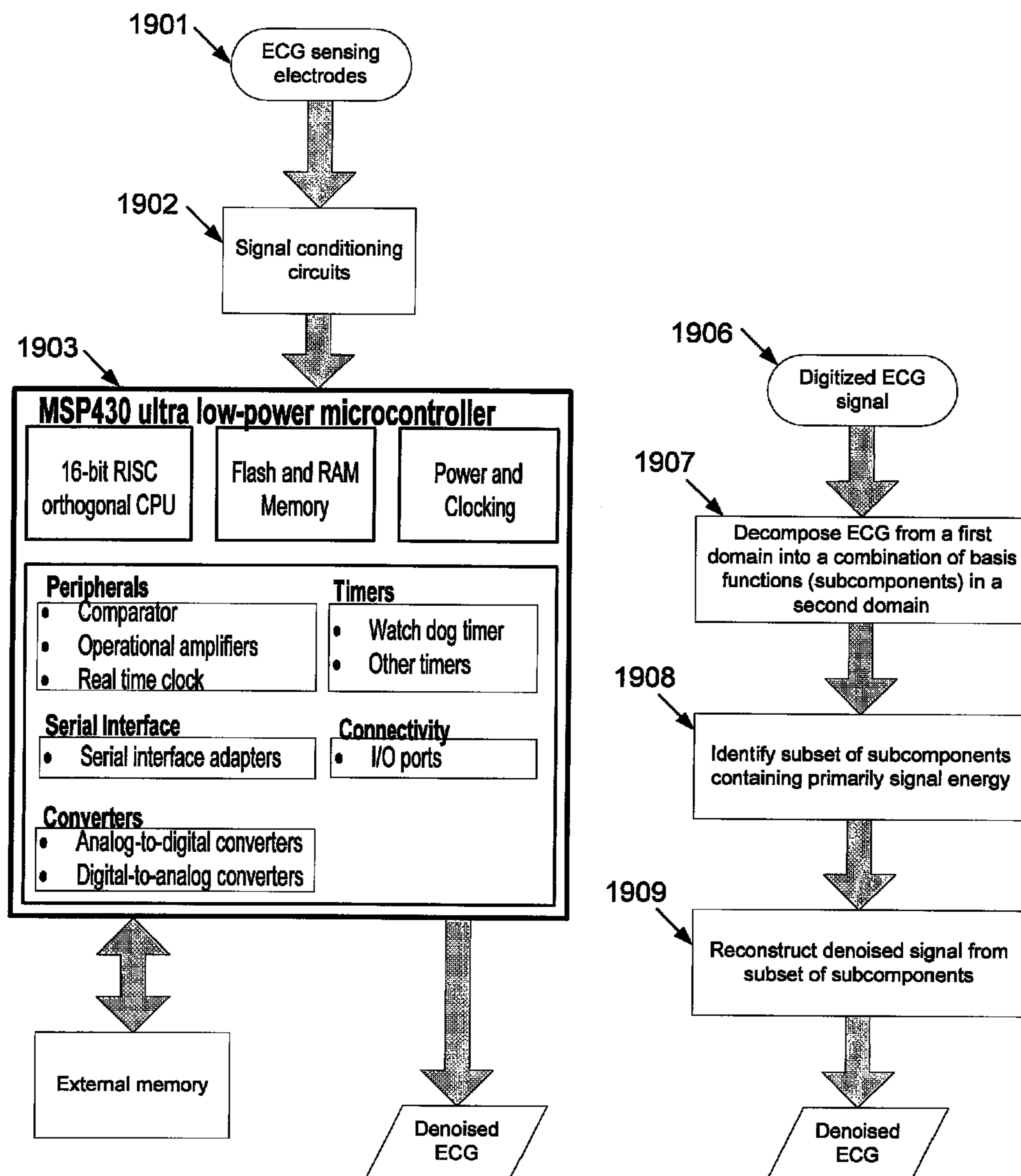
Figure 19 Apparatus for Improving SNR
