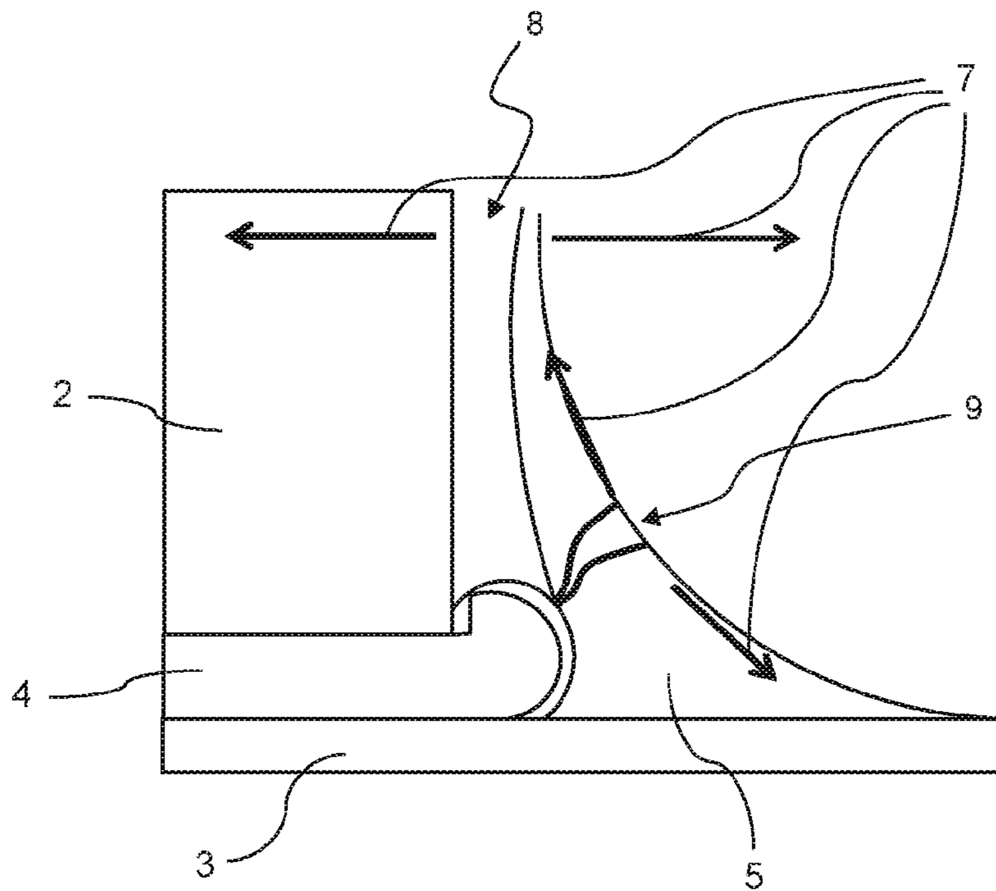
FIG. 2 (PRIOR ART)
