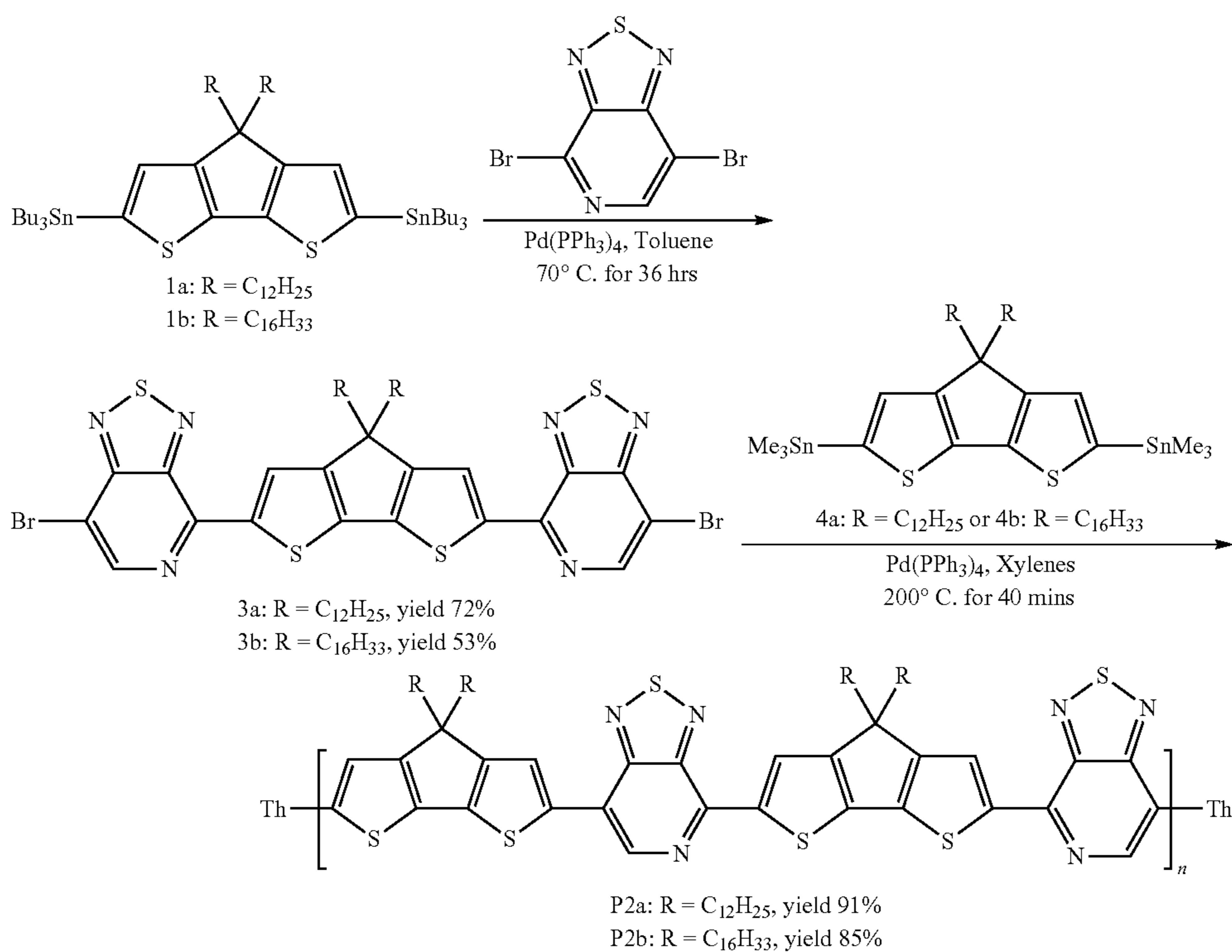
Scheme 2. Synthetic route of P2a and P2b
