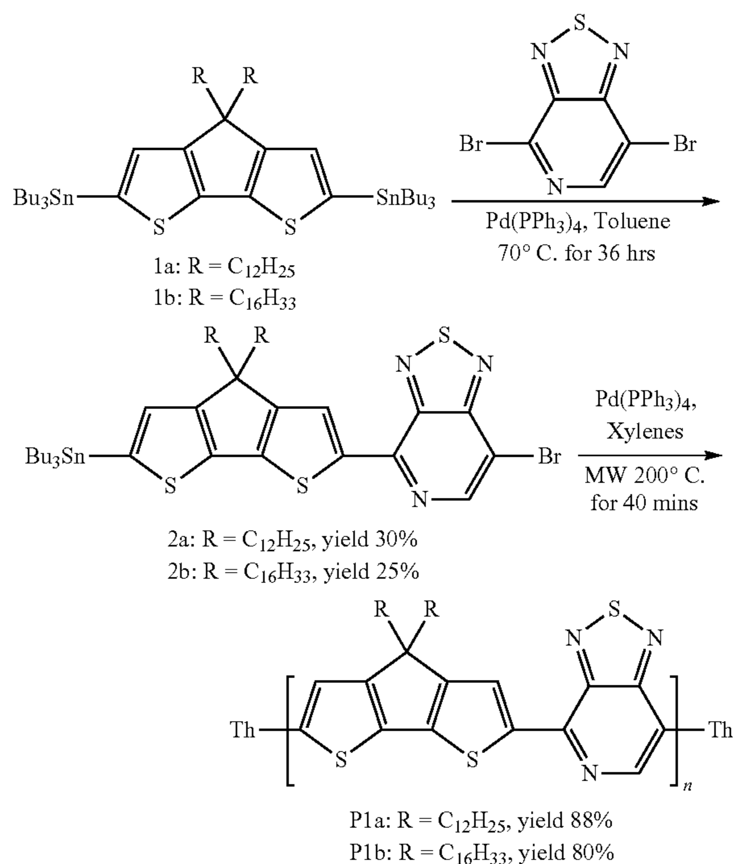
Scheme 1. Synthetic route of P1a and P1b
