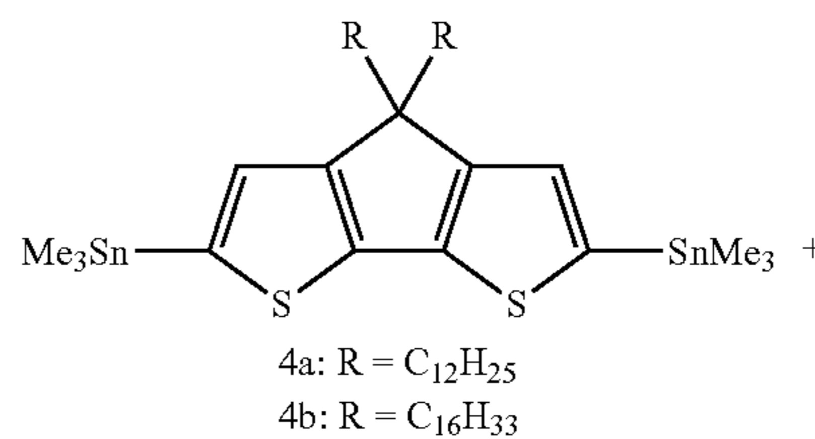
Scheme 3. Synthetic route of P3a and P3b.
