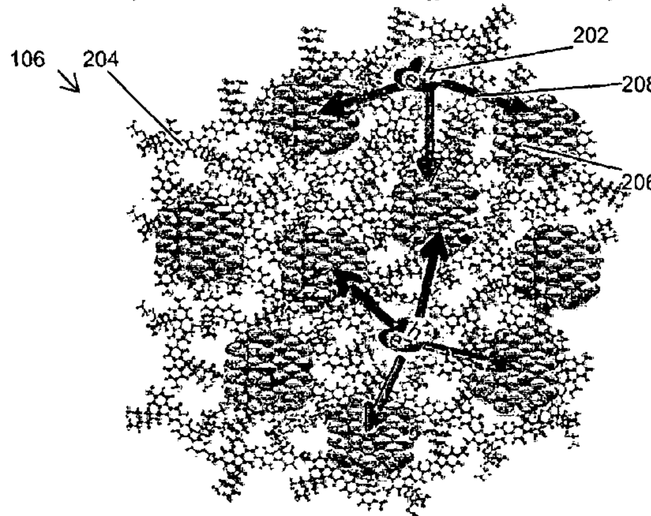
High QD loading Competition between exciton diffusion and transfer
