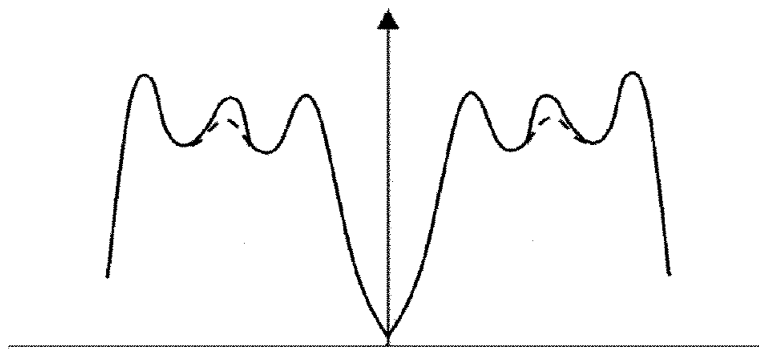
CURRENT DENSITY DISTRIBUTION IN DONUT-SHAPED PLASMA
