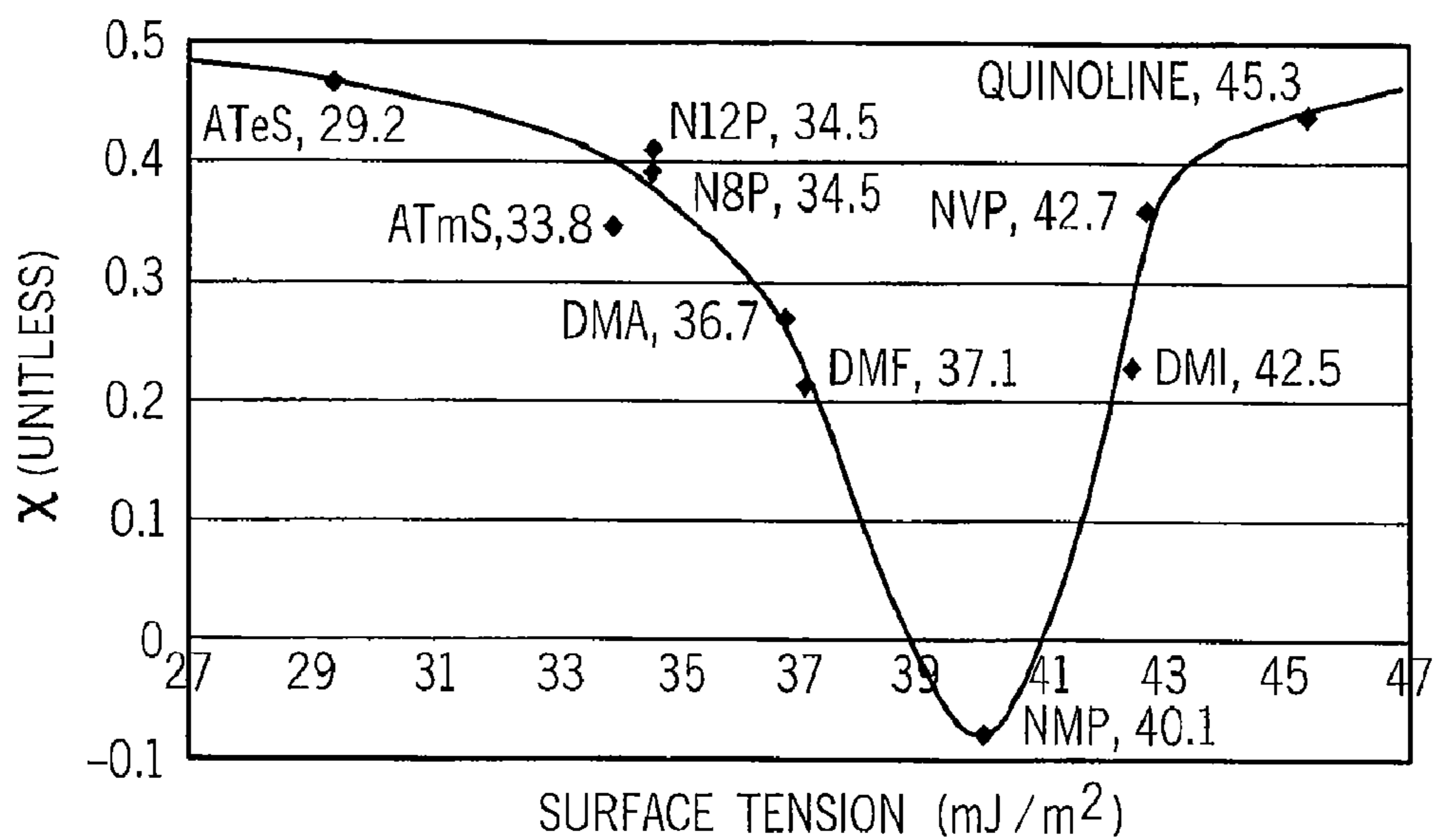
X VS. SURFACE TENSION FOR NANOTUBES IN VARIOUS SOLVENTS
