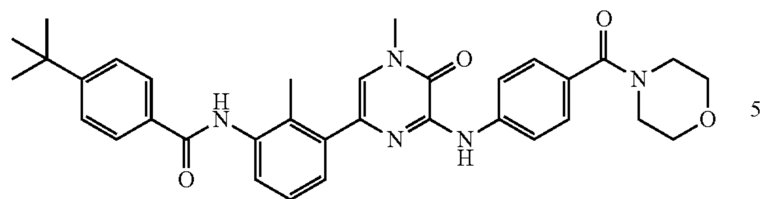
CGI-1746
