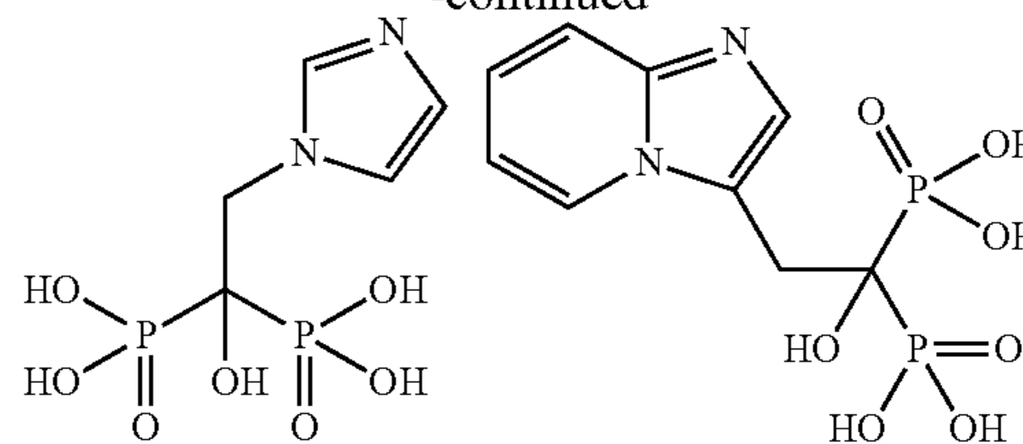
zoledronic acid
