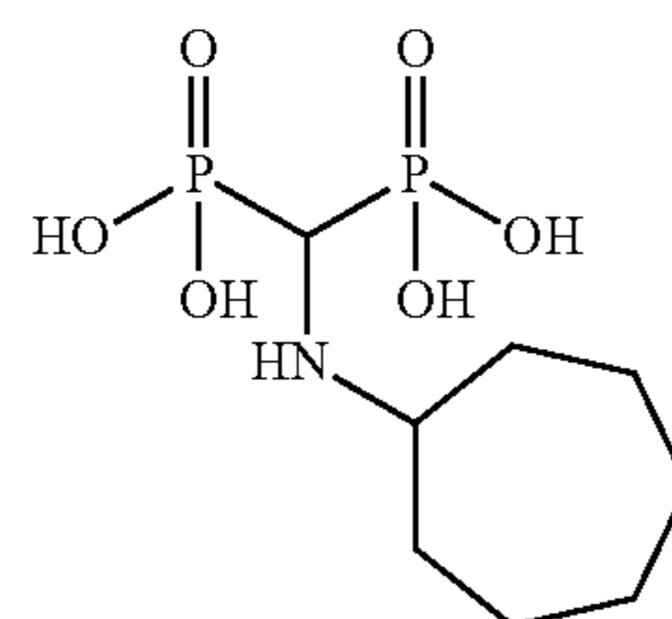
cimadronic acid
