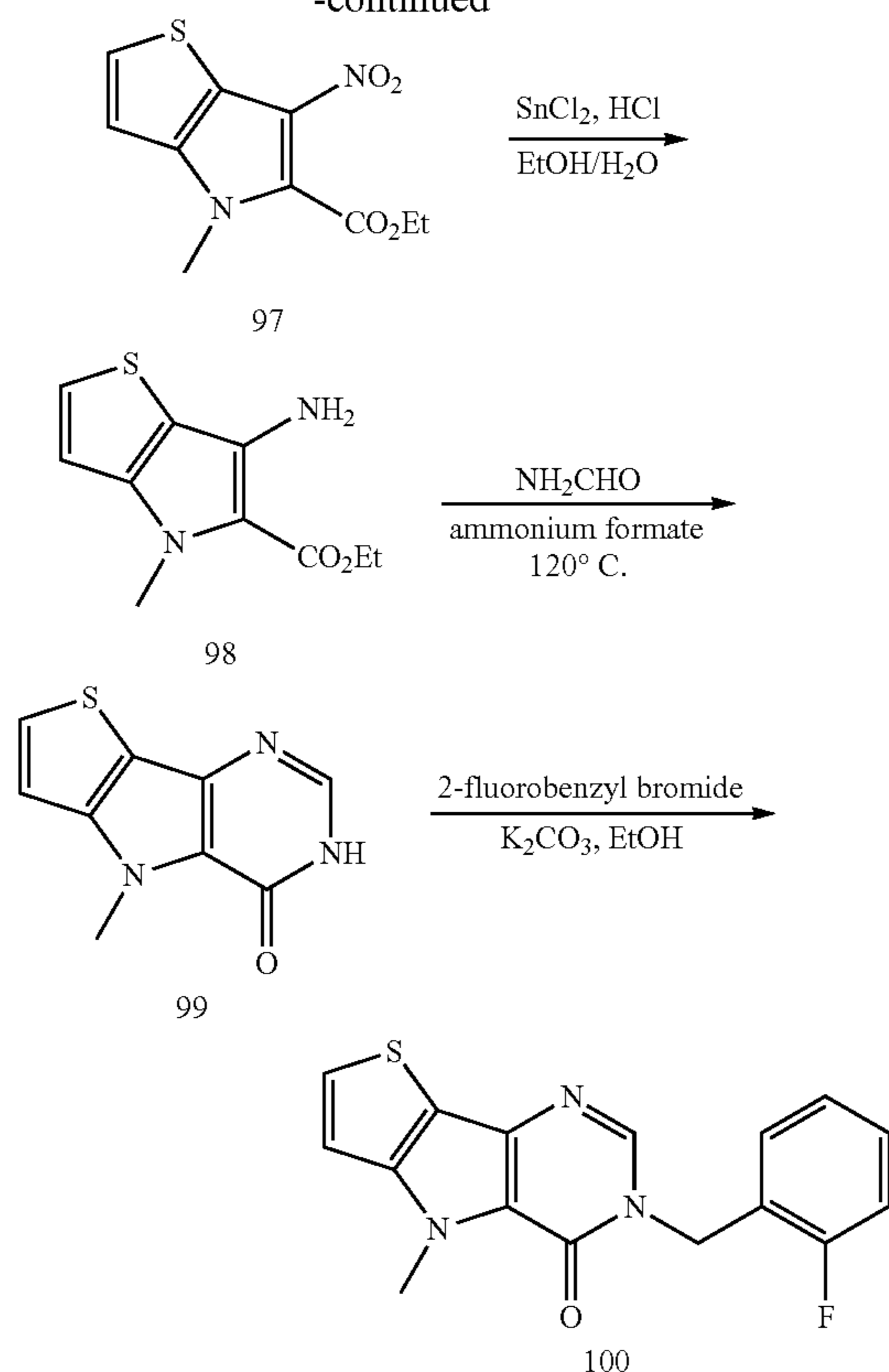
Ethyl-6-amino-4-methyl-4H-thieno[3,2-b]pyrrole-5-carboxylate (98)
