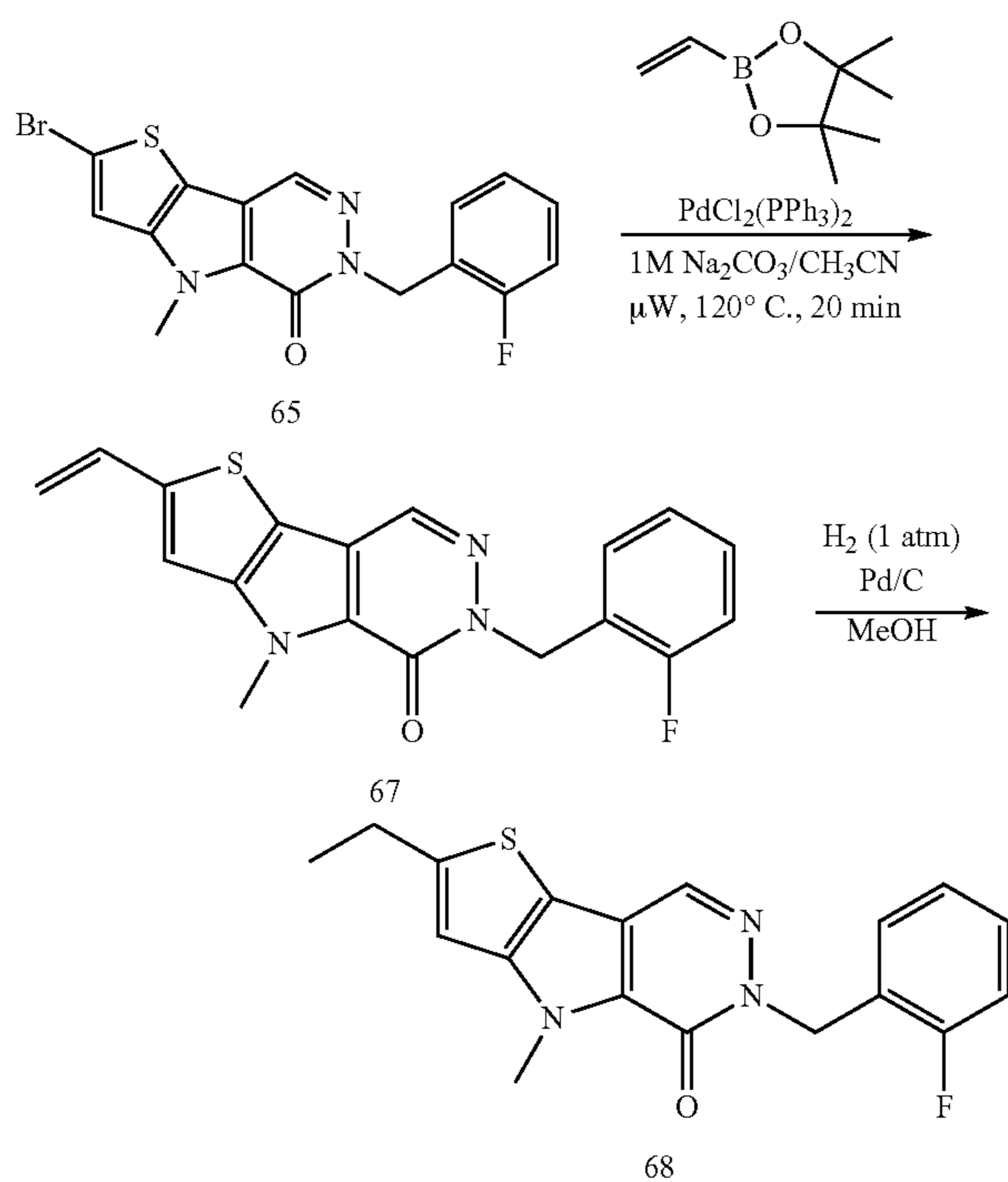
2-Vinyl-4-methyl-6-[(2-fluorophenyl)methyl]-4H-thieno[3,2-b]pyrrole[3,2-d]pyridazinone (67)
