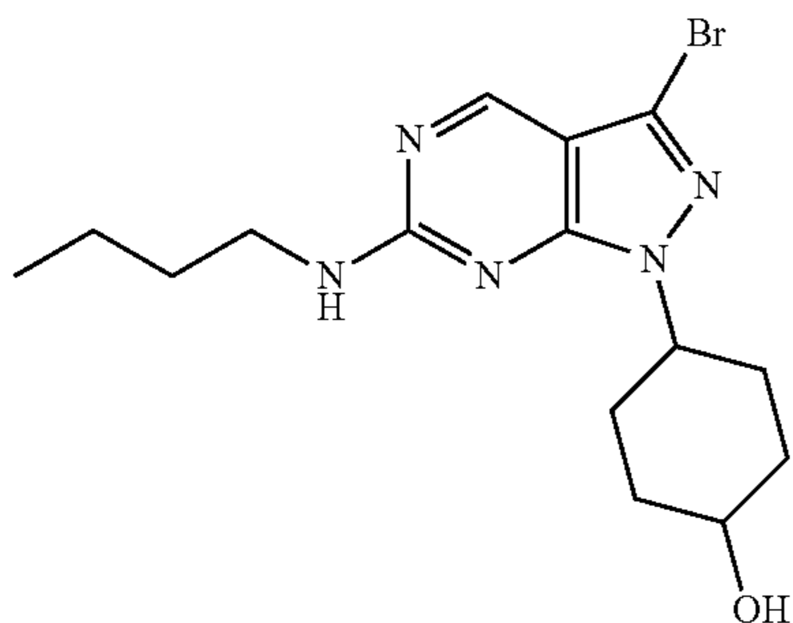
1-(4-hydroxy-cyclohexyl)-3-bromo-N-butyl-1H-pyrazolo[3,4-d]pyrimidin-6-amine
