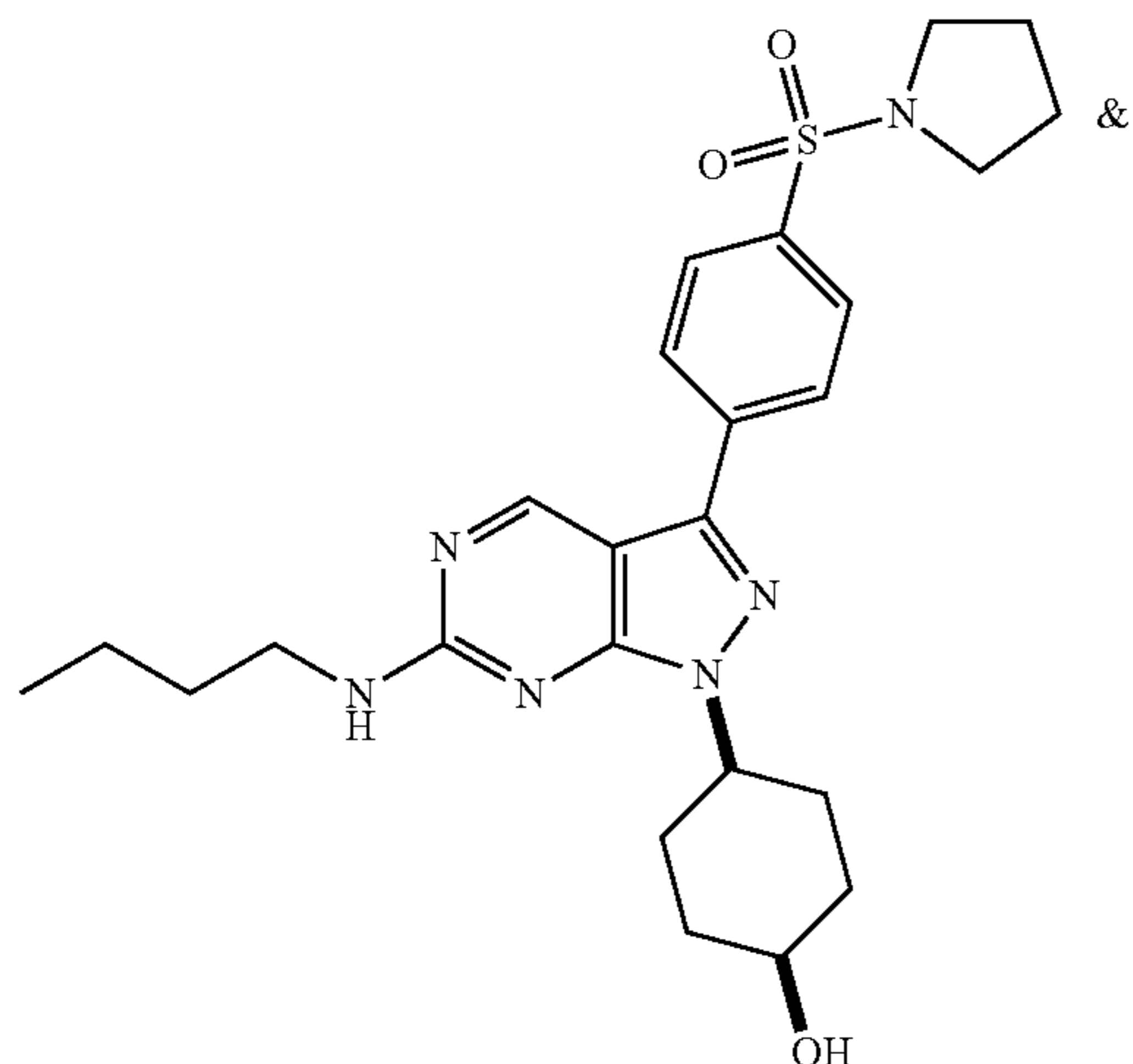
1-(4-hydroxy-cyclohexyl)-3-(4-piperidinsulfonyl-phenyl)-1H-pyrazolo[3,4-d]pyrimidin-6-amine
