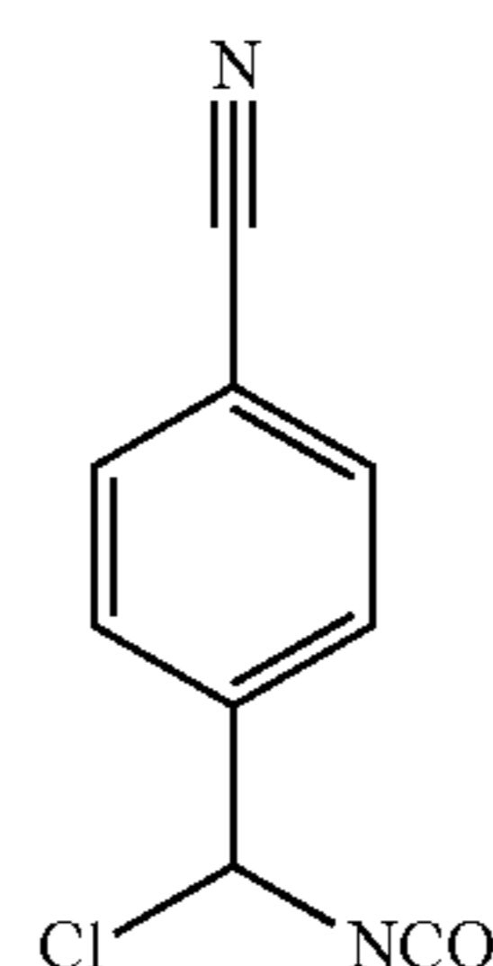
4-(Chloro(isocyanato)methyl)benzonitrile
