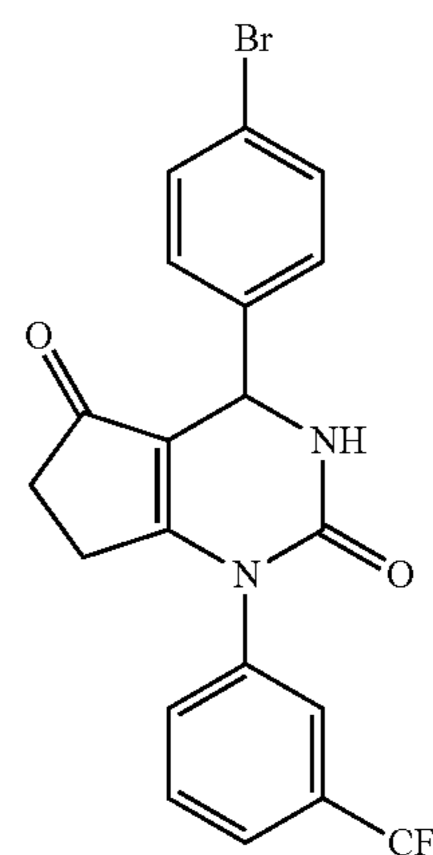
4-(4-Bromophenyl)-1-(3-(trifluoromethyl)phenyl)-3,4,6,7-tetrahydro-1H-cyclopenta[d]pyrimidine-2,5-dione
