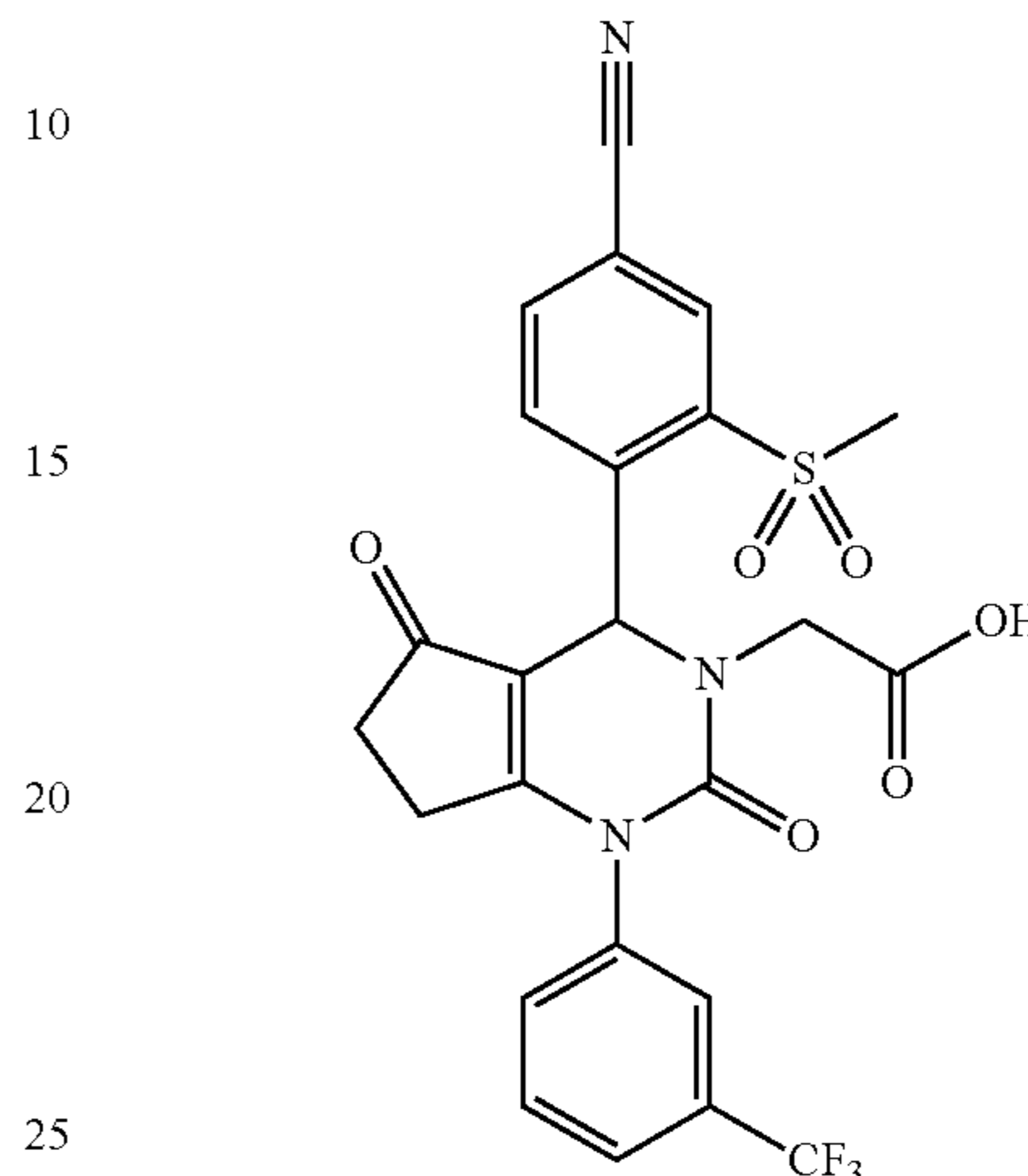
2-(4-(4-Cyano-2-(methylsulfonyl)phenyl)-2,5-dioxo-1-(3-(trifluoromethyl)phenyl)-6,7-dihydro-1H-cyclopenta[d]pyrimidin-3(2H,4H,5H)-yl)acetic acid
