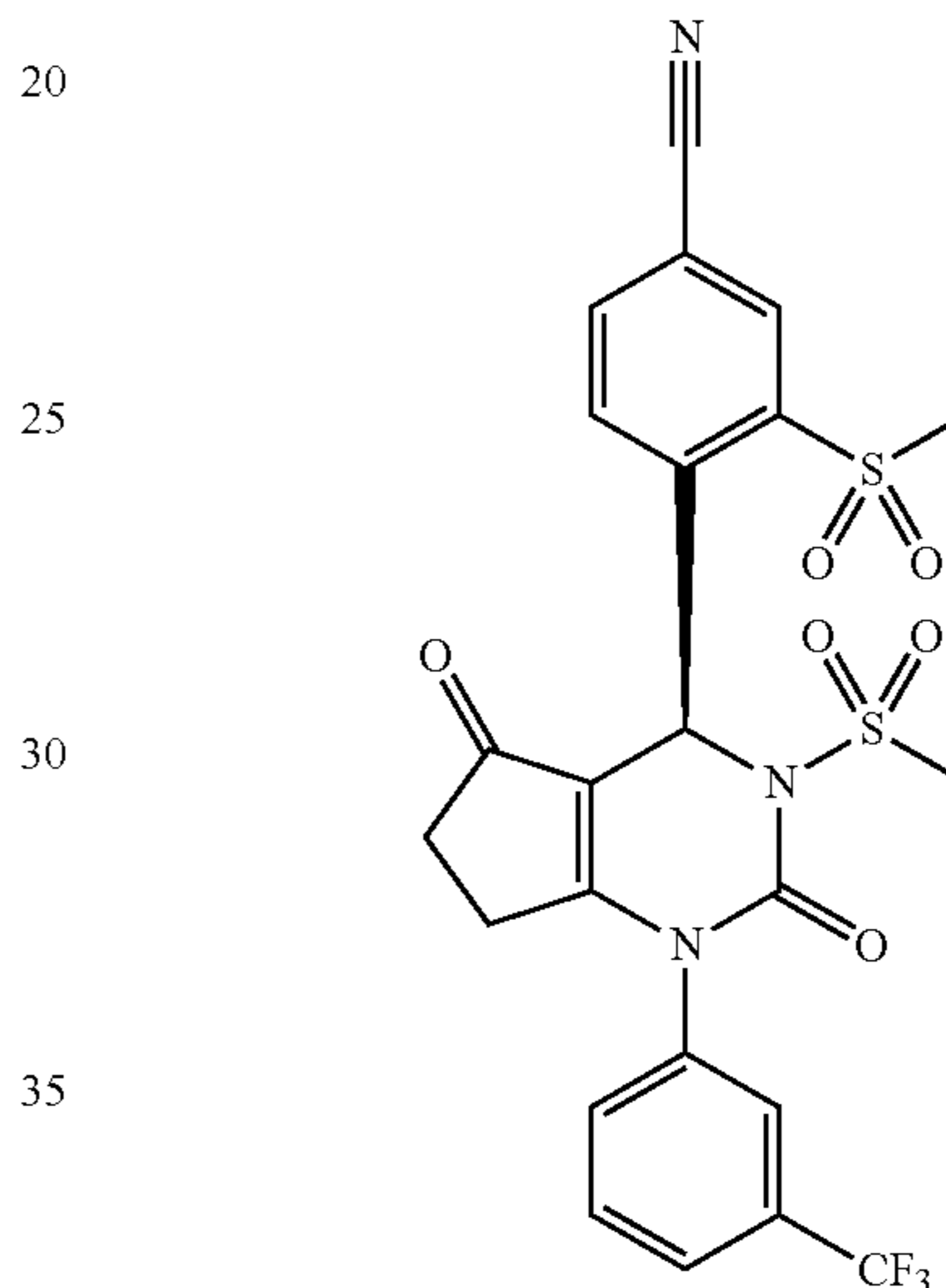
4-(3-(Ethylsulfonyl)-2,5-dioxo-1-(3-(trifluoromethyl)phenyl)-2,3,4,5,6,7-hexahydro-1H-cyclopenta[d]pyrimidin-4-yl)benzotrile
