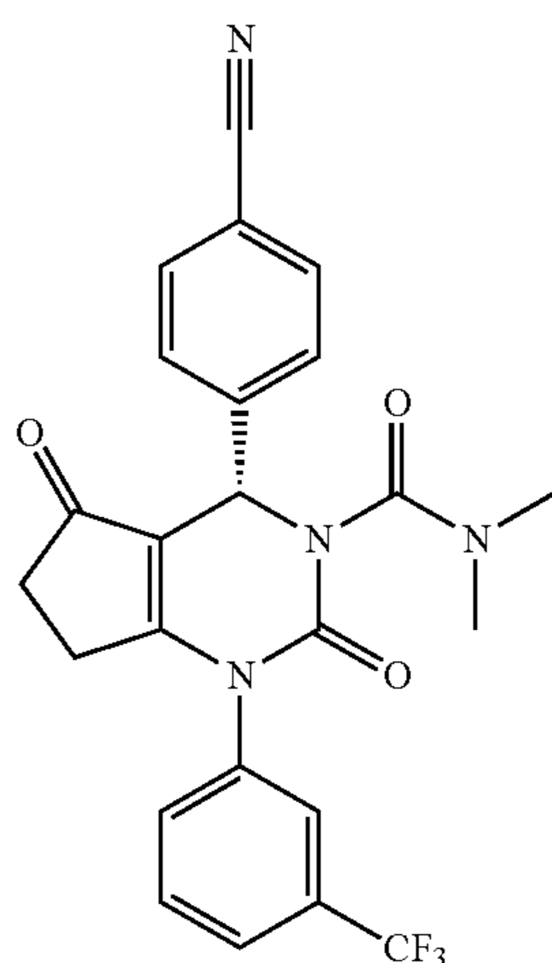
(S)-4-(4-Cyanophenyl)-N-methyl-2,5-dioxo-1-(3-(trifluoromethyl)phenyl)-4,5,6,7-tetrahydro-1H-cyclopenta[d]pyrimidine-3(2H)-carboxamide
