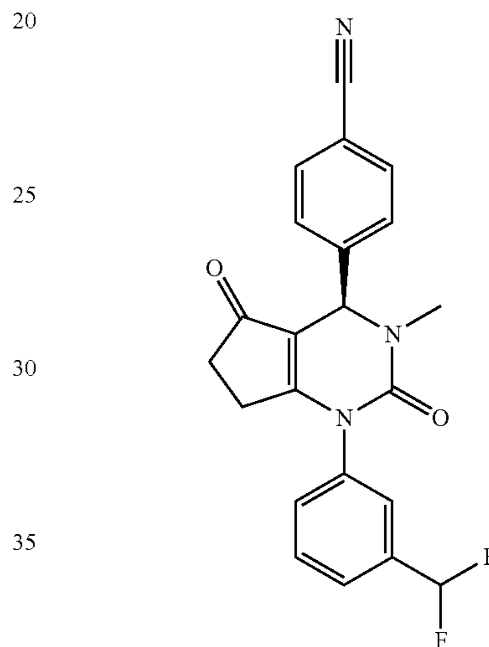
(R)-4-(1-(3-(Difluoromethyl)phenyl)-3-methyl-2,5-dioxo-2,3,4,5,6,7-hexahydro-1H-cyclopenta[d]pyrimidin-4-yl)benzonitrile
