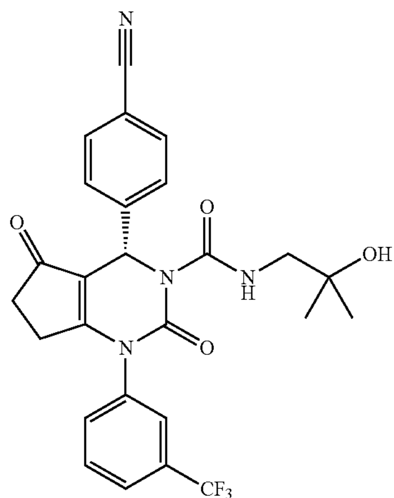
(S)-4-(4-Cyanophenyl)-N-(2-hydroxy-2-methylpropyl)-2,5-dioxo-1-(3-(trifluoromethyl)phenyl)-4,5,6,7-tetrahydro-1H-cyclopenta[d]pyrimidine-3(2H)-carboxamide
