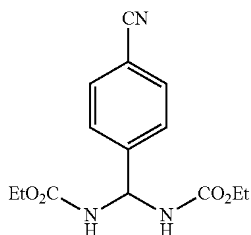
Diethyl (4-Cyanophenyl)methylenedicarbamate
