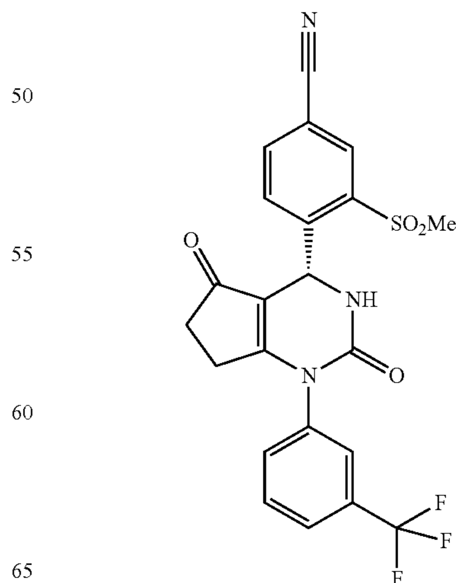
4-(2,5-Dioxo-1-(3-(trifluoromethyl)phenyl)-2,3,4,5,6,7-hexahydro-1H-cyclopenta[d]pyrimidin-4-yl)-3-(methylsulfonyl)benzonitrile
