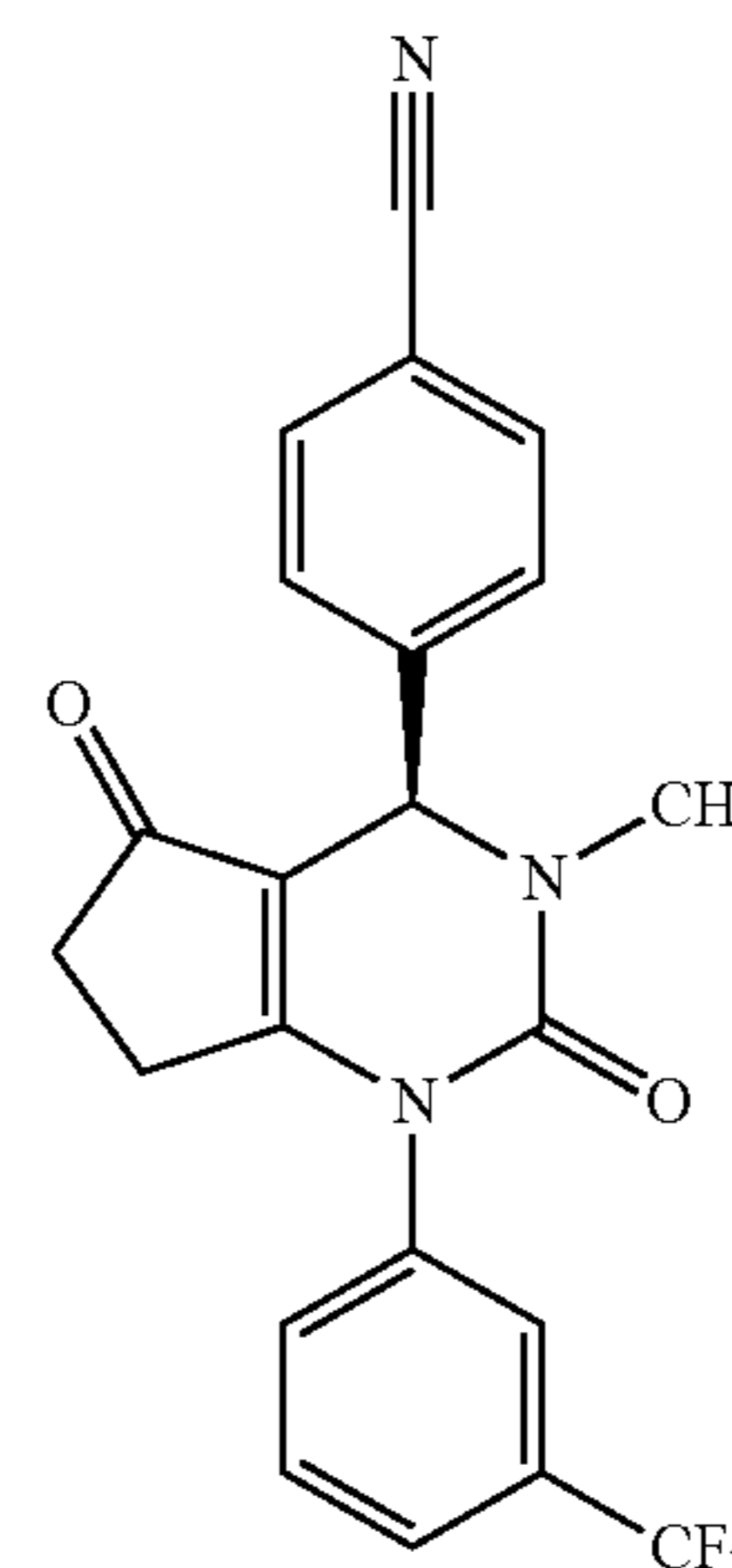
(R)-4-(3-Methyl-2,5-dioxo-1-(3-(trifluoromethyl)phenyl)-2,3,4,5,6,7-hexahydro-1H-cyclopenta[d]pyrimidin-4-yl)benzotrile
