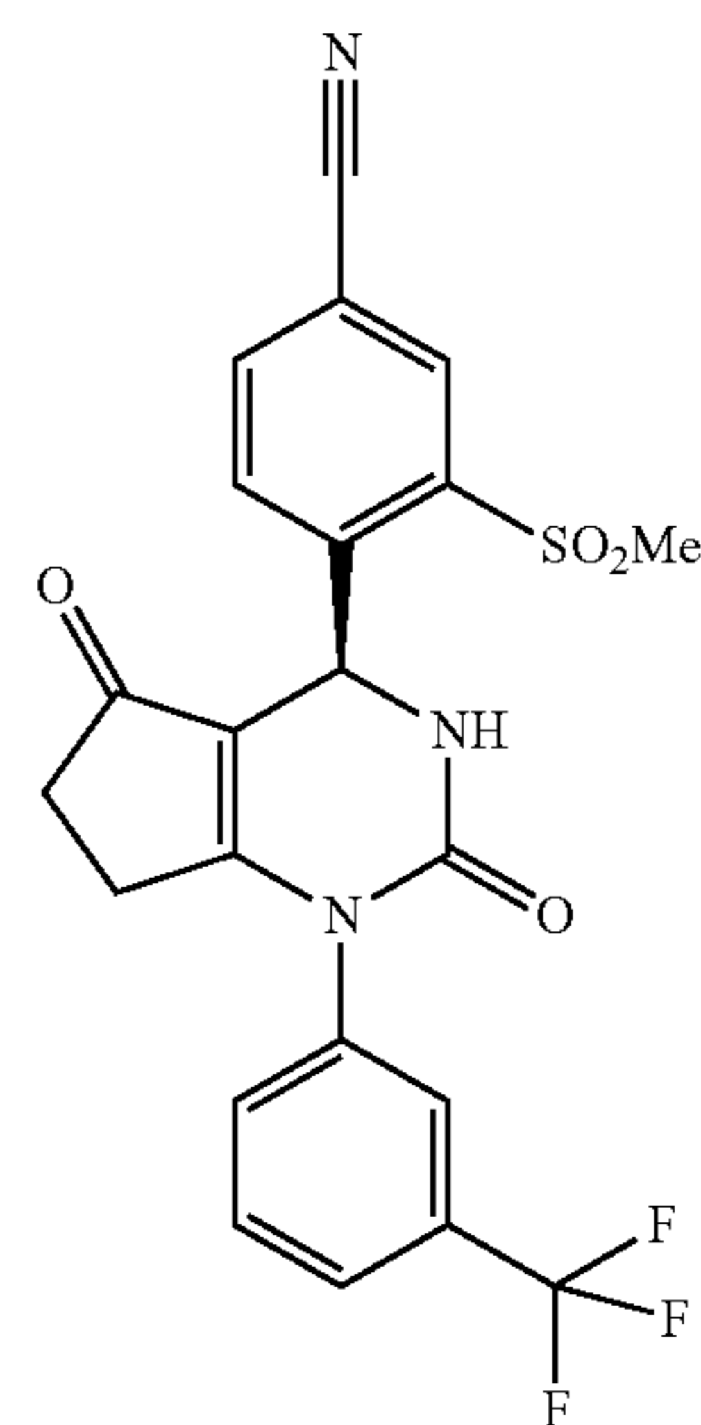
(S)-4-(2,5-Dioxo-1-(3-(trifluoromethyl)phenyl)-2,3,4,5,6,7-hexahydro-1H-cyclopenta[d]pyrimidin-4-yl)-3-(methylsulfonyl)benzotrile
