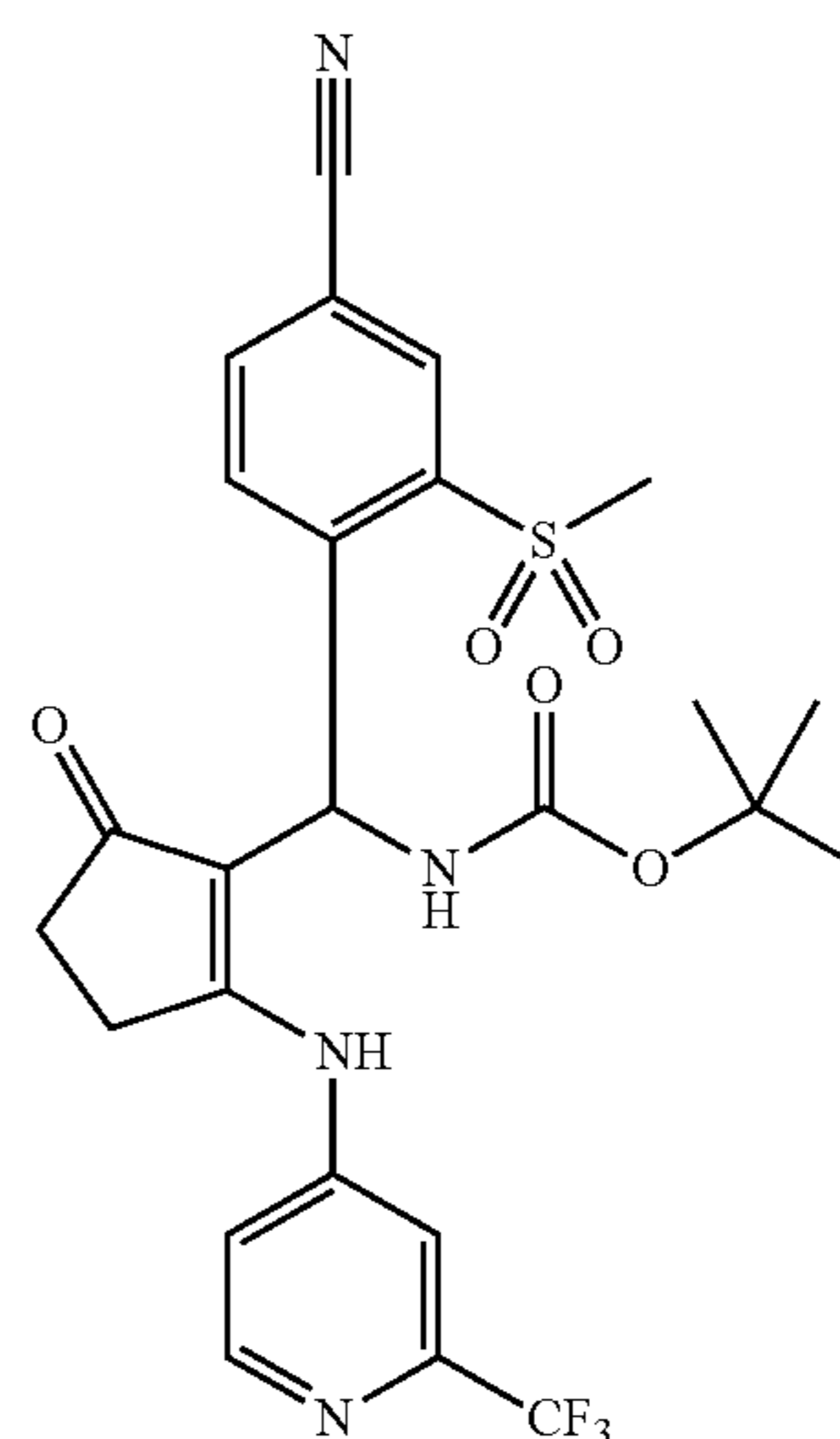
tert-Butyl (4-Cyano-2-(methylsulfonyl)phenyl)(5-oxo-2-(2-(trifluoromethyl)pyridin-4-ylamino)cyclopent-1-enyl)methylcarbamate
