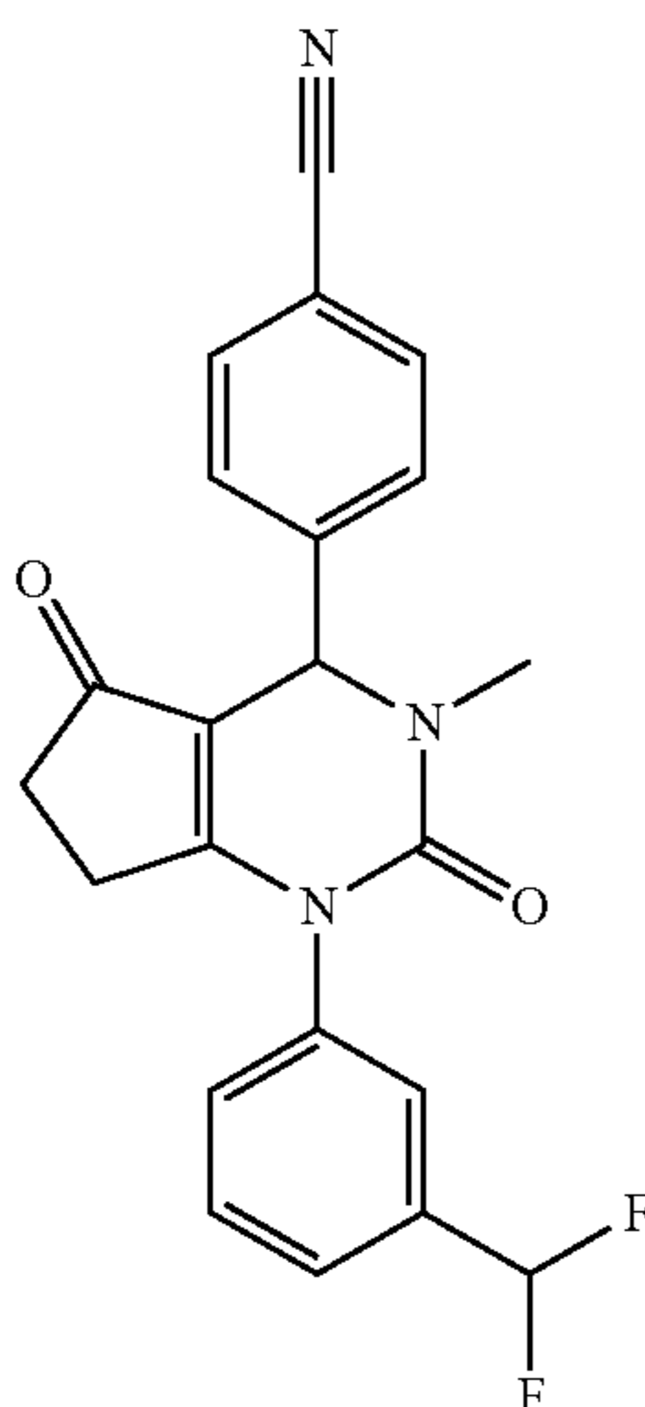
4-(1-(3-(Difluoromethyl)phenyl)-3-methyl-2,5-dioxo-2,3,4,5,6,7-hexahydro-1H-cyclopenta[d]pyrimidin-4-yl)benzonitrile
