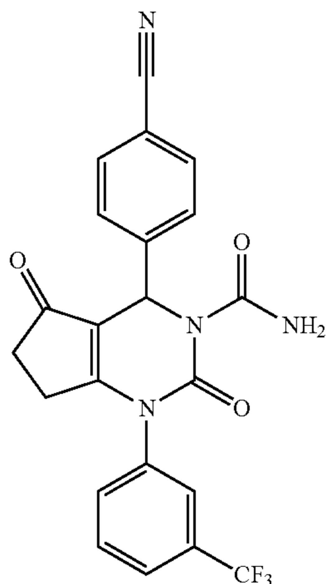
4-(4-Cyanophenyl)-2,5-dioxo-1-(3-(trifluoromethyl)phenyl)-4,5,6,7-tetrahydro-1H-cyclopenta[d]pyrimidine-3(2H)-carboxamide
