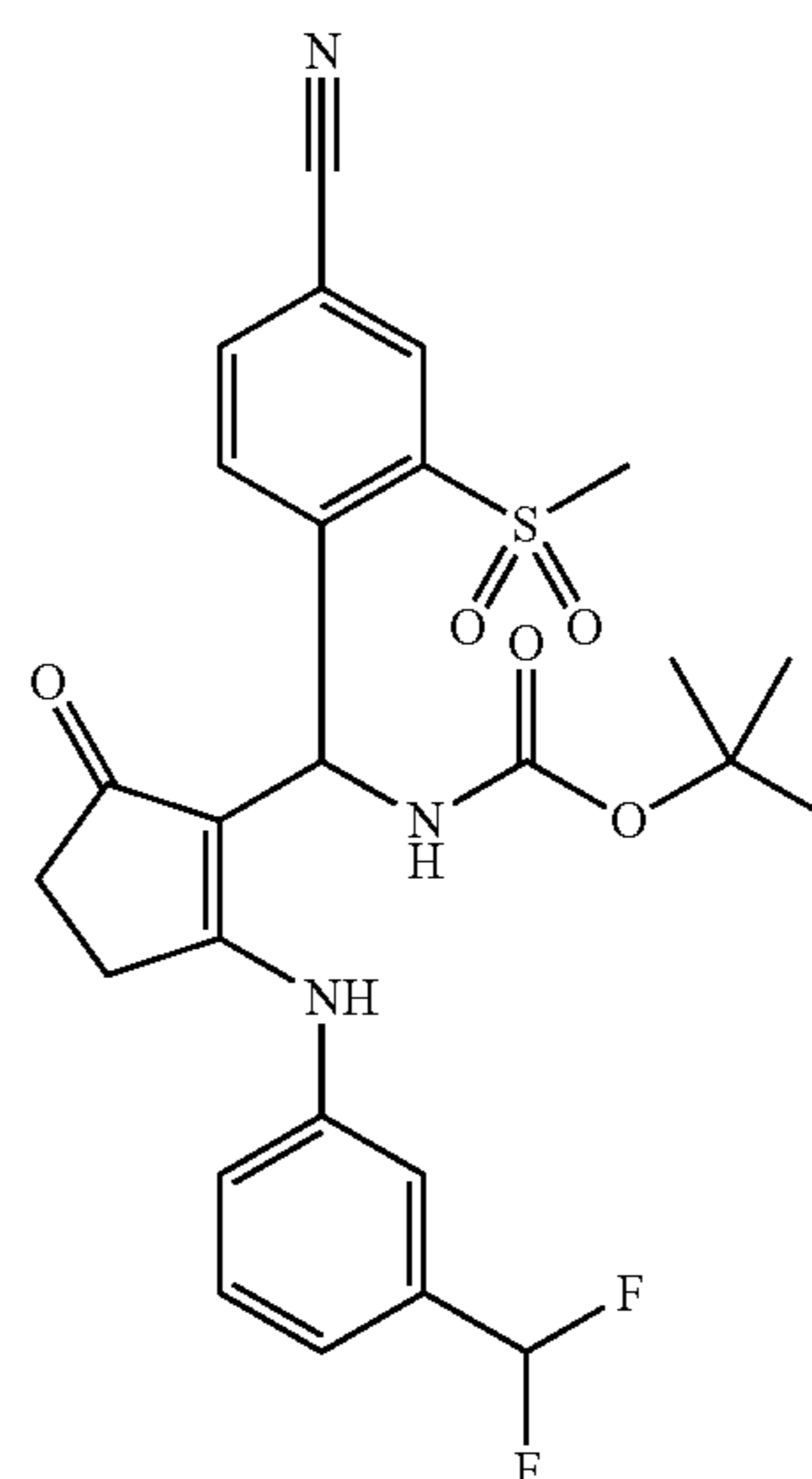
tert-Butyl (4-Cyano-2-(methylsulfonyl)phenyl)(2-(3-(difluoromethyl)phenylamino)cyclopent-1-en-5-yl)methylcarbamate
