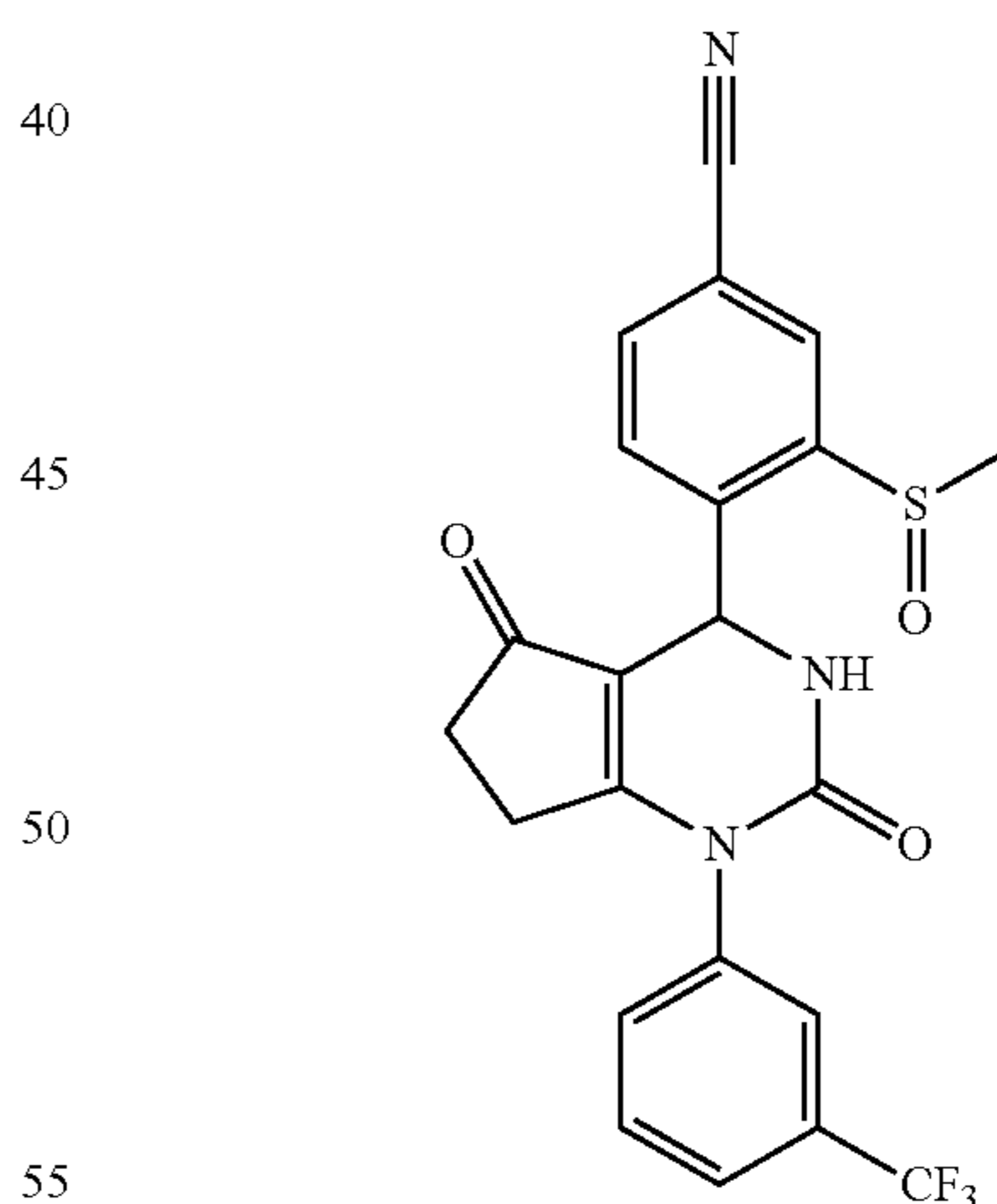
4-(2,5-Dioxo-1-(3-(trifluoromethyl)phenyl)-2,3,4,5,6,7-hexahydro-1H-cyclopenta[d]pyrimidin-4-yl)-3-(methylsulfonyl)benzonitrile
