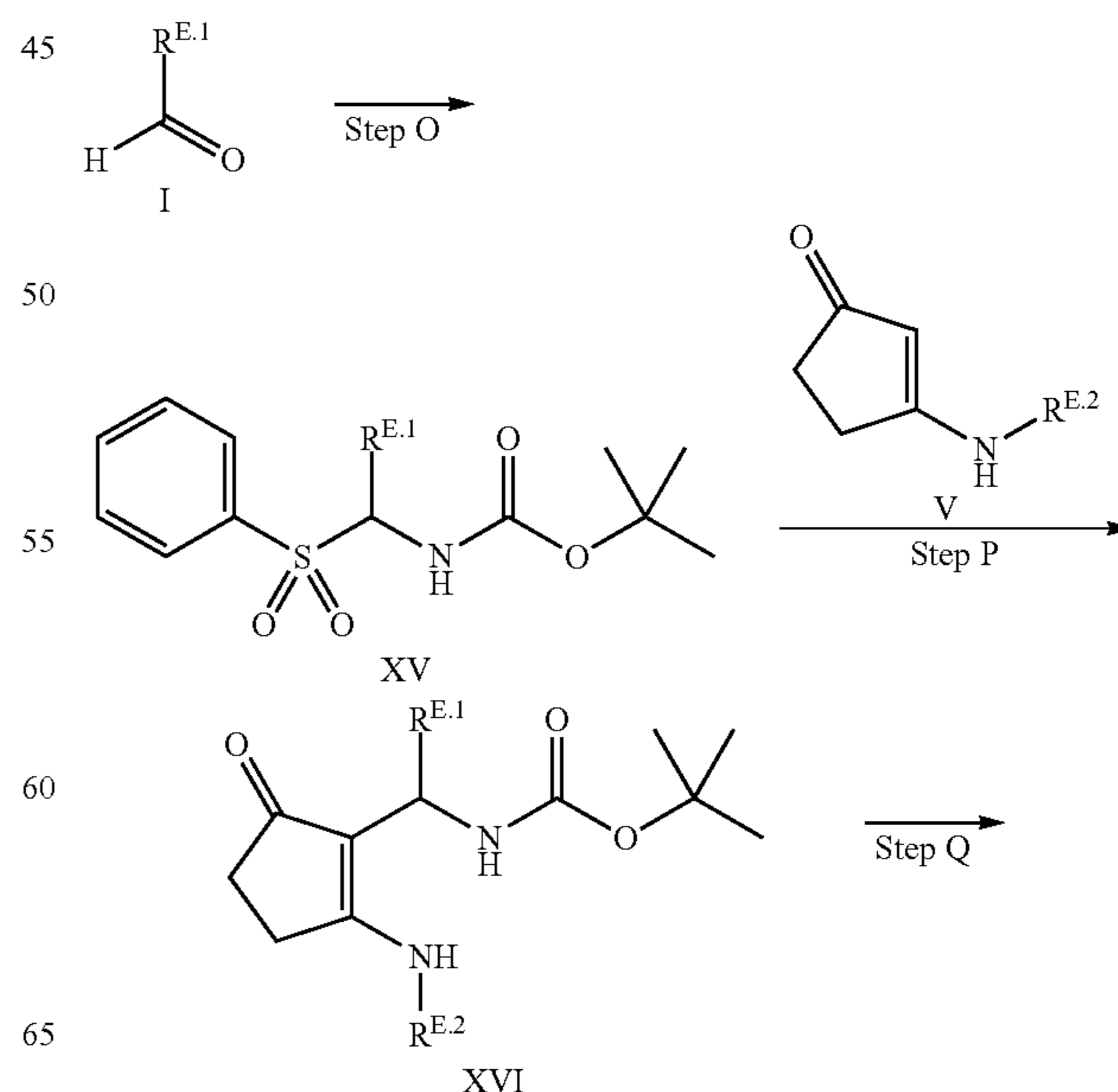
SCHEME 4
