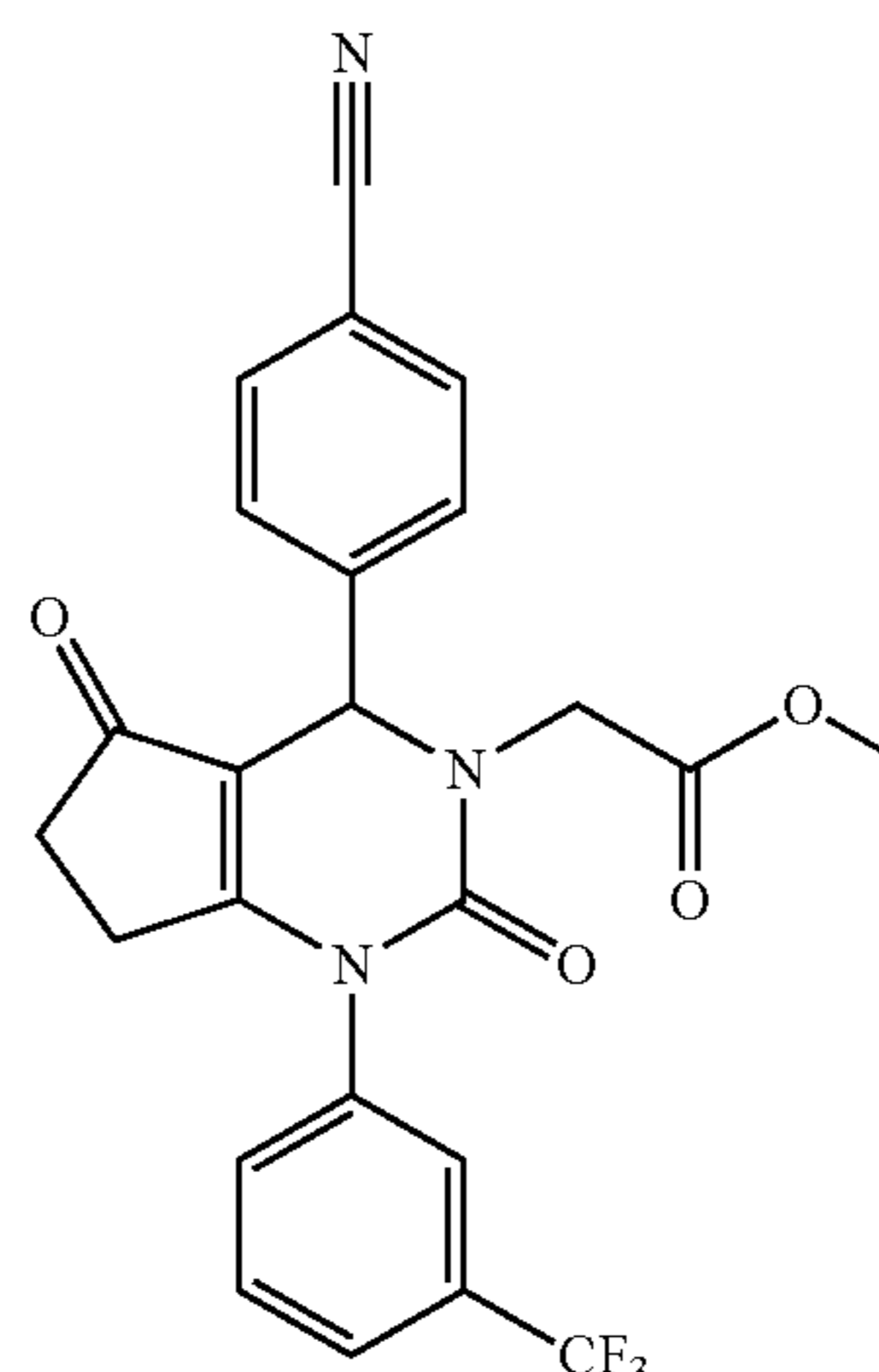
Methyl 2-(4-(4-Cyanophenyl)-2,5-dioxo-1-(3-(trifluoromethyl)phenyl)-6,7-dihydro-1H-cyclopenta[d]pyrimidin-3(2H,4H,5H)-yl)acetate
