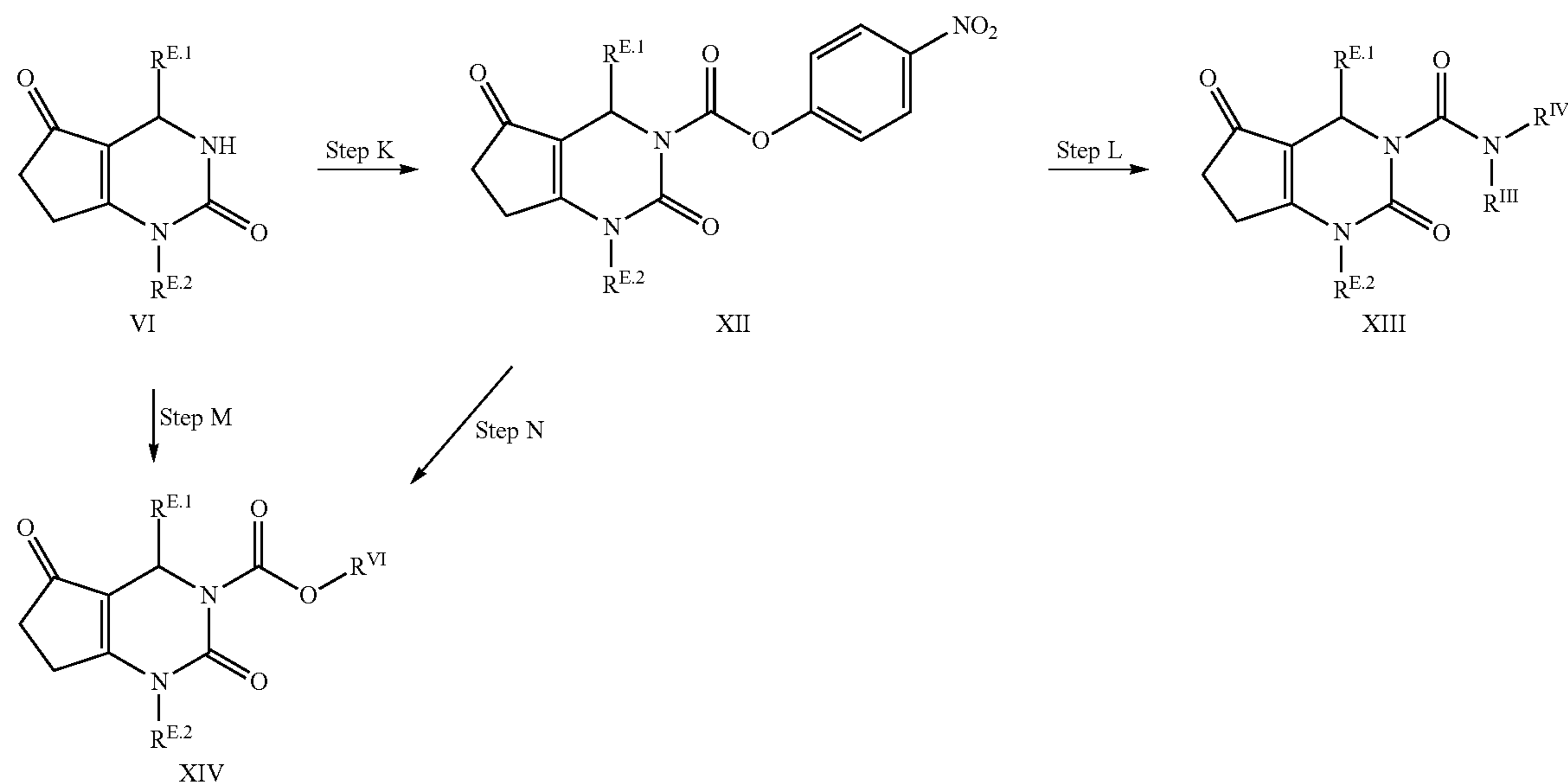
SCHEME 3
