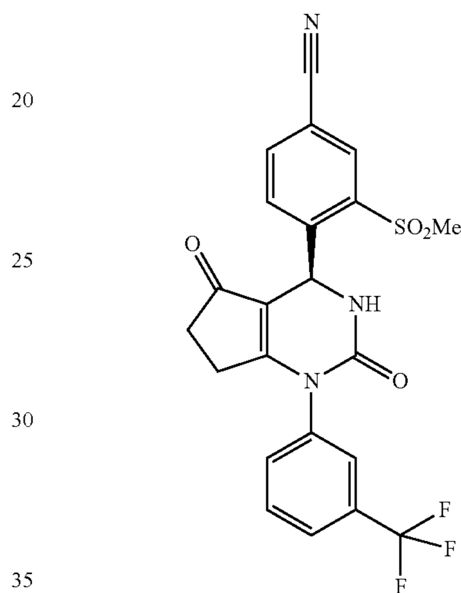
(S)-4-(2,5-Dioxo-1-(3-(trifluoromethyl)phenyl)-2,3,4,5,6,7-hexahydro-1H-cyclopenta[d]pyrimidin-4-yl)-3-(methylsulfonyl)benzonitrile
