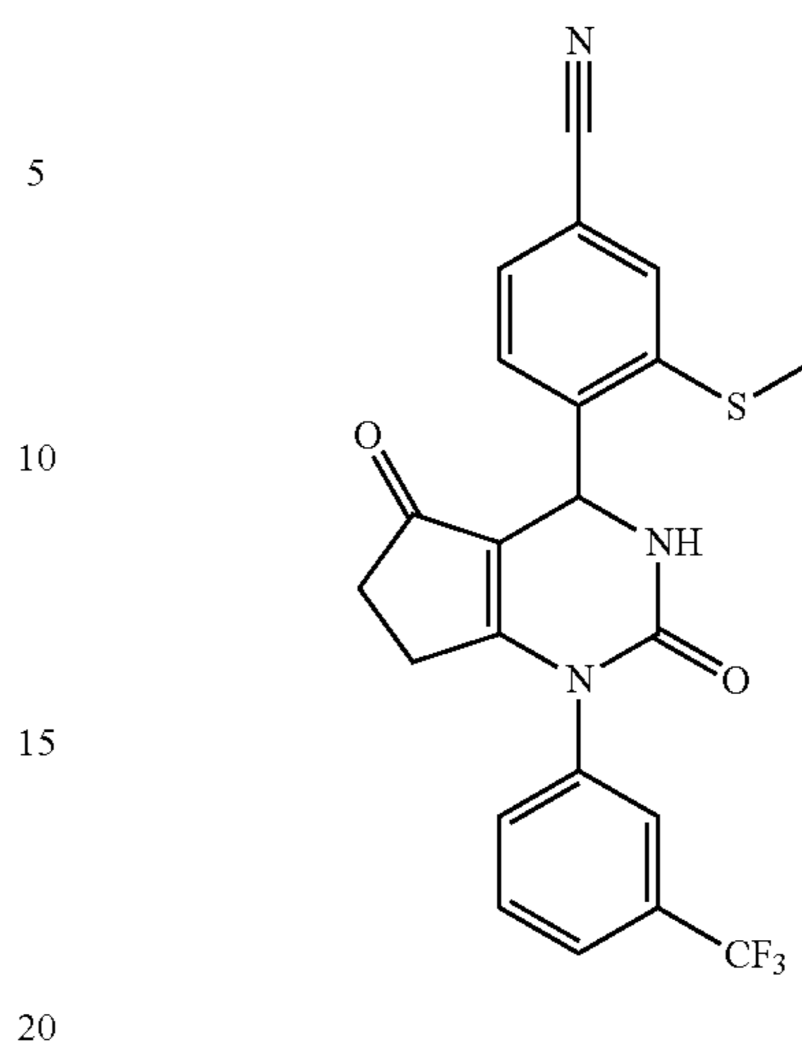
4-(2,5-Dioxo-1-(3-(trifluoromethyl)phenyl)-2,3,4,5,6,7-hexahydro-1H-cyclopenta[d]pyrimidin-4-yl)-3-(methylthio)benzonitrile
