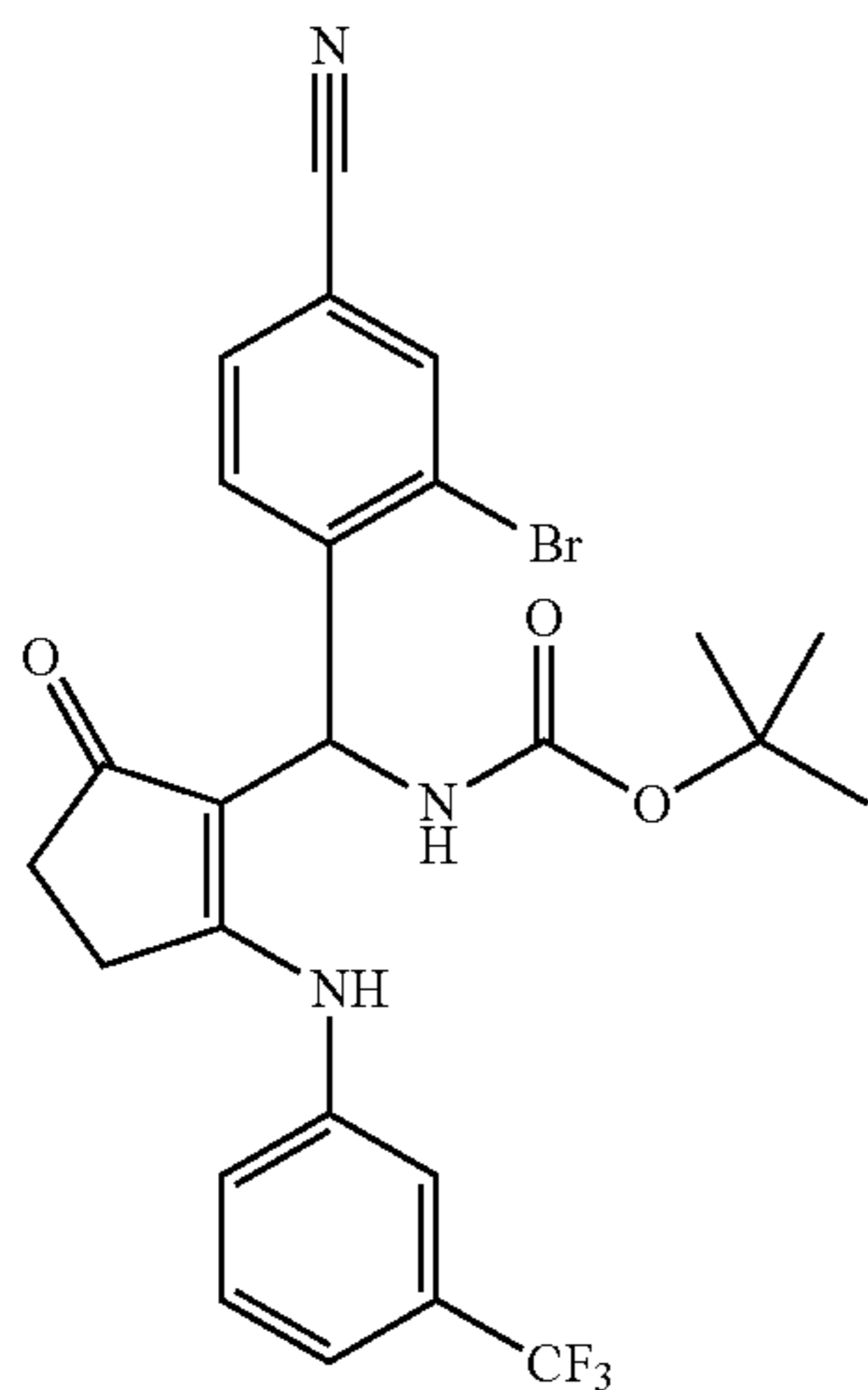
tert-Butyl (2-Bromo-4-cyanophenyl)(5-oxo-2-(3-(trifluoromethyl)phenylamino)cyclopent-1-enyl)methylcarbamate
