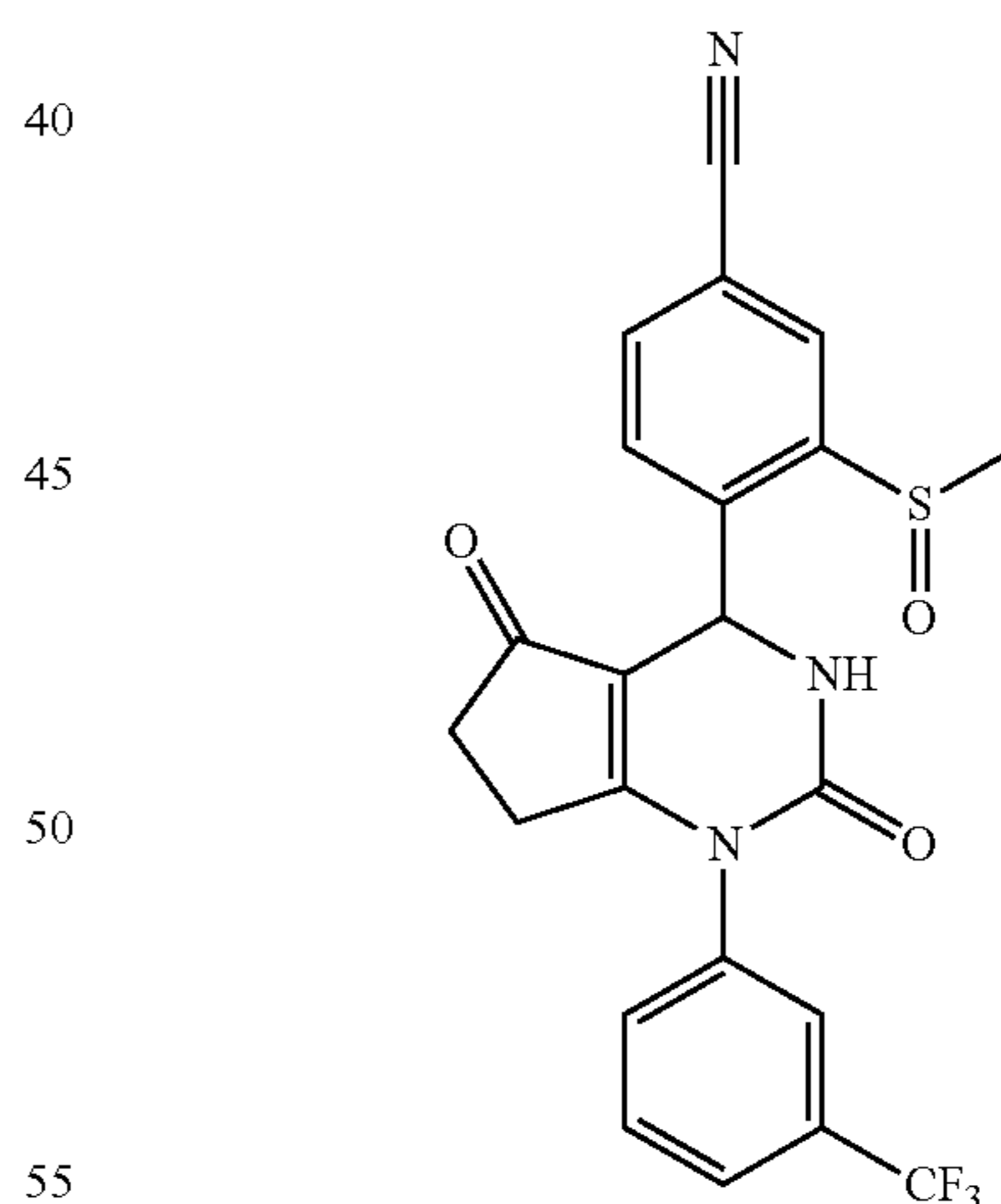
4-(2,5-Dioxo-1-(3-(trifluoromethyl)phenyl)-2,3,4,5,6,7-hexahydro-1H-cyclopenta[d]pyrimidin-4-yl)-3-(methylsulfonyl)benzonitrile
