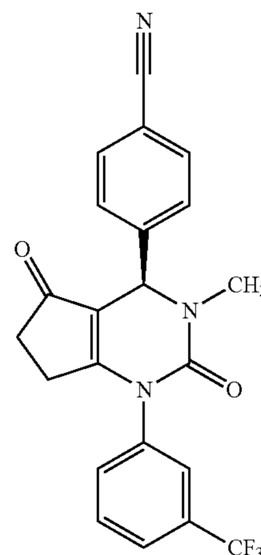
(R)-4-(3-Methyl-2,5-dioxo-1-(3-(trifluoromethyl)phenyl)-2,3,4,5,6,7-hexahydro-1H-cyclopenta[d]pyrimidin-4-yl)benzotrile
