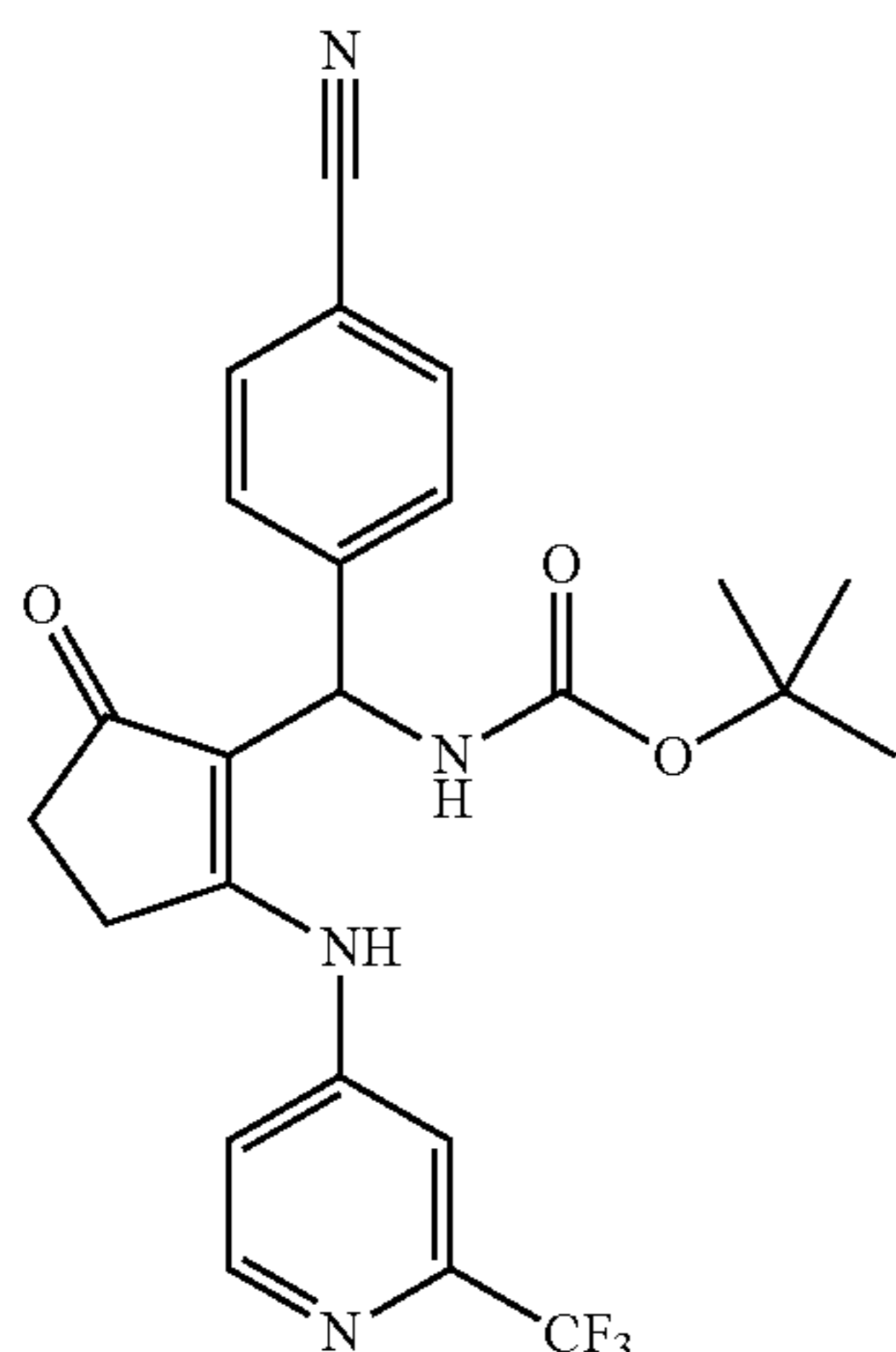
tert-Butyl(4-Cyanophenyl)(5-oxo-2-(2-(trifluoromethyl)pyridin-4-ylamino)cyclopent-1-enyl)methylcarbamate
