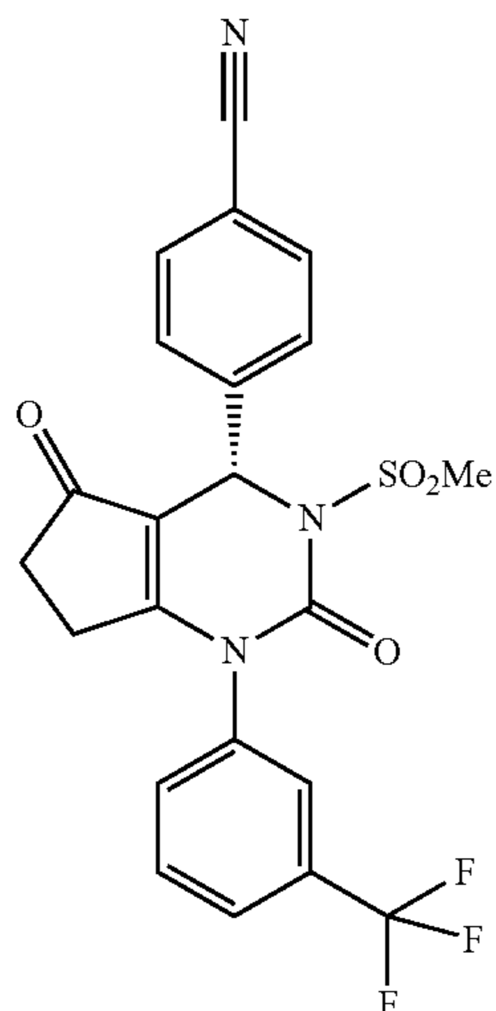
(S)-4-(3-(Methylsulfonyl)-2,5-dioxo-1-(3-(trifluoromethyl)phenyl)-2,3,4,5,6,7-hexahydro-1H-cyclopenta[d]pyrimidin-4-yl)benzonitrile
