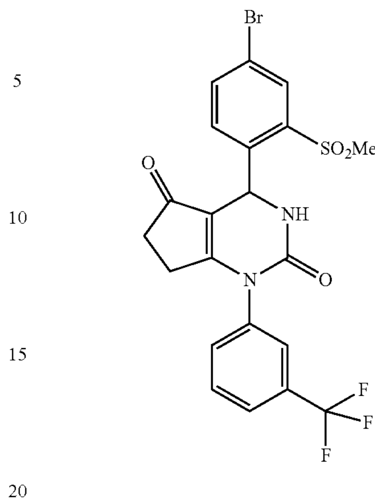
4-(4-Bromo-2-(methylsulfonyl)phenyl)-1-(3-(trifluoromethyl)phenyl)-3,4,6,7-tetrahydro-1H-cyclopenta[d]pyrimidine-2,5-dione
