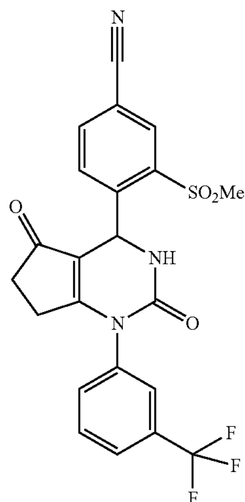
4-(2,5-Dioxo-1-(3-(trifluoromethyl)phenyl)-2,3,4,5,6,7-hexahydro-1H-cyclopenta[d]pyrimidin-4-yl)-3-(methylsulfonyl)benzotrile
