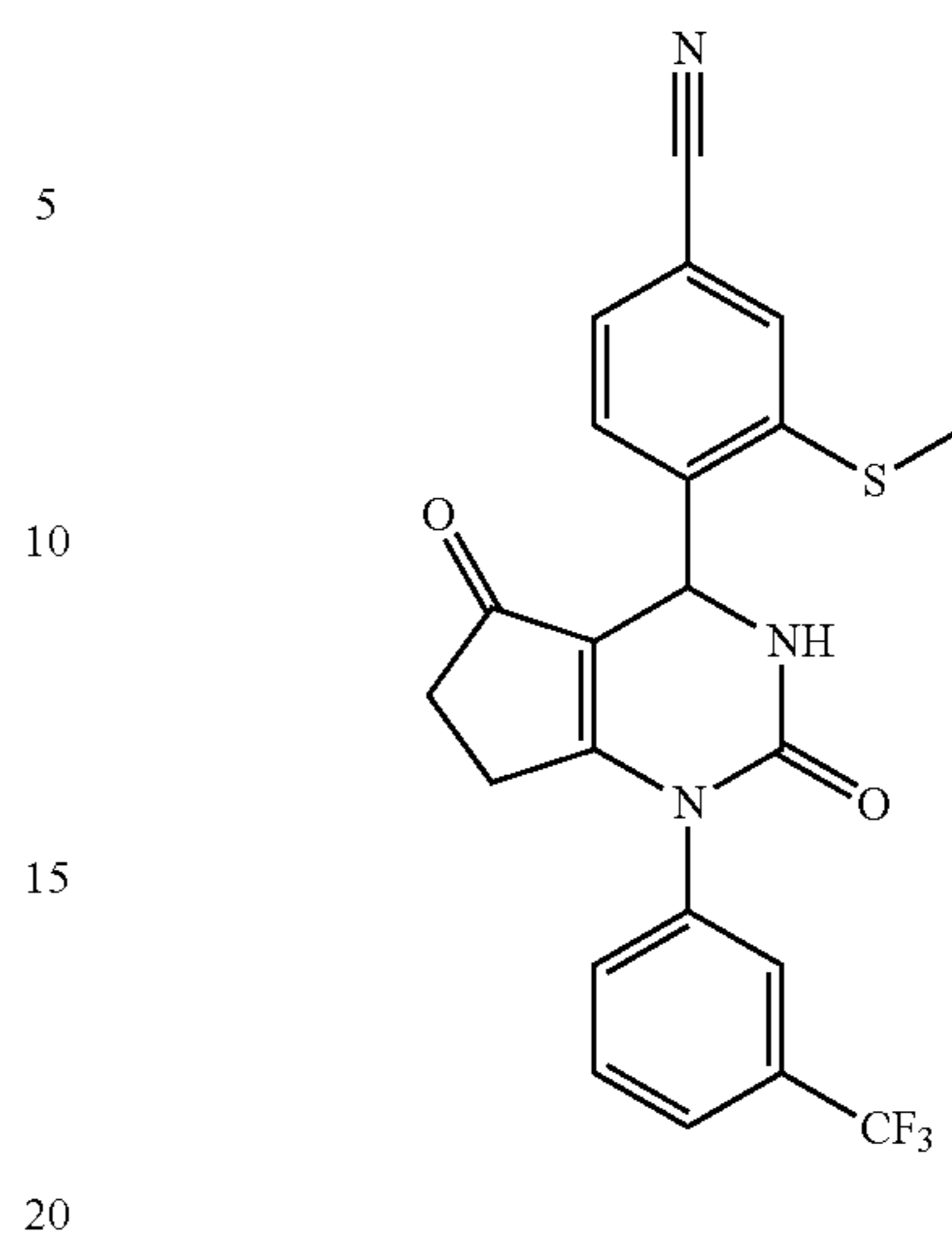
4-(2,5-Dioxo-1-(3-(trifluoromethyl)phenyl)-2,3,4,5,6,7-hexahydro-1H-cyclopenta[d]pyrimidin-4-yl)-3-(methylthio)benzonitrile
