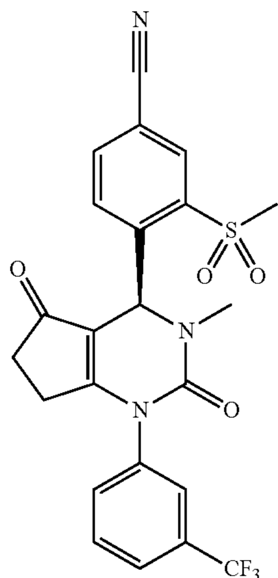
(S)-4-(3-Methyl-2,5-dioxo-1-(3-(trifluoromethyl)phenyl)-2,3,4,5,6,7-hexahydro-1H-cyclopenta[d]pyrimidin-4-yl)-3-(methylsulfonyl)benzonitrile
