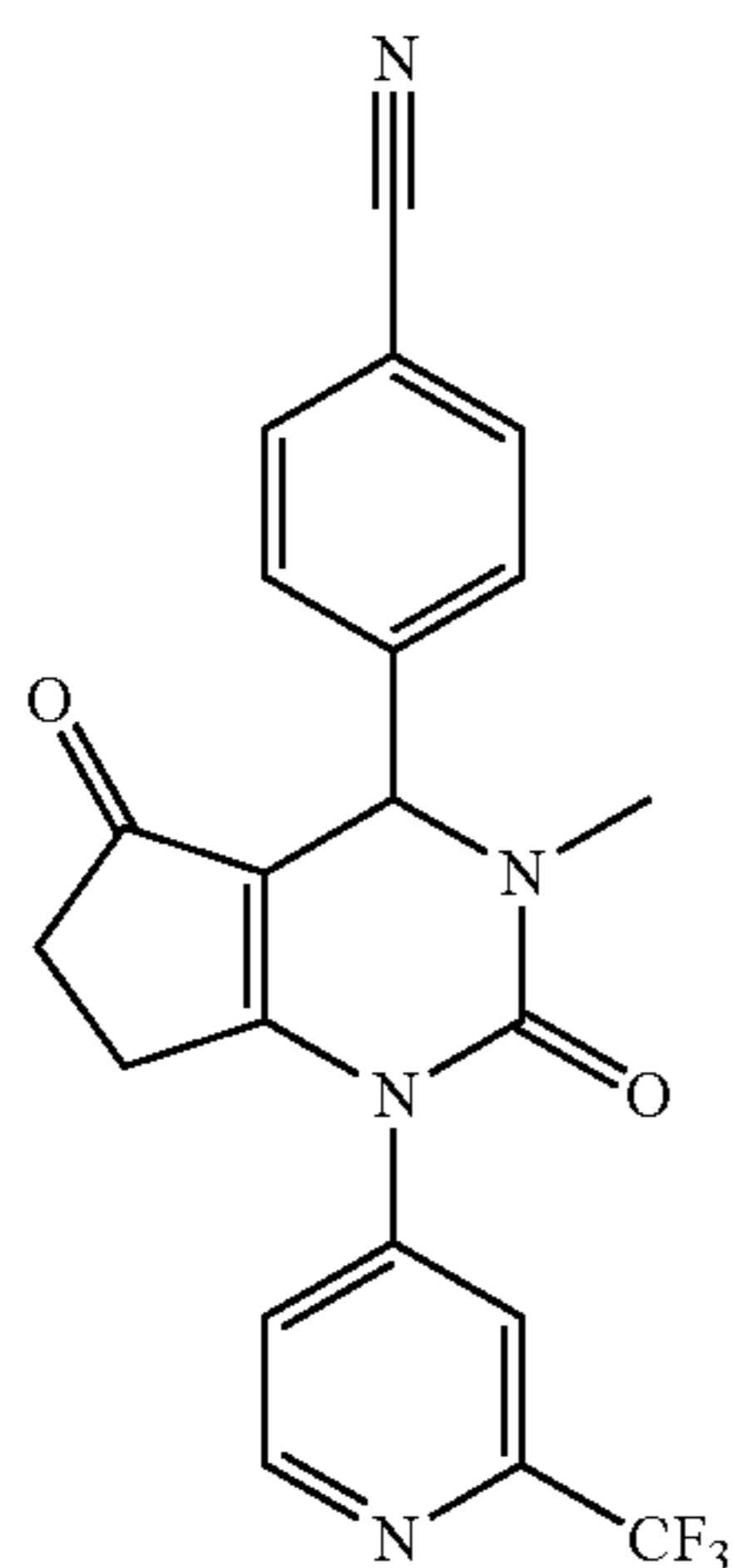
4-(3-Methyl-2,5-dioxo-1-(2-(trifluoromethyl)pyridin-4-yl)-2,3,4,5,6,7-hexahydro-1H-cyclopenta[d]pyrimidin-4-yl)benzonitrile
