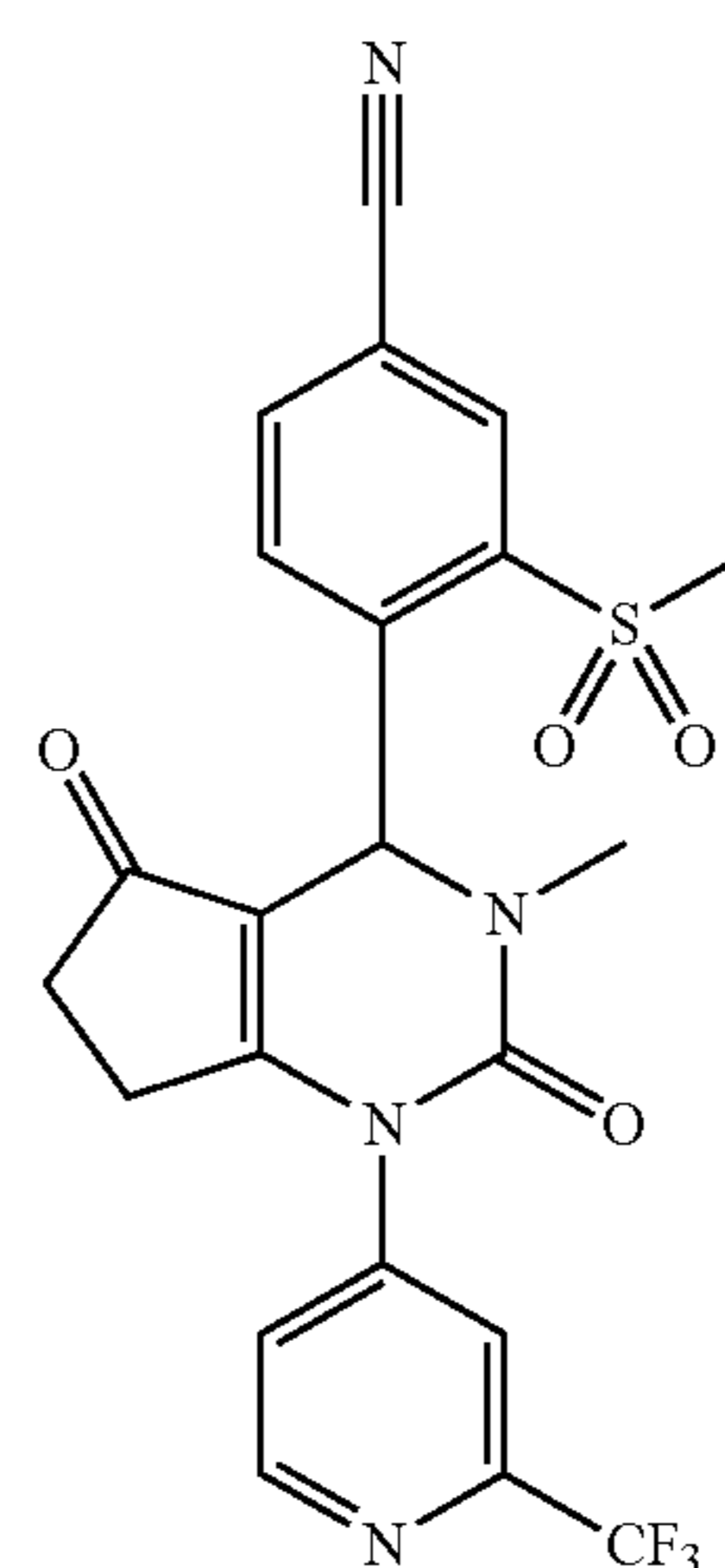
4-(3-Methyl-2,5-dioxo-1-(2-(trifluoromethyl)pyridin-4-yl)-2,3,4,5,6,7-hexahydro-1H-cyclopenta[d]pyrimidin-4-yl)-3-(methylsulfonyl)benzonitrile
