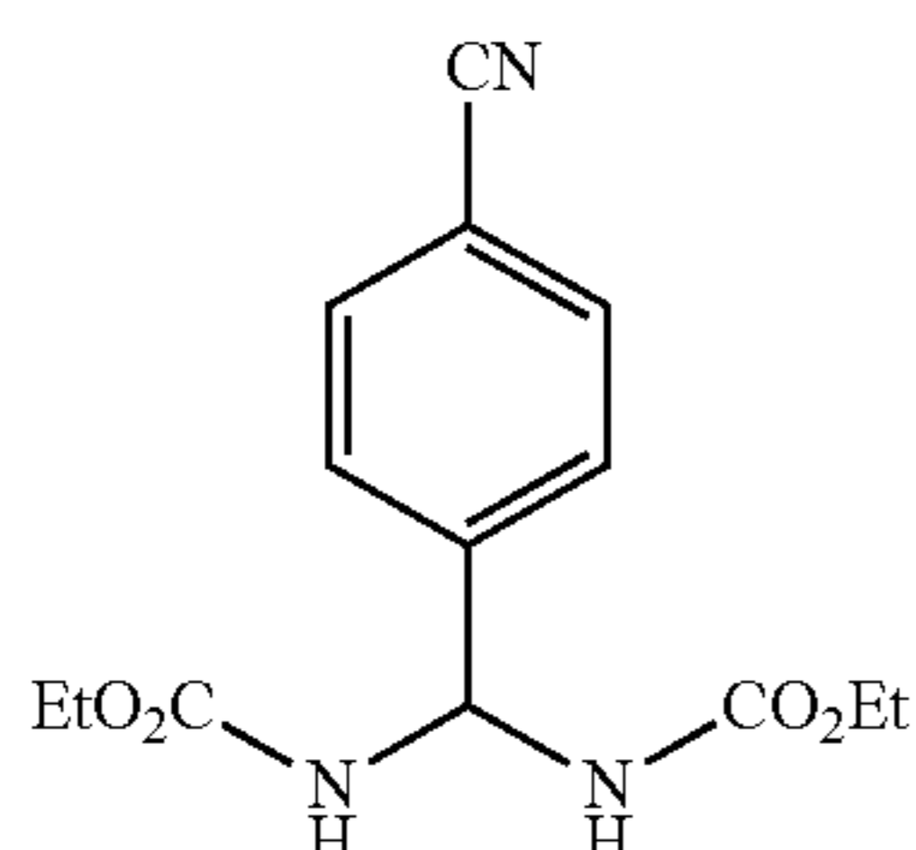
Diethyl (4-Cyanophenyl)methylenedicarbamate
