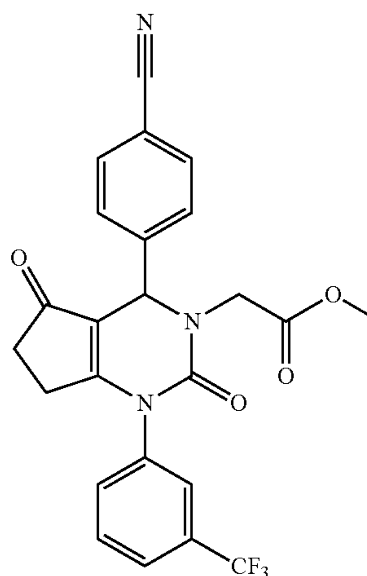
Methyl 2-(4-(4-Cyanophenyl)-2,5-dioxo-1-(3-(trifluoromethyl)phenyl)-6,7-dihydro-1H-cyclopenta[d]pyrimidin-3(2H,4H,5H)-yl)acetate
