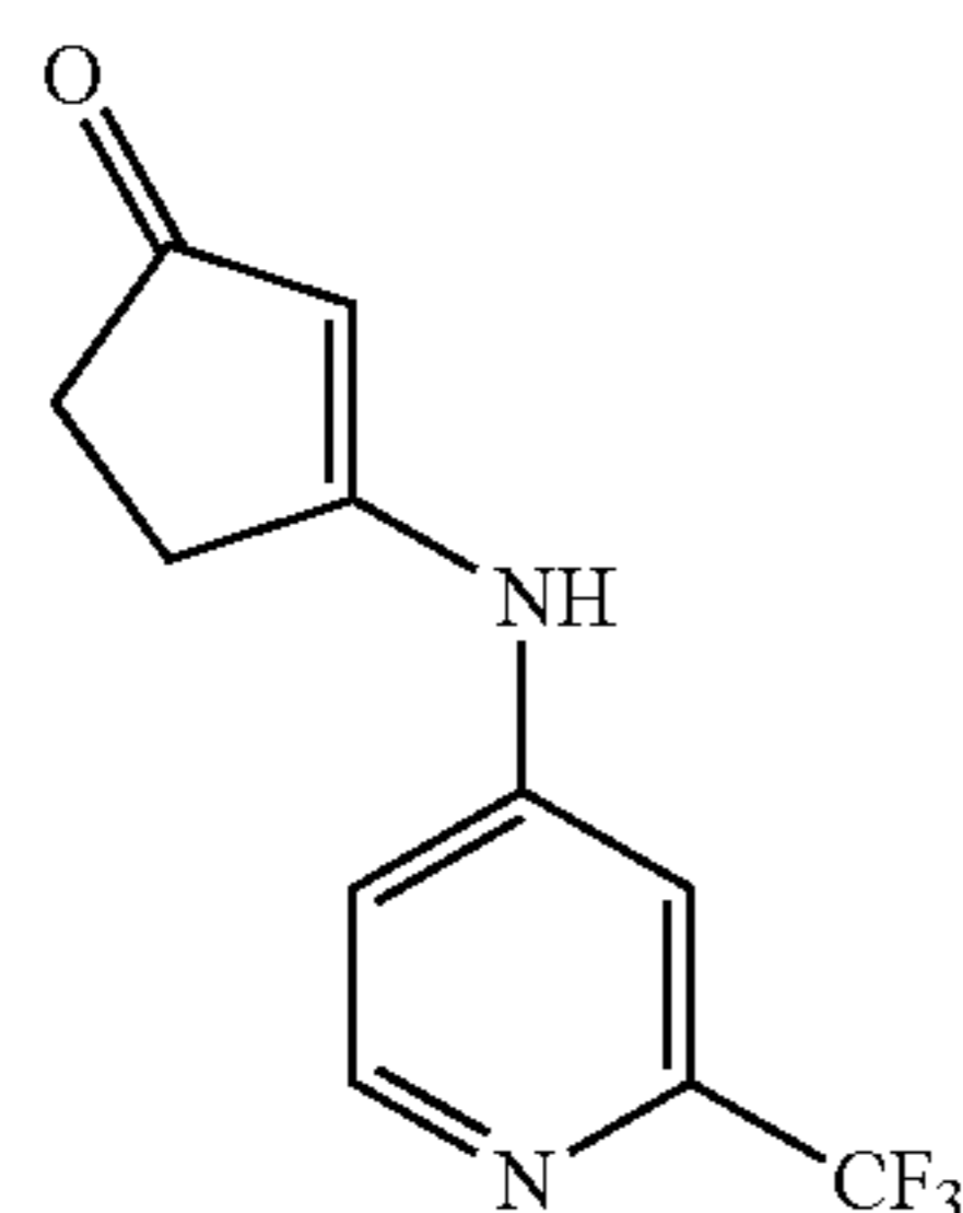
3-(2-(Trifluoromethyl)pyridin-4-ylamino)cyclopent-2-enone
