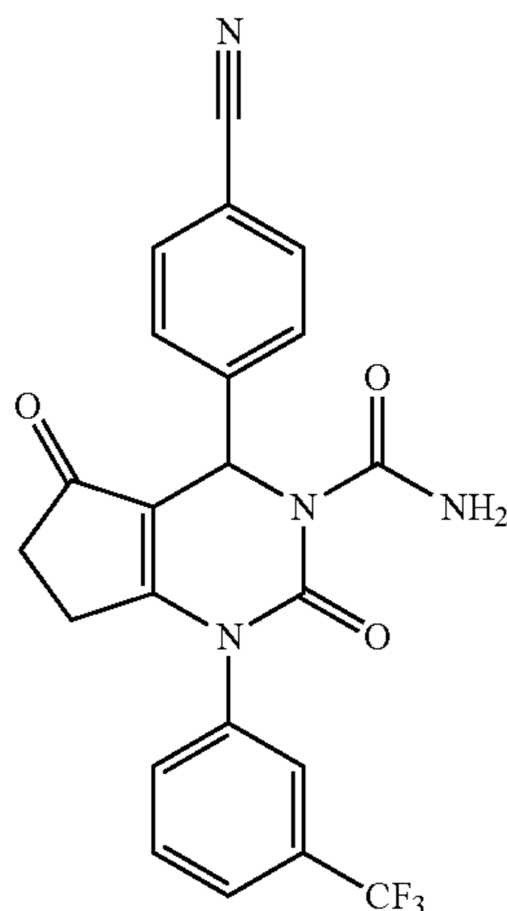
4-(4-Cyanophenyl)-2,5-dioxo-1-(3-(trifluoromethyl)phenyl)-4,5,6,7-tetrahydro-1H-cyclopenta[d]pyrimidine-3(2H)-carboxamide
