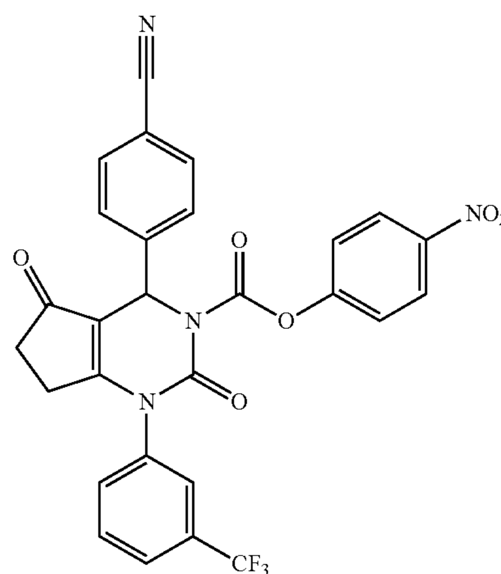
INTERMEDIATE 4
