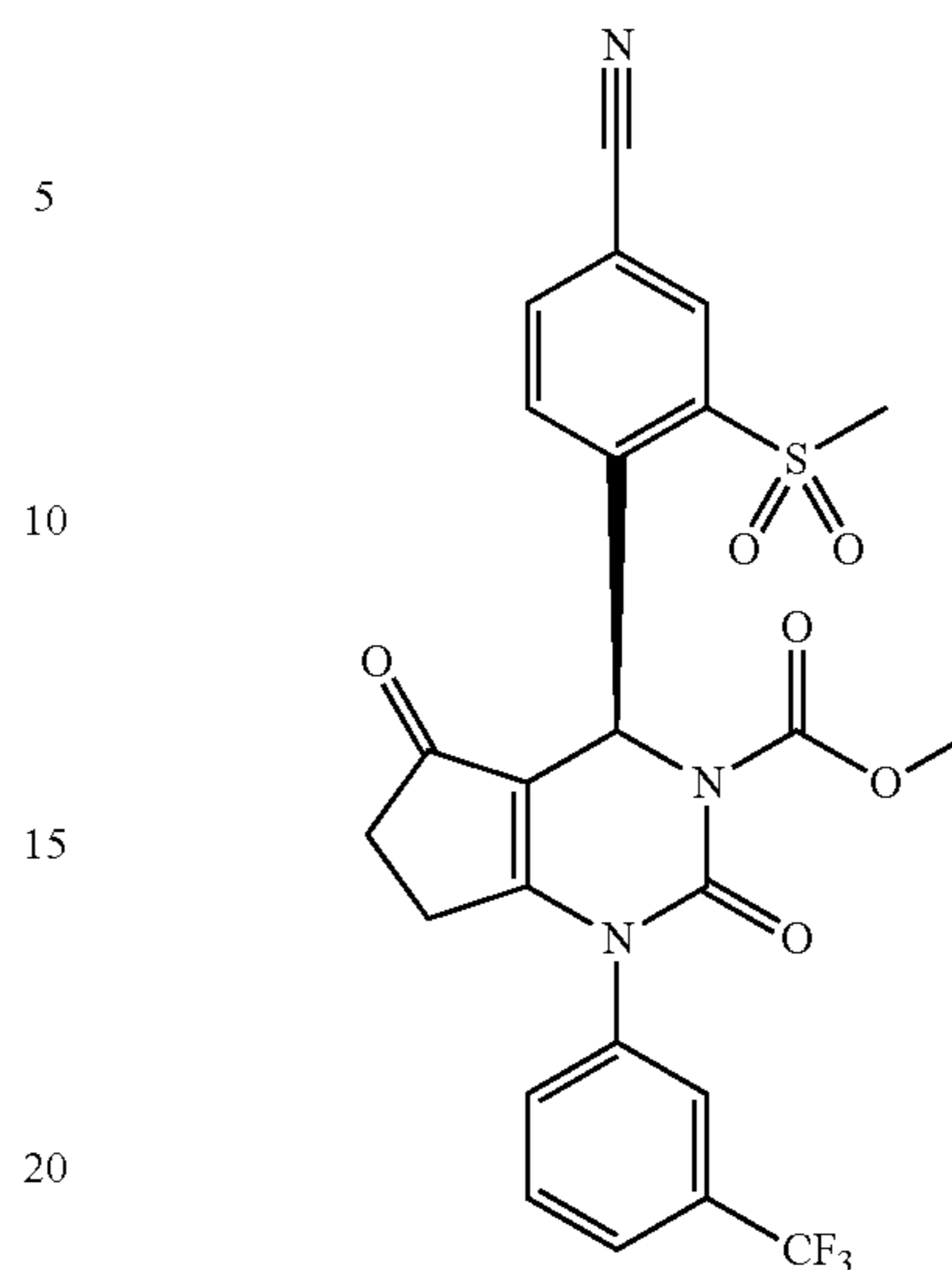
(S)-Methyl 4-(4-cyano-2-(methylsulfonyl)phenyl)-2,5-dioxo-1-(3-(trifluoromethyl)phenyl)-4,5,6,7-tetrahydro-1H-cyclopenta[d]pyrimidine-3(2H)-carboxylate
