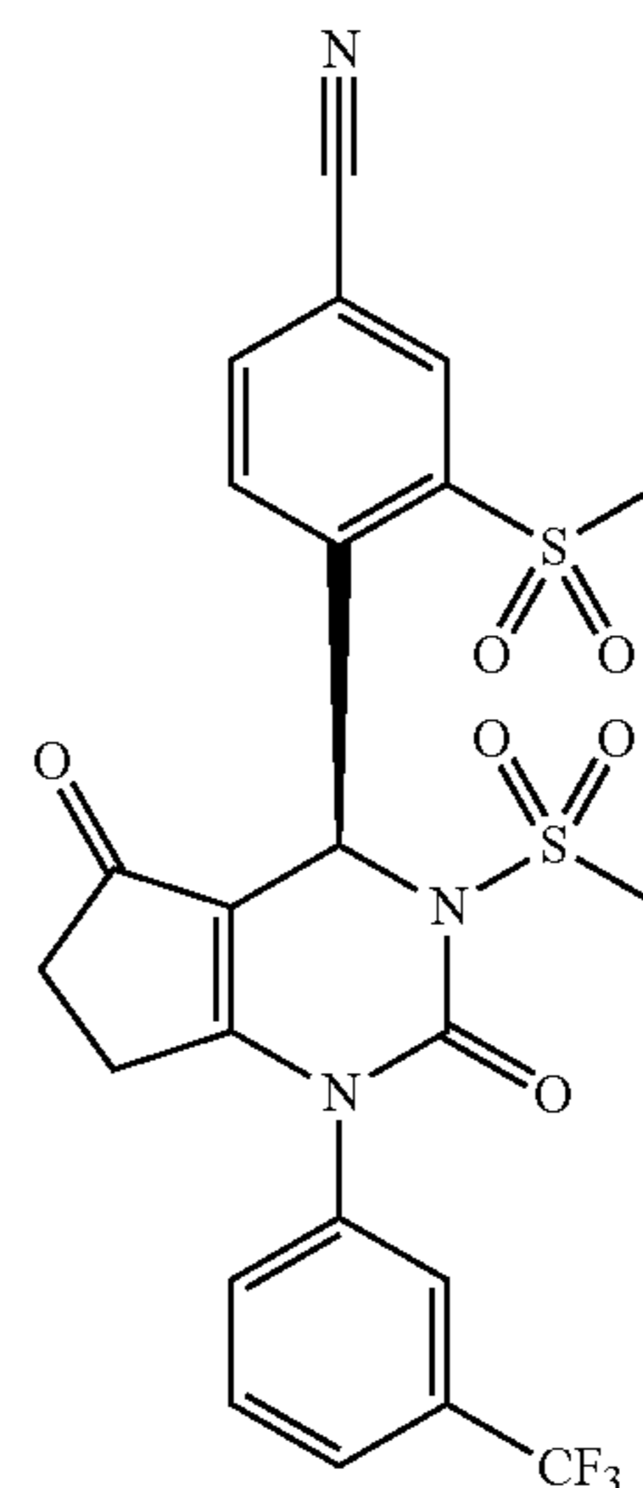
3-(Methylsulfonyl)-4-(3-(methylsulfonyl)-2,5-dioxo-1-(3-(trifluoromethyl)phenyl)-2,3,4,5,6,7-hexahydro-1H-cyclopenta[d]pyrimidin-4-yl)benzonitrile
