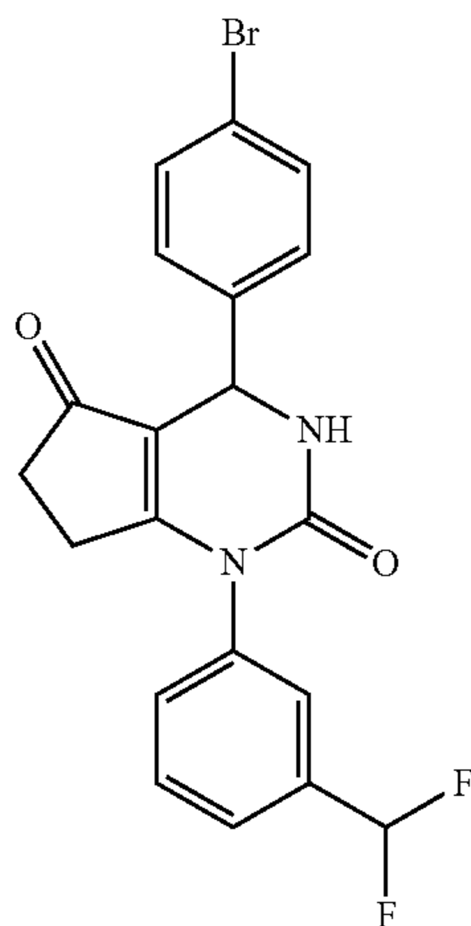
4-(4-Bromophenyl)-1-(3-(difluoromethyl)phenyl)-3,4,6,7-tetrahydro-1H-cyclopenta[d]pyrimidine-2,5-dione
