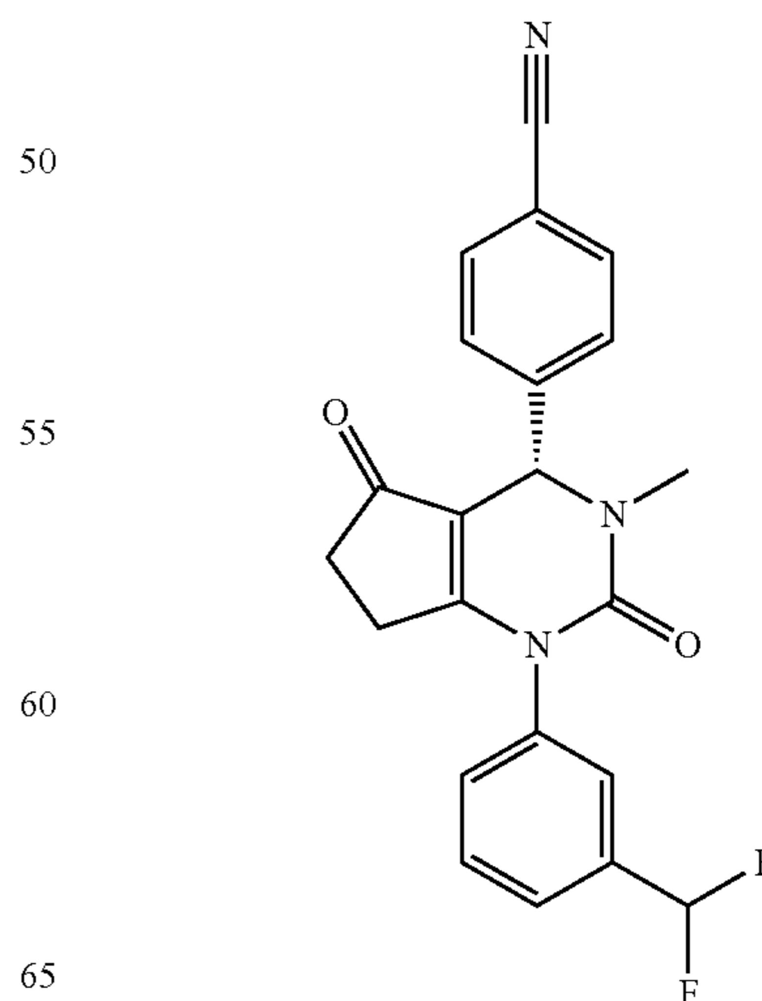
4-(1-(3-(Difluoromethyl)phenyl)-3-methyl-2,5-dioxo-2,3,4,5,6,7-hexahydro-1H-cyclopenta[d]pyrimidin-4-yl)benzonitrile
