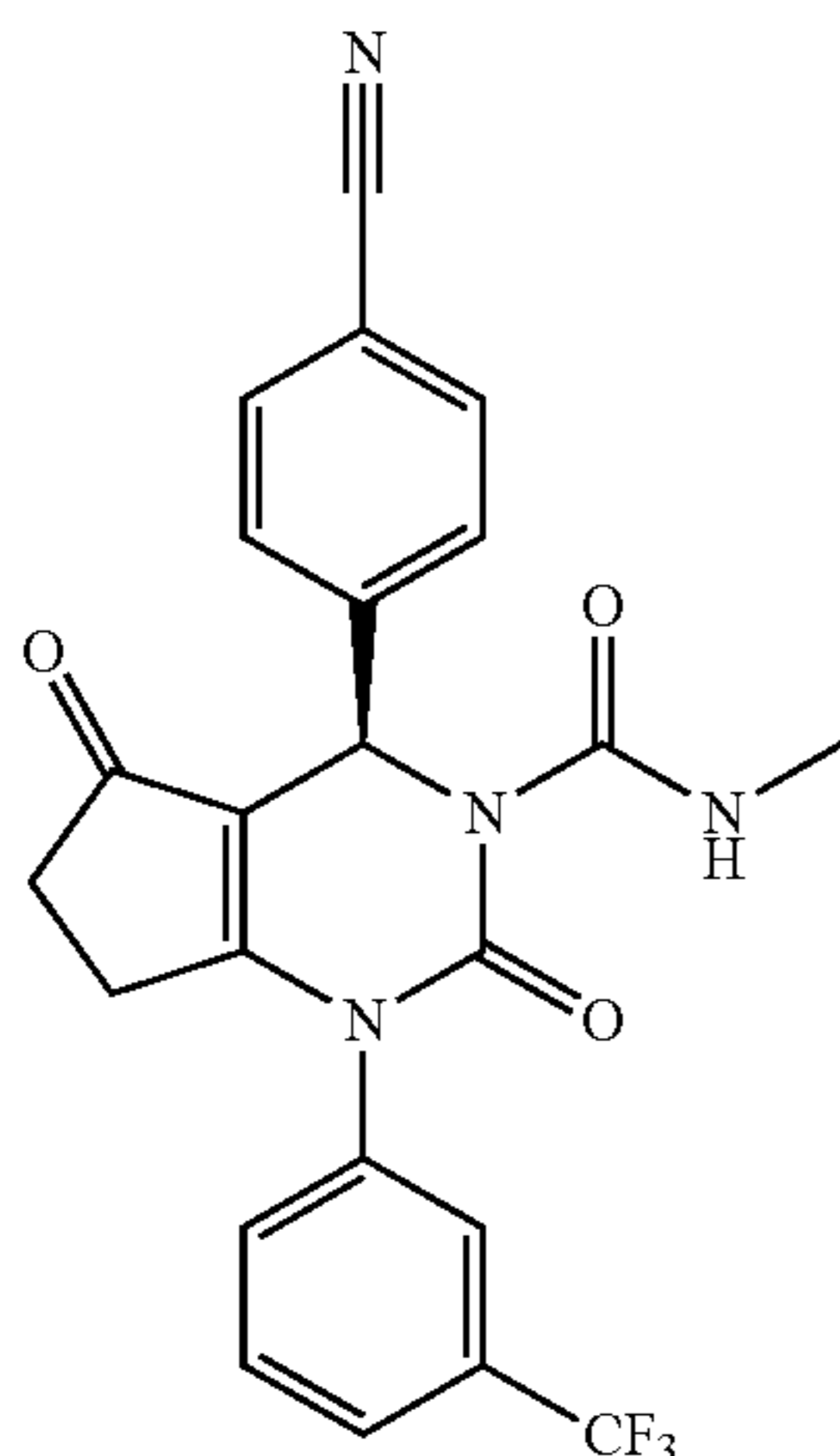
(R)-4-(4-Cyanophenyl)-N-methyl-2,5-dioxo-1-(3-(trifluoromethyl)phenyl)-4,5,6,7-tetrahydro-1H-cyclopenta[d]pyrimidine-3(2H)-carboxamide
