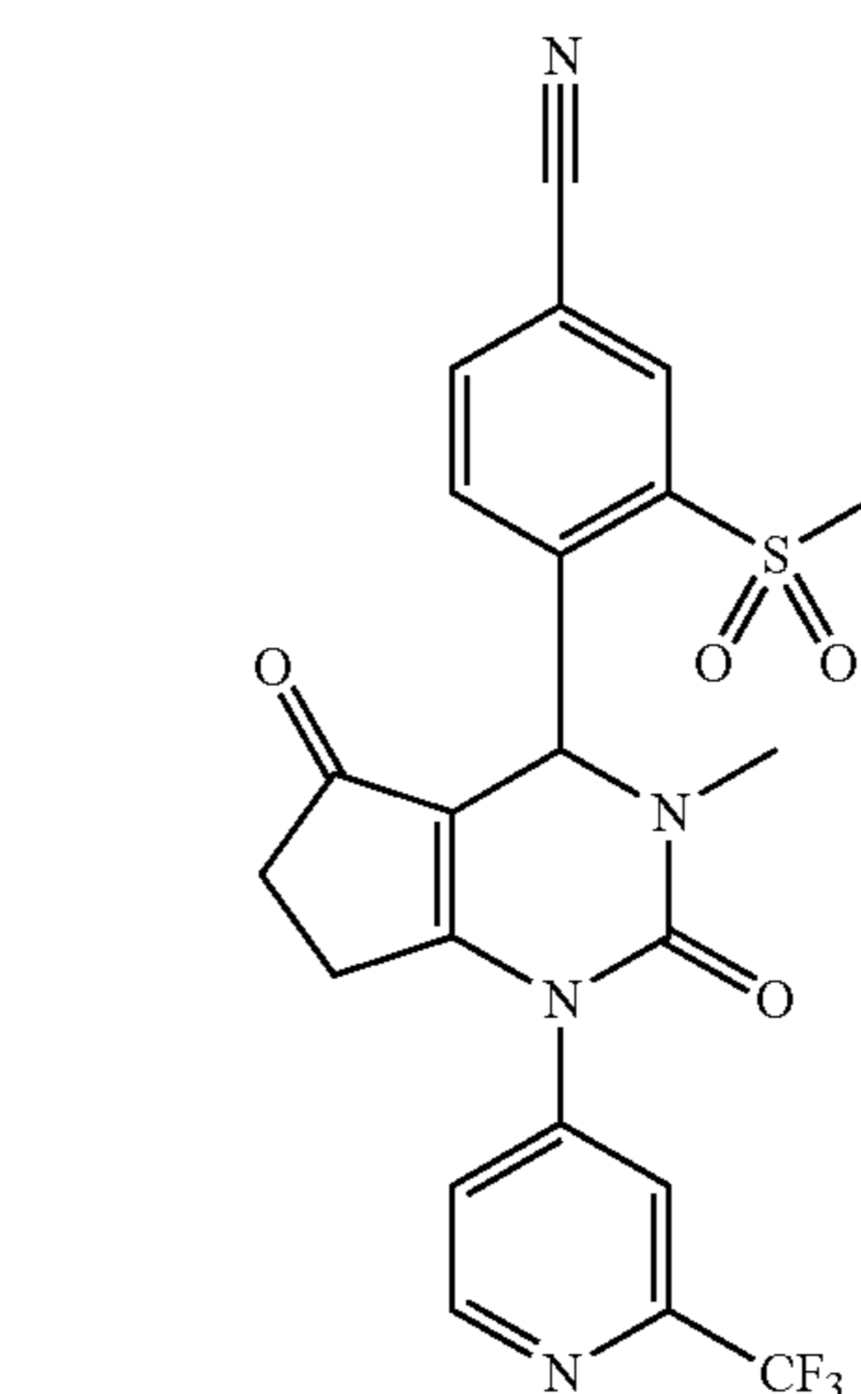
4-(3-Methyl-2,5-dioxo-1-(2-(trifluoromethyl)pyridin-4-yl)-2,3,4,5,6,7-hexahydro-1H-cyclopenta[d]pyrimidin-4-yl)-3-(methylsulfonyl)benzonitrile
