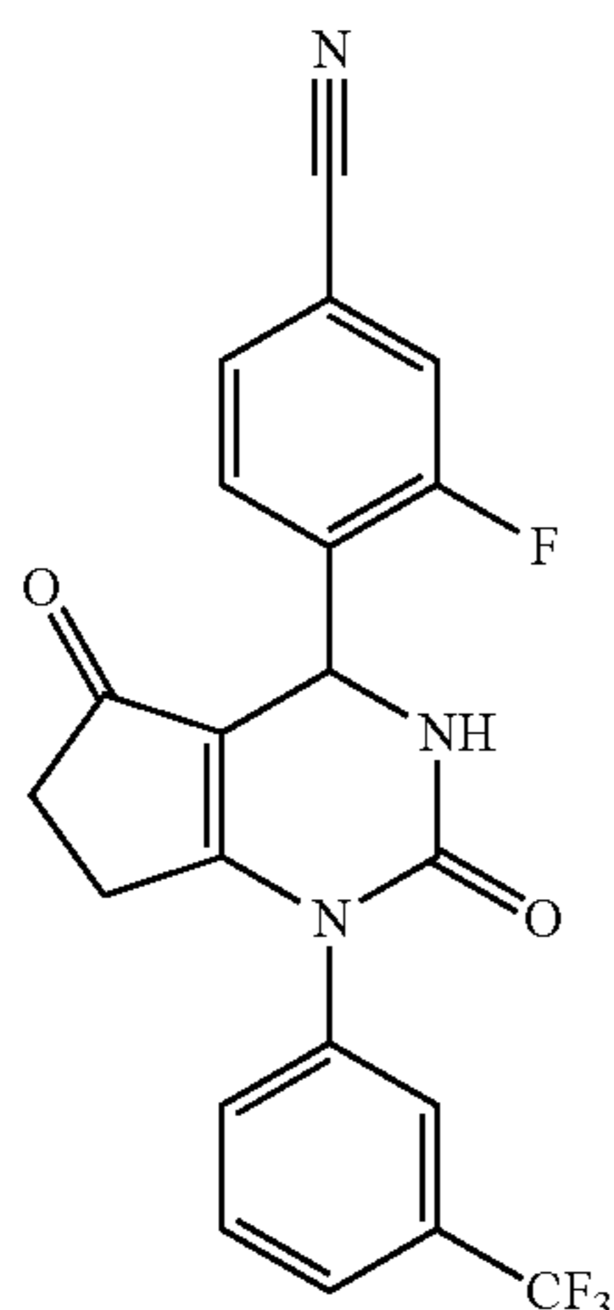
4-(2,5-Dioxo-1-(3-(trifluoromethyl)phenyl)-2,3,4,5,6,7-hexahydro-1H-cyclopenta[d]pyrimidin-4-yl)-3-fluorobenzonitrile
