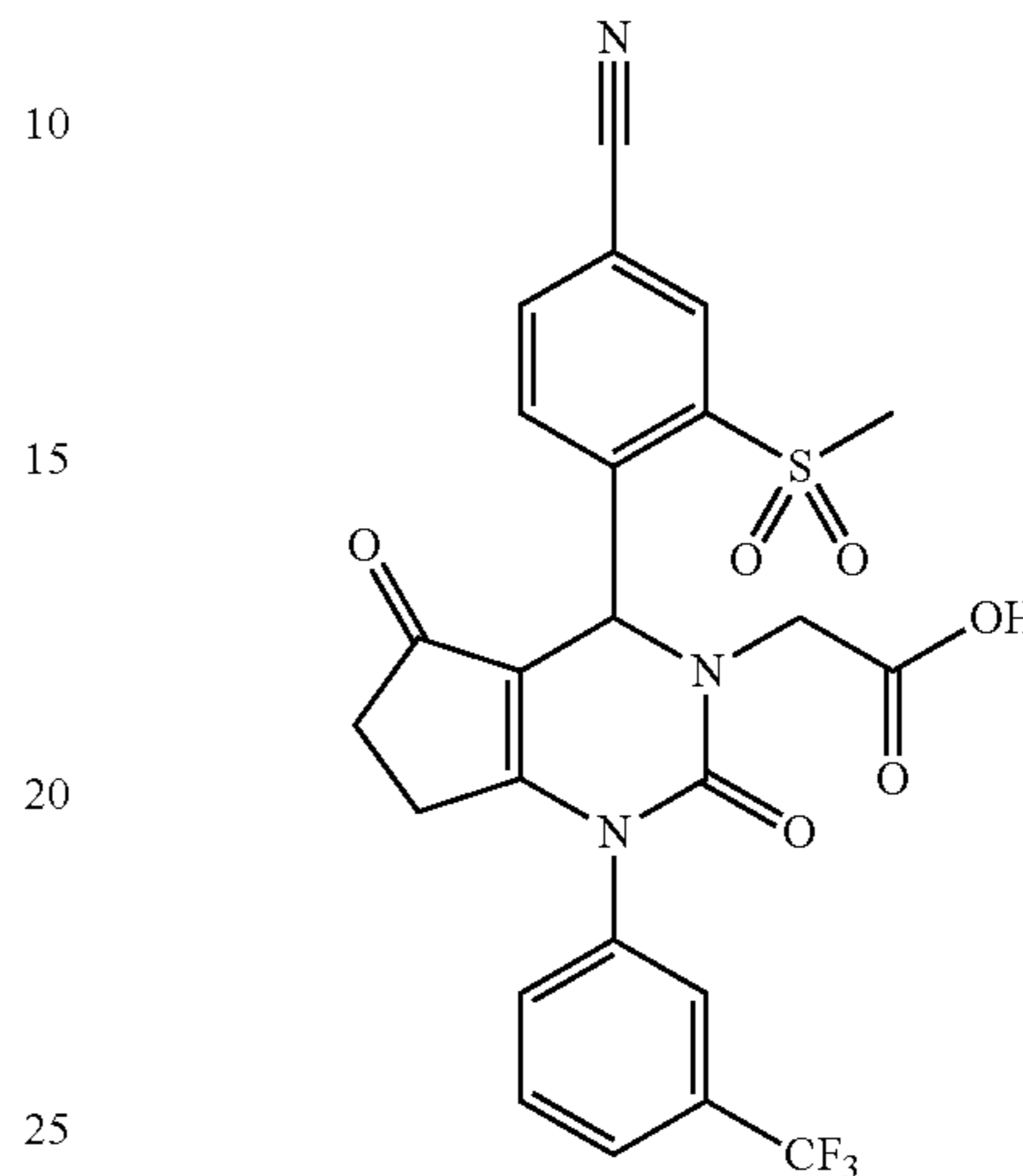
2-(4-(4-Cyano-2-(methylsulfonyl)phenyl)-2,5-dioxo-1-(3-(trifluoromethyl)phenyl)-6,7-dihydro-1H-cyclopenta[d]pyrimidin-3(2H,4H,5H)-yl)acetic acid
