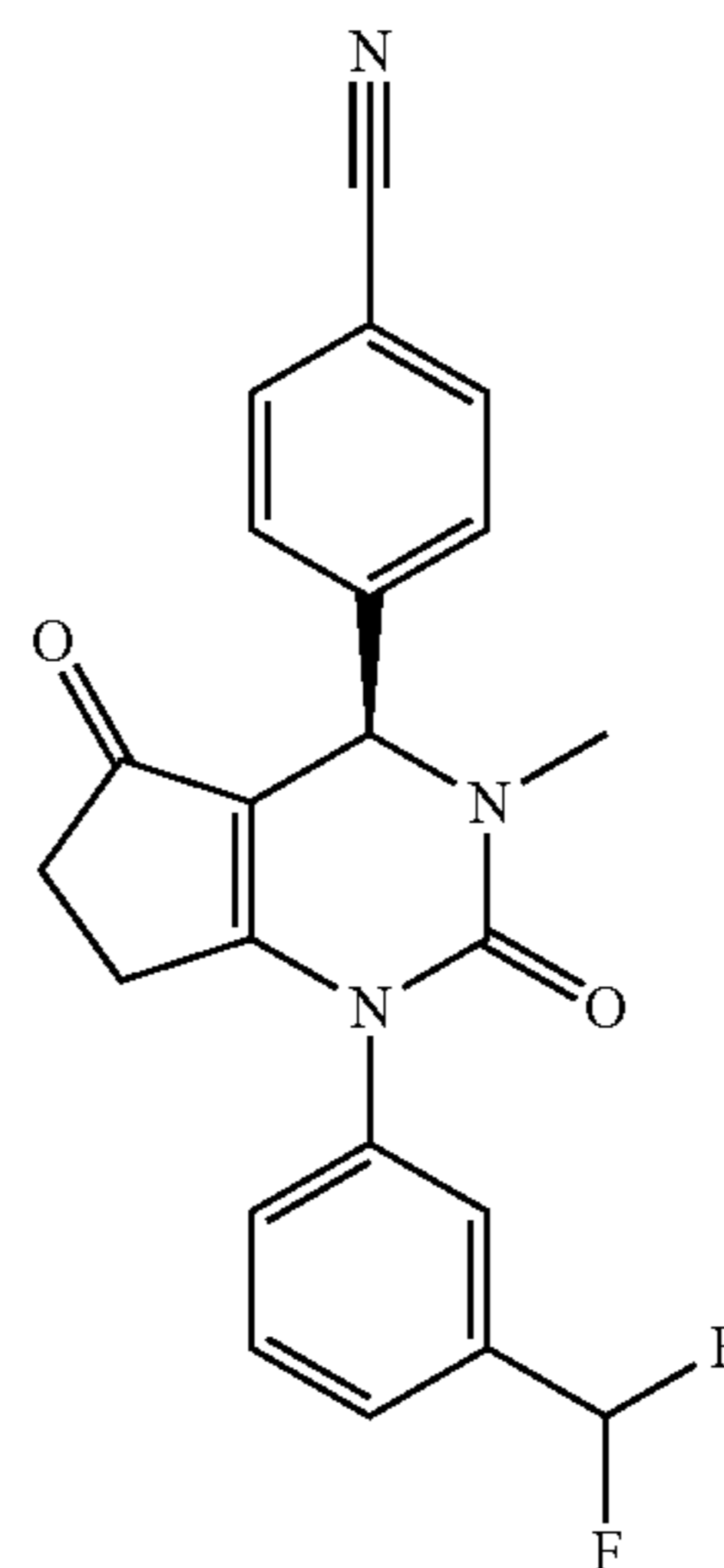
(R)-4-(1-(3-(Difluoromethyl)phenyl)-3-methyl-2,5-dioxo-2,3,4,5,6,7-hexahydro-1H-cyclopenta[d]pyrimidin-4-yl)benzonitrile
