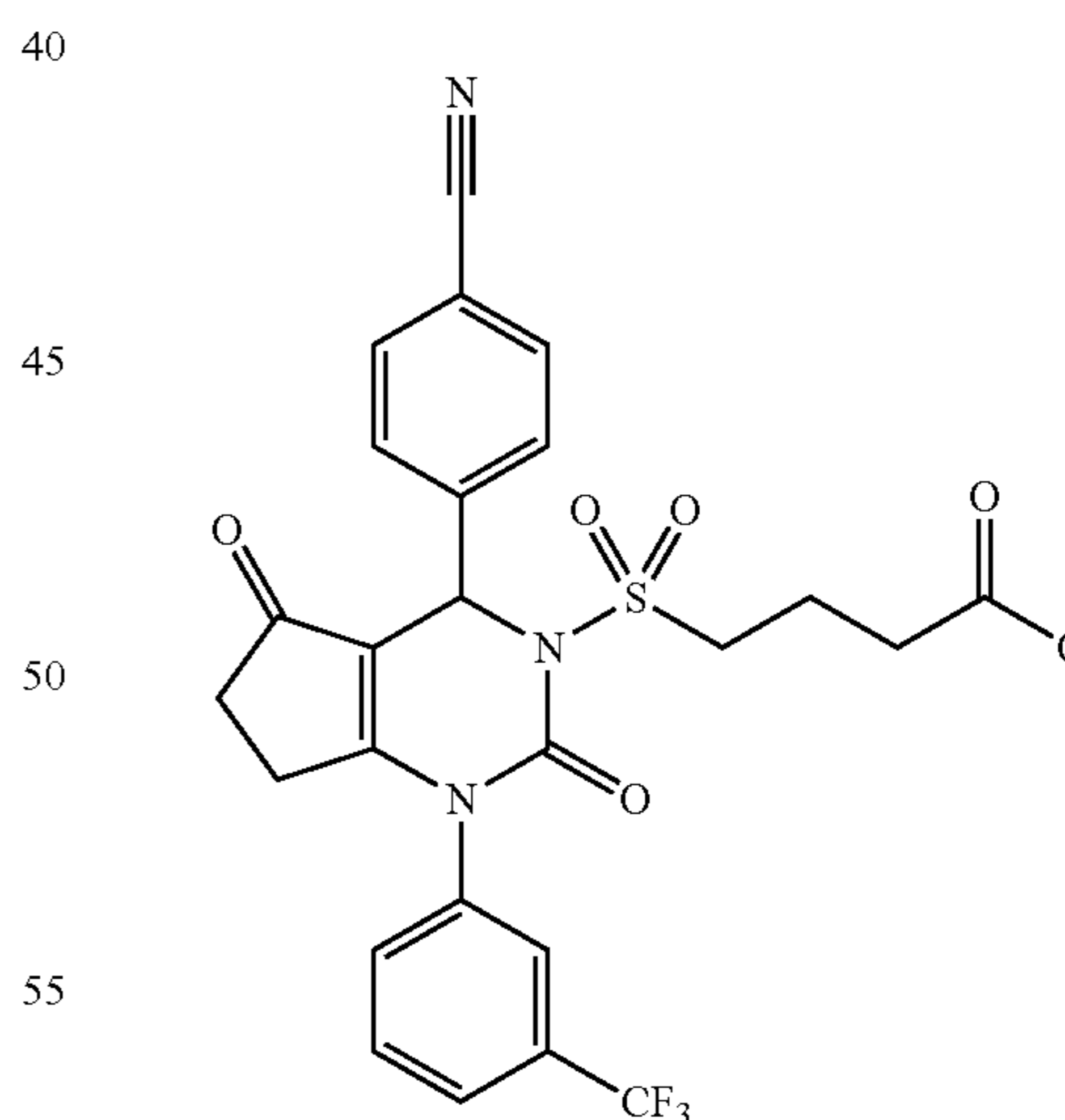
Methyl 4-(4-(4-Cyanophenyl)-2,5-dioxo-1-(3-(trifluoromethyl)phenyl)-6,7-dihydro-1H-cyclopenta[d]pyrimidin-3(2H,4H,5H)-ylsulfonyl)butanoate
