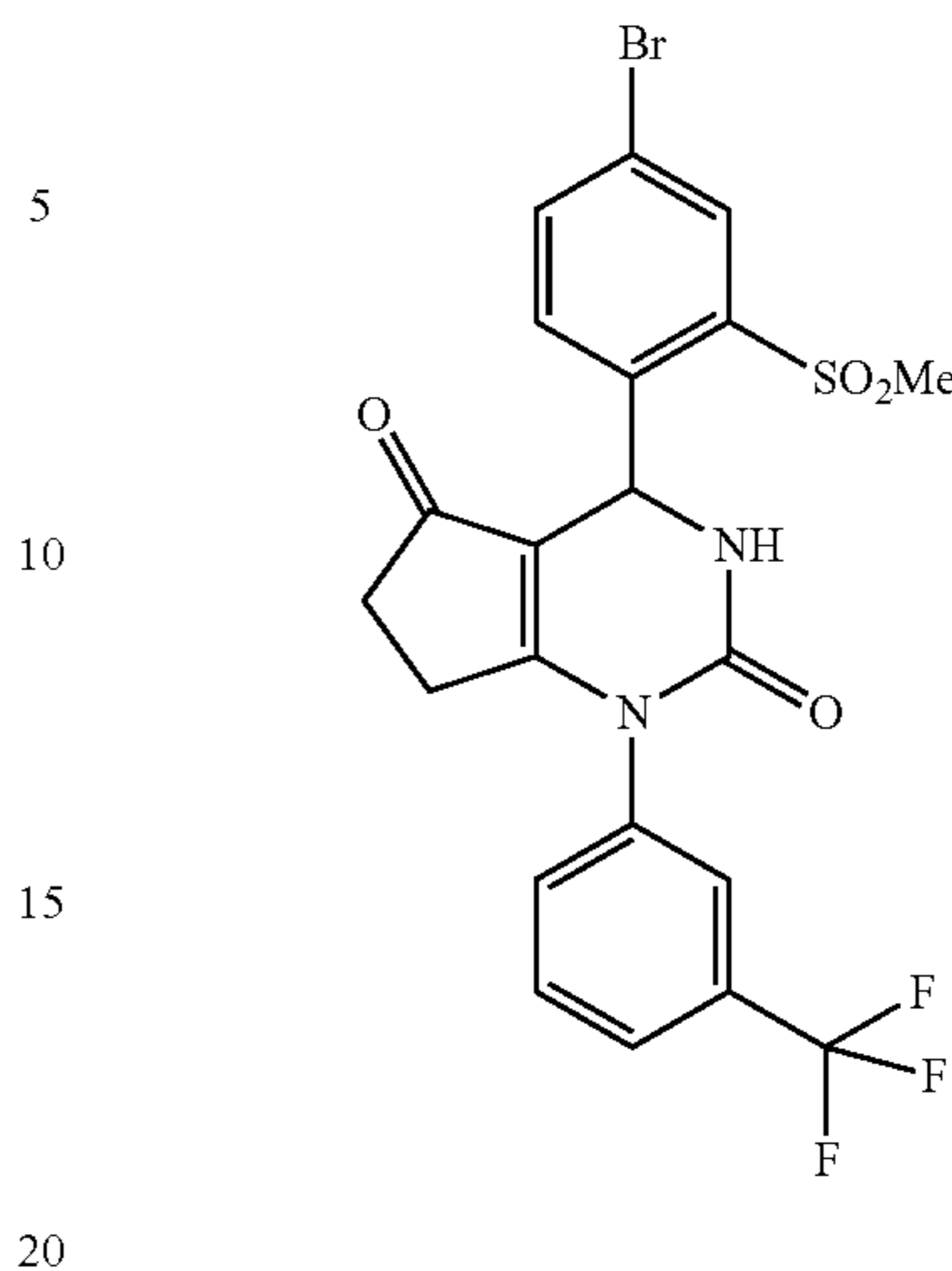
4-(4-Bromo-2-(methylsulfonyl)phenyl)-1-(3-(trifluoromethyl)phenyl)-3,4,6,7-tetrahydro-1H-cyclopenta[d]pyrimidine-2,5-dione
