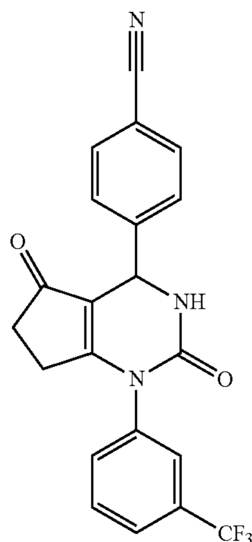
4-(2,5-Dioxo-1-(3-(trifluoromethyl)phenyl)-2,3,4,5,6,7-hexahydro-1H-cyclopenta[d]-pyrimidin-4-yl)benzotrile
