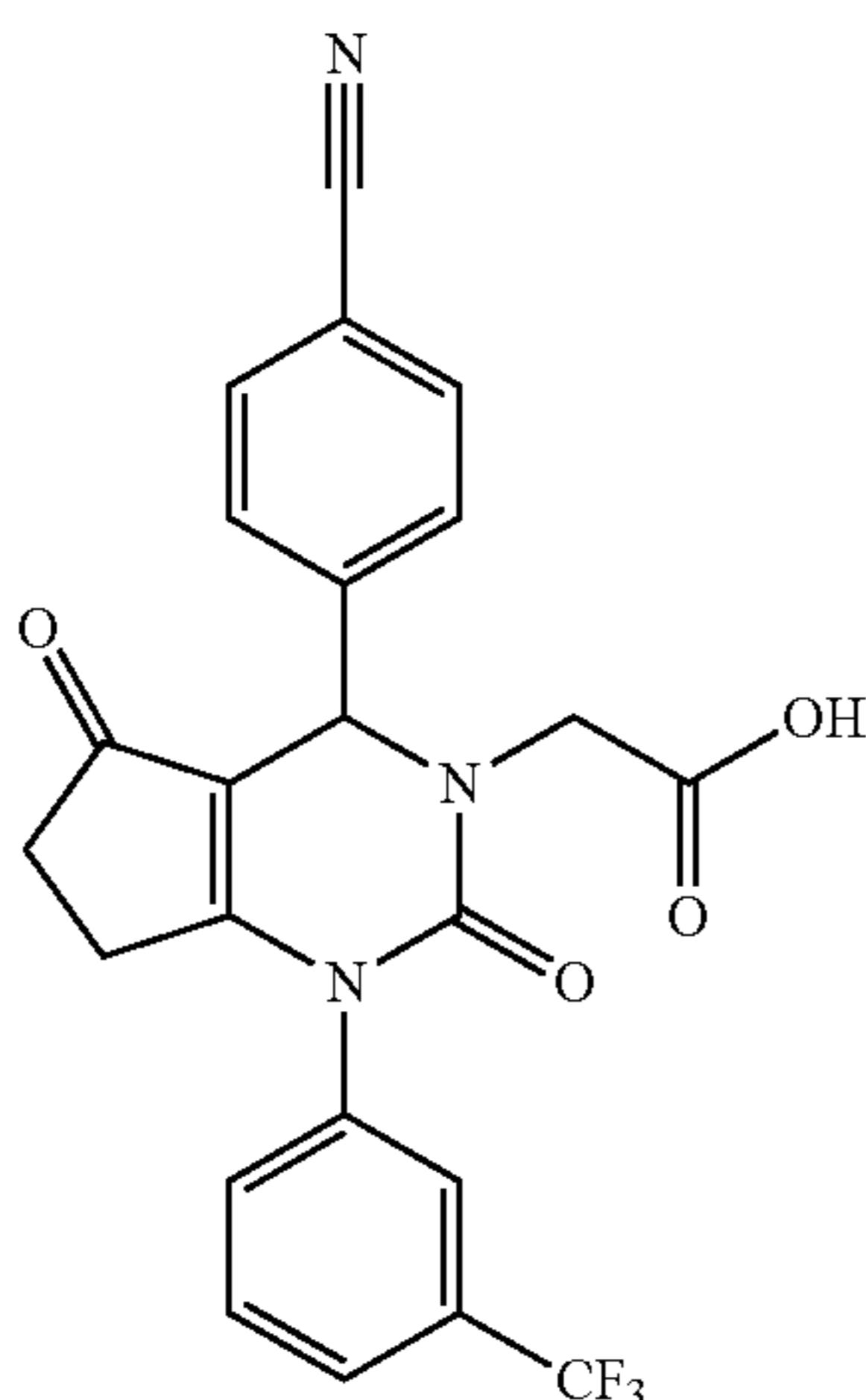
2-(4-(4-Cyanophenyl)-2,5-dioxo-1-(3-(trifluoromethyl)phenyl)-6,7-dihydro-1H-cyclopenta[d]pyrimidin-3(2H,4H,5H)-yl)acetic acid
