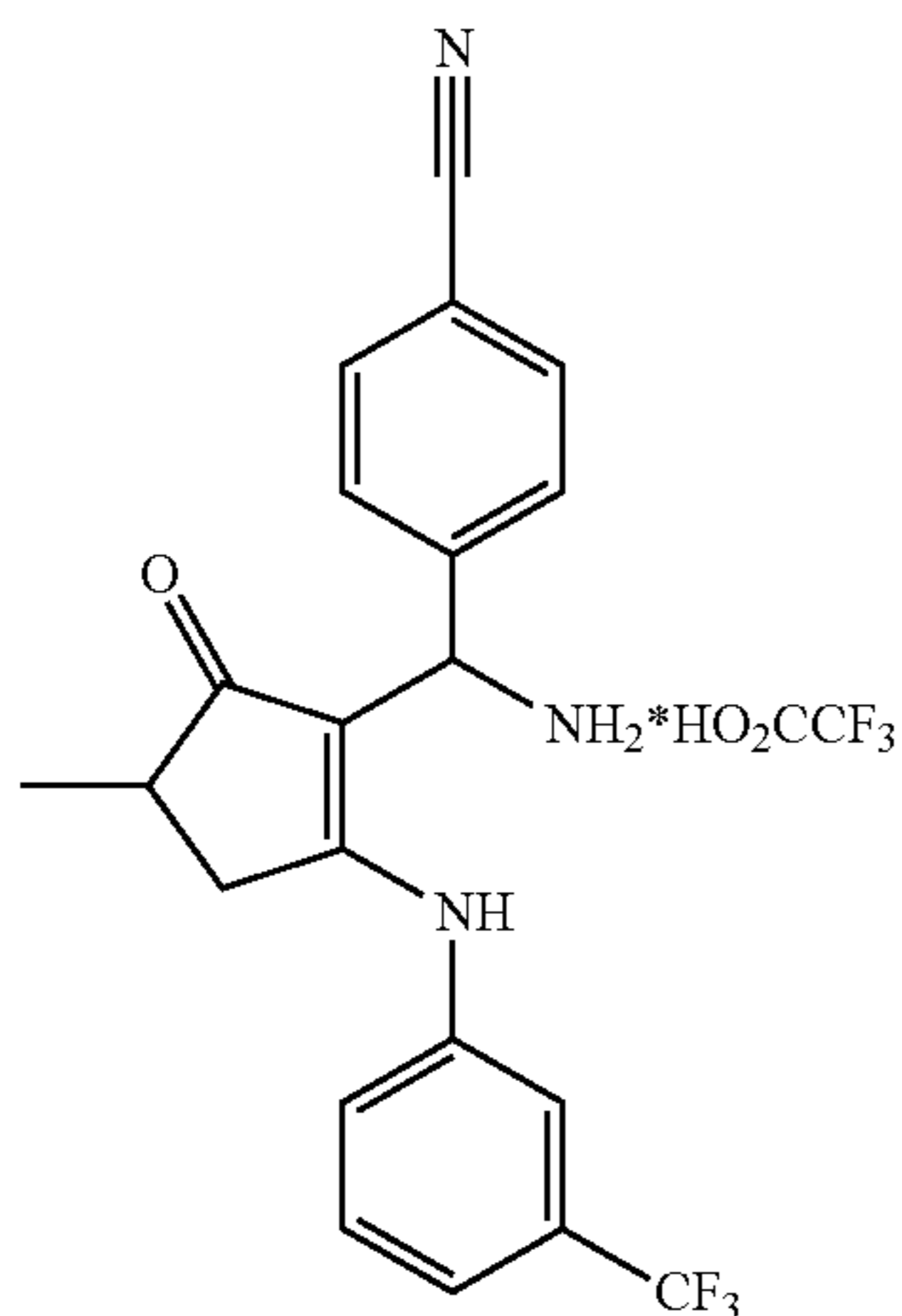
4-(Amino(4-methyl-5-oxo-2-(3-(trifluoromethyl)phenylamino)cyclopent-1-enyl)-methyl)benzotrile trifluoroacetate
